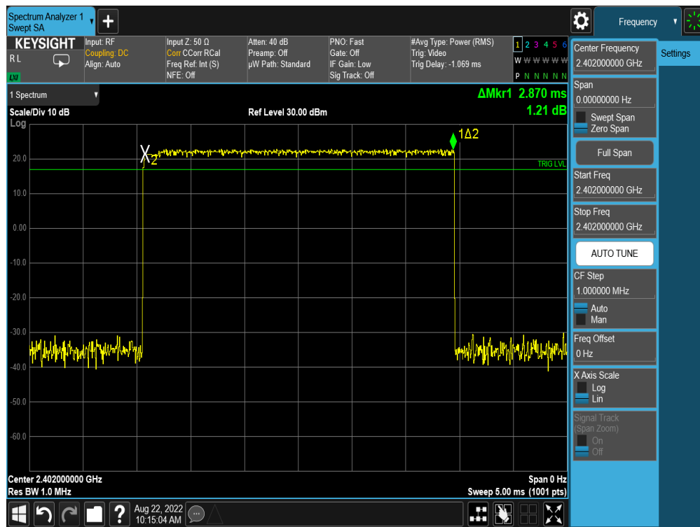
Plot 7-36. Time of Occupancy Plot (Bluetooth, 8DPSK, ePA)
