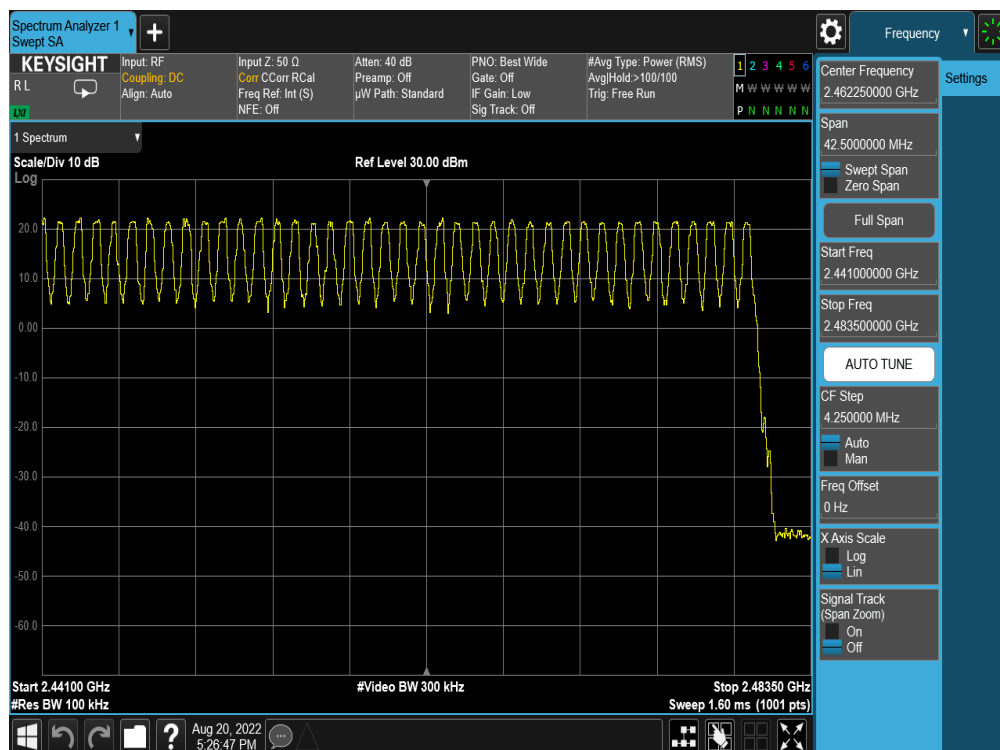
Plot 7-38. High End Spectrum Channel Hopping Plot (Bluetooth, GFSK, ePA)
