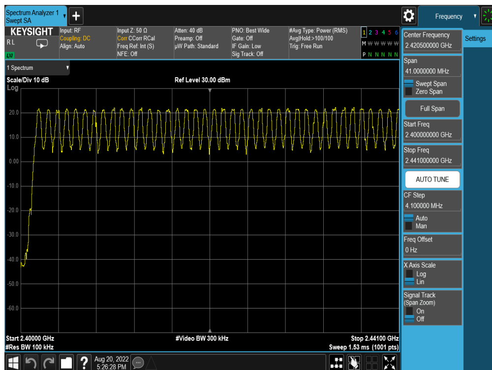
Plot 7-37. Low End Spectrum Channel Hopping Plot (Bluetooth, GFSK, ePA)
