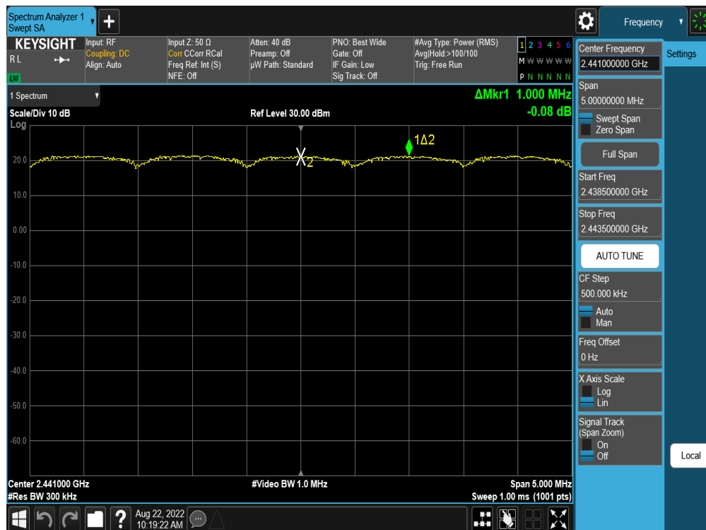
Plot 7-32. Channel Spacing Plot Antenna WF8 (Bluetooth, 8DPSK, ePA)
