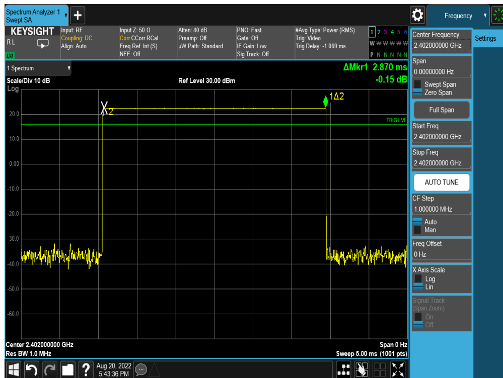
Plot 7-35. Time of Occupancy (Bluetooth, GFSK, ePA)
