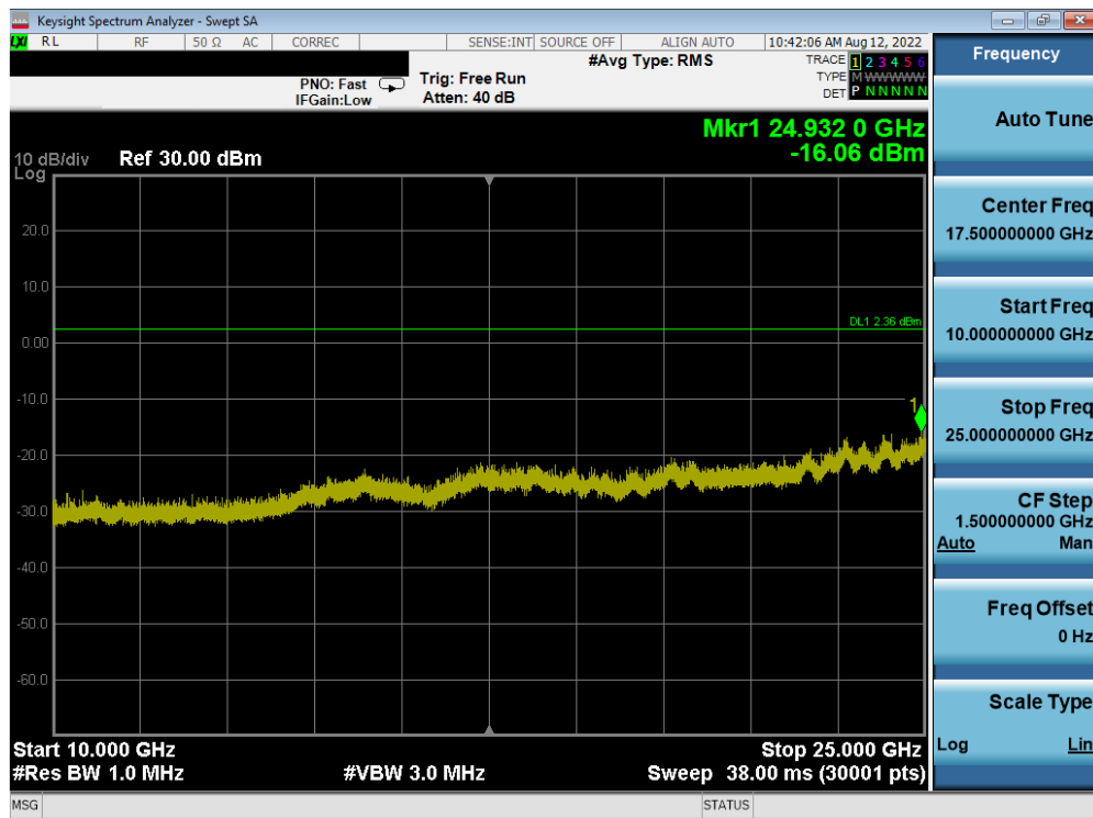
Plot 7-50. Conducted Spurious Plot (Bluetooth, GFSK, ePA – Ch. 78)
