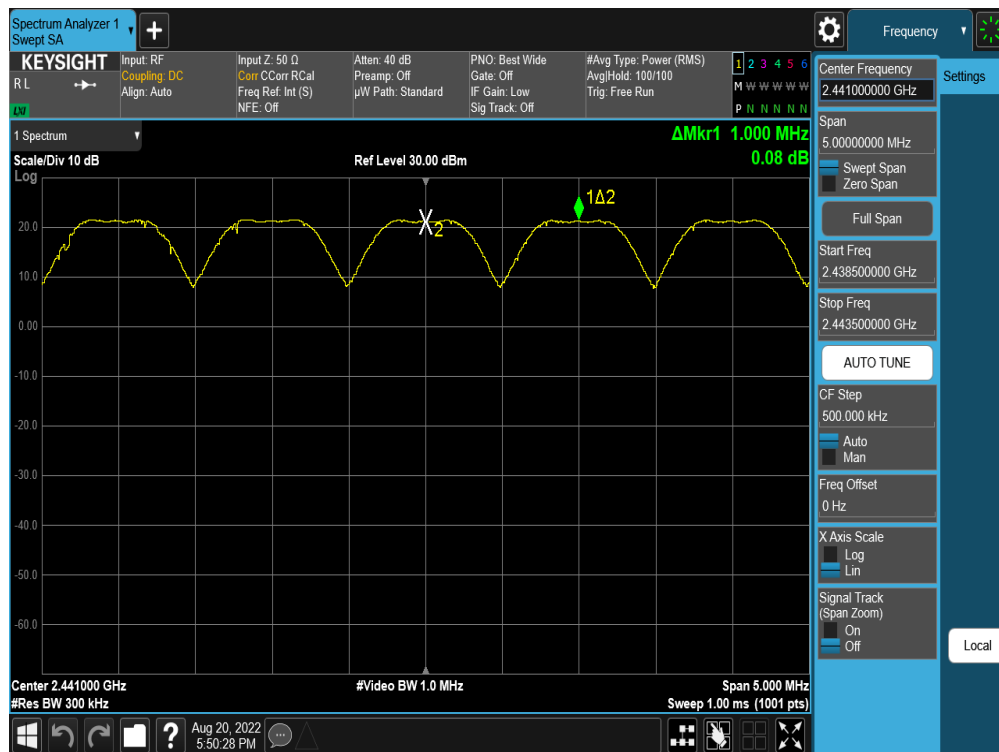
Plot 7-31. Channel Spacing Plot Antenna WF8 (Bluetooth, GFSK, ePA)
