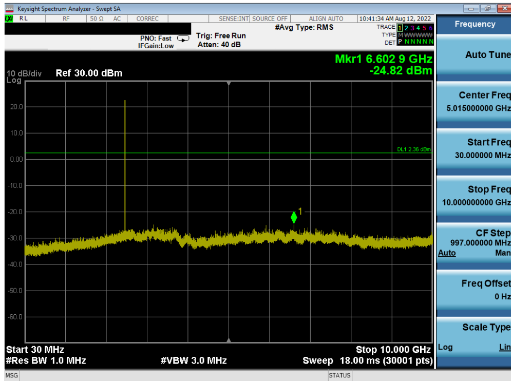
Plot 7-49. Conducted Spurious Plot (Bluetooth, GFSK, ePA – Ch. 78)
