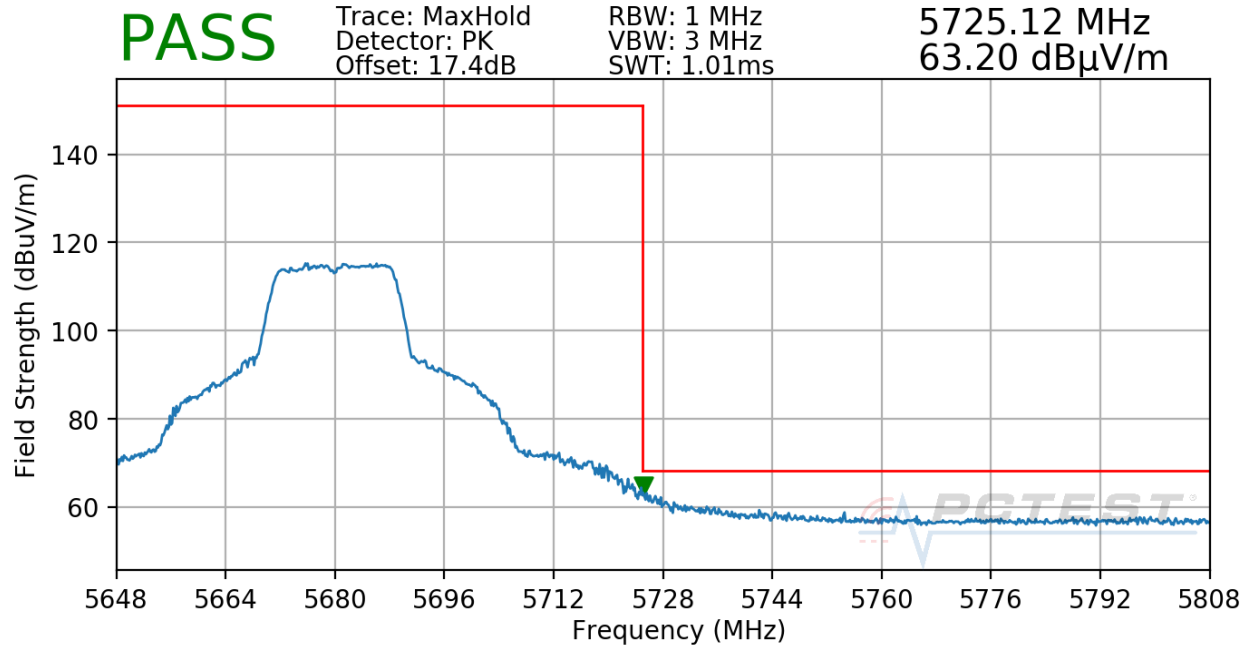
Plot 7-140. Antenna A (Pk, Ch.136, 802.11n, MCS7)
