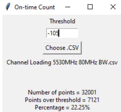
Figure 9-18. 5530MHz - Channel Loading Calculation - Mode 3 (80MHz)
