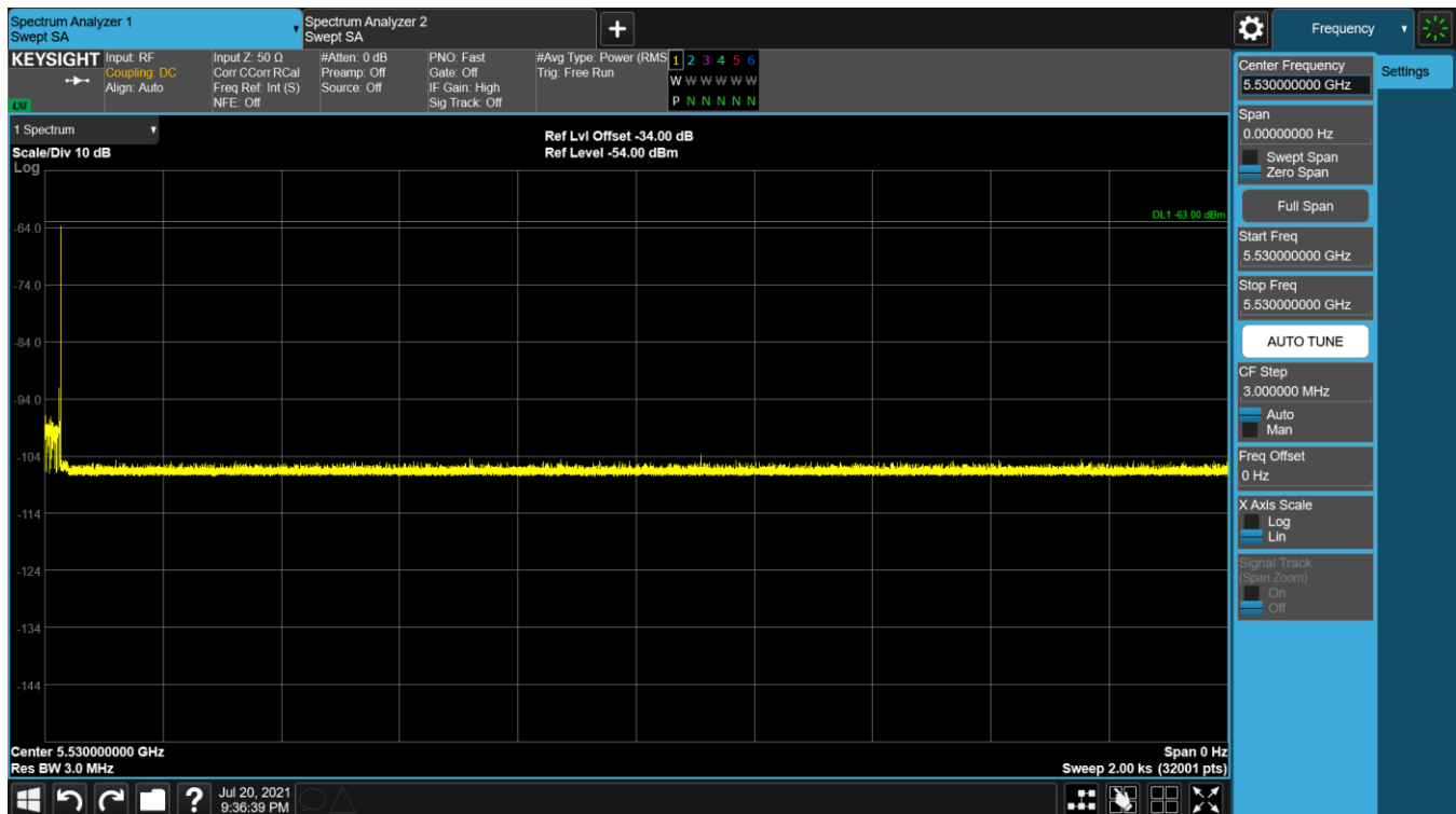
Figure 9-45. 5530MHz - Non-Occupancy Period (30 Minutes) - Mode 3 (80MHz)
