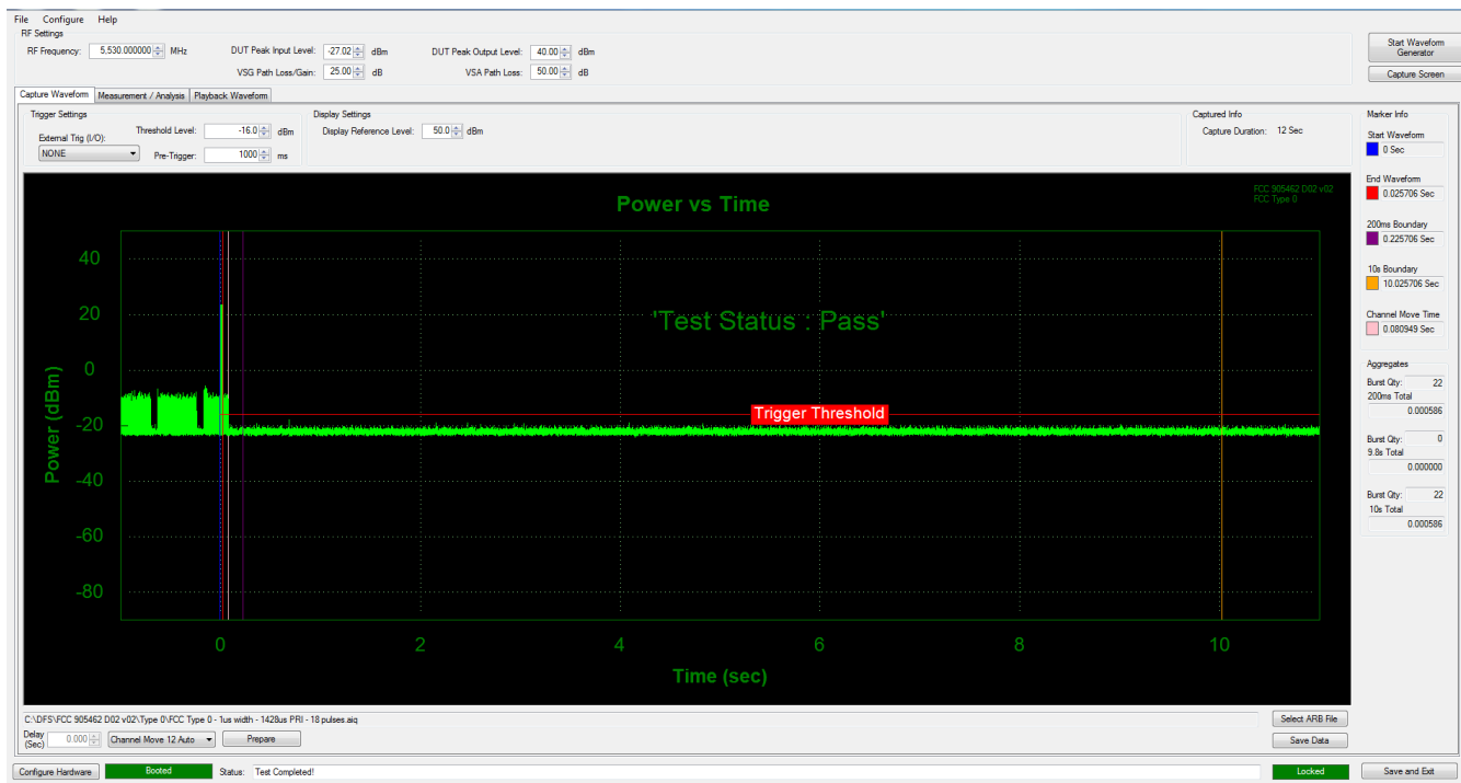
Figure 9-33. 5530MHz - Channel Move/ Closing Transmission Time - Mode 3 (80 MHz)
