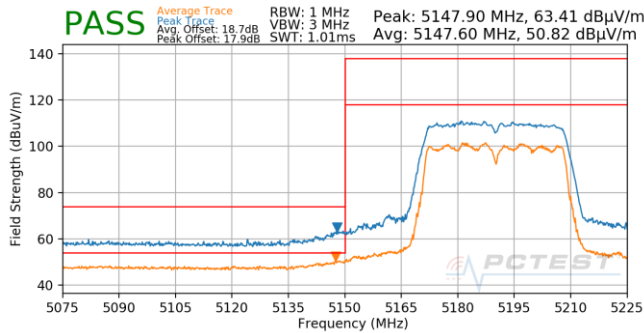
Plot 7-994. CDD (Pk & Avg, Ch.38, 802.11n, MCS13)
