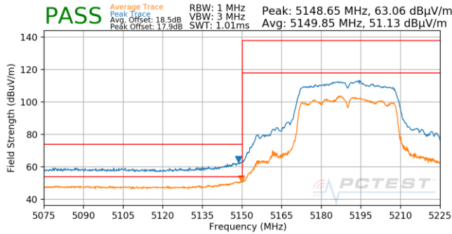
Plot 7-993. CDD (Pk & Avg, Ch.38, 802.11n, MCS11)
