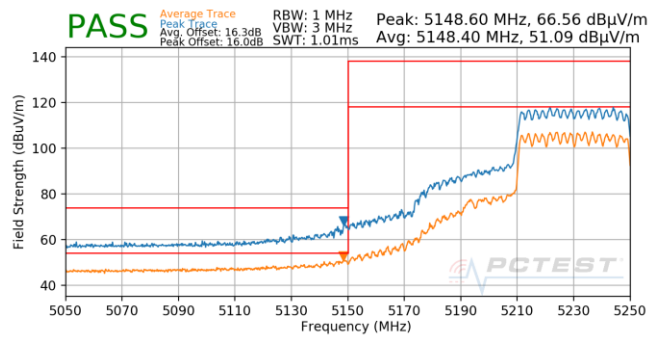
Plot 7-1026. SDM (Pk & Avg, Ch.46, 802.11ax(SU), MCS3)
