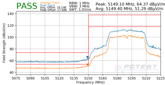
Plot 7-992. CDD (Pk & Avg, Ch.38, 802.11n, MCS8)
