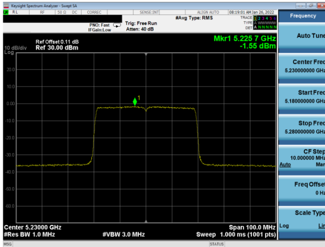
Plot 7-476. ISED SDM PSD Antenna WF7a (40MHz BW 11ax(SU) – Ch.46, MCS0)
