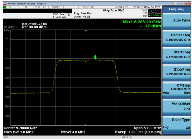
Plot 7-496. ISED PSD SDM Antenna WF7a (20MHz BW 11ax(SU) – Ch.40, MCS5)
