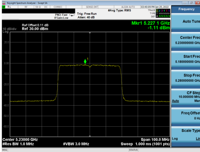
Plot 7-475. ISED PSD SDM Antenna WF8 (40MHz BW 11ax(SU) – Ch.46, MCS0)
