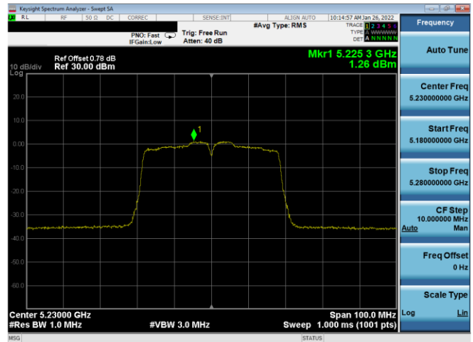
Plot 7-497. ISED PSD SDM Antenna WF8 (40MHz BW 11n – Ch.46, MCS13)
