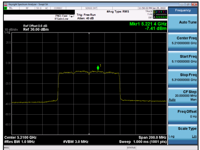
Plot 7-371. PSD CDD Antenna WF8 (80MHz BW 802.11ax(SU) – Ch. 42, MCS3)
