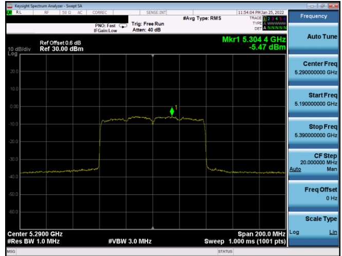
Plot 7-383. PSD CDD Antenna WF8 (80MHz BW 802.11ax(SU) – Ch. 58, MCS3)
