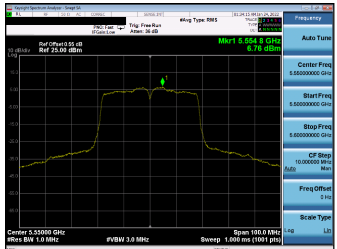
Plot 7-390. PSD SDM Antenna WF7a (40MHz BW 802.11n – Ch. 110, MCS11)
