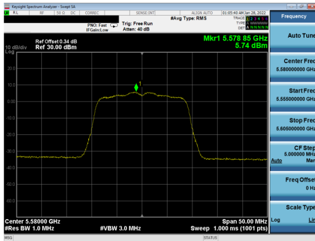
Plot 7-386. PSD SDM Antenna WF7a (20MHz BW 802.11n – Ch. 116, MCS11)
