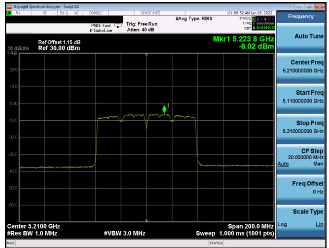
Plot 7-406. PSD CDD Antenna WF7a (80MHz BW 802.11ac – Ch. 42, MCS5)
