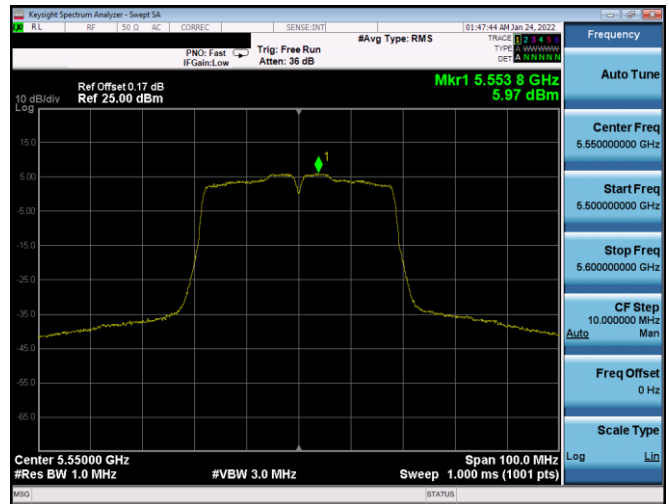
Plot 7-354. PSD SDM Antenna WF7a (40MHz BW 802.11n – Ch. 110, MCS8)
