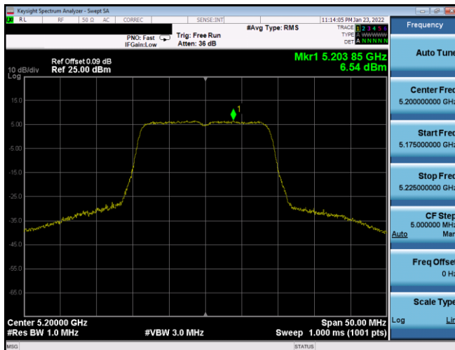
Plot 7-398. PSD SDM Antenna WF7a (20MHz BW 802.11n – Ch. 40, MCS13)
