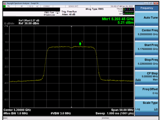
Plot 7-400. PSD SDM Antenna WF7a (20MHz BW 802.11ax(SU) – Ch. 40, MCS5)
