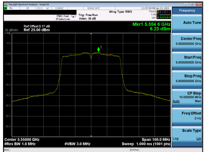
Plot 7-353. PSD SDM Antenna WF8 (40MHz BW 802.11n – Ch. 110, MCS8)
