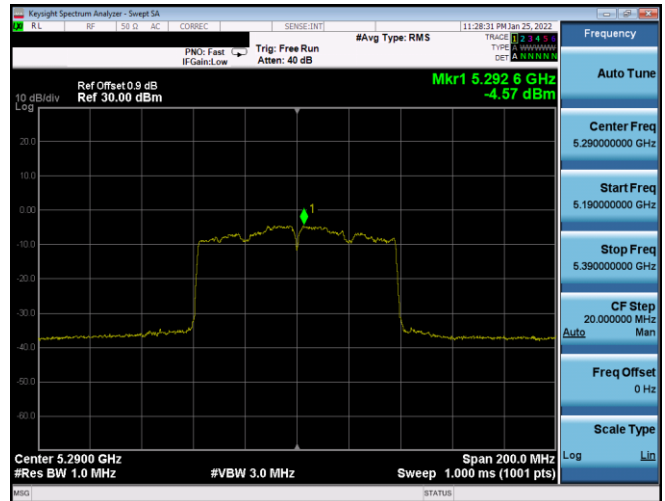
Plot 7-382. PSD CDD Antenna WF7a (80MHz BW 802.11ac – Ch. 58, MCS3)
