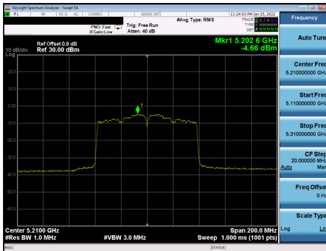
Plot 7-369. PSD CDD Antenna WF8 (80MHz BW 802.11ac – Ch. 42, MCS3)
