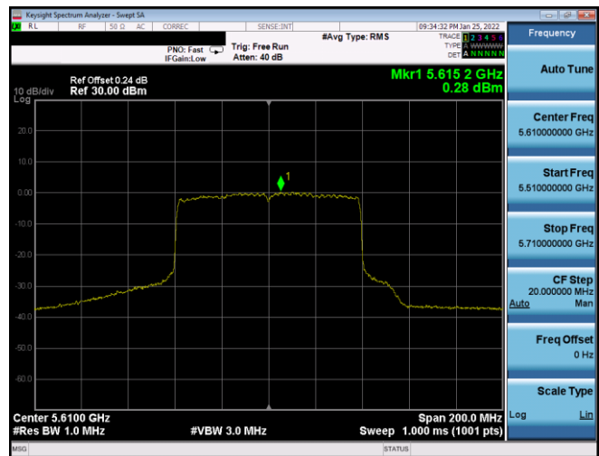
Plot 7-359. PSD CDD Antenna WF8 (80MHz BW 802.11ax(SU) – Ch. 122, MCS0)
