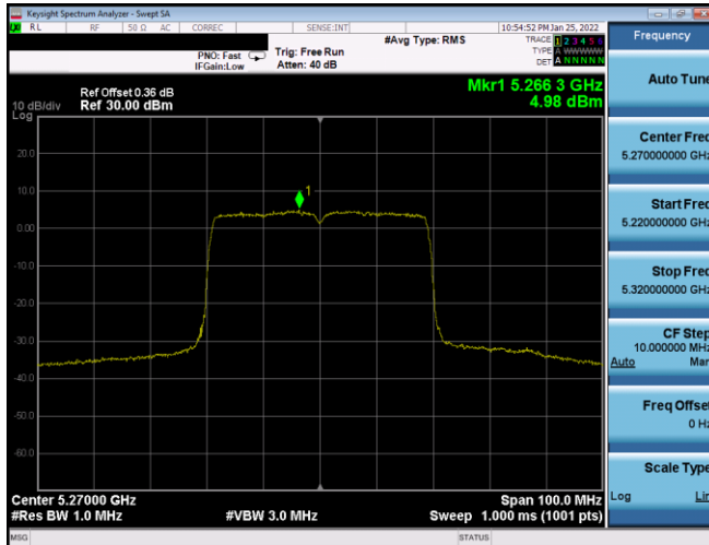
Plot 7-380. PSD SDM Antenna WF7a (40MHz BW 802.11ax(SU) – Ch. 54, MCS3)
