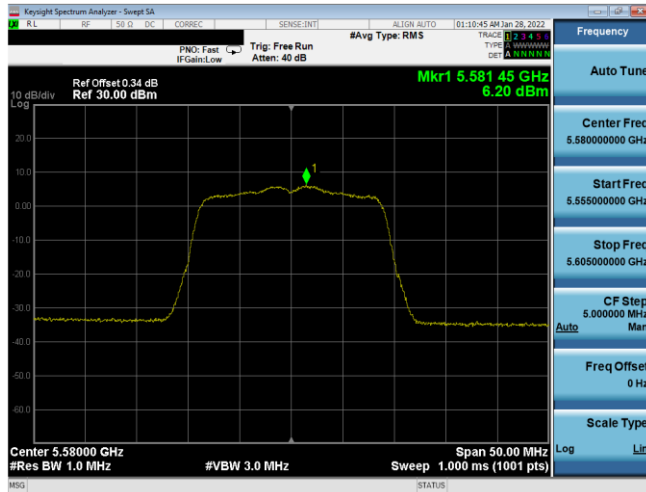
Plot 7-385. PSD SDM Antenna WF8 (20MHz BW 802.11n – Ch. 116, MCS11)
