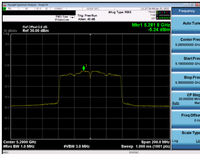
Plot 7-381. PSD CDD Antenna WF8 (80MHz BW 802.11ac – Ch. 58, MCS3)
