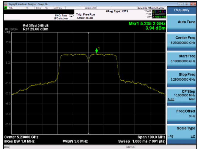
Plot 7-401. PSD SDM Antenna WF8 (40MHz BW 802.11n – Ch. 46, MCS13)
