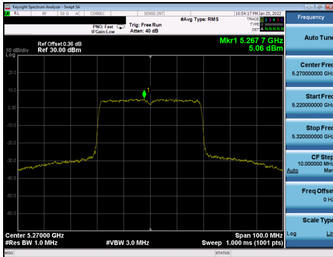
Plot 7-379. PSD SDM Antenna WF8 (40MHz BW 802.11ax(SU) – Ch. 54, MCS3)
