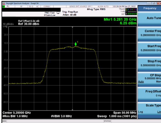
Plot 7-373. PSD SDM Antenna WF8 (20MHz BW 802.11n – Ch. 56, MCS11)
