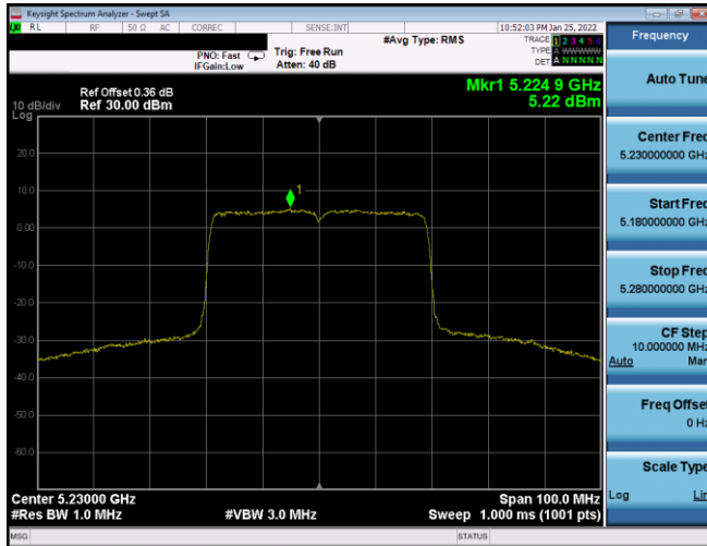
Plot 7-368. PSD SDM Antenna WF7a (40MHz BW 802.11ax(SU) – Ch. 46, MCS3)
