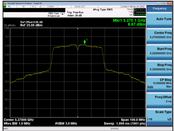
Plot 7-377. PSD SDM Antenna WF8 (40MHz BW 802.11n – Ch. 54, MCS11)
