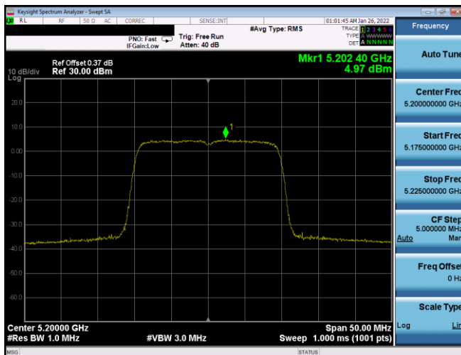
Plot 7-399. PSD SDM Antenna WF8 (20MHz BW 802.11ax(SU) – Ch. 40, MCS5)
