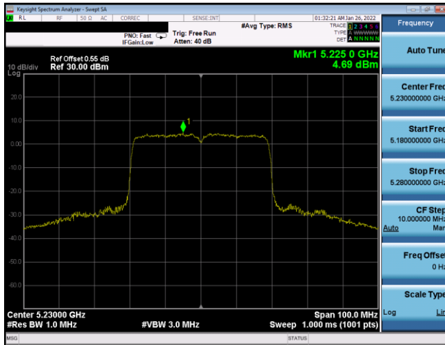
Plot 7-403. PSD SDM Antenna WF8 (40MHz BW 802.11ax(SU) – Ch. 46, MCS5)
