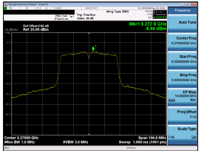
Plot 7-378. PSD SDM Antenna WF7a (40MHz BW 802.11n – Ch. 54, MCS11)
