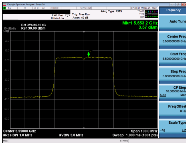
Plot 7-355. PSD SDM Antenna WF8 (40MHz BW 802.11ax(SU) – Ch. 110, MCS0)
