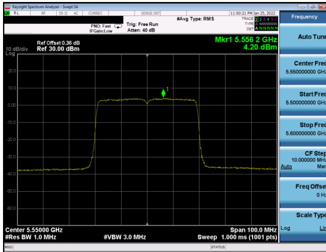
Plot 7-392. PSD CDD Antenna WF7a (40MHz BW 802.11ax(SU) – Ch. 110, MCS3)
