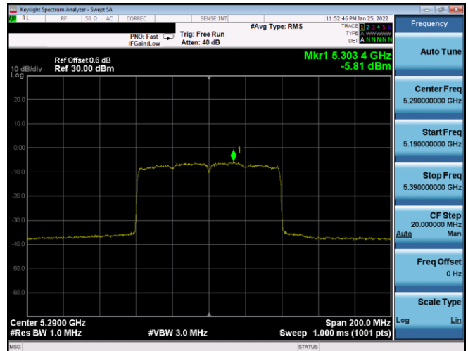
Plot 7-384. PSD CDD Antenna WF7a (80MHz BW 802.11ax(SU) – Ch. 58, MCS3)
