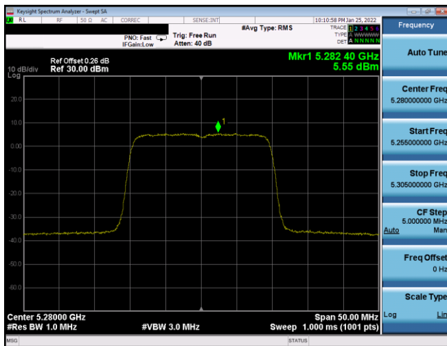
Plot 7-375. PSD SDM Antenna WF8 (20MHz BW 802.11ax(SU) – Ch. 56, MCS3)
