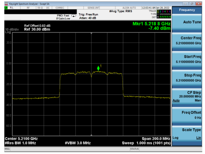
Plot 7-408. PSD CDD Antenna WF7a (80MHz BW 802.11ax(SU) – Ch. 42, MCS5)
