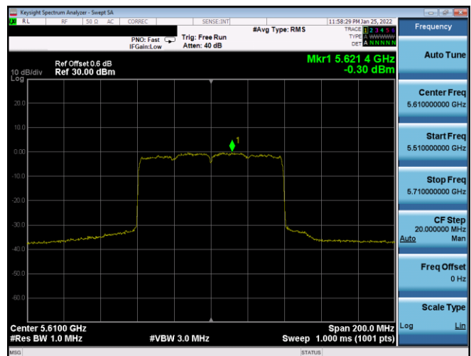
Plot 7-396. PSD CDD Antenna WF7a (80MHz BW 802.11ax(SU) – Ch. 122, MCS3)
