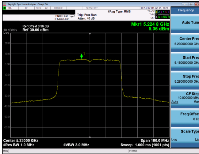
Plot 7-367. PSD SDM Antenna WF8 (40MHz BW 802.11ax(SU) – Ch. 46, MCS3)
