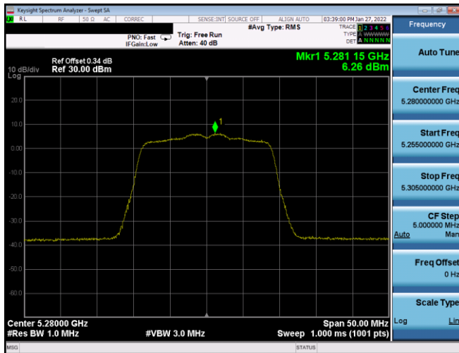
Plot 7-374. PSD SDM Antenna WF7a (20MHz BW 802.11n – Ch. 56, MCS11)
