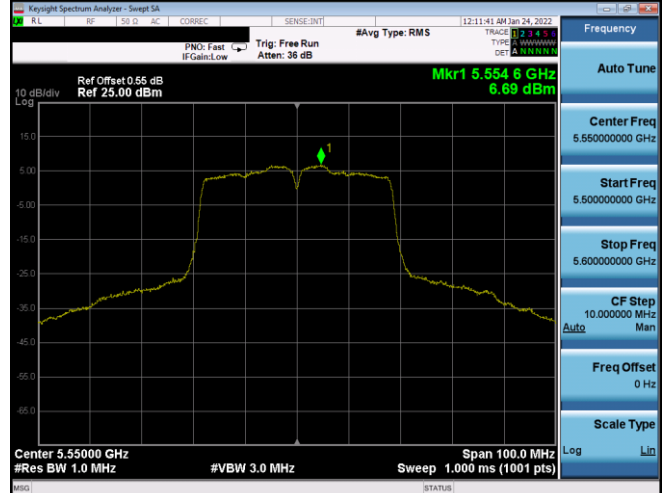
Plot 7-389. PSD CDD Antenna WF8 (40MHz BW 802.11n – Ch. 110, MCS11)
