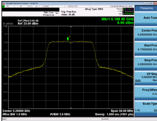
Plot 7-397. PSD SDM Antenna WF8 (20MHz BW 802.11n – Ch. 40, MCS13)
