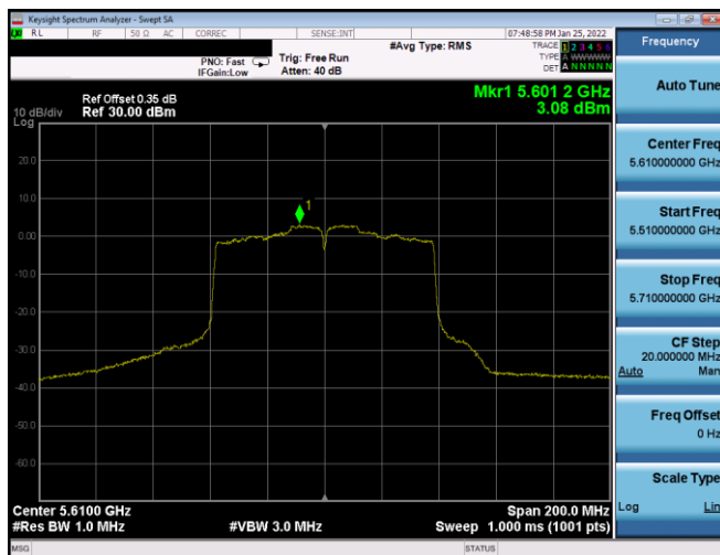
Plot 7-357. PSD CDD Antenna WF8 (80MHz BW 802.11ac – Ch. 122, MCS0)
