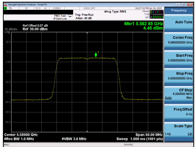
Plot 7-352. PSD SDM Antenna WF7a (20MHz BW 802.11ax(SU) – Ch. 116, MCS0)
