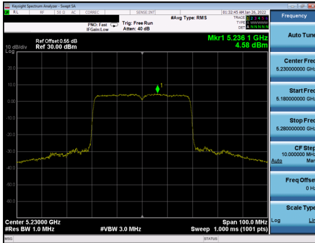
Plot 7-404. PSD SDM Antenna WF7a (40MHz BW 802.11ax(SU) – Ch. 46, MCS5)
