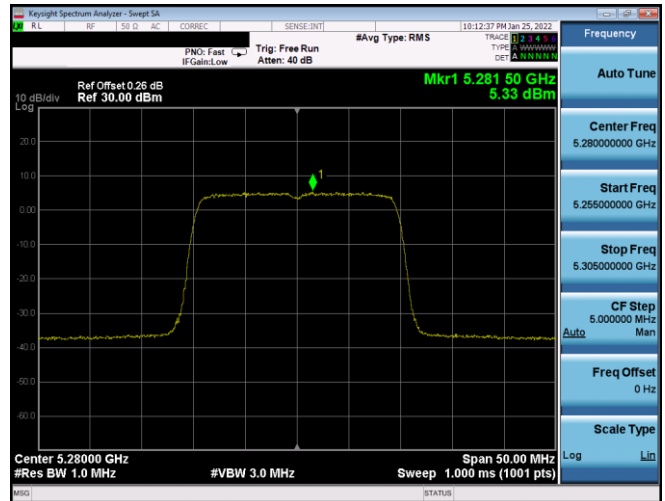
Plot 7-376. PSD SDM Antenna WF7a (20MHz BW 802.11ax(SU) – Ch. 56, MCS3)
