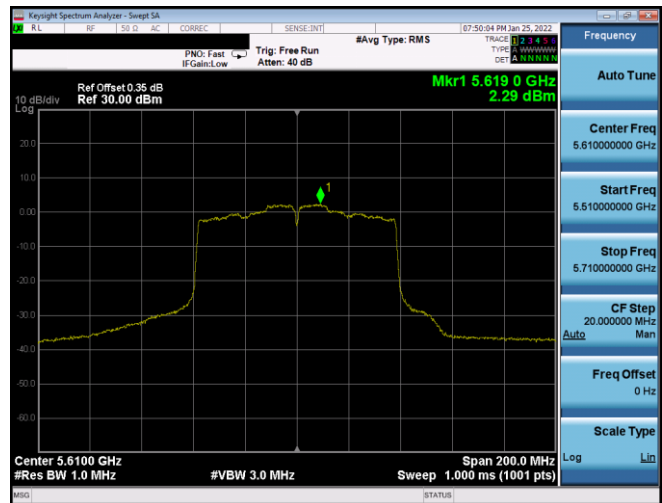
Plot 7-358. PSD CDD Antenna WF7a (80MHz BW 802.11ac – Ch. 122, MCS0)
