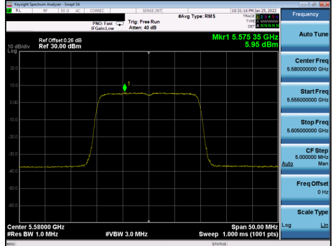
Plot 7-388. PSD SDM Antenna WF7a (20MHz BW 802.11ax(SU) – Ch. 116, MCS3)
