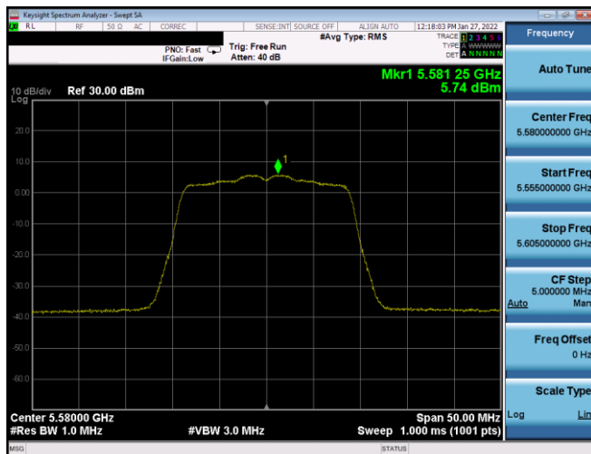
Plot 7-350. PSD SDM Antenna WF7a (20MHz BW 802.11n – Ch. 116, MCS8)
