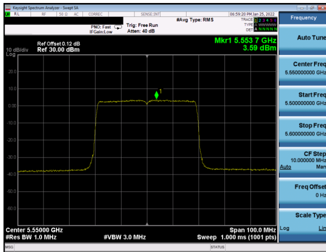
Plot 7-356. PSD SDM Antenna WF7a (40MHz BW 802.11ax(SU) – Ch. 110, MCS0)
