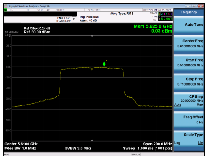
Plot 7-360. PSD CDD Antenna WF7a (80MHz BW 802.11ax(SU) – Ch. 122, MCS0)
