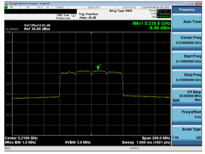
Plot 7-407. PSD CDD Antenna WF8 (80MHz BW 802.11ax(SU) – Ch. 42, MCS5)
