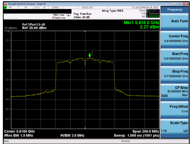
Plot 7-394. PSD CDD Antenna WF7a (80MHz BW 802.11ac – Ch. 122, MCS3)
