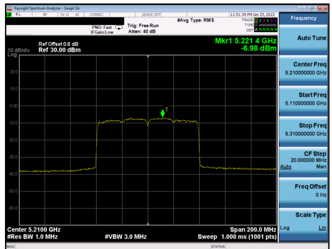
Plot 7-372. PSD CDD Antenna WF7a (80MHz BW 802.11ax(SU) – Ch. 42, MCS3)
