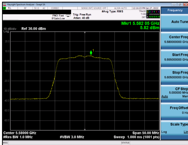
Plot 7-349. PSD SDM Antenna WF8 (20MHz BW 802.11n – Ch. 116, MCS8)
