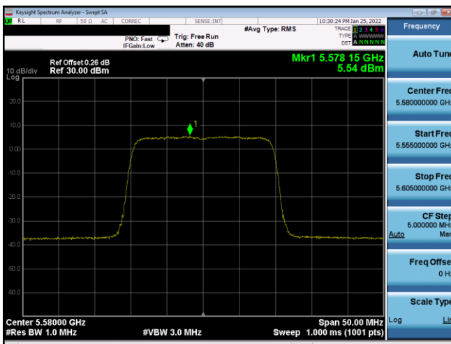
Plot 7-387. PSD SDM Antenna WF8 (20MHz BW 802.11ax(SU) – Ch. 116, MCS3)
