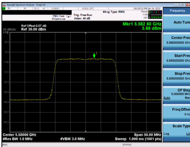
Plot 7-351. PSD SDM Antenna WF8 (20MHz BW 802.11ax(SU) – Ch. 116, MCS0)
