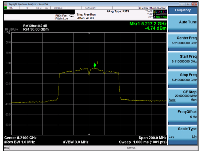
Plot 7-370. PSD CDD Antenna WF7a (80MHz BW 802.11ac – Ch. 42, MCS3)
