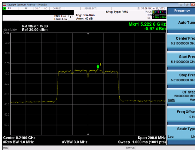
Plot 7-405. PSD CDD Antenna WF8 (80MHz BW 802.11ac – Ch. 42, MCS5)
