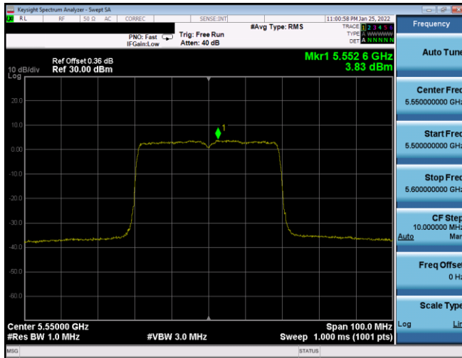
Plot 7-391. PSD CDD Antenna WF8 (40MHz BW 802.11ax(SU) – Ch. 110, MCS3)
