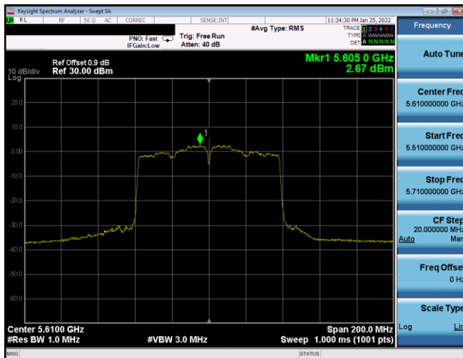
Plot 7-393. PSD CDD Antenna WF8 (80MHz BW 802.11ac – Ch. 122, MCS3)
