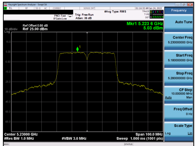
Plot 7-402. PSD SDM Antenna WF7a (40MHz BW 802.11n – Ch. 46, MCS13)
