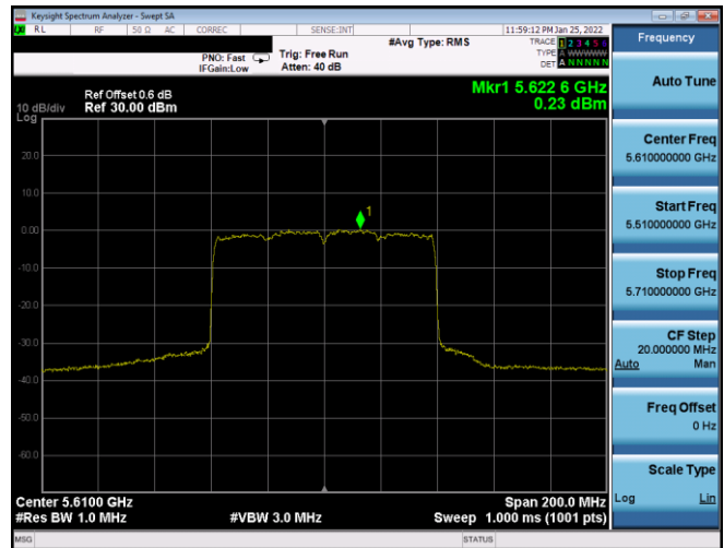
Plot 7-395. PSD CDD Antenna WF8 (80MHz BW 802.11ax(SU) – Ch. 122, MCS3)
