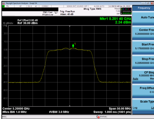
Plot 7-307. ISED PSD Antenna WF7a (20MHz BW 11n – Ch.40, MCS0)
