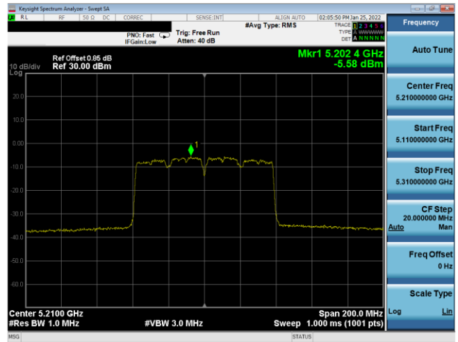
Plot 7-323. ISED PSD Antenna WF7a (80MHz BW 11ac – Ch.42, MCS5)
