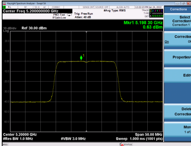
Plot 7-308. ISED PSD Antenna WF7a (20MHz BW 11ax(SU) – Ch.40, MCS0)
