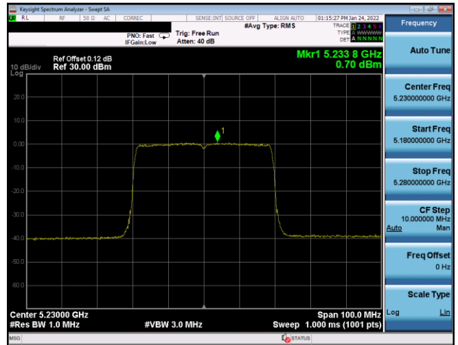
Plot 7-310. ISED PSD Antenna WF7a (40MHz BW 11ax(SU) – Ch.46, MCS0)
