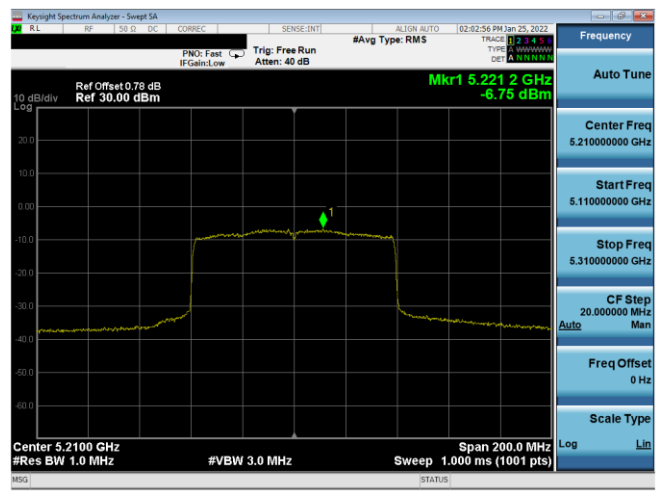
Plot 7-324. ISED PSD Antenna WF7a (80MHz BW 11ax(SU) – Ch.42, MCS5)
