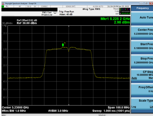
Plot 7-321. ISED PSD Antenna WF7a (40MHz BW 11n – Ch.46, MCS5)
