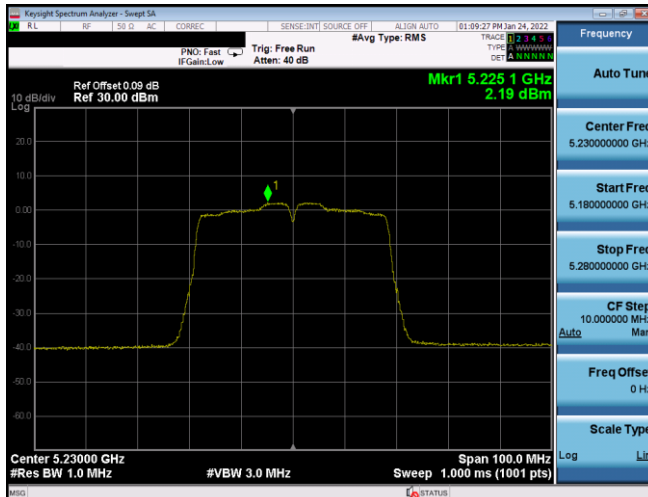
Plot 7-309. ISED PSD Antenna WF7a (40MHz BW 11n – Ch.46, MCS0)
