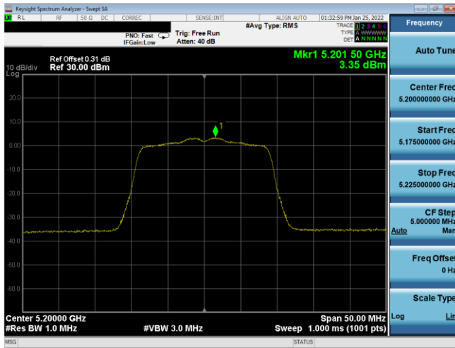
Plot 7-319. ISED PSD Antenna WF7a (20MHz BW 11n – Ch.40, MCS5)
