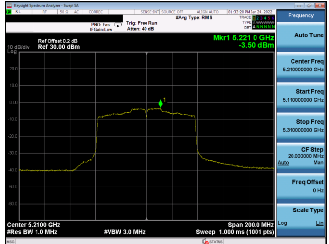
Plot 7-311. ISED PSD Antenna WF7a (80MHz BW 11ac – Ch.42, MCS0)
