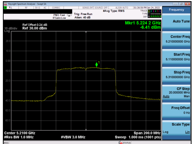
Plot 7-312. ISED PSD Antenna WF7a (80MHz BW 11ax(SU) – Ch.42, MCS0)
