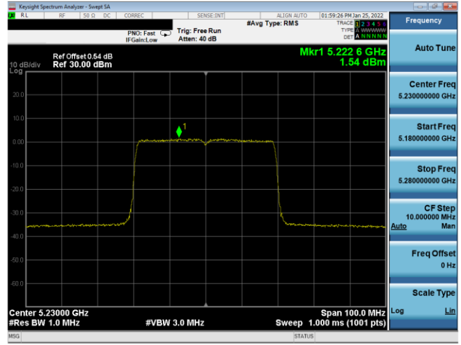
Plot 7-322. ISED PSD Antenna WF7a (40MHz BW 11ax(SU) – Ch.46, MCS5)
