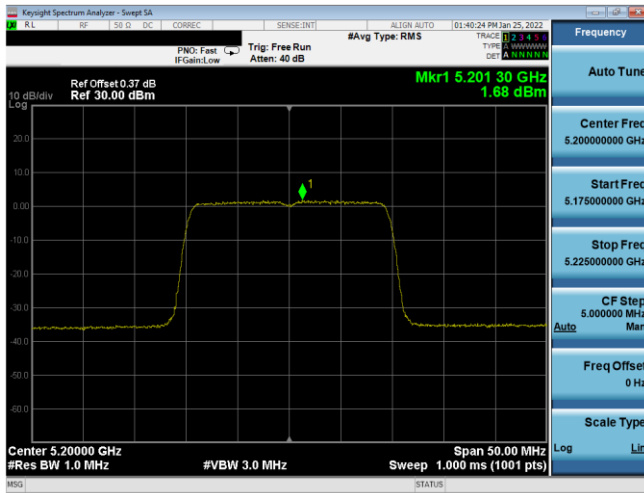
Plot 7-320. ISED PSD Antenna WF7a (20MHz BW 11ax(SU) – Ch.40, MCS5)
