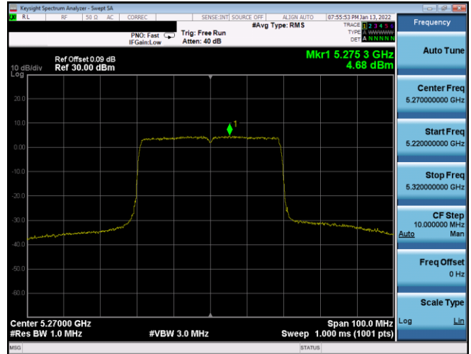
Plot 7-154. PSD Antenna WF8 (40MHz BW 802.11ax(SU) - Ch. 54, MCS0)
