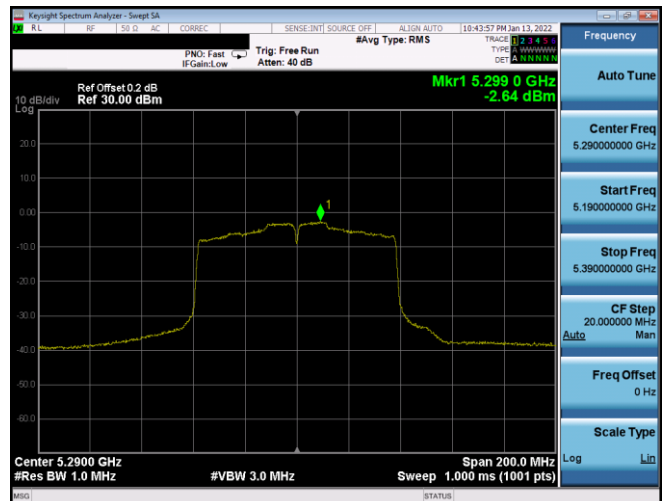
Plot 7-155. PSD Antenna WF8 (80MHz BW 802.11ac - Ch. 58, MCS0)
