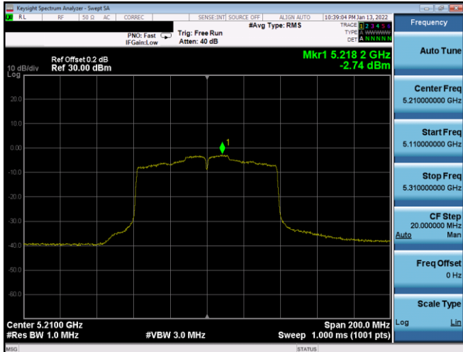
Plot 7-149. PSD Antenna WF8 (80MHz BW 802.11ac - Ch. 42, MCS0)
