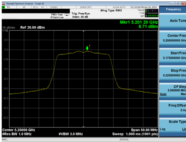
Plot 7-145. PSD Antenna WF8 (20MHz BW 802.11n - Ch. 40, MCS0)
