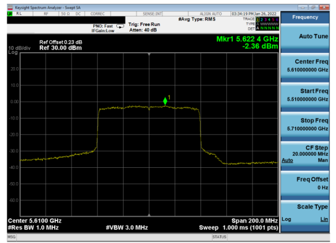
Plot 7-162. PSD Antenna WF8 (80MHz BW 802.11ax(SU) – Ch. 122, MCS0)
