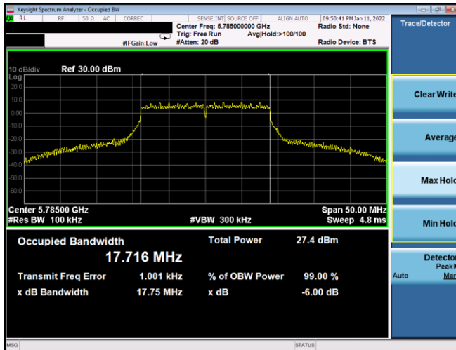
Plot 7-139. 6dB BW & 99% OBW Antenna WF7a (20MHz BW 802.11n – Ch. 157, MCS5)
