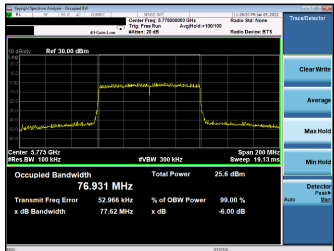
Plot 7-144. 6dB BW & 99% OBW Antenna WF7a (80MHz BW 802.11ax(SU) – Ch. 155, MCS5)
