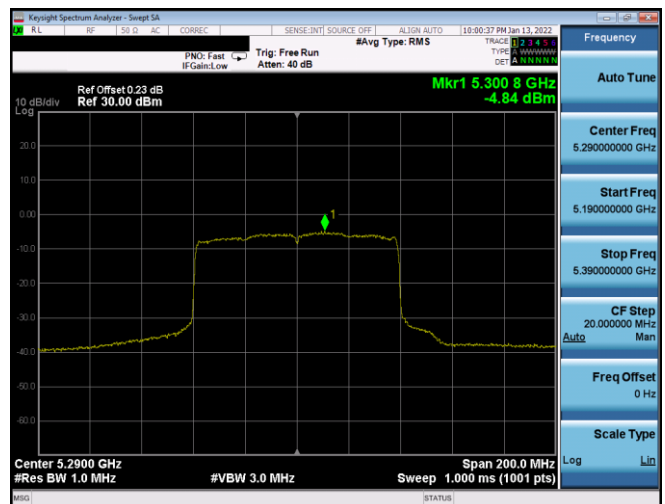
Plot 7-156. PSD Antenna WF8 (80MHz BW 802.11ax(SU) - Ch. 58, MCS0)
