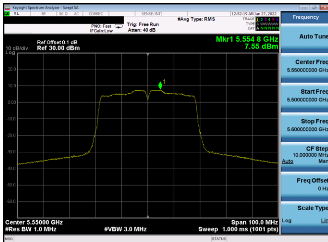
Plot 7-159. PSD Antenna WF8 (40MHz BW 802.11n – Ch. 110, MCS0)
