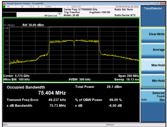
Plot 7-137. 6dB BW & 99% OBW Antenna WF7a (80MHz BW 802.11ac – Ch. 155, MCS3)
