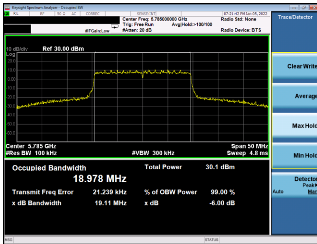
Plot 7-116. 6dB BW & 99% OBW Antenna WF8 (20MHz BW 802.11ax(SU) – Ch. 157, MCS3)
