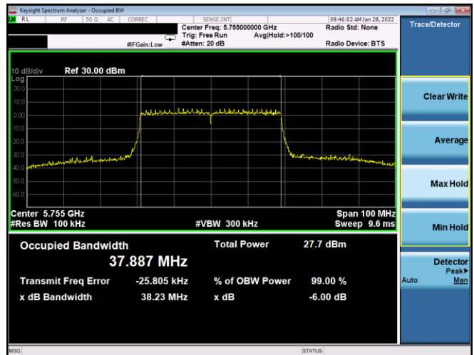
Plot 7-130. 6dB BW & 99% OBW Antenna WF7a (40MHz BW 802.11ax(SU) – Ch. 151, MCS0)
