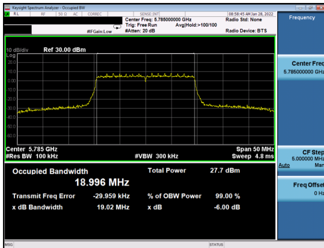
Plot 7-110. 6dB BW & 99% OBW Antenna WF8 (20MHz BW 802.11ax(SU) – Ch. 157, MCS0)
