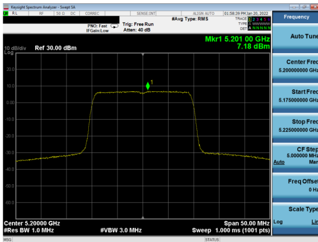
Plot 7-146. PSD Antenna WF8 (20MHz BW 802.11ax(SU) - Ch. 40, MCS0)
