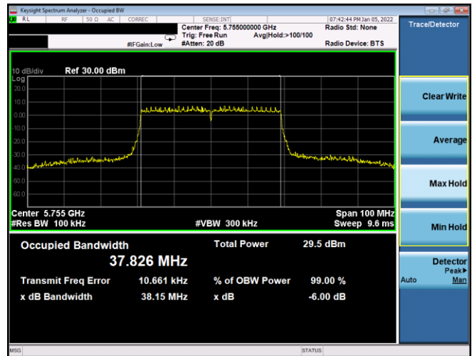
Plot 7-112. 6dB BW & 99% OBW Antenna WF8 (40MHz BW 802.11ax(SU) – Ch. 151, MCS0)
