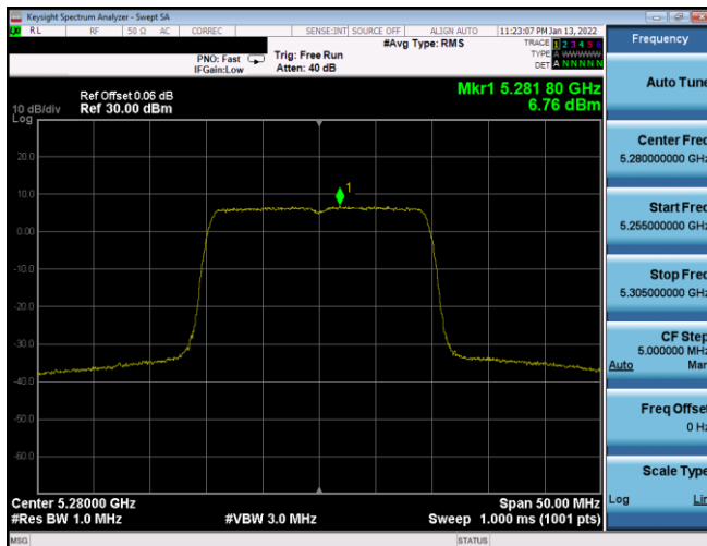
Plot 7-152. PSD Antenna WF8 (20MHz BW 802.11ax(SU) - Ch. 56, MCS0)
