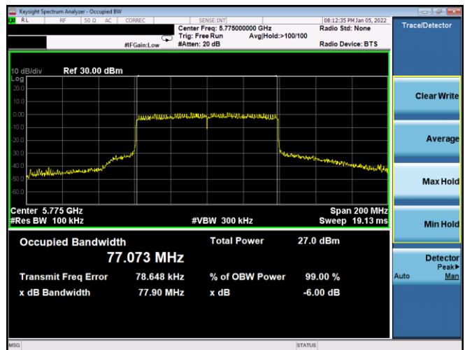
Plot 7-120. 6dB BW & 99% OBW Antenna WF8 (80MHz BW 802.11ax(SU) – Ch. 155, MCS3)
