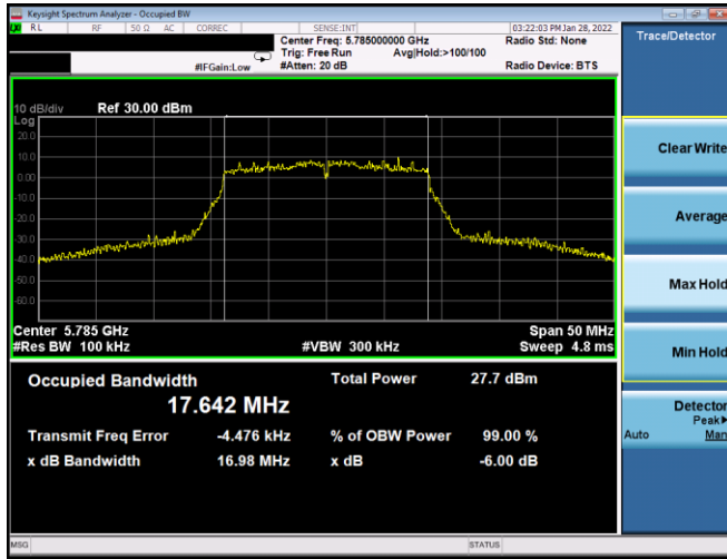
Plot 7-133. 6dB BW & 99% OBW Antenna WF7a (20MHz BW 802.11n – Ch. 157, MCS3)
