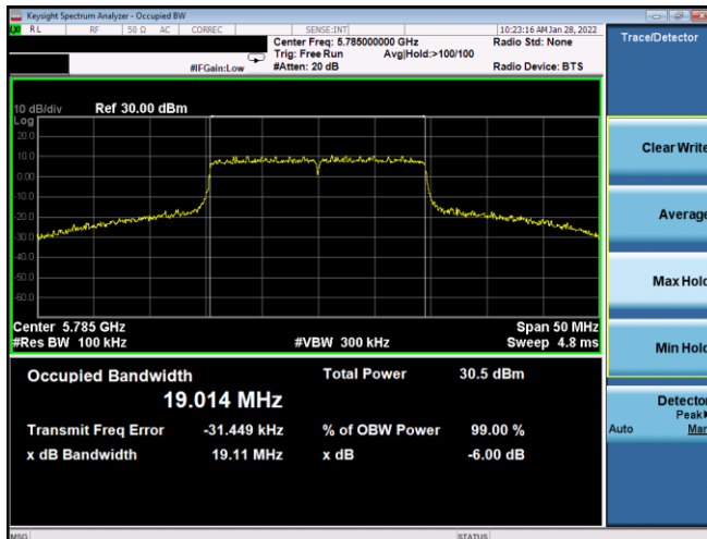
Plot 7-140. 6dB BW & 99% OBW Antenna WF7a (20MHz BW 802.11ax(SU) – Ch. 157, MCS5)
