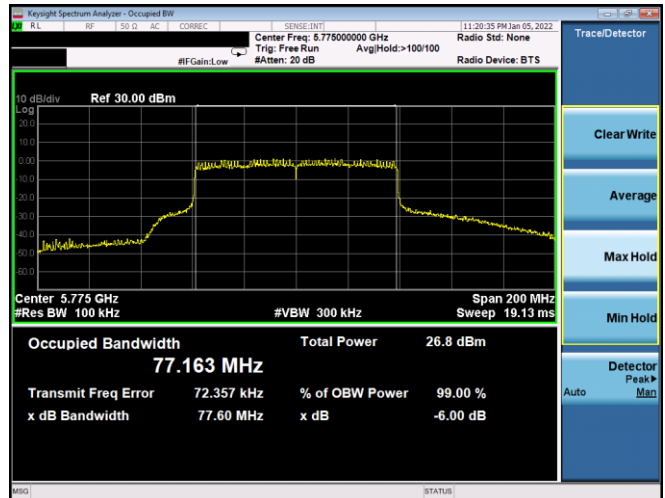
Plot 7-132. 6dB BW & 99% OBW Antenna WF7a (80MHz BW 802.11ax(SU) – Ch. 155, MCS0)
