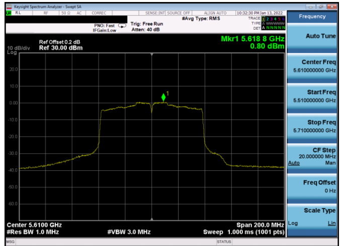
Plot 7-161. PSD Antenna WF8 (80MHz BW 802.11ac – Ch. 122, MCS0)
