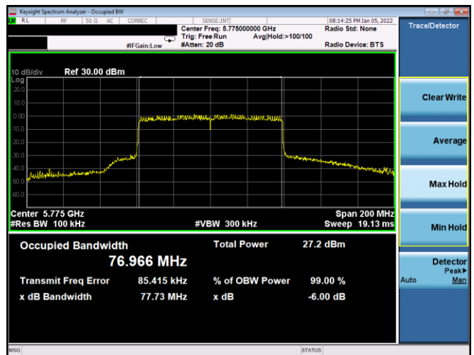
Plot 7-126. 6dB BW & 99% OBW Antenna WF8 (80MHz BW 802.11ax(SU) – Ch. 155, MCS5)
