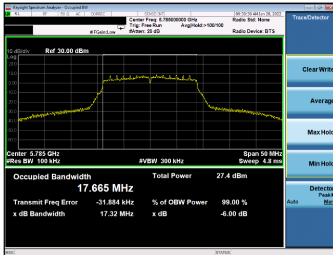
Plot 7-127. 6dB BW & 99% OBW Antenna WF7a (20MHz BW 802.11n – Ch. 157, MCS0)
