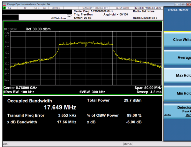
Plot 7-115. 6dB BW & 99% OBW Antenna WF8 (20MHz BW 802.11n – Ch. 157, MCS3)
