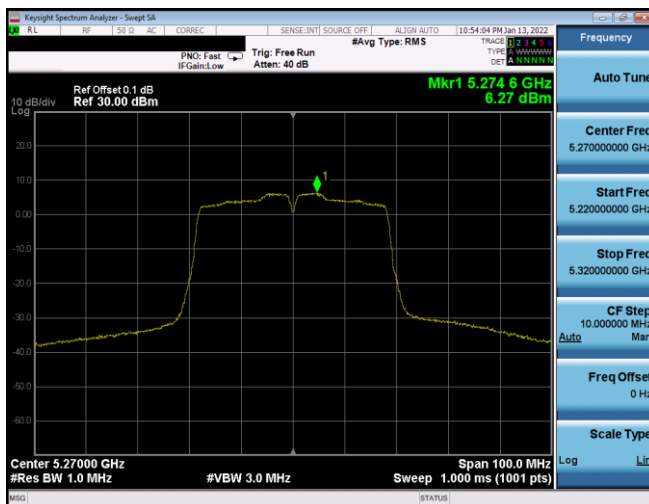
Plot 7-153. PSD Antenna WF8 (40MHz BW 802.11n - Ch. 54, MCS0)
