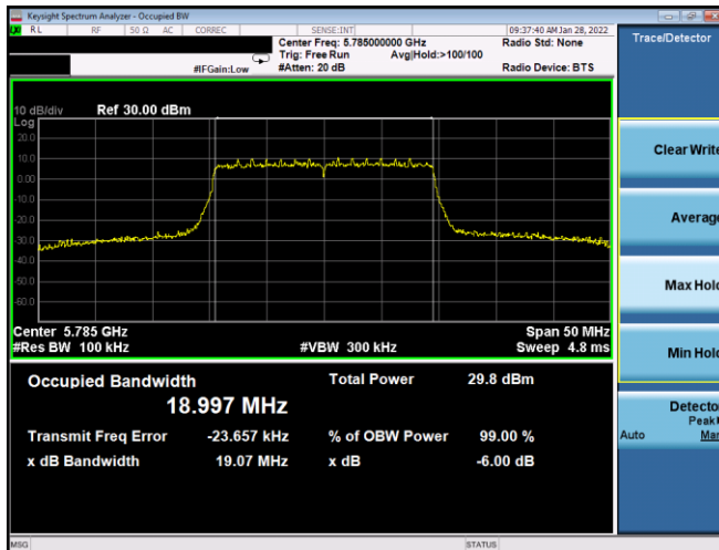
Plot 7-128. 6dB BW & 99% OBW Antenna WF7a (20MHz BW 802.11ax(SU) – Ch. 157, MCS0)
