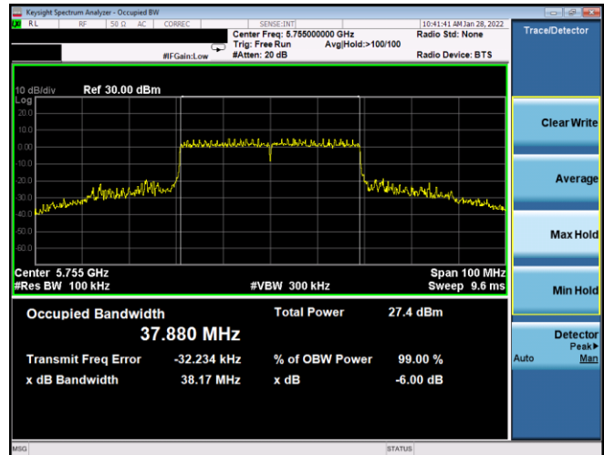
Plot 7-142. 6dB BW & 99% OBW Antenna WF7a (40MHz BW 802.11ax(SU) – Ch. 151, MCS5)
