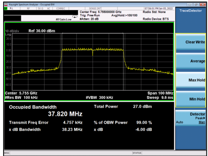
Plot 7-118. 6dB BW & 99% OBW Antenna WF8 (40MHz BW 802.11ax(SU) – Ch. 151, MCS3)
