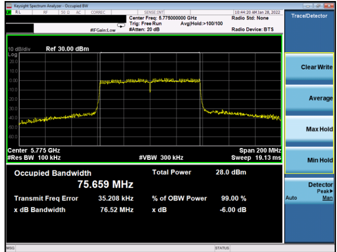
Plot 7-131. 6dB BW & 99% OBW Antenna WF7a (80MHz BW 802.11ac – Ch. 155, MCS0)
