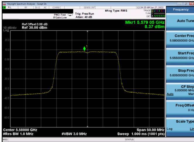
Plot 7-158. PSD Antenna WF8 (20MHz BW 802.11ax(SU) – Ch. 116, MCS0)
