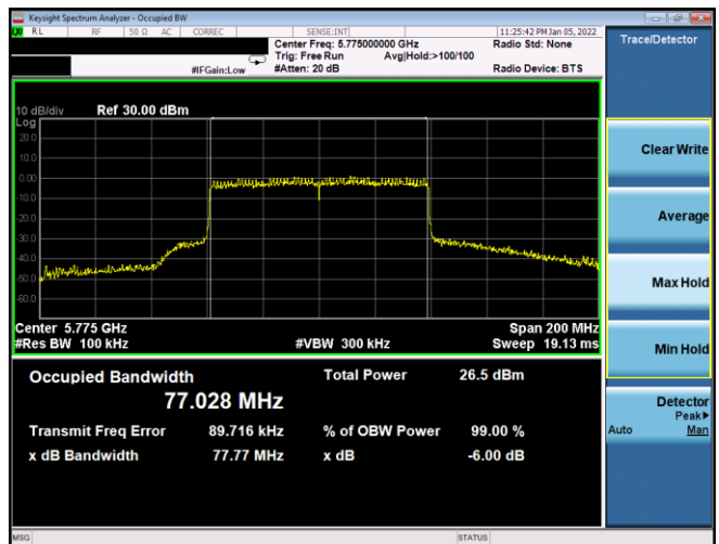
Plot 7-138. 6dB BW & 99% OBW Antenna WF7a (80MHz BW 802.11ax(SU) – Ch. 155, MCS3)
