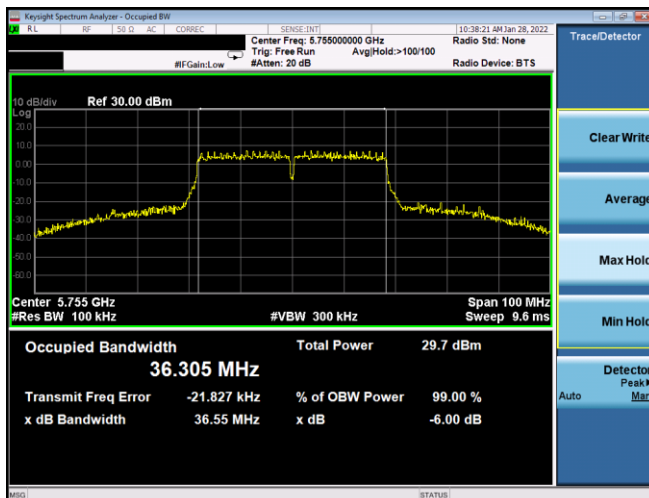
Plot 7-141. 6dB BW & 99% OBW Antenna WF7a (40MHz BW 802.11n – Ch. 151, MCS5)
