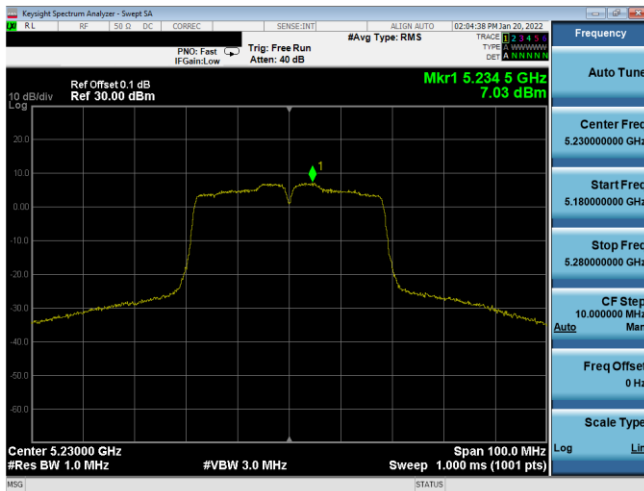
Plot 7-147. PSD Antenna WF8 (40MHz BW 802.11n - Ch. 46, MCS0)
