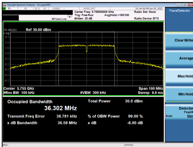
Plot 7-123. 6dB BW & 99% OBW Antenna WF8 (40MHz BW 802.11n – Ch. 151, MCS5)
