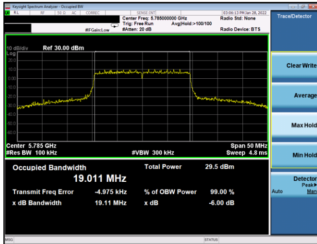
Plot 7-134. 6dB BW & 99% OBW Antenna WF7a (20MHz BW 802.11ax(SU) – Ch. 157, MCS3)
