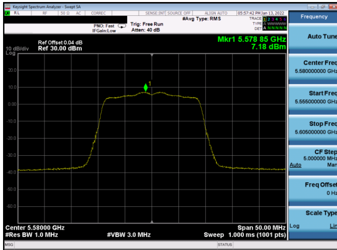
Plot 7-157. PSD Antenna WF8 (20MHz BW 802.11n – Ch. 116, MCS0)
