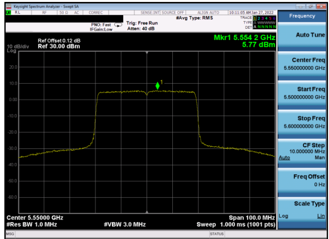
Plot 7-160. PSD Antenna WF8 (40MHz BW 802.11ax(SU) – Ch. 110, MCS0)
