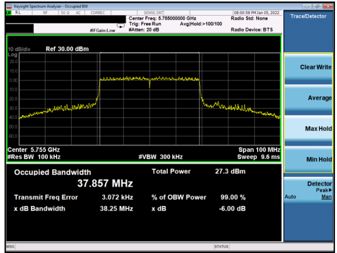
Plot 7-124. 6dB BW & 99% OBW Antenna WF8 (40MHz BW 802.11ax(SU) – Ch. 151, MCS5)
