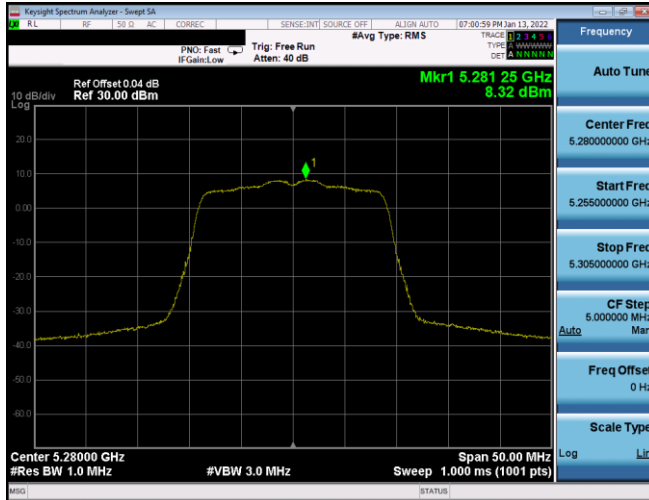
Plot 7-151. PSD Antenna WF8 (20MHz BW 802.11n - Ch. 56, MCS0)
