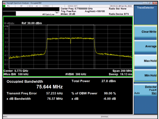
Plot 7-125. 6dB BW & 99% OBW Antenna WF8 (80MHz BW 802.11ac – Ch. 155, MCS5)
