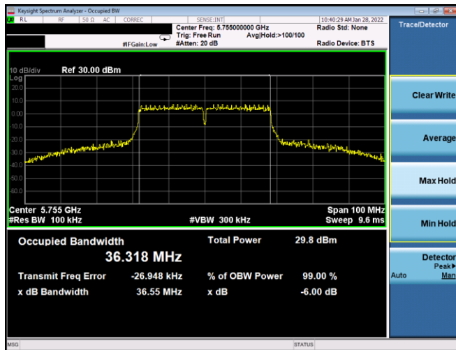
Plot 7-135. 6dB BW & 99% OBW Antenna WF7a (40MHz BW 802.11n – Ch. 151, MCS3)
