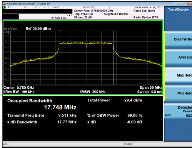
Plot 7-121. 6dB BW & 99% OBW Antenna WF8 (20MHz BW 802.11n – Ch. 157, MCS5)
