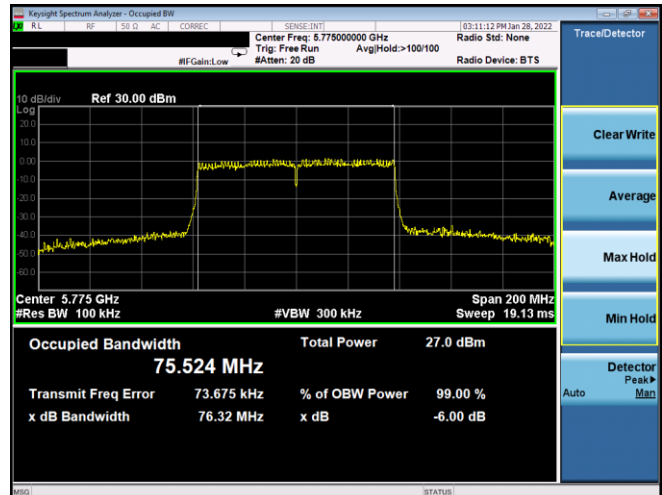
Plot 7-143. 6dB BW & 99% OBW Antenna WF7a (80MHz BW 802.11ac – Ch. 155, MCS5)
