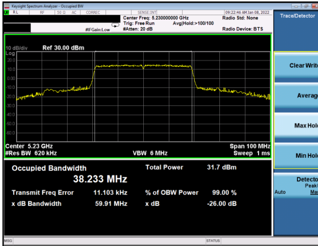
Plot 7-44. 26dB BW & 99% OBW Antenna WF7a (40MHz BW 11ax – RU484 – Ch.46)
