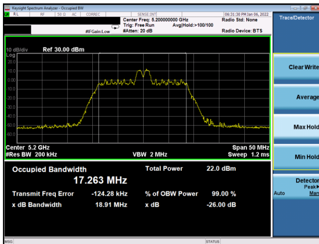
Plot 7-2. 26dB BW & 99% OBW Antenna WF8 (20MHz BW 11ax Index 4 – RU26 – Ch.40)
