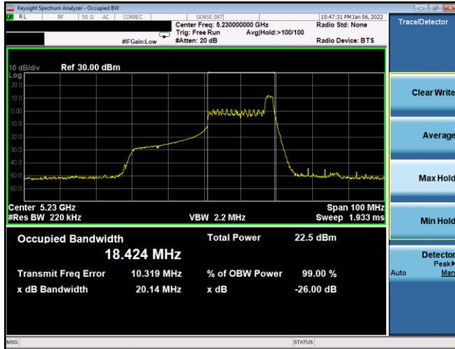
Plot 7-7. 26dB BW & 99% OBW Antenna WF8 (40MHz BW 11ax Index 17 – RU26 – Ch.46)
