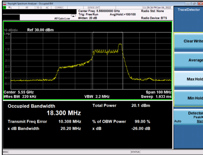
Plot 7-31. 26dB BW & 99% OBW Antenna WF8 (40MHz BW 11ax Index 17 – RU26 – Ch.110)
