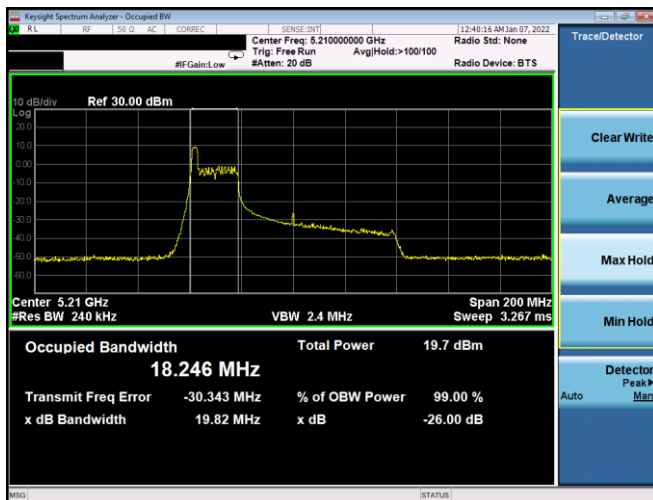
Plot 7-9. 26dB BW & 99% OBW Antenna WF8 (80MHz BW 11ax Index 0 – RU26 – Ch.42)
