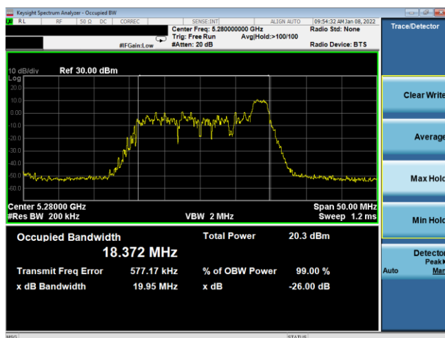
Plot 7-51. 26dB BW & 99% OBW Antenna WF7a (20MHz BW 11ax Index 8 – RU26 – Ch.56)
