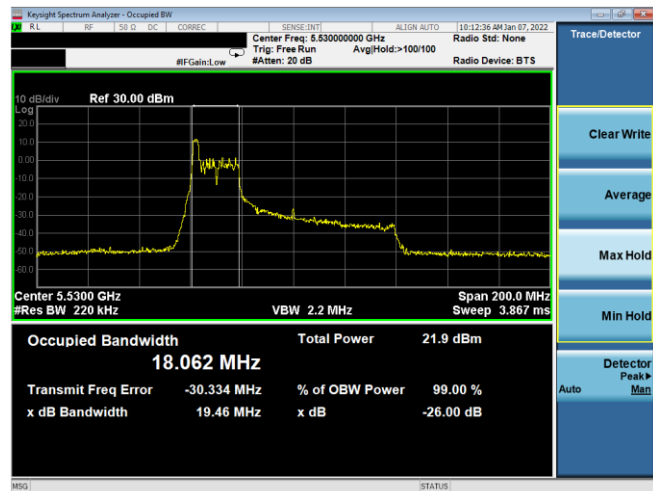
Plot 7-33. 26dB BW & 99% OBW Antenna WF8 (80MHz BW 11ax Index 0 – RU26 – Ch.106)
