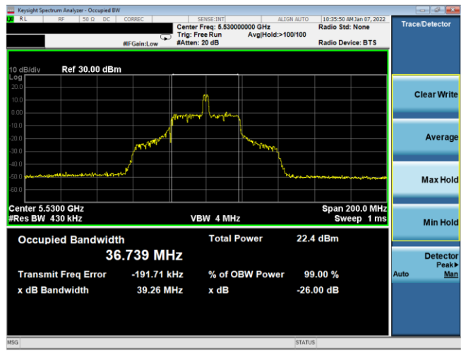
Plot 7-34. 26dB BW & 99% OBW Antenna WF8 (80MHz BW 11ax Index 18 – RU26 – Ch.106)
