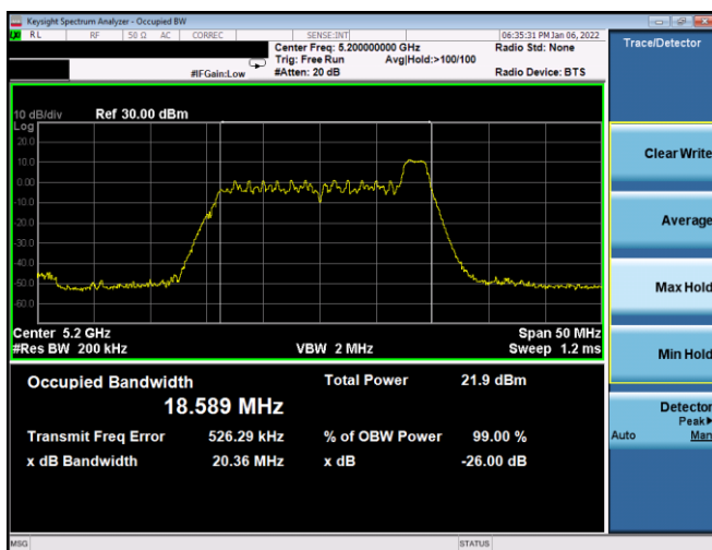
Plot 7-3. 26dB BW & 99% OBW Antenna WF8 (20MHz BW 11ax Index 8– RU26 – Ch.40)
