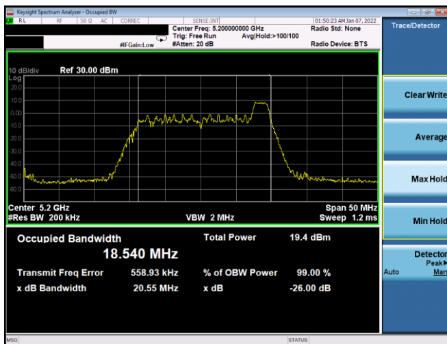
Plot 7-39. 26dB BW & 99% OBW Antenna WF7a (20MHz BW 11ax Index 8 – RU26 – Ch.40)
