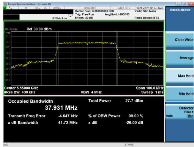
Plot 7-32. 26dB BW & 99% OBW Antenna WF8 (40MHz BW 11ax – RU484 – Ch.110)
