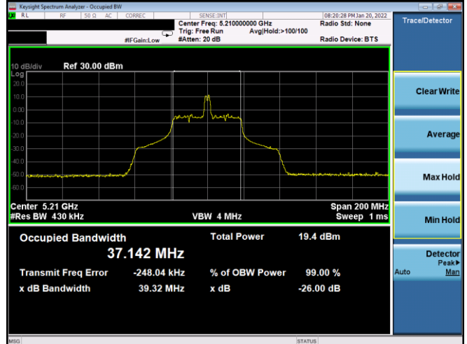
Plot 7-46. 26dB BW & 99% OBW Antenna WF7a (80MHz BW 11ax Index 18 – RU26 – Ch.42)
