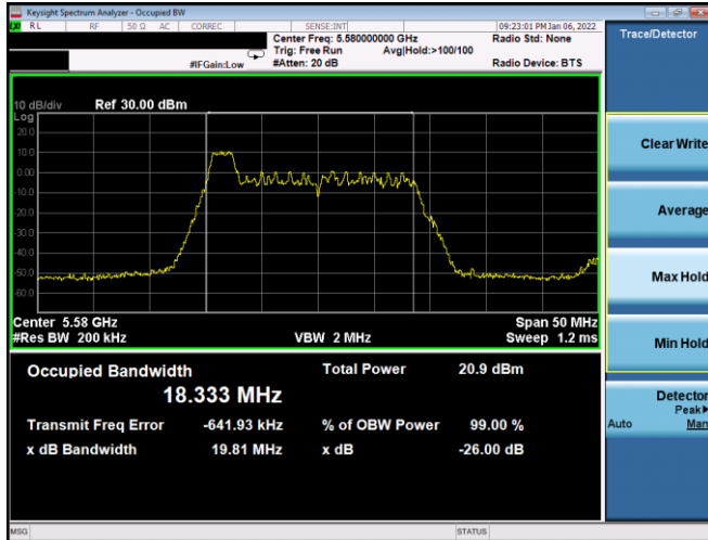
Plot 7-25. 26dB BW & 99% OBW Antenna WF8 (20MHz BW 11ax Index 0 – RU26 – Ch.116)
