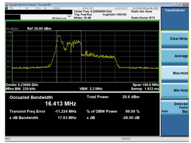
Plot 7-41. 26dB BW & 99% OBW Antenna WF7a (40MHz BW 11ax Index 0 – RU26 – Ch.46)
