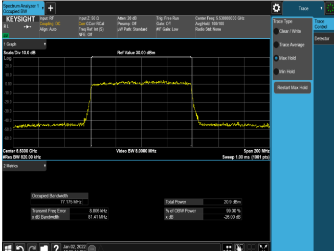
Plot 7-36. 26dB BW & 99% OBW Antenna WF8 (80MHz BW 11ax – RU996 – Ch.106)
