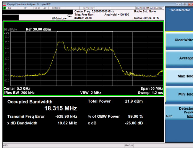
Plot 7-1. 26dB BW & 99% OBW Antenna WF8 (20MHz BW 11ax Index 0 – RU26 – Ch.40)
