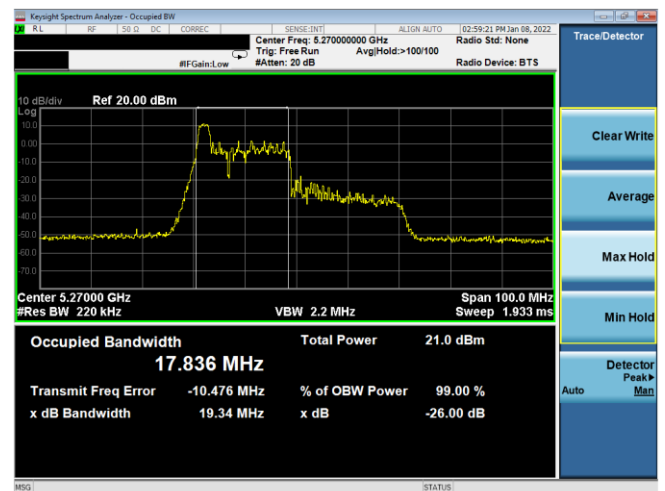
Plot 7-53. 26dB BW & 99% OBW Antenna WF7a (40MHz BW 11ax Index 0 – RU26 – Ch.54)
