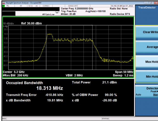
Plot 7-37. 26dB BW & 99% OBW Antenna WF7a (20MHz BW 11ax Index 0 – RU26 – Ch.40)
