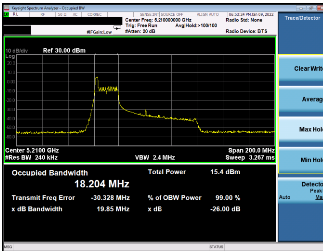
Plot 7-45. 26dB BW & 99% OBW Antenna WF7a (80MHz BW 11ax Index 0 – RU26 – Ch.42)
