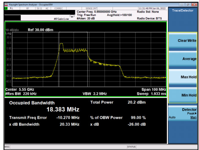
Plot 7-29. 26dB BW & 99% OBW Antenna WF8 (40MHz BW 11ax Index 0 – RU26 – Ch.110)
