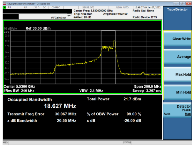
Plot 7-35. 26dB BW & 99% OBW Antenna WF8 (80MHz BW 11ax Index 36 – RU26 – Ch.106)
