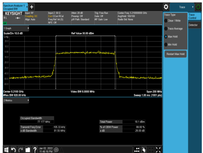
Plot 7-48. 26dB BW & 99% OBW Antenna WF7a (80MHz BW 11ax – RU996 – Ch.42)
