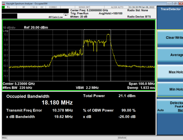
Plot 7-43. 26dB BW & 99% OBW Antenna WF7a (40MHz BW 11ax Index 17 – RU26 – Ch.46)
