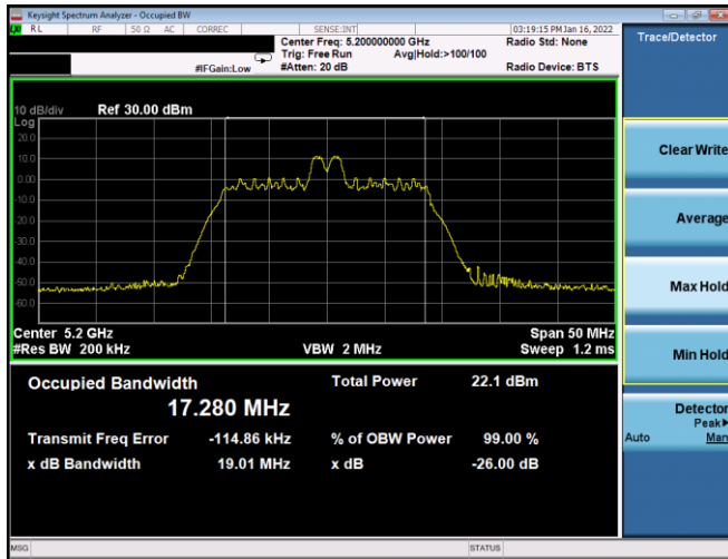
Plot 7-38. 26dB BW & 99% OBW Antenna WF7a (20MHz BW 11ax Index 4 – RU26 – Ch.40)
