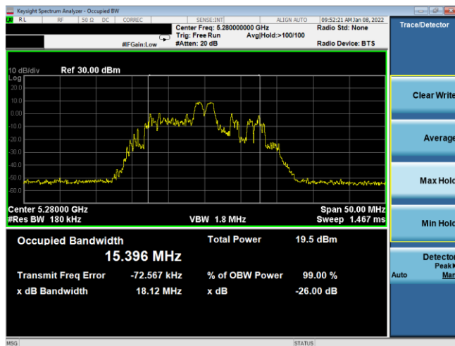
Plot 7-50. 26dB BW & 99% OBW Antenna WF7a (20MHz BW 11ax Index 4 – RU26 – Ch.56)
