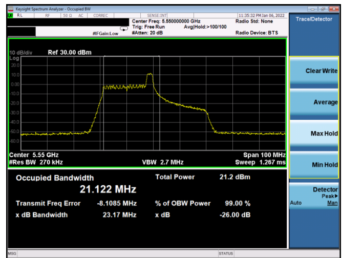
Plot 7-30. 26dB BW & 99% OBW Antenna WF8 (40MHz BW 11ax Index 8 – RU26 – Ch.110)
