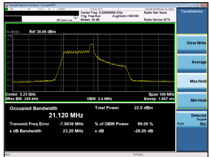
Plot 7-42. 26dB BW & 99% OBW Antenna WF7a (40MHz BW 11ax Index 8 – RU26 – Ch.46)
