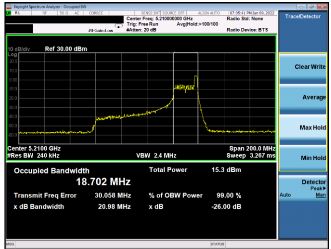
Plot 7-47. 26dB BW & 99% OBW Antenna WF7a (80MHz BW 11ax Index 36 – RU26 – Ch.42)
