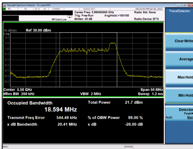
Plot 7-27. 26dB BW & 99% OBW Antenna WF8 (20MHz BW 11ax Index 8– RU26 – Ch.116)
