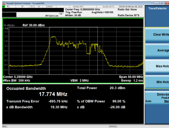
Plot 7-49. 26dB BW & 99% OBW Antenna WF7a (20MHz BW 11ax Index 0 – RU26 – Ch.56)
