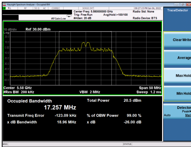
Plot 7-26. 26dB BW & 99% OBW Antenna WF8 (20MHz BW 11ax Index 4 – RU26 – Ch.116)
