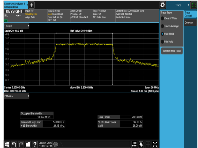
Plot 7-40. 26dB BW & 99% OBW Antenna WF7a (20MHz BW 11ax – RU242 – Ch.40)
