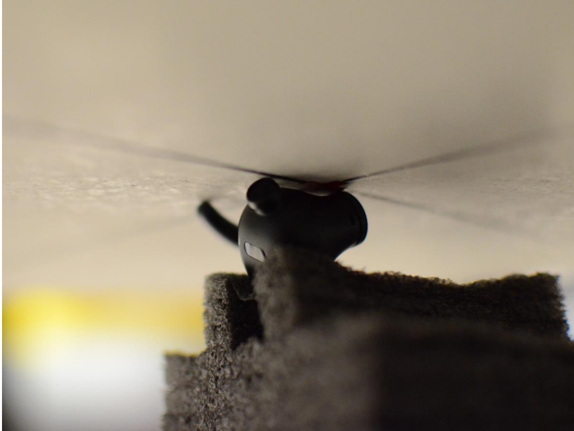
SAR Test Setup Photo 1: Head, Right Earbud, 0 mm
