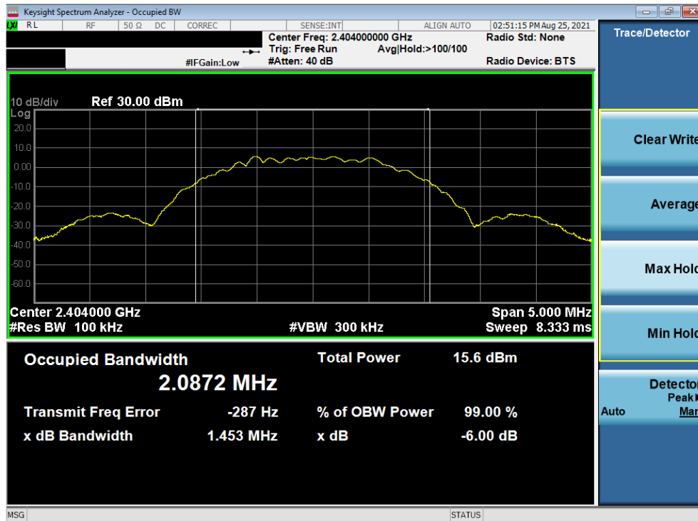
Plot 7-4. 6dB Bandwidth & 99% OBW Plot (Bluetooth (LE), 2Mbps – Ch. 1)
