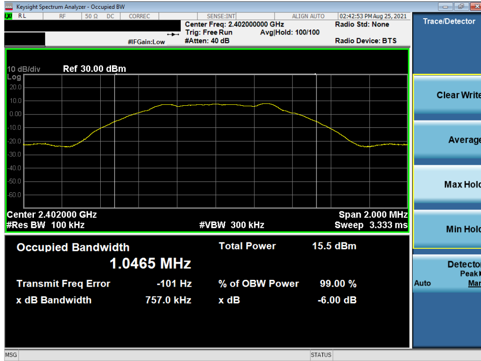
Plot 7-1. 6dB Bandwidth & 99% OBW Plot (Bluetooth (LE), 1Mbps – Ch. 0)
