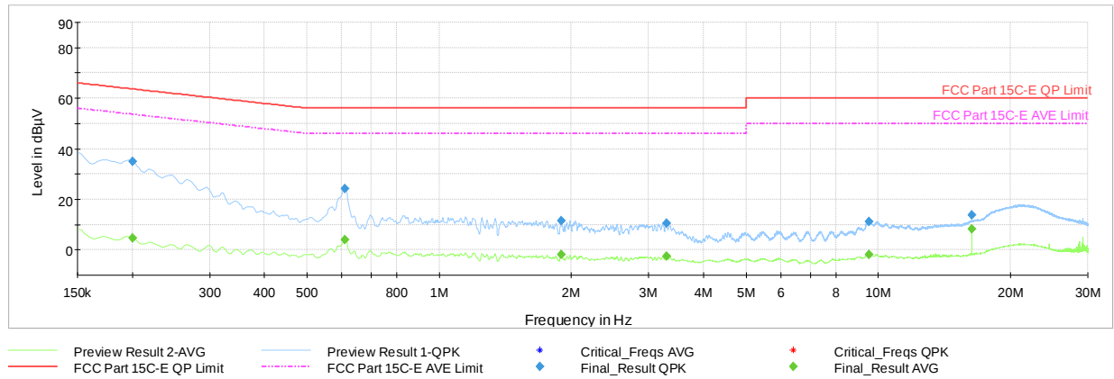
Plot 7-33. AC Line Conducted Emission with Bluetooth LE (1Mbps – Ch.19, L1, with charging case power by Host PC via USB-C cable)
