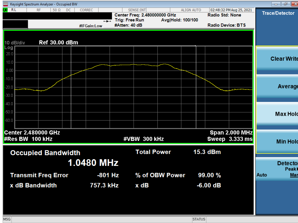
Plot 7-3. 6dB Bandwidth & 99% OBW Plot (Bluetooth (LE), 1Mbps – Ch. 39)
