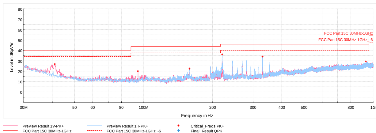
Plot 7-32. Radiated Spurious Emission Below 1GHz (1Mbps – Ch.19, Pol. H & V, with AC/DC Adapter + charging case + USB-C cable)
