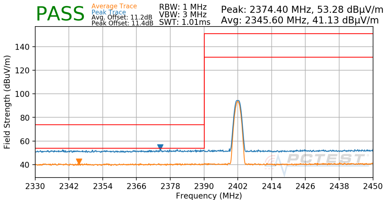
Plot 7-28. Radiated Restricted Lower Band Edge Measurement (Average & Peak)
