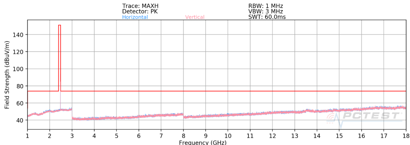
Plot 7-25. Radiated Spurious Emission Above 1GHz (1Mbps – Ch. 39, Ant. Pol. H & V)
