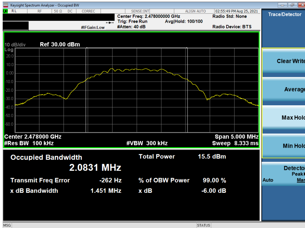
Plot 7-6. 6dB Bandwidth & 99% OBW Plot (Bluetooth (LE), 2Mbps – Ch. 38)
