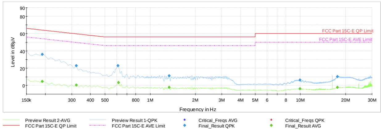
Plot 7-34. AC Line Conducted Emission with Bluetooth LE (1Mbps – Ch.19, N, with charging case powered by Host PC via USB-C cable)
