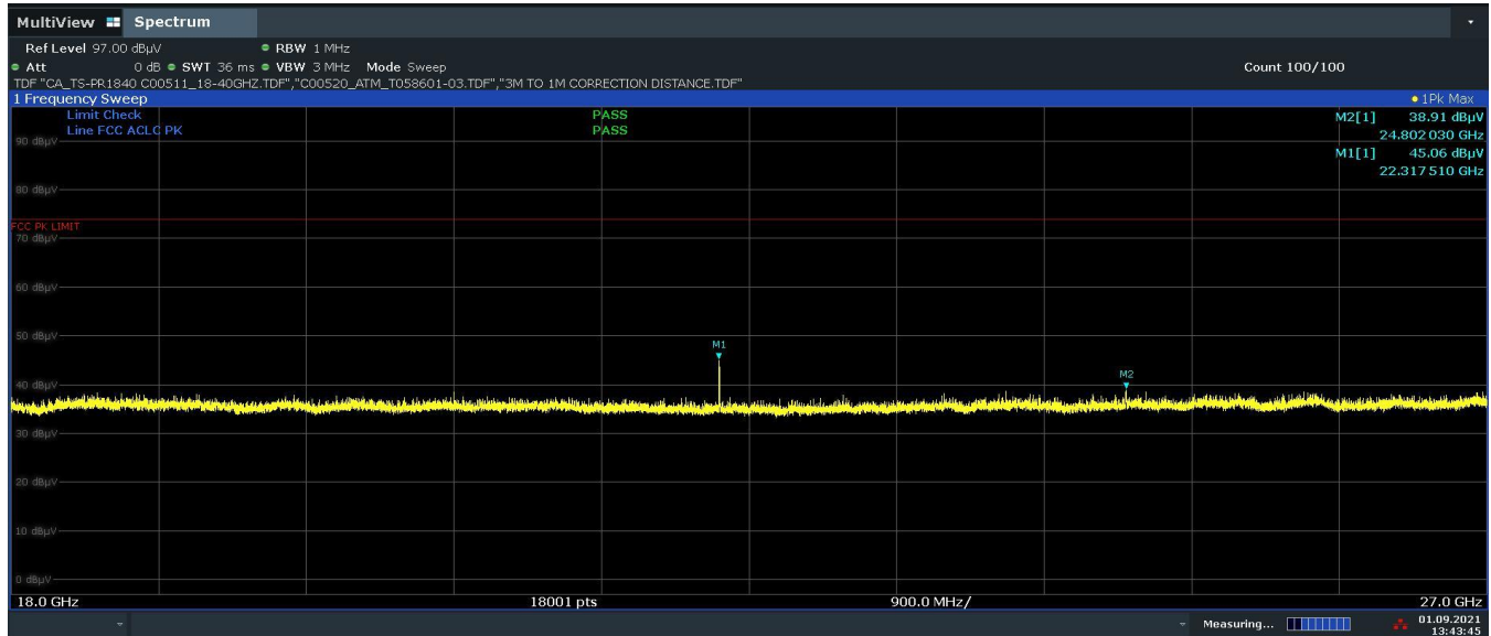
Plot 7-26. Radiated Spurious Plot Above 18GHz (1Mbps – Ch.39, Pol. H)
