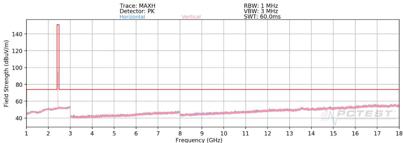
Plot 7-24. Radiated Spurious Emission Above 1GHz (1Mbps – Ch. 19, Ant. Pol. H & V)
