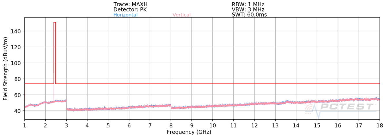
Plot 7-23. Radiated Spurious Emission Above 1GHz (1Mbps – Ch. 0, Ant. Pol. H & V)
