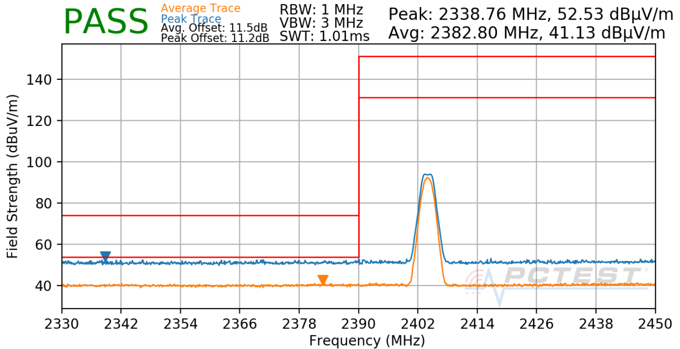
Plot 7-30. Radiated Restricted Lower Band Edge Measurement (Average & Peak)
