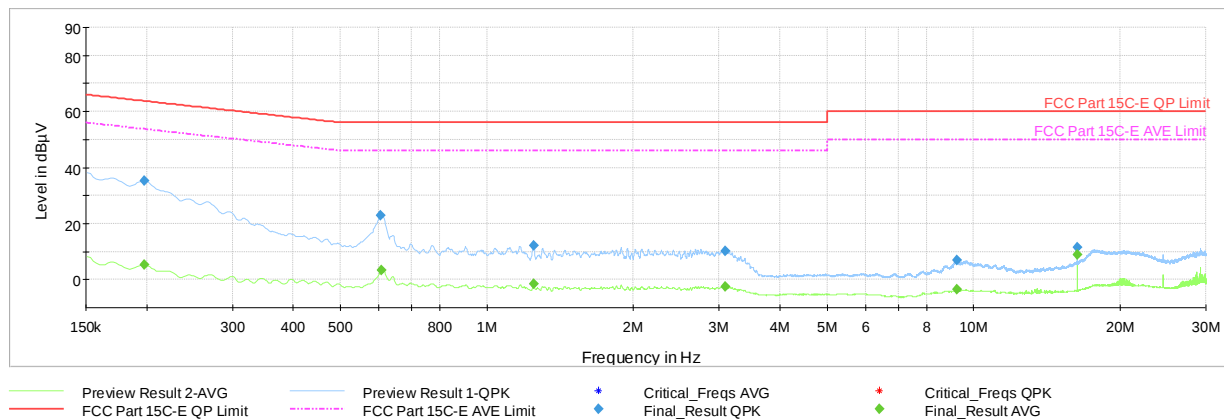
Plot 7-40. AC Line-Conducted Emissions (N, GFSK – Ch.39 with charging case powered by Host PC via USB-C cable)
