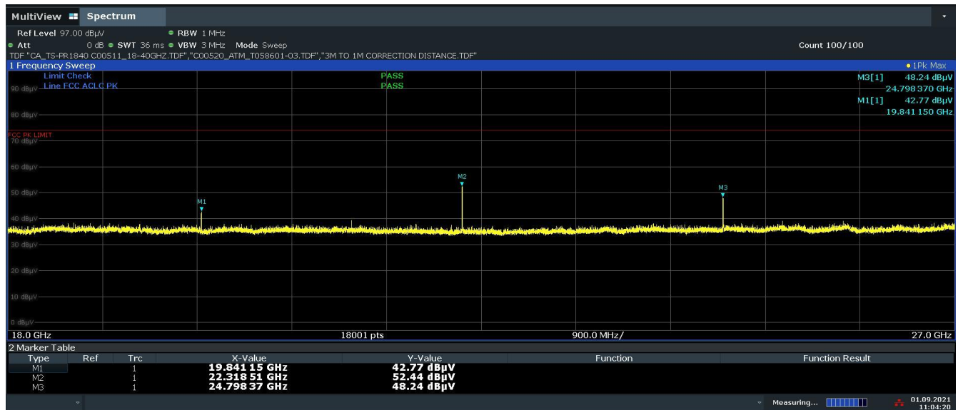
Plot 7-33. Radiated Spurious Emissions above 18GHz (GFSK – Ch.78, Pol. V)
