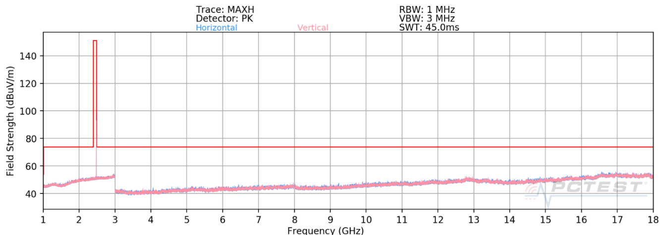
Plot 7-31. Radiated Spurious Emissions above 1GHz (BT GFSK – Ch. 78)
