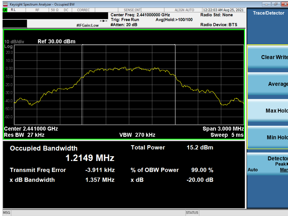
Plot 7-5. Conducted 20dB and 99% OBW Plot (Bluetooth, 8DPSK – Ch. 39)
