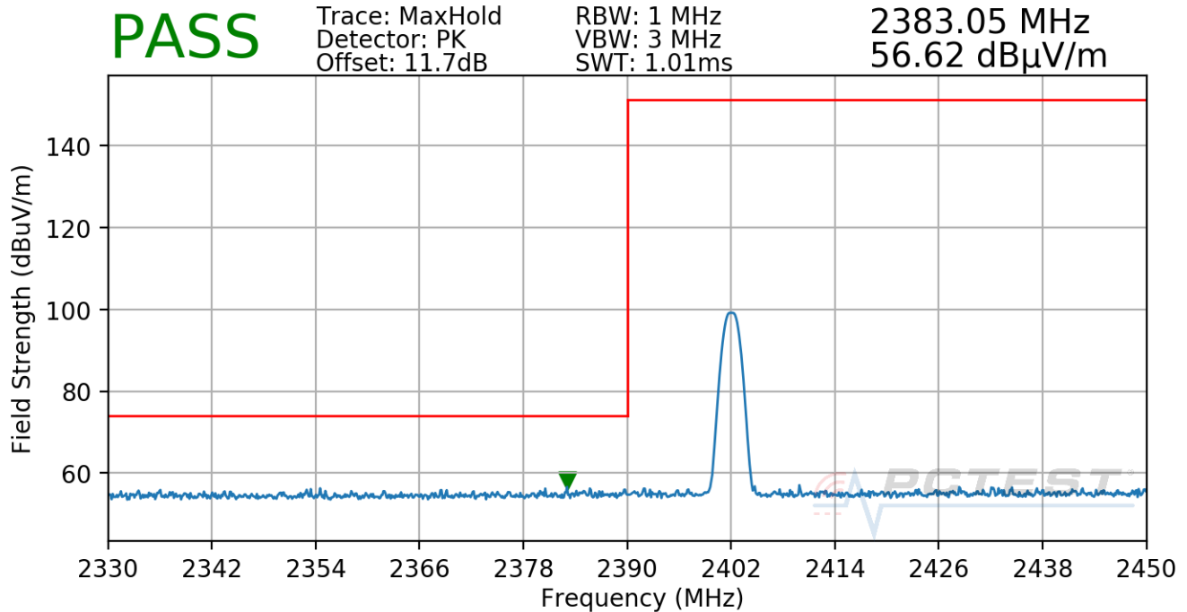
Plot 7-34. Radiated Restricted Lower Band Edge Measurement (Peak)
