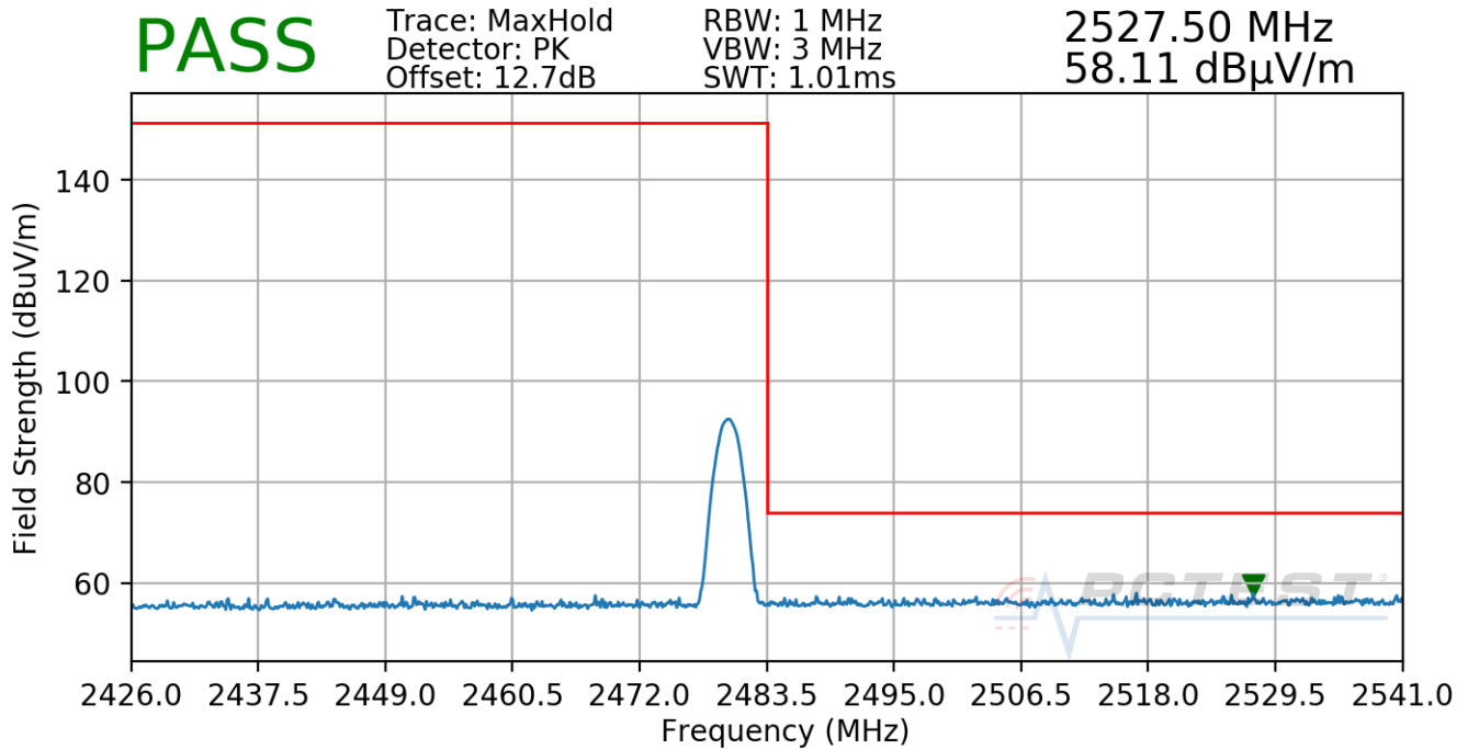
Plot 7-37. Radiated Restricted Upper Band Edge Measurement (Peak)
