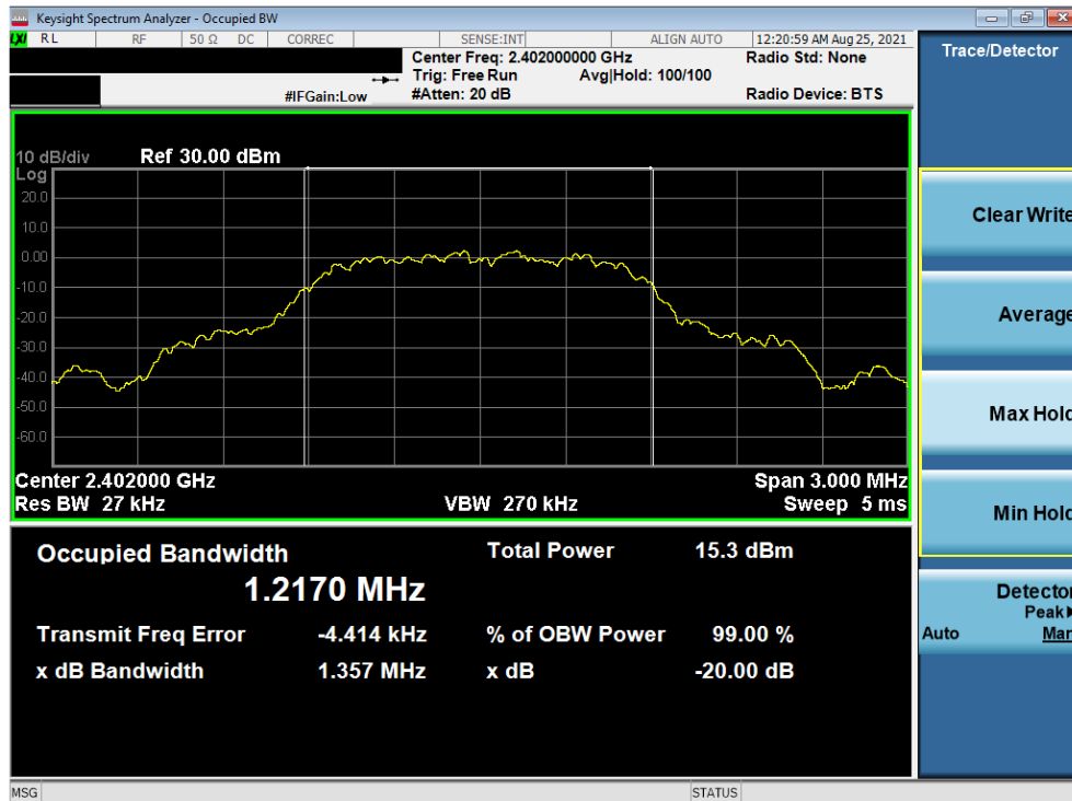
Plot 7-4. Conducted 20dB and 99% OBW Plot (Bluetooth, 8DPSK – Ch. 0)
