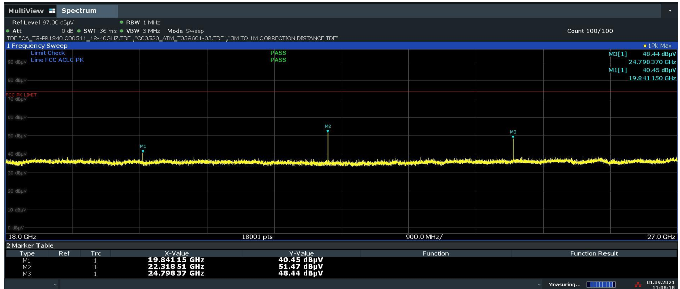
Plot 7-32. Radiated Spurious Emissions above 18GHz (GFSK – Ch.78, Pol. H)
