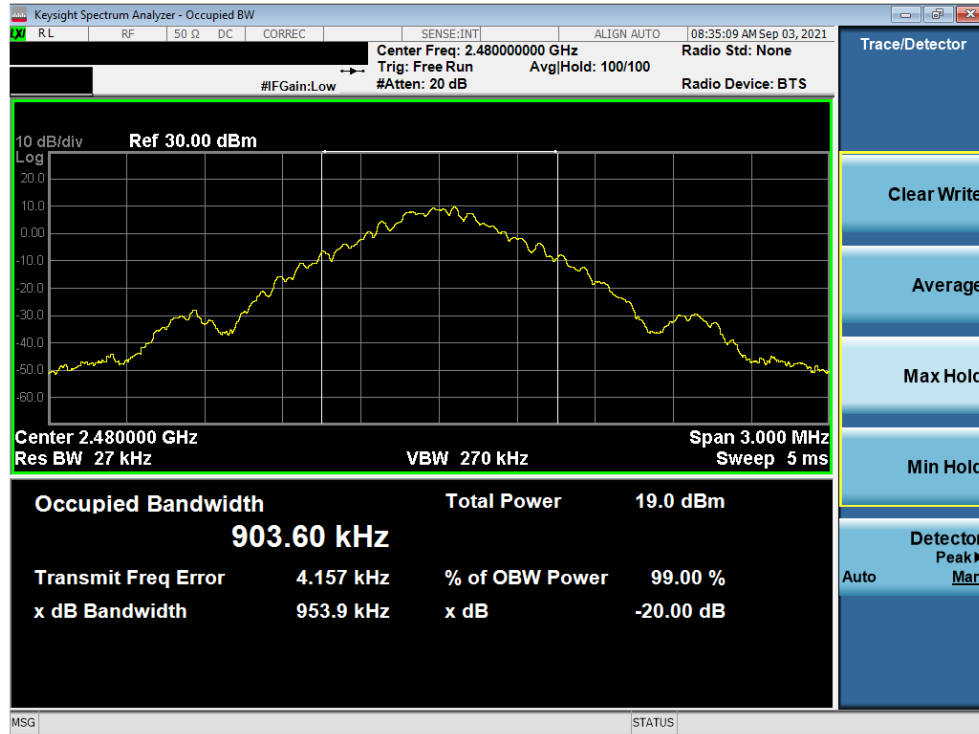
Plot 7-3. Conducted 20dB and 99% OBW Plot (Bluetooth, GFSK – Ch. 78)
