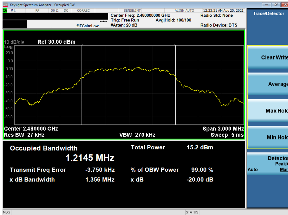
Plot 7-6. Conducted 20dB and 99% OBW Plot (Bluetooth, 8DPSK – Ch. 78)
