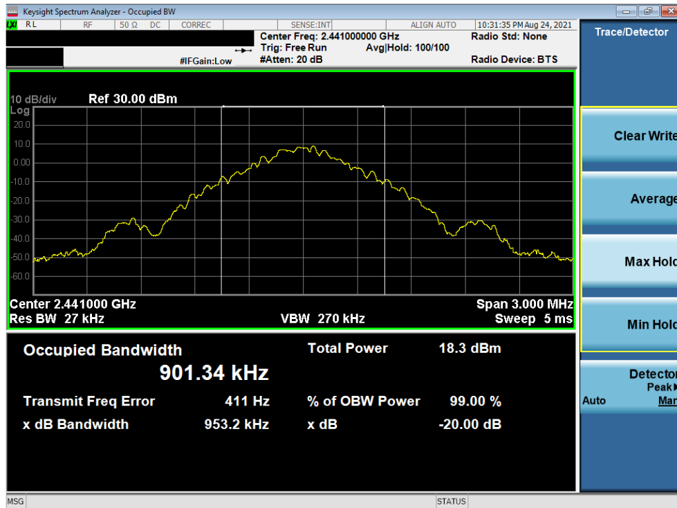
Plot 7-2. Conducted 20dB and 99% OBW Plot (Bluetooth, GFSK – Ch. 39)
