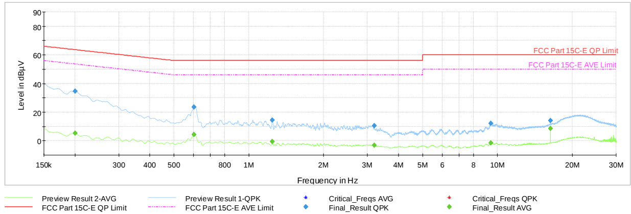
Plot 7-39. AC Line-Conducted Emissions (L1, GFSK – Ch.39 with charging case powered by Host PC via USB-C cable)
