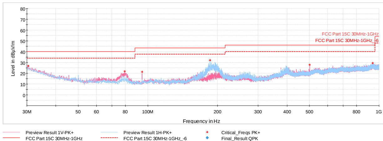
Plot 7-38. Radiated Spurious Emissions below 1GHz (GFSK – Ch.39, Pol. H & V, with charging case powered by Host PC via USB-C cable)
