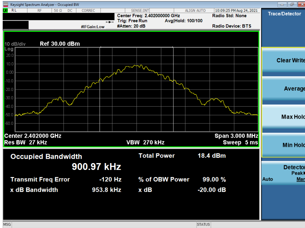
Plot 7-1. Conducted 20dB and 99% OBW Plot (Bluetooth, GFSK – Ch. 0)
