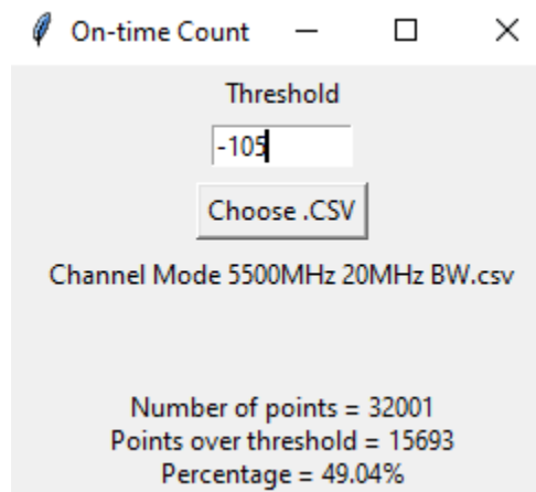
Figure 9-20. 5500MHz - Channel Loading Calculation - Mode 4 (20MHz)
