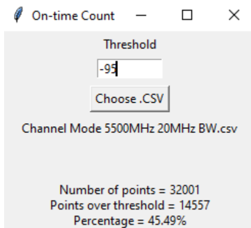
Figure 9-14. 5500MHz - Channel Loading Calculation - Mode 3 (20MHz)
