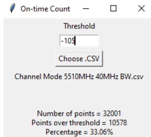
Figure 9-16. 5510MHz - Channel Loading Calculation - Mode 3 (40MHz)
