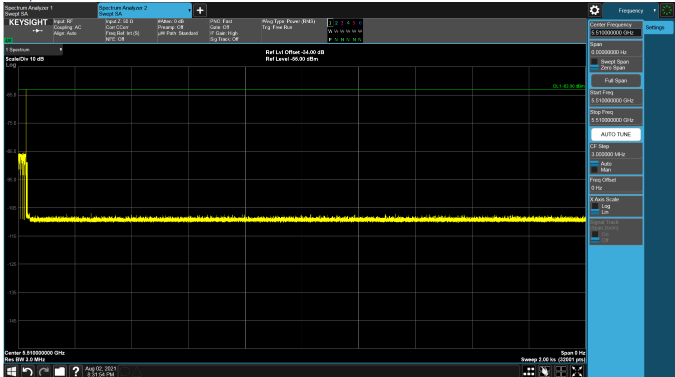
Figure 9-47. 5510MHz - Non-Occupancy Period (30 Minutes) - Mode 4 (40MHz)
