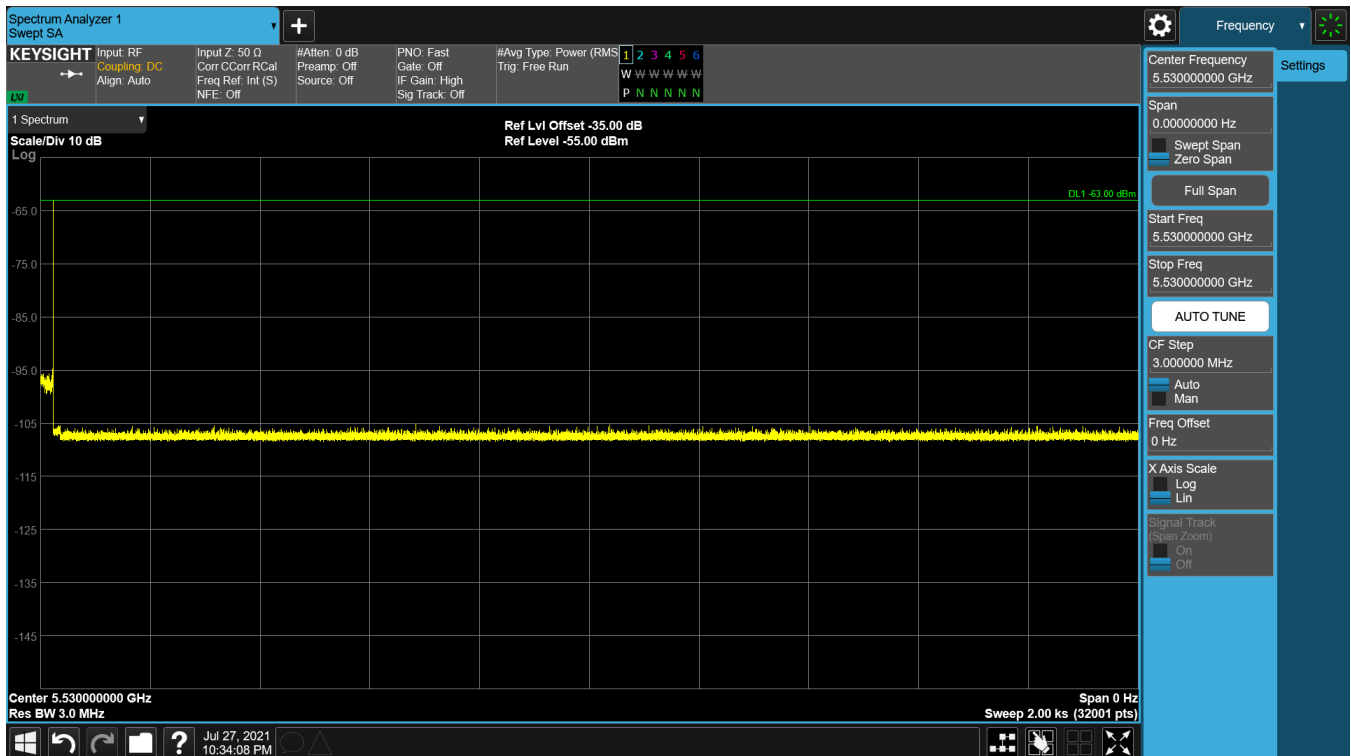
Figure 9-39. 5530MHz - Non-Occupancy Period (30 Minutes) - Mode 1 (80MHz)
