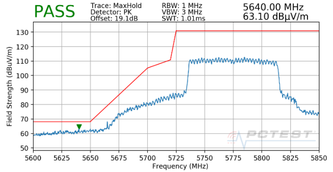
Plot 7-1869. CDD (Pk, Ch.155, 802.11ax(SU), MCS2)
