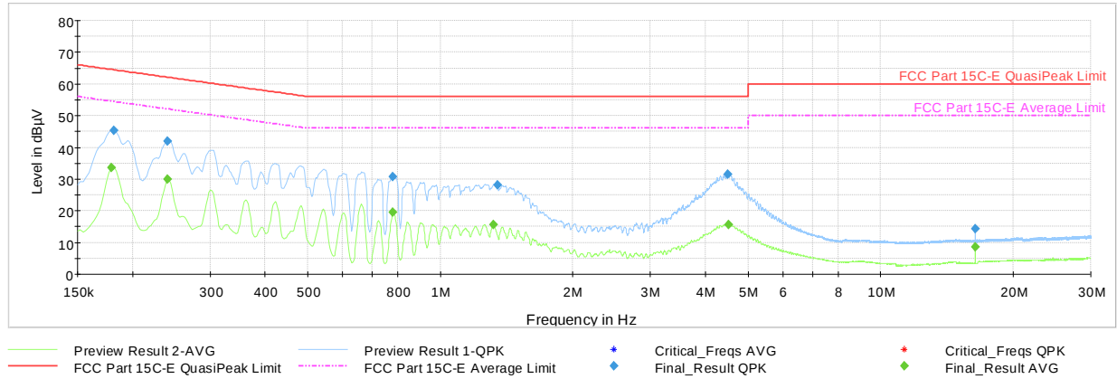
Plot 7-1879. AC Line Conducted Plot with 802.11n CDD/SDM Primary – Ch.36 (L1), with AC/DC adapter
