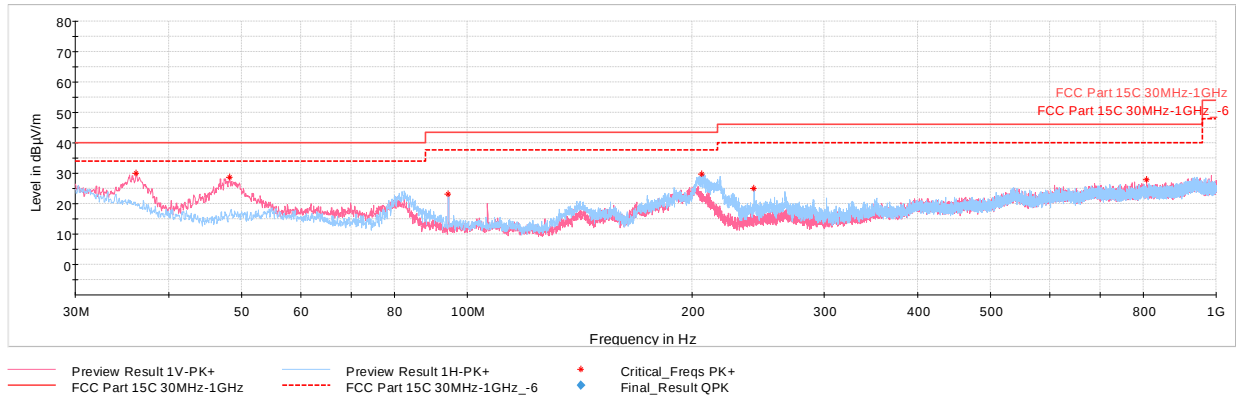
Plot 7-1875. Radiated Spurious Emissions below 1GHz CDD/SDM Primary, 802.11n, Ch.36 with AC/DC Adapter
