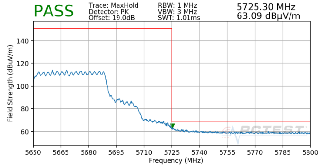
Plot 7-1824. CDD (Pk, Ch.134, 802.11ax(SU), MCS2)
