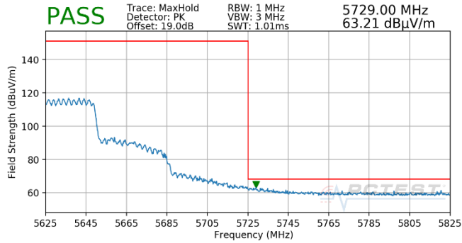
Plot 7-1821. (FCC Only) CDD (Pk, Ch.126, 802.11ax(SU), MCS2)
