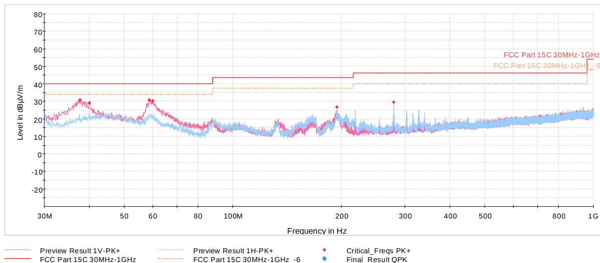
Plot 7-1876. Radiated Spurious Emissions below 1GHz CDD/SDM Primary, 802.11ax (SU), Ch.36 with AC/DC Adapter
