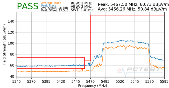
Plot 7-1840. CDD (Pk & Avg, Ch.106, 802.11ac, MCS3)
