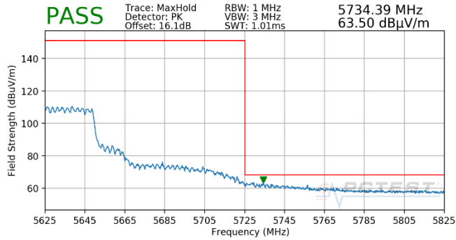
Plot 7-1866. (FCC Only) CDD (Pk, Ch.122, 802.11ax(SU), MCS2)
