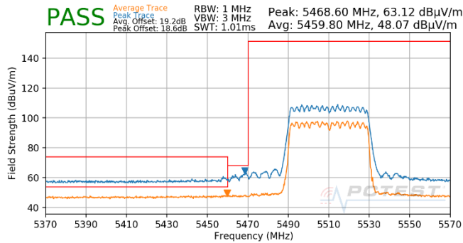
Plot 7-1811. CDD (Pk & Avg, Ch.102, 802.11ax(SU), MCS5)
