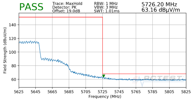
Plot 7-1822. (FCC Only) CDD (Pk, Ch.126, 802.11ax(SU), MCS3)
