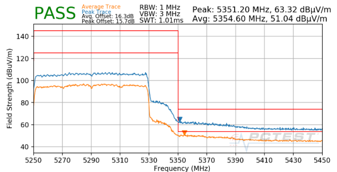
Plot 7-1858. CDD (Pk & Avg, Ch.58, 802.11ax(SU), MCS3)
