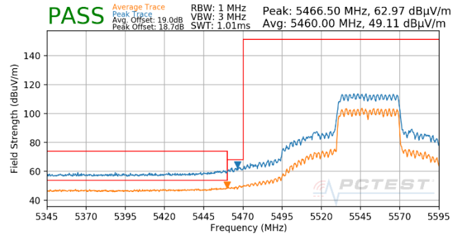
Plot 7-1812. CDD (Pk & Avg, Ch.110, 802.11ax(SU), MCS2)
