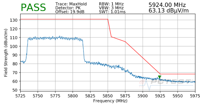
Plot 7-1874. CDD (Pk, Ch.155, 802.11ax(SU), MCS5)
