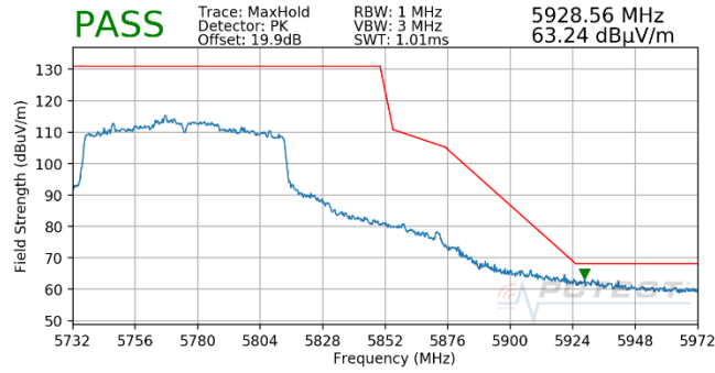
Plot 7-1851. CDD (Pk, Ch.155, 802.11ac, MCS2)
