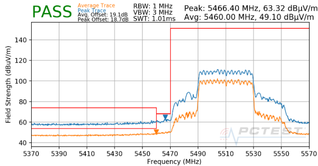
Plot 7-1810. CDD (Pk & Avg, Ch.102, 802.11ax(SU), MCS3)
