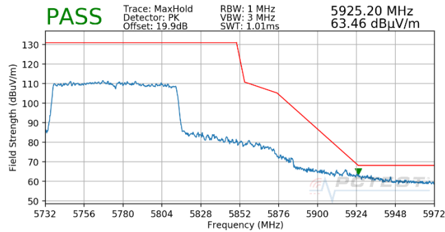
Plot 7-1853. CDD (Pk, Ch.155, 802.11ac, MCS5)
