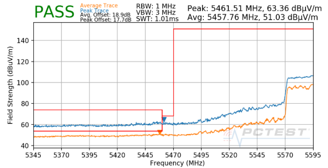
Plot 7-1844. (FCC Only) CDD (Pk & Avg, Ch.122, 802.11ac, MCS5)
