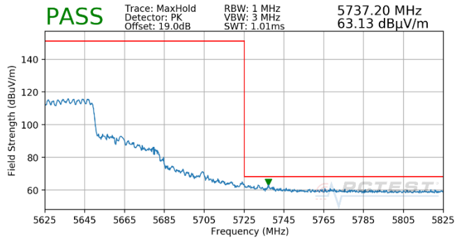
Plot 7-1823. (FCC Only) CDD (Pk, Ch.126, 802.11ax(SU), MCS5)
