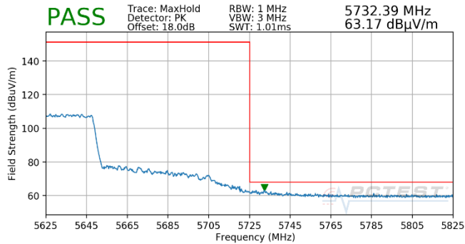
Plot 7-1847. (FCC Only) CDD (Pk, Ch.122, 802.11ac, MCS5)
