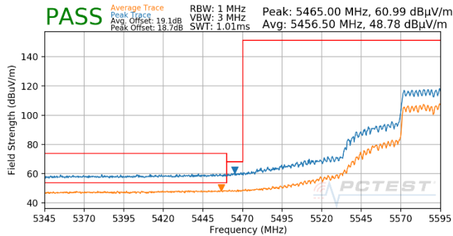
Plot 7-1816. (FCC Only) CDD (Pk & Avg, Ch.118, 802.11ax(SU), MCS3)
