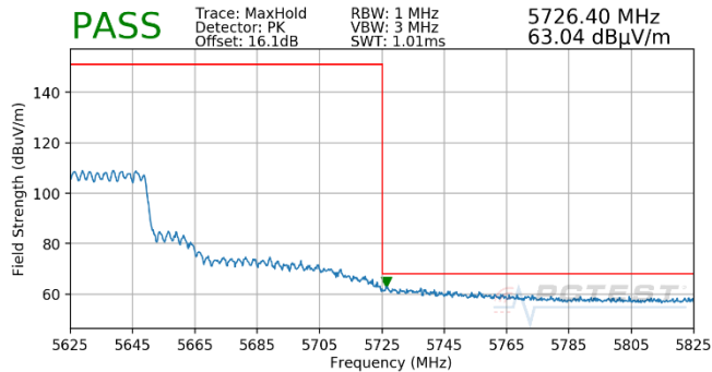
Plot 7-1867. (FCC Only) CDD (Pk, Ch.122, 802.11ax(SU), MCS3)
