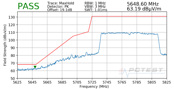
Plot 7-1850. CDD (Pk, Ch.155, 802.11ac, MCS5)
