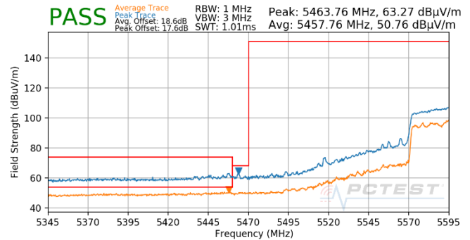
Plot 7-1843. (FCC Only) CDD (Pk & Avg, Ch.122, 802.11ac, MCS3)
