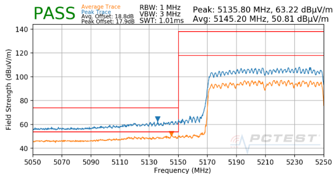
Plot 7-1856. CDD (Pk & Avg, Ch.42, 802.11ax(SU), MCS5)
