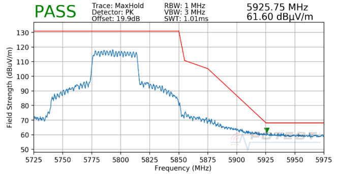
Plot 7-1830. CDD (Pk, Ch.159, 802.11ax(SU), MCS2)
