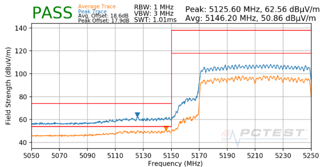
Plot 7-1855. CDD (Pk & Avg, Ch.42, 802.11ax(SU), MCS3)
