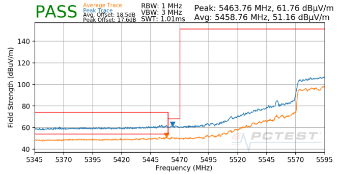
Plot 7-1842. (FCC Only) CDD (Pk & Avg, Ch.122, 802.11ac, MCS2)
