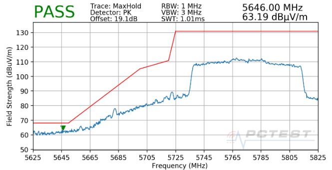
Plot 7-1849. CDD (Pk, Ch.155, 802.11ac, MCS3)
