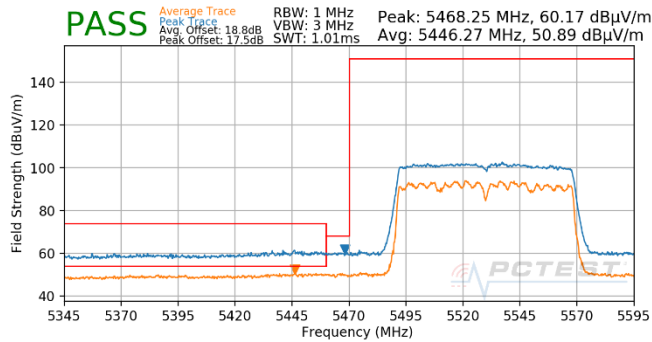
Plot 7-1841. CDD (Pk & Avg, Ch.106, 802.11ac, MCS5)
