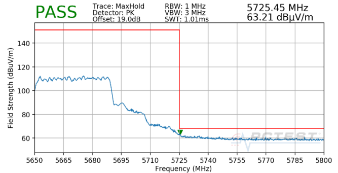
Plot 7-1825. CDD (Pk, Ch.134, 802.11ax(SU), MCS3)
