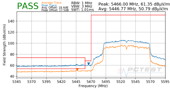
Plot 7-1839. CDD (Pk & Avg, Ch.106, 802.11ac, MCS2)
