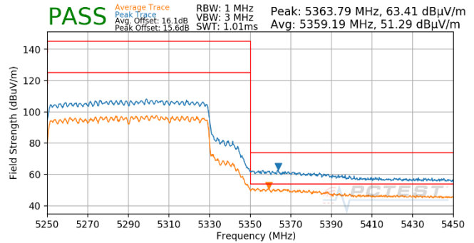
Plot 7-1857. CDD (Pk & Avg, Ch.58, 802.11ax(SU), MCS2)
