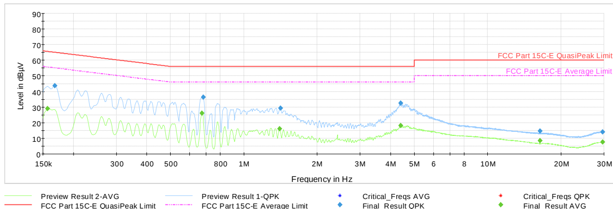
Plot 7-1880. AC Line Conducted Plot with 802.11n CDD/SDM Primary – Ch.36 (N), with AC/DC adapter
