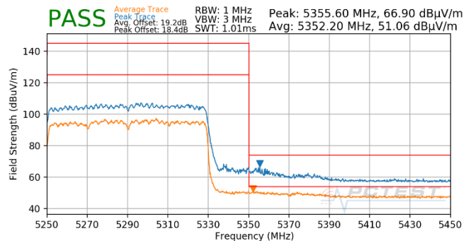
Plot 7-1859. CDD (Pk & Avg, Ch.58, 802.11ax(SU), MCS5)
