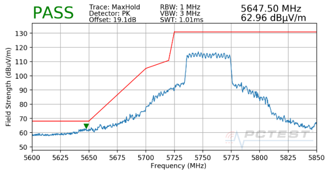
Plot 7-1829. CDD (Pk, Ch.151, 802.11ax(SU), MCS5)
