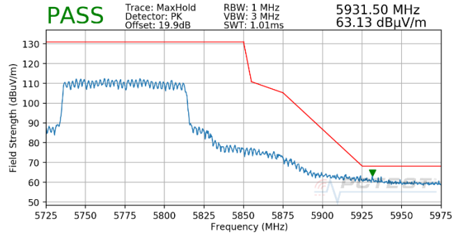
Plot 7-1872. CDD (Pk, Ch.155, 802.11ax(SU), MCS2)
