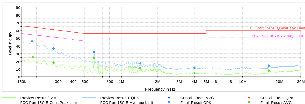
Plot 7-1882. AC Line Conducted Plot with 802.11ax (SU) CDD/SDM Primary – Ch.36 (N), with Laptop
