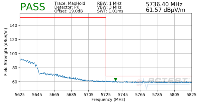
Plot 7-1818. (FCC Only) CDD (Pk, Ch.118, 802.11ax(SU), MCS2)
