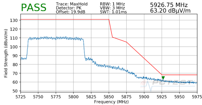
Plot 7-1873. CDD (Pk, Ch.155, 802.11ax(SU), MCS3)
