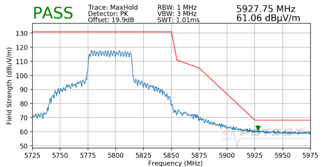
Plot 7-1831. CDD (Pk, Ch.159, 802.11ax(SU), MCS3)
