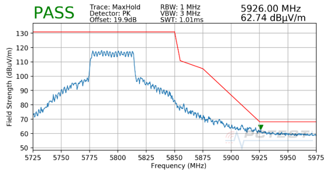
Plot 7-1832. CDD (Pk, Ch.159, 802.11ax(SU), MCS5)
