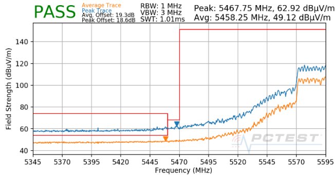
Plot 7-1817. (FCC Only) CDD (Pk & Avg, Ch.118, 802.11ax(SU), MCS5)
