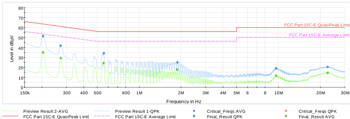
Plot 7-1883. AC Line Conducted Plot with 802.11n CDD/SDM Diversity – Ch.36 (L1), with Laptop
