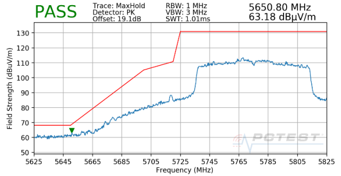
Plot 7-1848. CDD (Pk, Ch.155, 802.11ac, MCS2)
