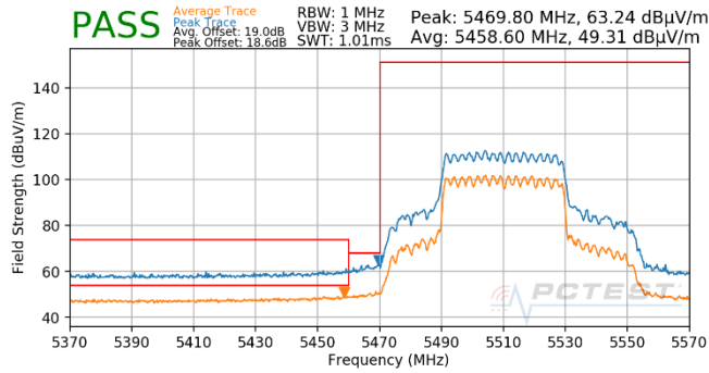
Plot 7-1809. CDD (Pk & Avg, Ch.102, 802.11ax(SU), MCS2)
