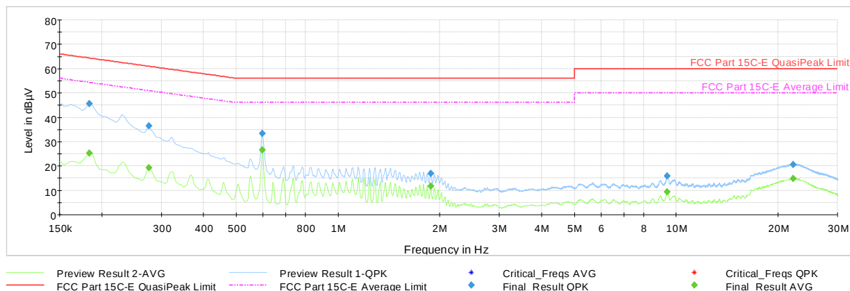
Plot 7-1881. AC Line Conducted Plot with 802.11ax (SU) CDD/SDM Primary – Ch.36 (L1), with Laptop
