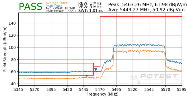
Plot 7-1860. CDD (Pk & Avg, Ch.106, 802.11ax(SU), MCS2)
