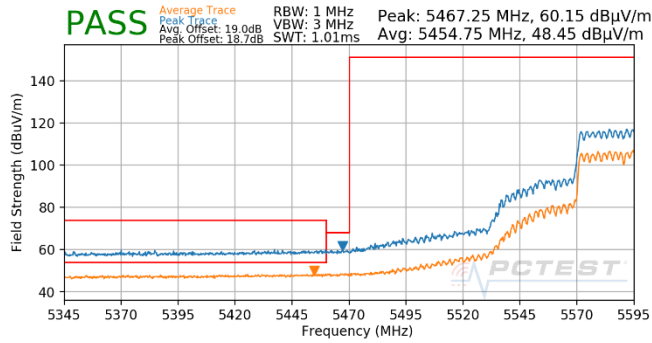
Plot 7-1815. (FCC Only) CDD (Pk & Avg, Ch.118, 802.11ax(SU), MCS2)
