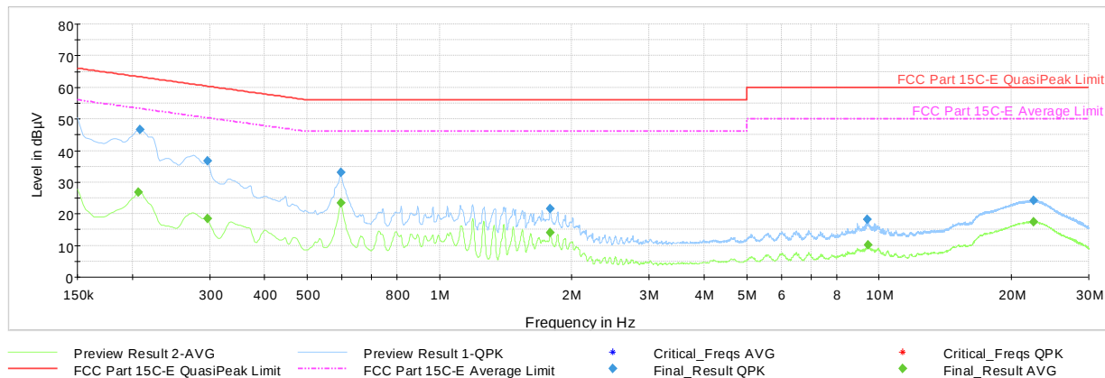
Plot 7-1885. AC Line Conducted Plot with 802.11ax (SU) CDD/SDM Diversity – Ch.36 (L1), with Laptop
