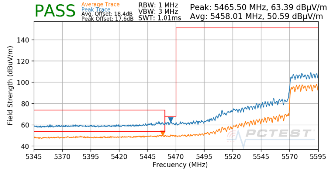
Plot 7-1864. (FCC Only) CDD (Pk & Avg, Ch.122, 802.11ax(SU), MCS3)
