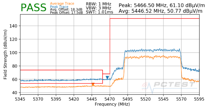
Plot 7-1861. CDD (Pk & Avg, Ch.106, 802.11ax(SU), MCS3)
