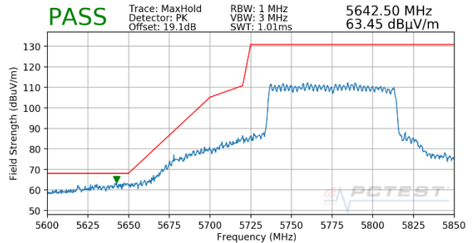
Plot 7-1870. CDD (Pk, Ch.155, 802.11ax(SU), MCS3)
