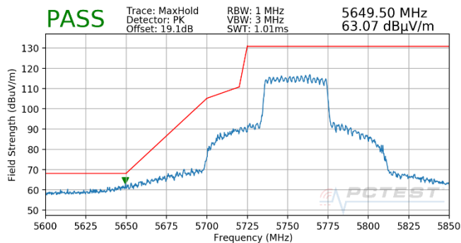
Plot 7-1828. CDD (Pk, Ch.151, 802.11ax(SU), MCS3)
