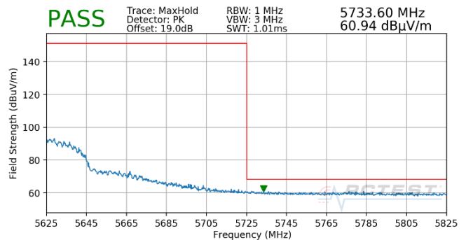
Plot 7-1819. (FCC Only) CDD (Pk, Ch.118, 802.11ax(SU), MCS3)
