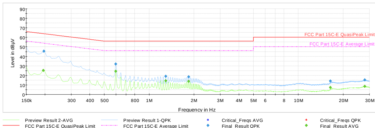
Plot 7-1886. AC Line Conducted Plot with 802.11ax (SU) CDD/SDM Diversity – Ch.36 (N), with Laptop
