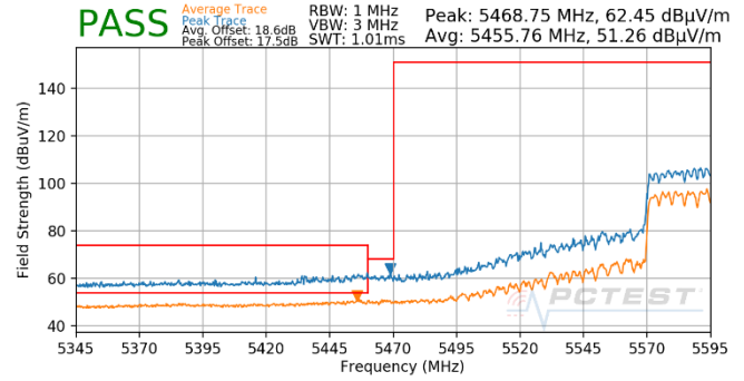
Plot 7-1865. (FCC Only) CDD (Pk & Avg, Ch.122, 802.11ax(SU), MCS5)
