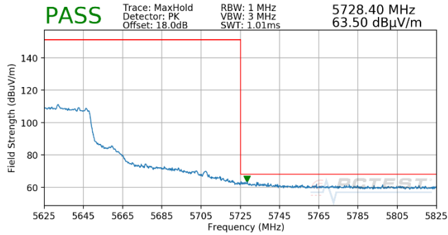
Plot 7-1845. (FCC Only) CDD (Pk, Ch.122, 802.11ac, MCS2)
