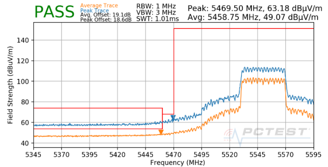
Plot 7-1813. CDD (Pk & Avg, Ch.110, 802.11ax(SU), MCS3)
