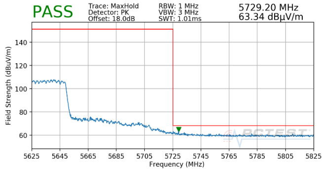
Plot 7-1868. (FCC Only) CDD (Pk, Ch.122, 802.11ax(SU), MCS5)
