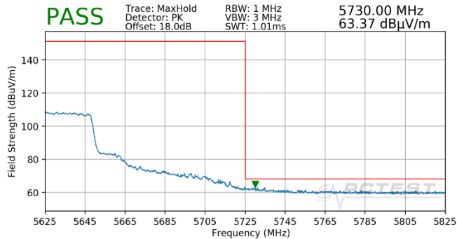
Plot 7-1846. (FCC Only) CDD (Pk, Ch.122, 802.11ac, MCS3)
