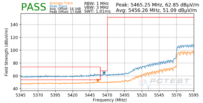
Plot 7-1863. (FCC Only) CDD (Pk & Avg, Ch.122, 802.11ax(SU), MCS2)
