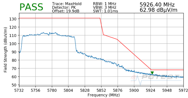
Plot 7-1852. CDD (Pk, Ch.155, 802.11ac, MCS3)
