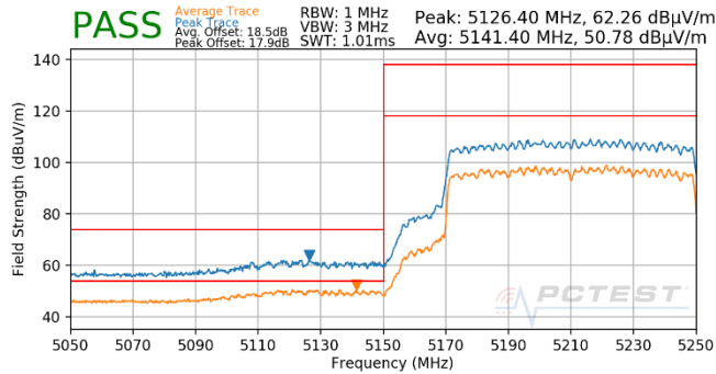
Plot 7-1854. CDD (Pk & Avg, Ch.42, 802.11ax(SU), MCS2)
