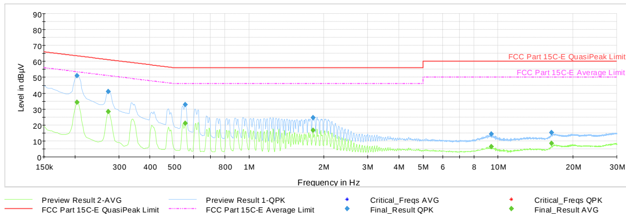
Plot 7-1884. AC Line Conducted Plot with 802.11n CDD/SDM Diversity – Ch.36 (N), with Laptop
