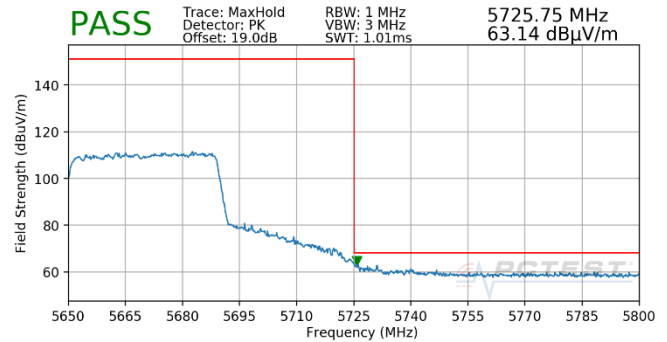
Plot 7-1826. CDD (Pk, Ch.134, 802.11ax(SU), MCS5)
