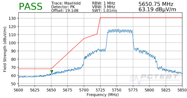
Plot 7-1827. CDD (Pk, Ch.151, 802.11ax(SU), MCS2)
