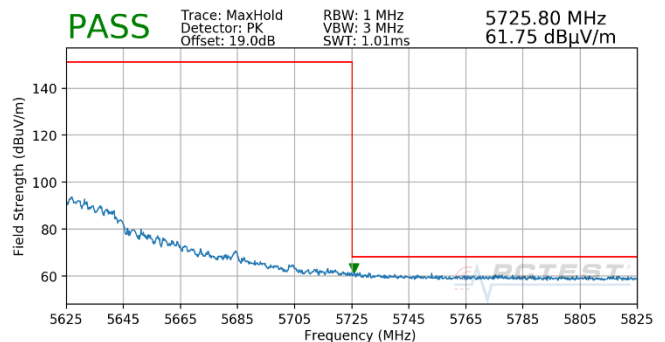
Plot 7-1820. (FCC Only) CDD (Pk, Ch.118, 802.11ax(SU), MCS5)
