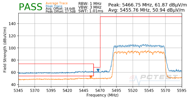
Plot 7-1862. CDD (Pk & Avg, Ch.106, 802.11ax(SU), MCS5)
