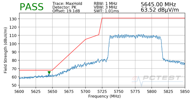
Plot 7-1871. CDD (Pk, Ch.155, 802.11ax(SU), MCS5)
