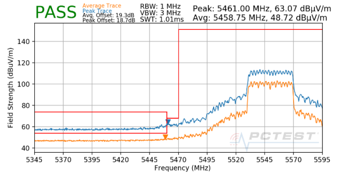
Plot 7-1814. CDD (Pk & Avg, Ch.110, 802.11ax(SU), MCS5)
