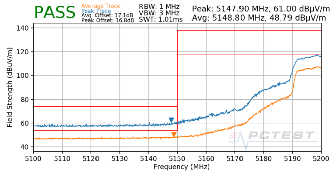
Plot 7-1710. SDM (Pk & Avg, Ch.40, 802.11n, MCS11)
