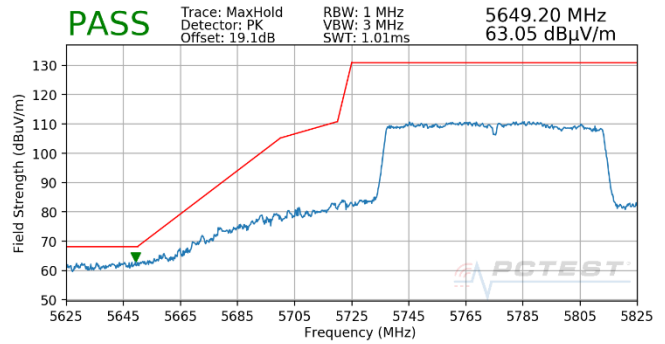
Plot 7-1682. CDD (Pk, Ch.155, 802.11ac, MCS5)
