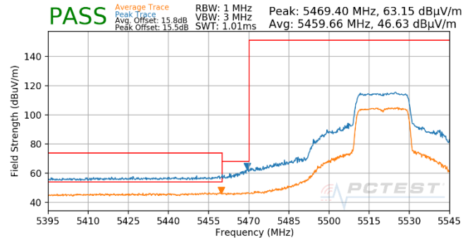
Plot 7-1410. Antenna 1b (Pk & Avg, Ch.104, 802.11ax(SU), MCS5)
