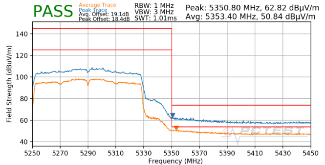
Plot 7-1321. Antenna 3b (Pk & Avg, Ch.58, 802.11ac, MCS3)
