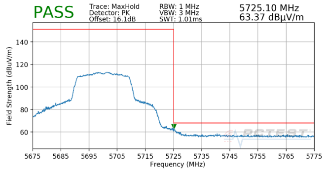
Plot 7-1240. Antenna 3b (Pk, Ch.140, 802.11ax(SU), MCS2)
