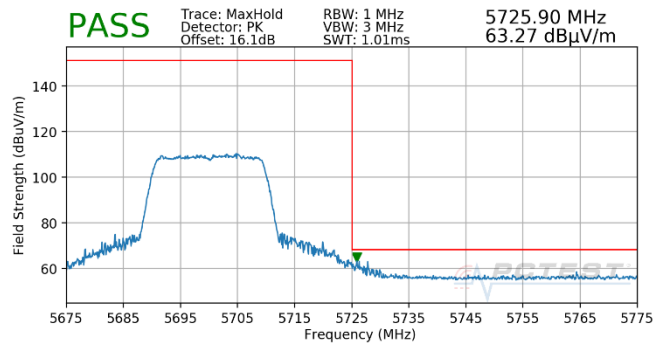
Plot 7-1242. Antenna 3b (Pk, Ch.140, 802.11ax(SU), MCS5)
