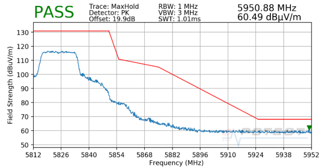
Plot 7-1212. Antenna 3b (Pk, Ch.165, 802.11n, MCS5)
