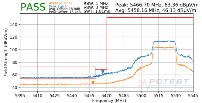
Plot 7-1230. Antenna 3b (Pk & Avg, Ch.104, 802.11ax(SU), MCS5)
