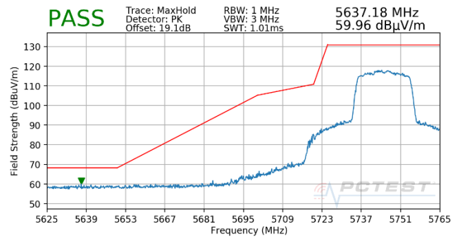
Plot 7-1063. Antenna 5T (Pk, Ch.149, 802.11ax(SU), MCS2)
