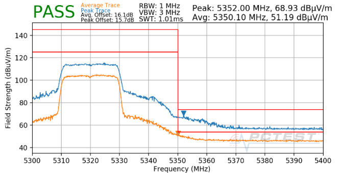
Plot 7-1044. Antenna 5T (Pk & Avg, Ch.64, 802.11ax(SU), MCS5)
