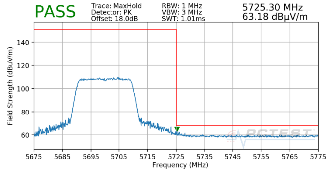
Plot 7-1062. Antenna 5T (Pk, Ch.140, 802.11ax(SU), MCS5)
