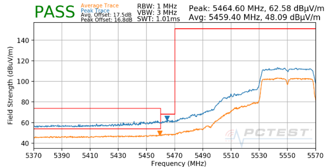
Plot 7-1086. Antenna 5T (Pk & Avg, Ch.110, 802.11n, MCS5)
