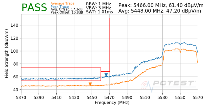
Plot 7-1085. Antenna 5T (Pk & Avg, Ch.110, 802.11n, MCS3)
