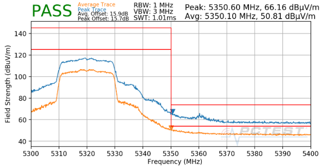
Plot 7-1043. Antenna 5T (Pk & Avg, Ch.64, 802.11ax(SU), MCS3)
