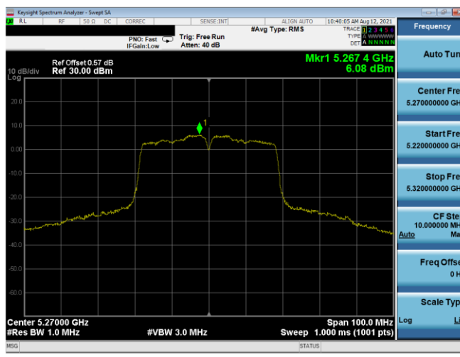
Plot 7-720. PSD SDM Antenna 1b (40MHz BW 802.11n - Ch. 54, MCS11)
