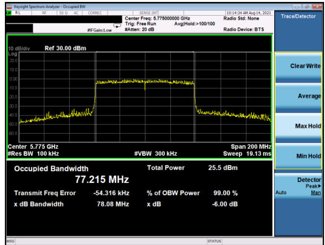
Plot 7-216. 6dB BW & 99% OBW Antenna 1b (80MHz BW 802.11ax(SU) - Ch. 155, MCS5)
