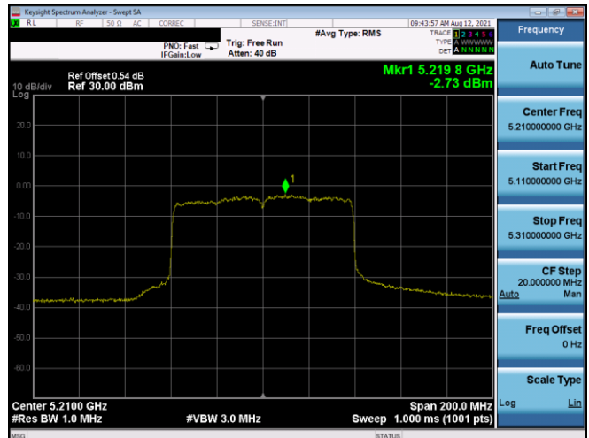
Plot 7-222. PSD Antenna 5T (80MHz BW 802.11ax(SU) – Ch. 42, MCS2)
