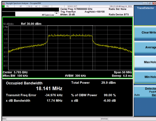
Plot 7-193. 6dB BW & 99% OBW Antenna 3b (20MHz BW 802.11n - Ch. 157, MCS5)
