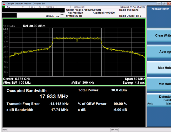
Plot 7-175. 6dB BW & 99% OBW Antenna 5T (20MHz BW 802.11n – Ch. 157, MCS5)
