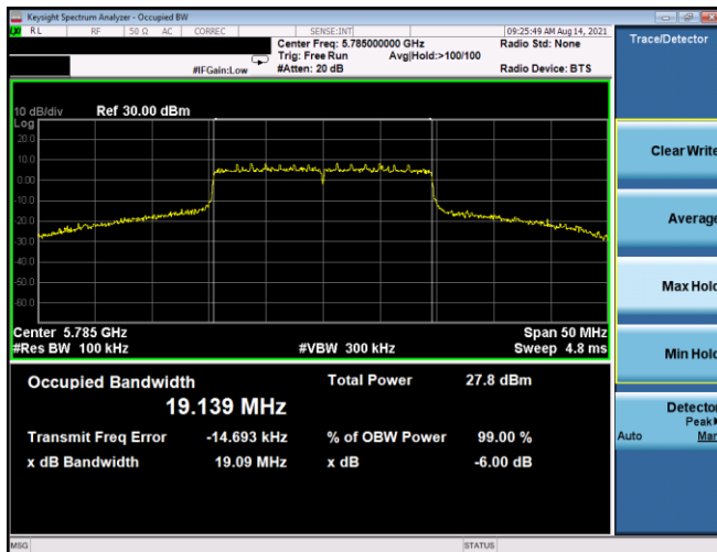
Plot 7-194. 6dB BW & 99% OBW Antenna 3b (20MHz BW 802.11ax(SU) - Ch. 157, MCS5)
