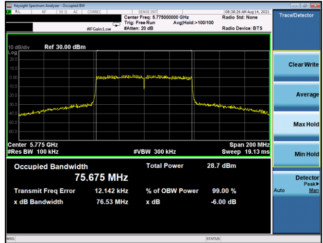
Plot 7-179. 6dB BW & 99% OBW Antenna 5T (80MHz BW 802.11ac – Ch. 155, MCS5)
