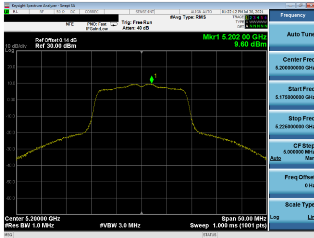
Plot 7-217. PSD Antenna 5T (20MHz BW 802.11n – Ch. 40, MCS2)
