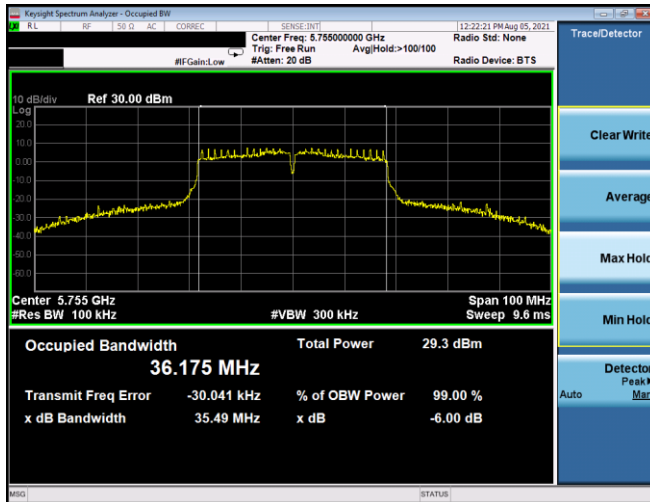
Plot 7-201. 6dB BW & 99% OBW Antenna 1b (40MHz BW 802.11n – Ch. 151, MCS2)
