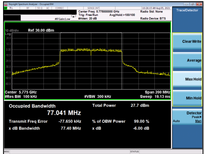
Plot 7-186. 6dB BW & 99% OBW Antenna 3b (80MHz BW 802.11ax(SU) – Ch. 155, MCS2)
