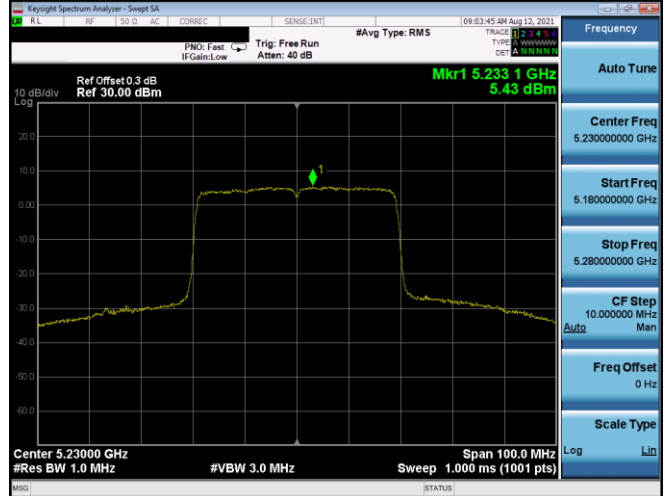
Plot 7-220. PSD Antenna 5T (40MHz BW 802.11ax(SU) – Ch. 46, MCS2)
