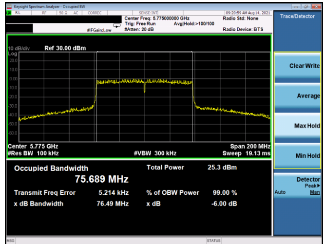
Plot 7-197. 6dB BW & 99% OBW Antenna 3b (80MHz BW 802.11ac - Ch. 155, MCS5)
