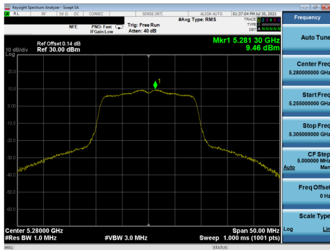
Plot 7-223. PSD Antenna 5T (20MHz BW 802.11n – Ch. 56, MCS2)
