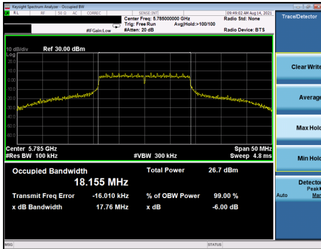
Plot 7-211. 6dB BW & 99% OBW Antenna 1b (20MHz BW 802.11n - Ch. 157, MCS5)
