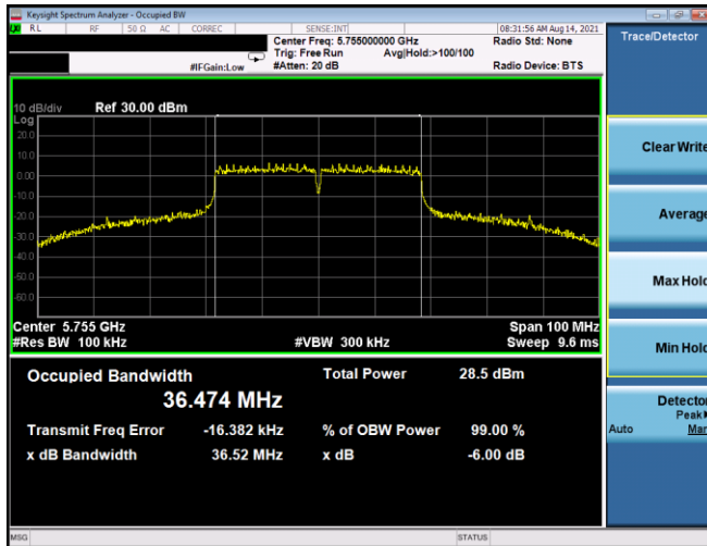
Plot 7-177. 6dB BW & 99% OBW Antenna 5T (40MHz BW 802.11n – Ch. 151, MCS5)
