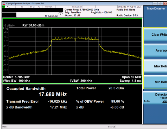
Plot 7-181. 6dB BW & 99% OBW Antenna 3b (20MHz BW 802.11n – Ch. 157, MCS2)
