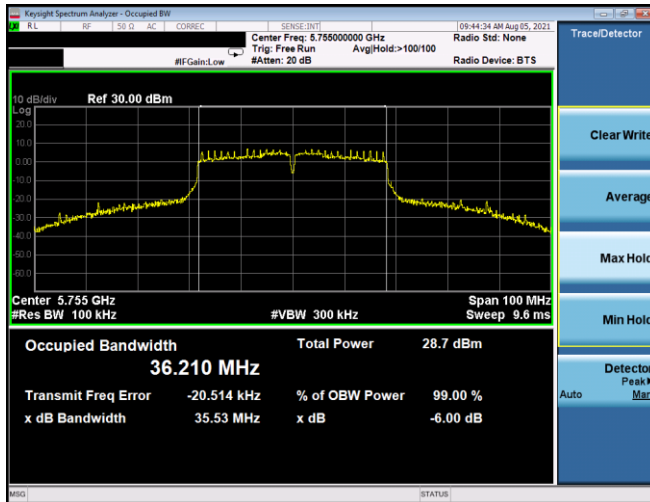
Plot 7-183. 6dB BW & 99% OBW Antenna 3b (40MHz BW 802.11n – Ch. 151, MCS2)
