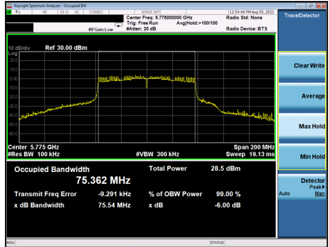
Plot 7-203. 6dB BW & 99% OBW Antenna 1b (80MHz BW 802.11ac – Ch. 155, MCS2)
