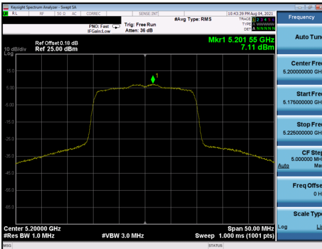
Plot 7-218. PSD Antenna 5T (20MHz BW 802.11ax(SU) – Ch. 40, MCS2)
