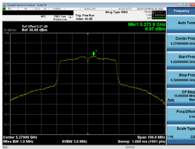
Plot 7-225. PSD Antenna 5T (40MHz BW 802.11n – Ch. 54, MCS2)
