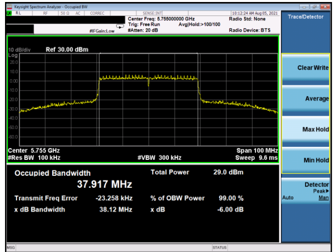
Plot 7-184. 6dB BW & 99% OBW Antenna 3b (40MHz BW 802.11ax(SU) – Ch. 151, MCS2)
