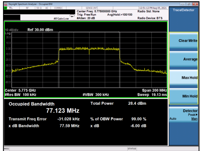
Plot 7-204. 6dB BW & 99% OBW Antenna 1b (80MHz BW 802.11ax(SU) – Ch. 155, MCS2)
