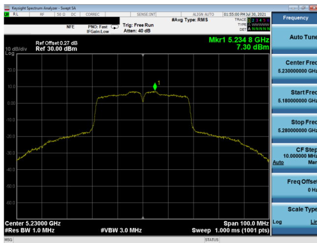
Plot 7-219. PSD Antenna 5T (40MHz BW 802.11n – Ch. 46, MCS2)
