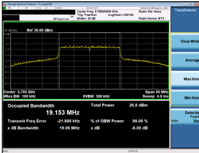
Plot 7-212. 6dB BW & 99% OBW Antenna 1b (20MHz BW 802.11ax(SU) - Ch. 157, MCS5)
