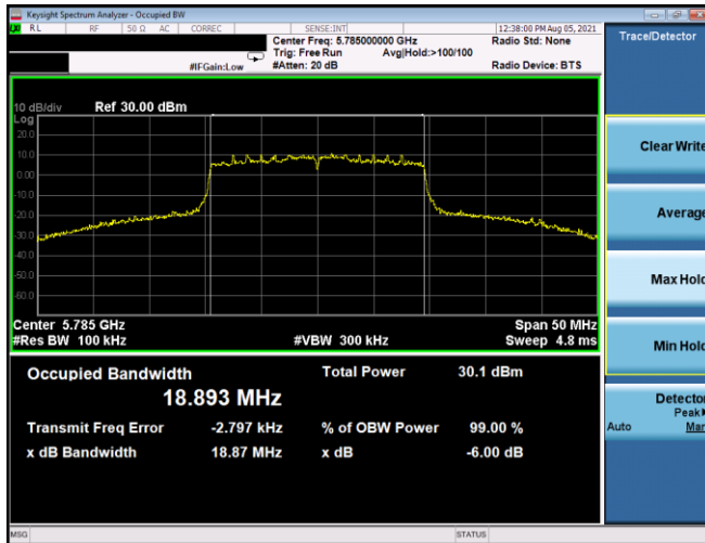
Plot 7-200. 6dB BW & 99% OBW Antenna 1b (20MHz BW 802.11ax(SU) – Ch. 157, MCS2)
