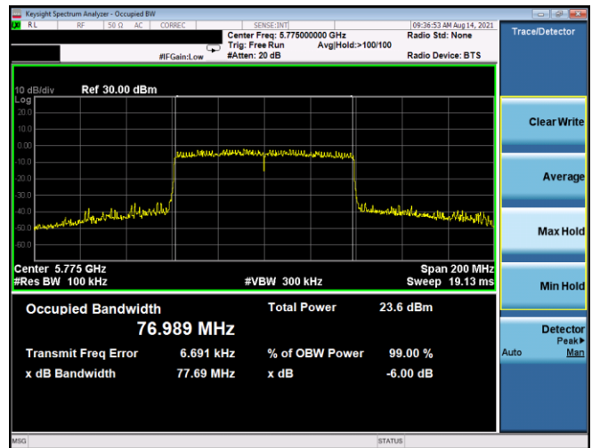
Plot 7-198. 6dB BW & 99% OBW Antenna 3b (80MHz BW 802.11ax(SU) - Ch. 155, MCS5)
