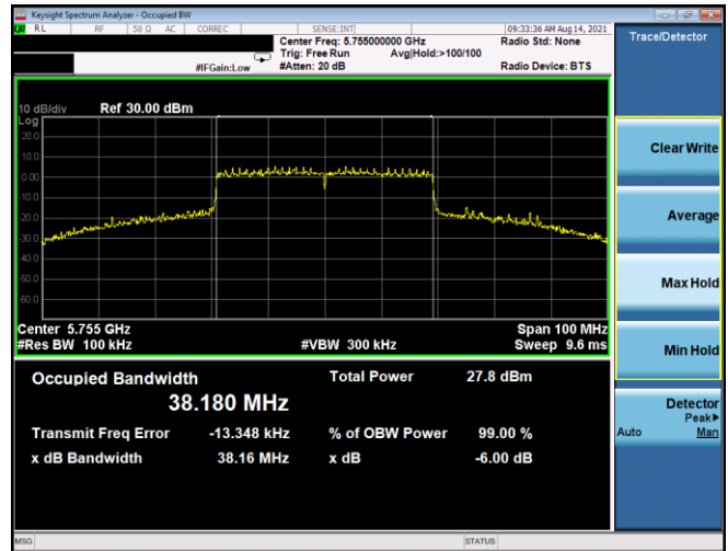
Plot 7-196. 6dB BW & 99% OBW Antenna 3b (40MHz BW 802.11ax(SU) - Ch. 151, MCS5)
