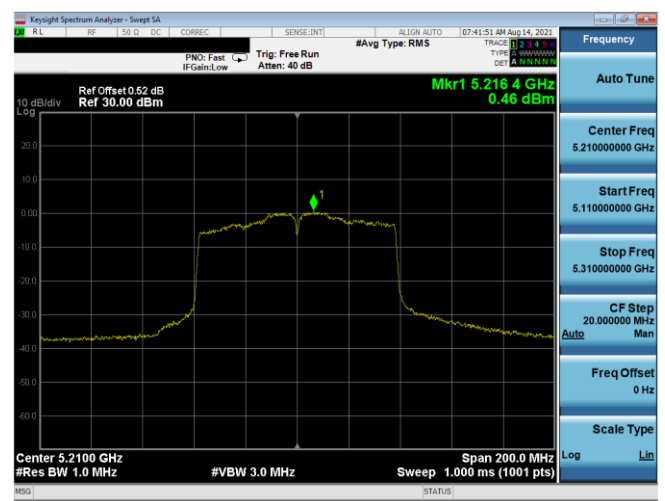
Plot 7-221. PSD Antenna 5T (80MHz BW 802.11ac – Ch. 42, MCS2)
