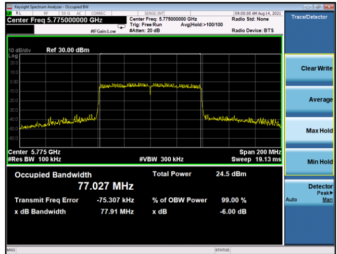
Plot 7-180. 6dB BW & 99% OBW Antenna 5T (80MHz BW 802.11ax(SU) – Ch. 155, MCS5)
