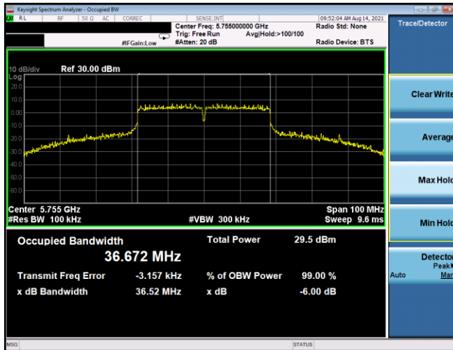
Plot 7-213. 6dB BW & 99% OBW Antenna 1b (40MHz BW 802.11n - Ch. 151, MCS5)
