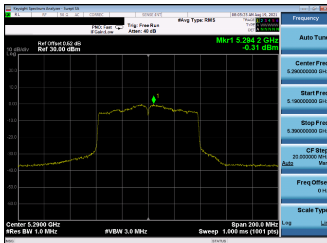
Plot 7-227. PSD Antenna 5T (80MHz BW 802.11ac – Ch. 58, MCS2)
