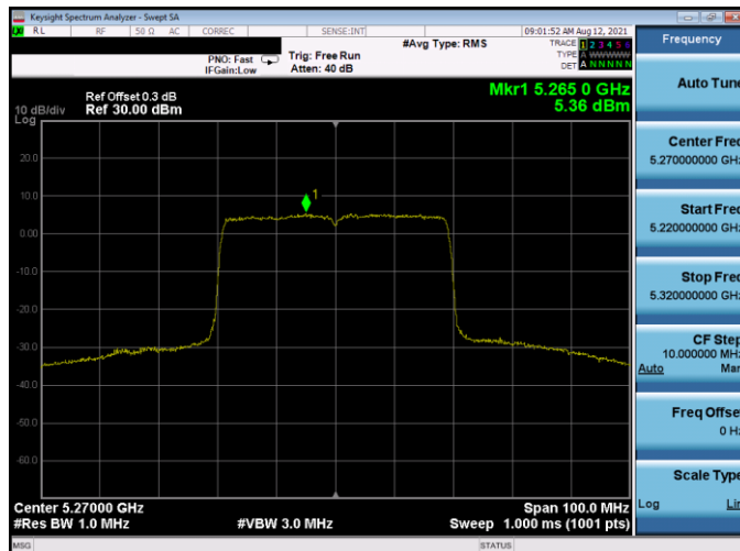
Plot 7-226. PSD Antenna 5T (40MHz BW 802.11ax(SU) – Ch. 54, MCS2)
