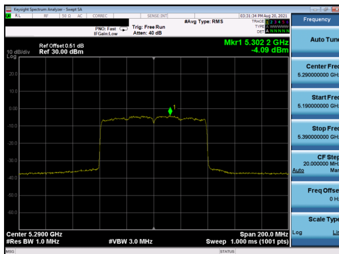
Plot 7-228. PSD Antenna 5T (80MHz BW 802.11ax(SU) – Ch. 58, MCS2)
