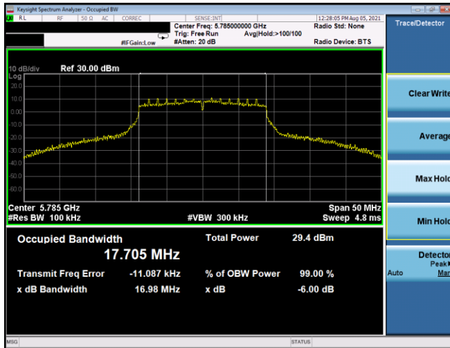
Plot 7-199. 6dB BW & 99% OBW Antenna 1b (20MHz BW 802.11n – Ch. 157, MCS2)
