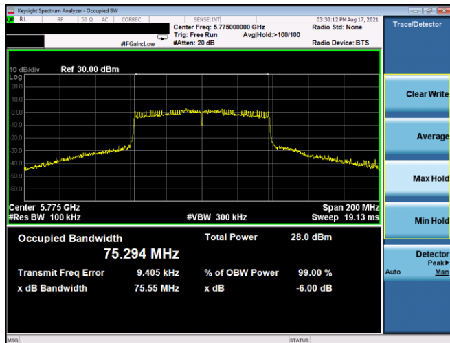
Plot 7-173. 6dB BW & 99% OBW Antenna 5T (80MHz BW 802.11ac – Ch. 155, MCS3)
