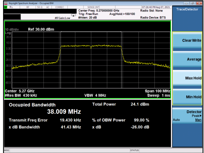
Plot 7-136. 26dB BW & 99% OBW Antenna 1b (40MHz BW 802.11ax(SU) – Ch. 54, MCS3)
