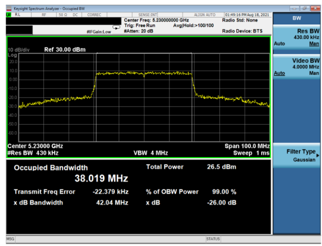
Plot 7-130. 26dB BW & 99% OBW Antenna 1b (40MHz BW 802.11ax(SU) – Ch. 46, MCS3)
