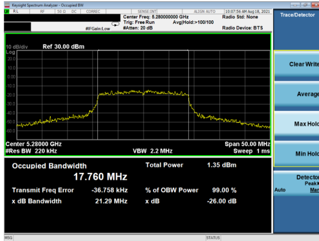
Plot 7-133. 26dB BW & 99% OBW Antenna 1b (20MHz BW 802.11n – Ch. 56, MCS3)
