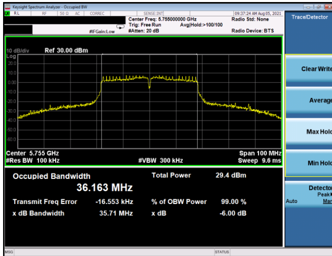
Plot 7-165. 6dB BW & 99% OBW Antenna 5T (40MHz BW 802.11n – Ch. 151, MCS2)
