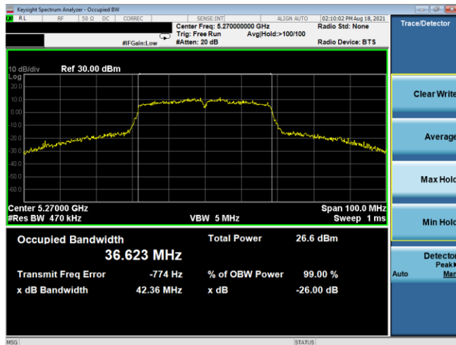
Plot 7-135. 26dB BW & 99% OBW Antenna 1b (40MHz BW 802.11n – Ch. 54, MCS3)
