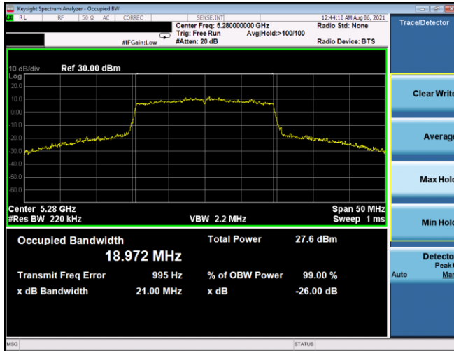
Plot 7-134. 26dB BW & 99% OBW Antenna 1b (20MHz BW 802.11ax(SU) – Ch. 56, MCS3)
