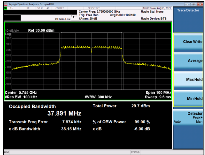
Plot 7-166. 6dB BW & 99% OBW Antenna 5T (40MHz BW 802.11ax(SU) – Ch. 151, MCS2)
