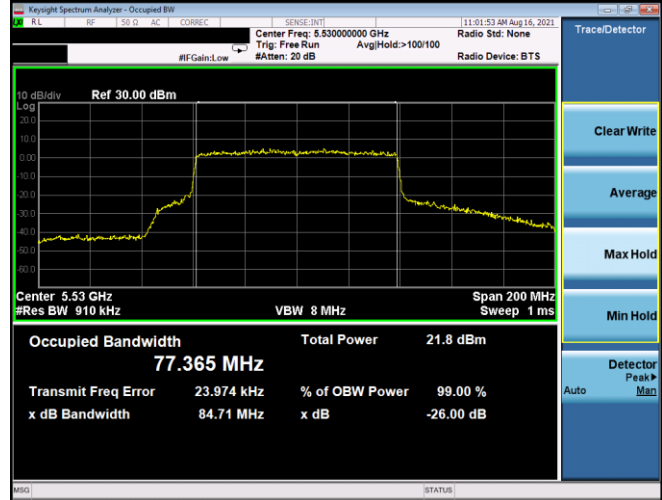
Plot 7-72. 26dB BW & 99% OBW Antenna 3b (80MHz BW 802.11ax(SU) – Ch. 106, MCS2)
