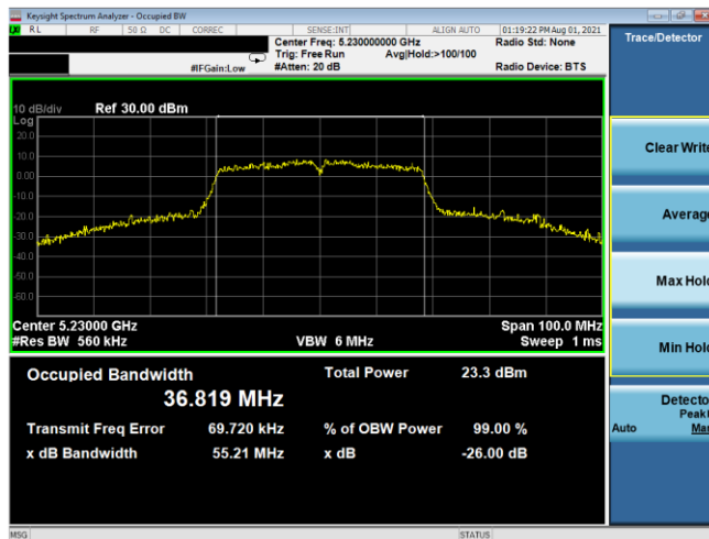
Plot 7-111. 26dB BW & 99% OBW Antenna 1b (40MHz BW 802.11n – Ch. 46, MCS2)
