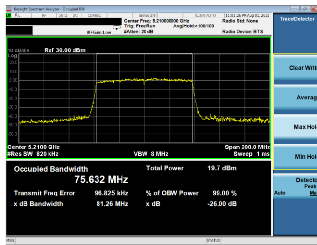
Plot 7-95. 26dB BW & 99% OBW Antenna 3b (80MHz BW 802.11ac – Ch. 42, MCS5)
