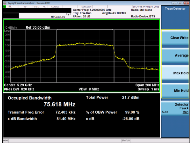
Plot 7-65. 26dB BW & 99% OBW Antenna 3b (80MHz BW 802.11ac – Ch. 58, MCS2)
