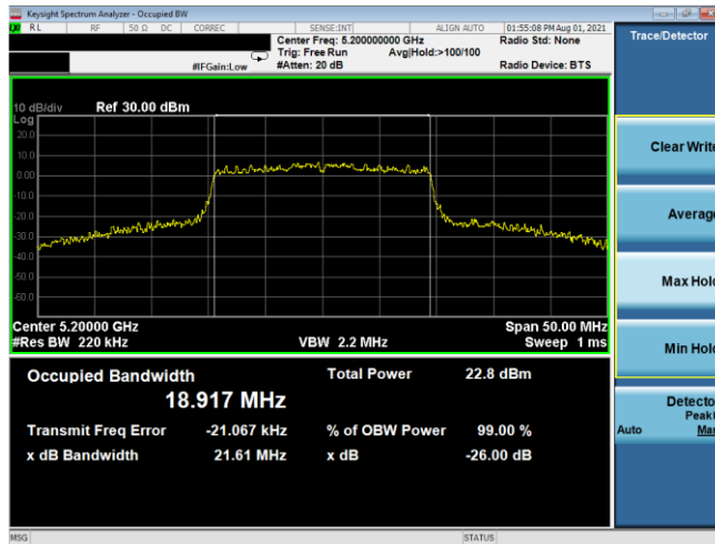
Plot 7-110. 26dB BW & 99% OBW Antenna 1b (20MHz BW 802.11ax(SU) – Ch. 40, MCS2)
