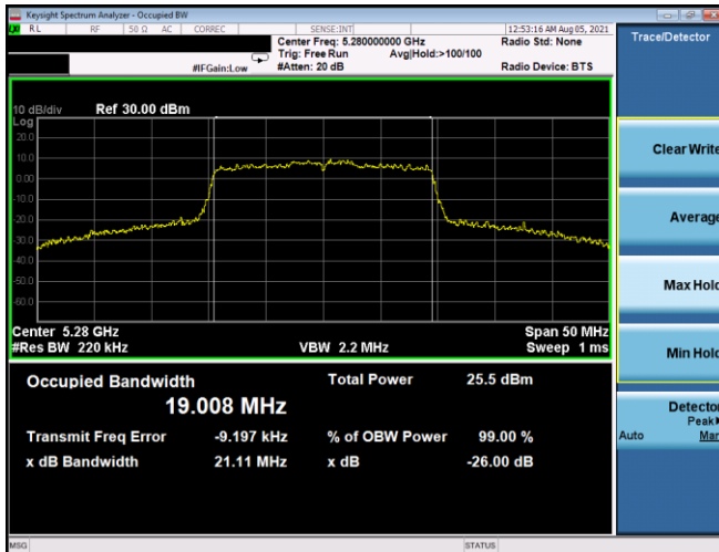
Plot 7-62. 26dB BW & 99% OBW Antenna 3b (20MHz BW 802.11ax(SU) – Ch. 56, MCS2)
