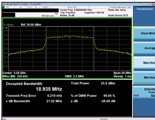
Plot 7-68. 26dB BW & 99% OBW Antenna 3b (20MHz BW 802.11ax(SU) – Ch. 116, MCS2)
