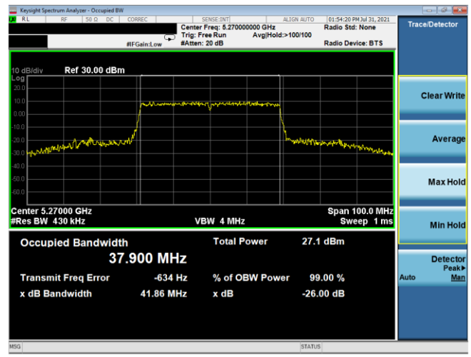
Plot 7-64. 26dB BW & 99% OBW Antenna 3b (40MHz BW 802.11ax(SU) – Ch. 54, MCS2)
