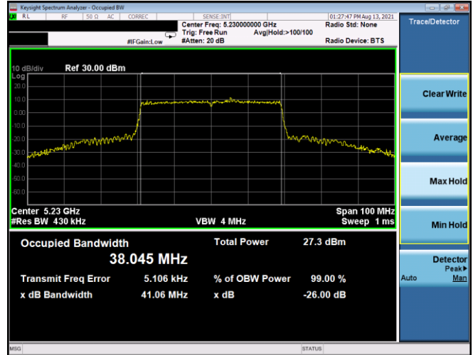
Plot 7-40. 26dB BW & 99% OBW Antenna 5T (40MHz BW 802.11ax(SU) – Ch. 46, MCS5)
