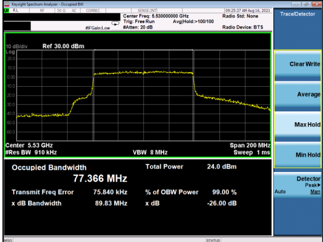
Plot 7-18. 26dB BW & 99% OBW Antenna 5T (80MHz BW 802.11ax(SU) – Ch. 106, MCS2)
