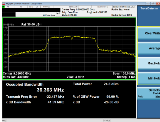
Plot 7-15. 26dB BW & 99% OBW Antenna 5T (40MHz BW 802.11n – Ch. 110, MCS2)
