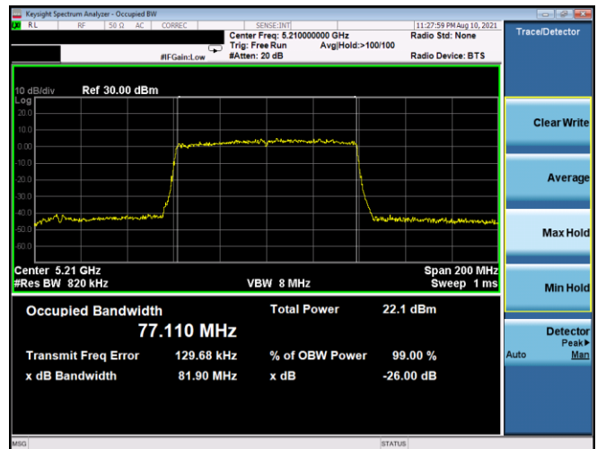
Plot 7-42. 26dB BW & 99% OBW Antenna 5T (80MHz BW 802.11ax(SU) – Ch. 42, MCS5)
