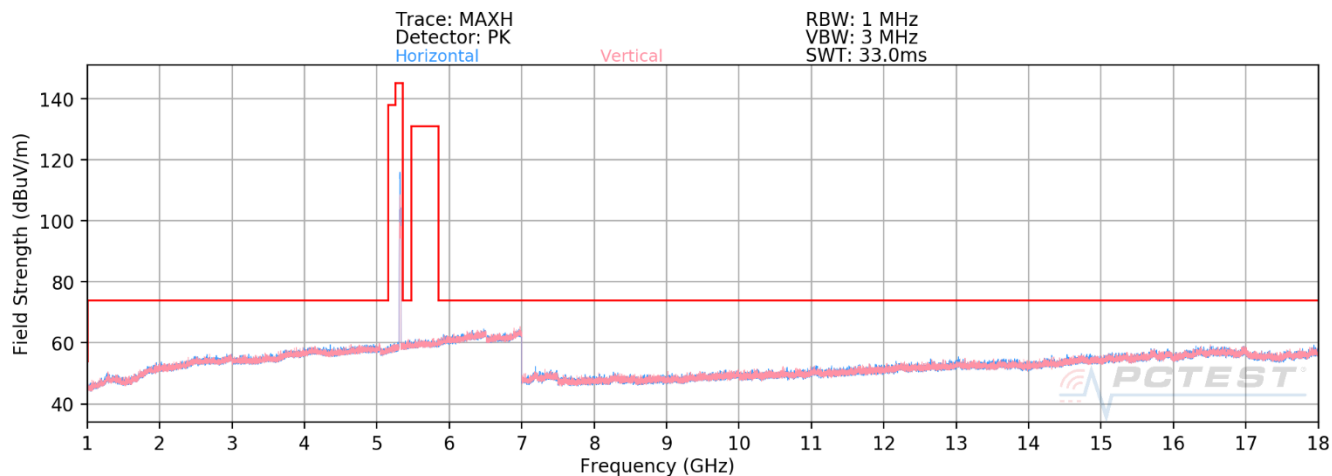
Plot 7-686. RSE above 1GHz SDM Diversity (11ax – Ch.64 – RU26)
