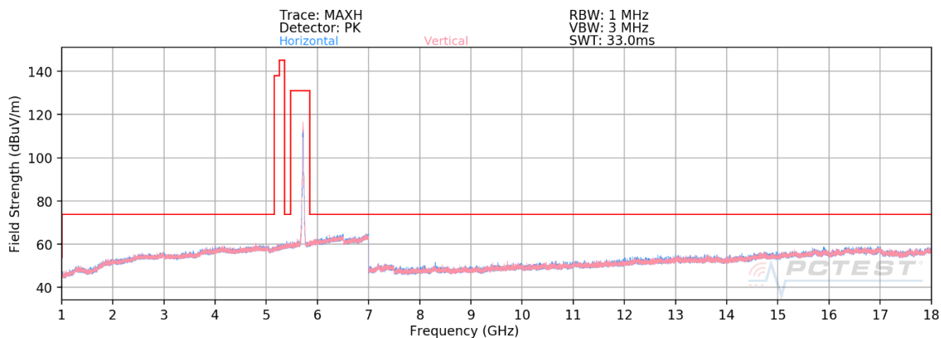
Plot 7-671. RSE above 1GHz CDD Primary (11ax – Ch.144 – RU242)
