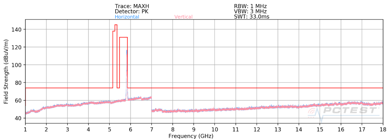
Plot 7-716. RSE above 1GHz CDD Diversity (11ax – Ch.165 – RU242)
