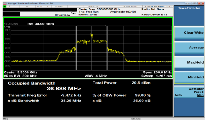
Plot 7-34. 26dB BW & 99% OBW Antenna 5T (80MHz BW 11ax Index 18 - RU26 - Ch.106)
