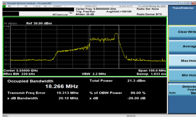
Plot 7-31. 26dB BW & 99% OBW Antenna 5T (40MHz BW 11ax Index 17 - RU26 - Ch.110)
