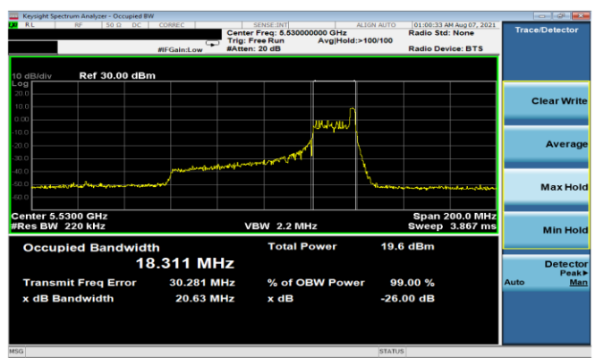
Plot 7-35. 26dB BW & 99% OBW Antenna 5T (80MHz BW 11ax Index 36 - RU26 - Ch.106)
