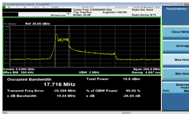
Plot 7-33. 26dB BW & 99% OBW Antenna 5T (80MHz BW 11ax Index 0 - RU26 - Ch.106)
