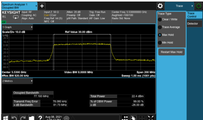
Plot 7-36. 26dB BW & 99% OBW Antenna 5T (80MHz BW 11ax - RU996 - Ch.106)
