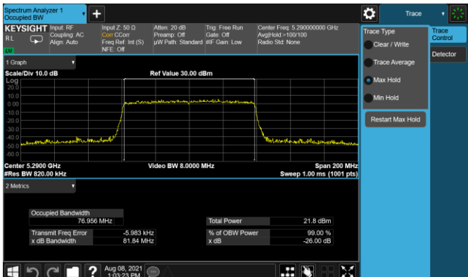
Plot 7-24. 26dB BW & 99% OBW Antenna 5T (80MHz BW 11ax - RU996 - Ch.58)
