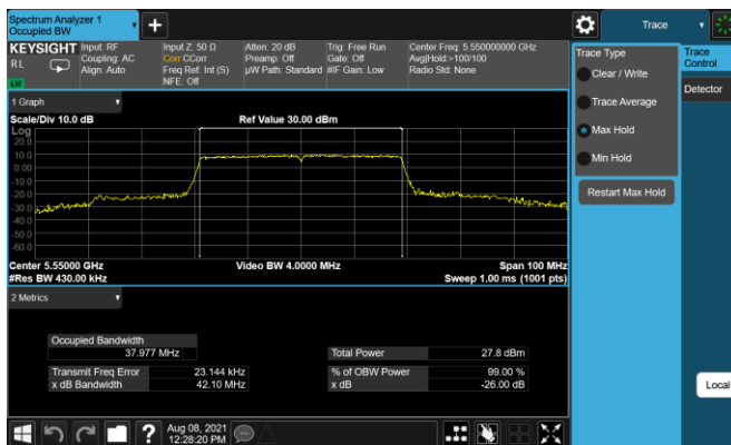
Plot 7-32. 26dB BW & 99% OBW Antenna 5T (40MHz BW 11ax - RU484 - Ch.110)
