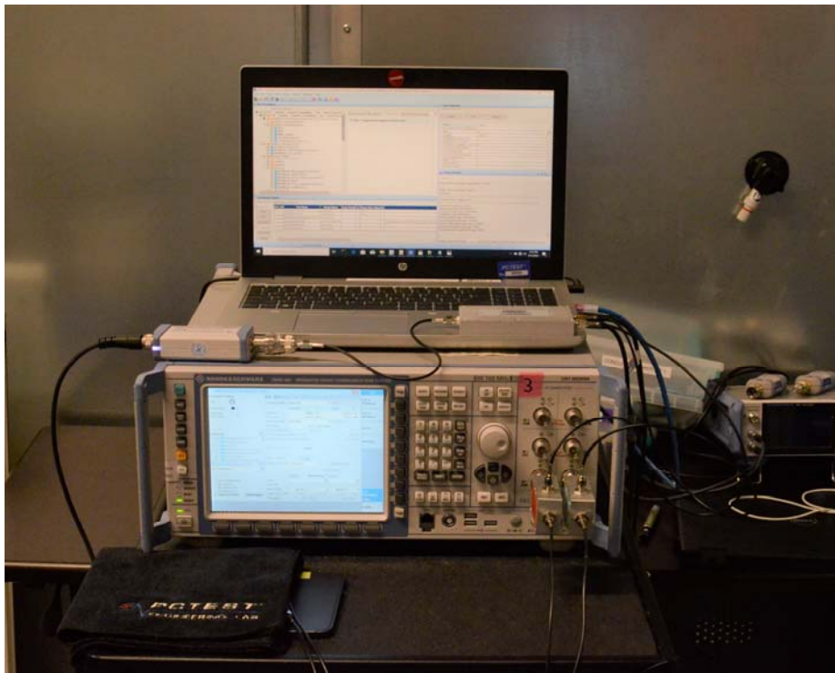
Test Setup Photo 2 – Conducted Test Setup (Figure 5-1b)
