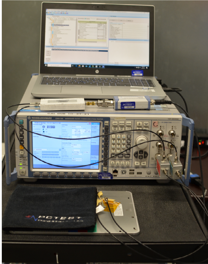
Test Setup Photo 2 – Conducted Test Setup (Figure 5-1b)
