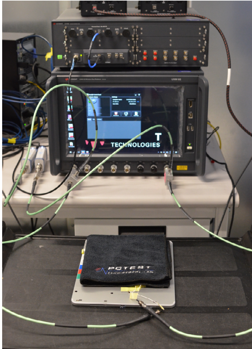
Test Setup Photo 5 – Conducted Test Setup (Figure 5-1e)
