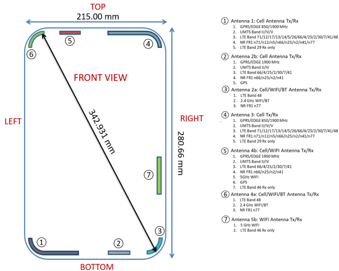
Figure E-1 DUT Antenna Locations
