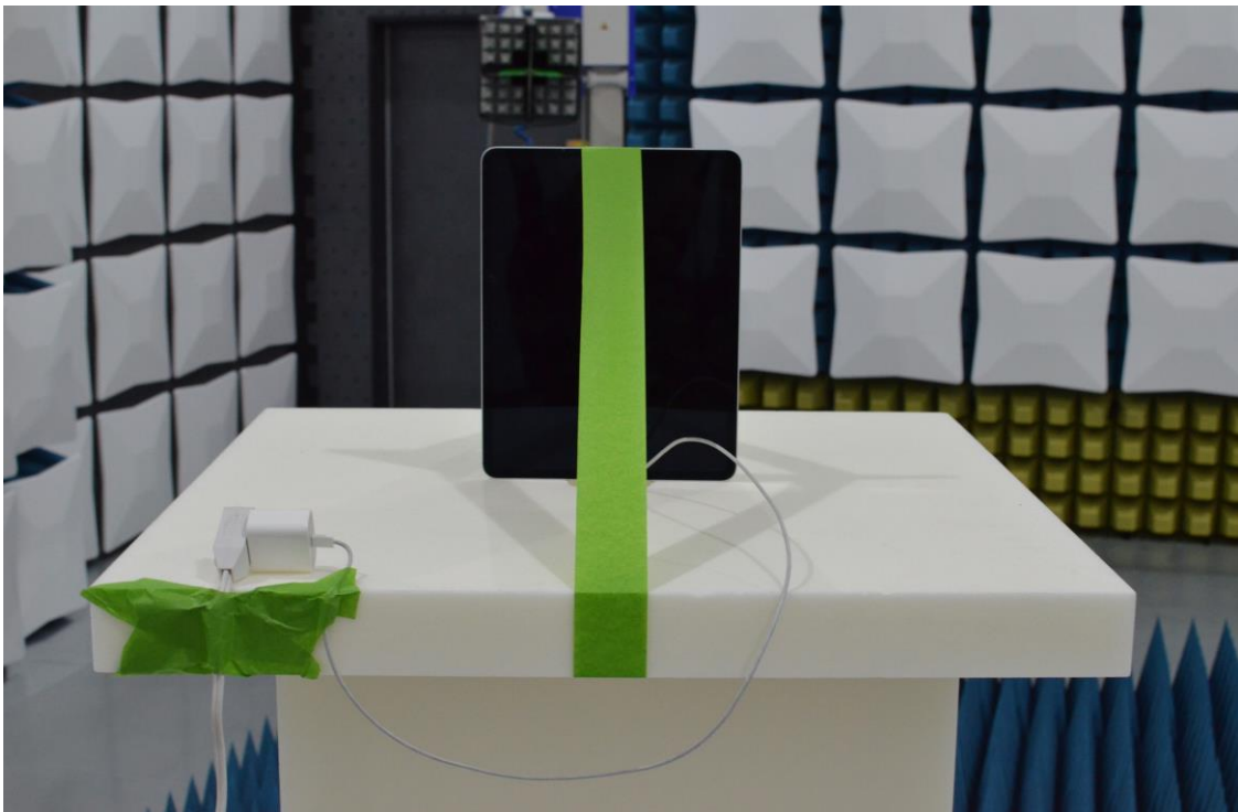
Figure 10: 1-18GHz Test Setup (Rear View)
