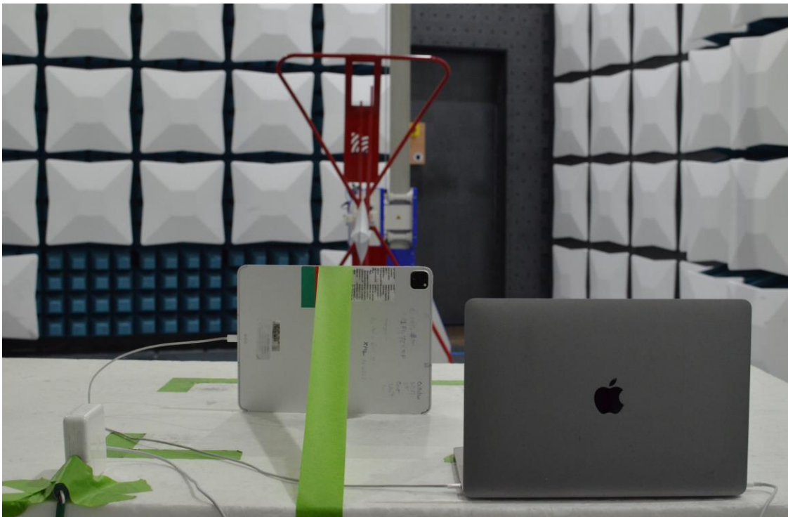
Figure 20: 30MHz-1GHz Test Setup (Rear View)
