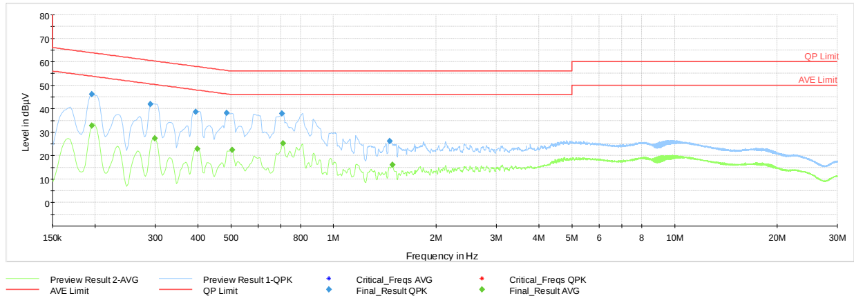
Plot 6-5. AC Line Conducted Plot (L1, Charging Rate 10C, with AC/DC Adapter)
