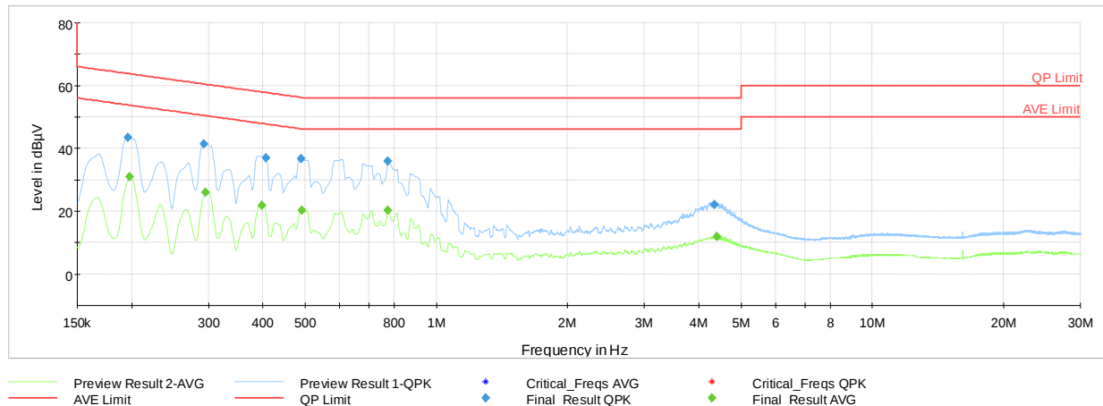
Plot 6-6. AC Line Conducted Plot (N, Charging Rate 10C, with AC/DC Adapter)
