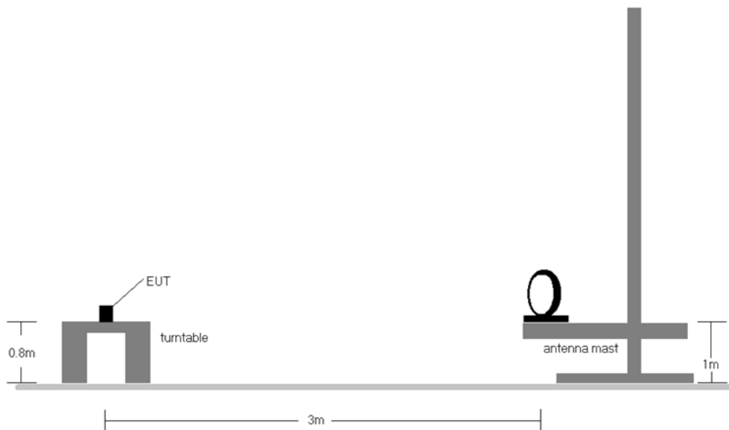
Figure 6-1. Test Setup
