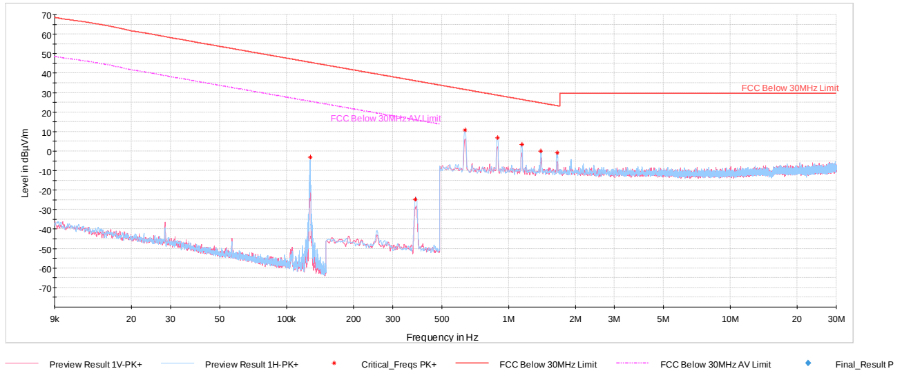
Plot 6-3. Radiated Spurious Emissions 9kHz-30MHz (Charging Rate 10C, with AC/DC Adapter)
