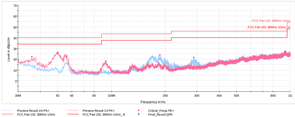
Plot 6-4. Radiated Spurious Emissions 30MHz-1GHz (Charging Rate 10C, with AC/DC Adapter)
