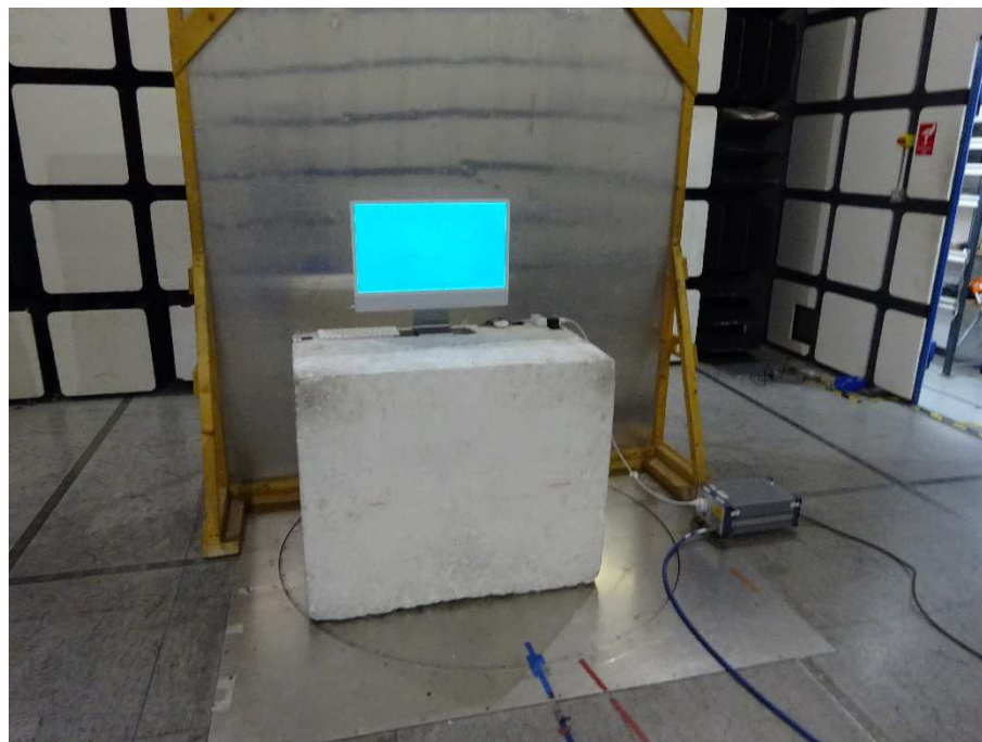
Figure 4 - Conducted Disturbance at Mains Terminals
