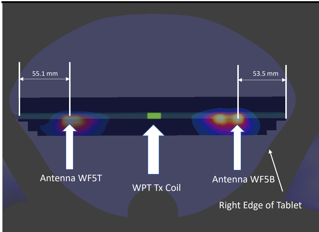
Figure 2 Right Edge Overlay Showing Localization of Simultaneous Peaks
