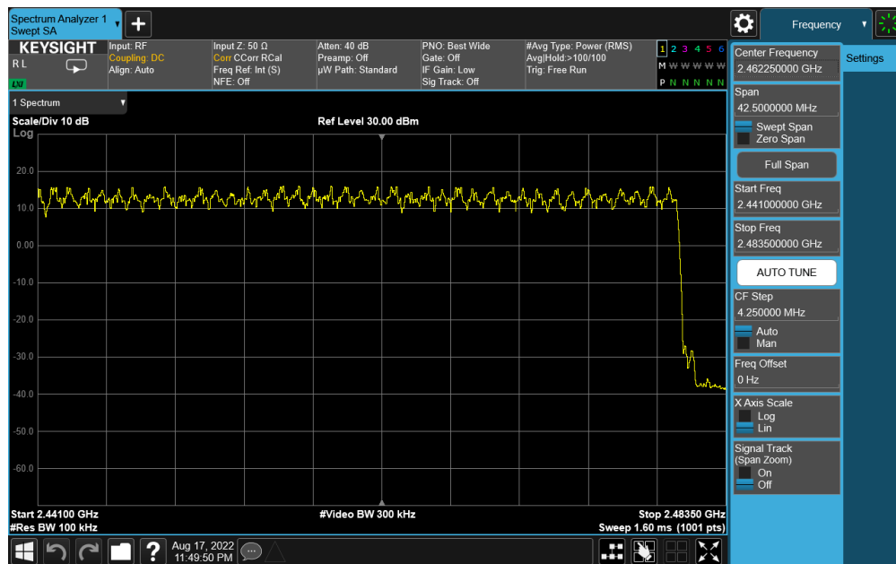
Plot 7-44. High End Spectrum Channel Hopping Plot Antenna 2a (Bluetooth, 8DPSK, ePA, 2.4GHz)
