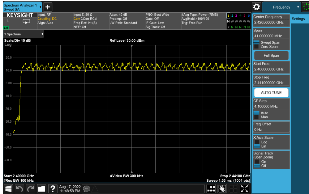
Plot 7-43. Low End Spectrum Channel Hopping Plot Antenna 2a (Bluetooth, 8DPSK, ePA, 2.4GHz)
