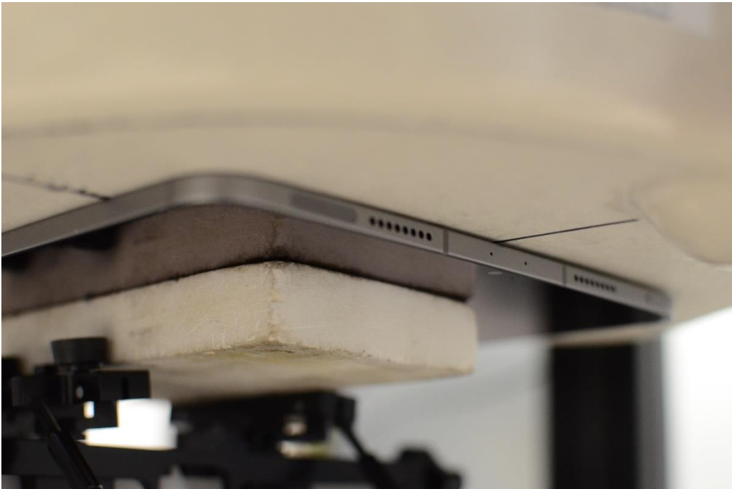
SAR Test Setup Photo 1: Back Side at 0.0 cm – Antenna 3/4a/4b
