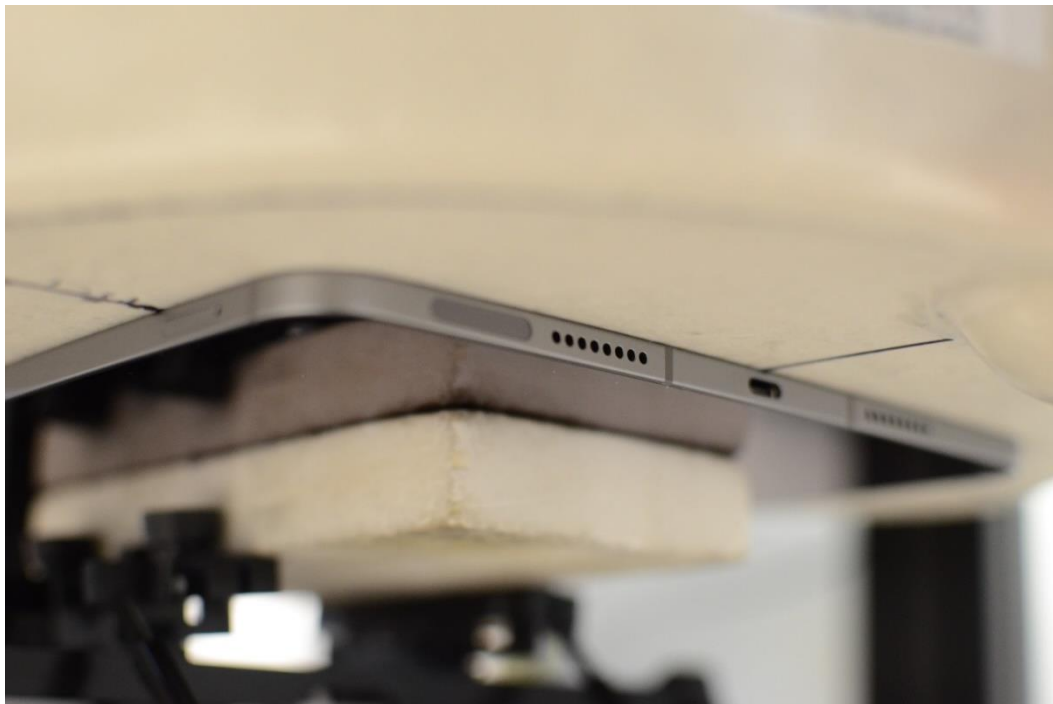
SAR Test Setup Photo 2: Back Side at 0.0 cm – Antenna 1/2a/2b/5b
