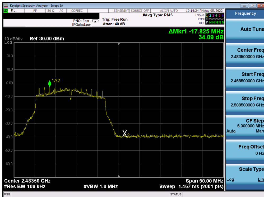
Plot 7-352. Band Edge Plot Antenna 2a (802.11g – Ch. 13) – 18Mbps
