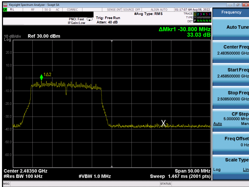
Plot 7-413. Band Edge Plot Antenna 2a (802.11n (2.4GHz) - Ch. 13) - MCS5
