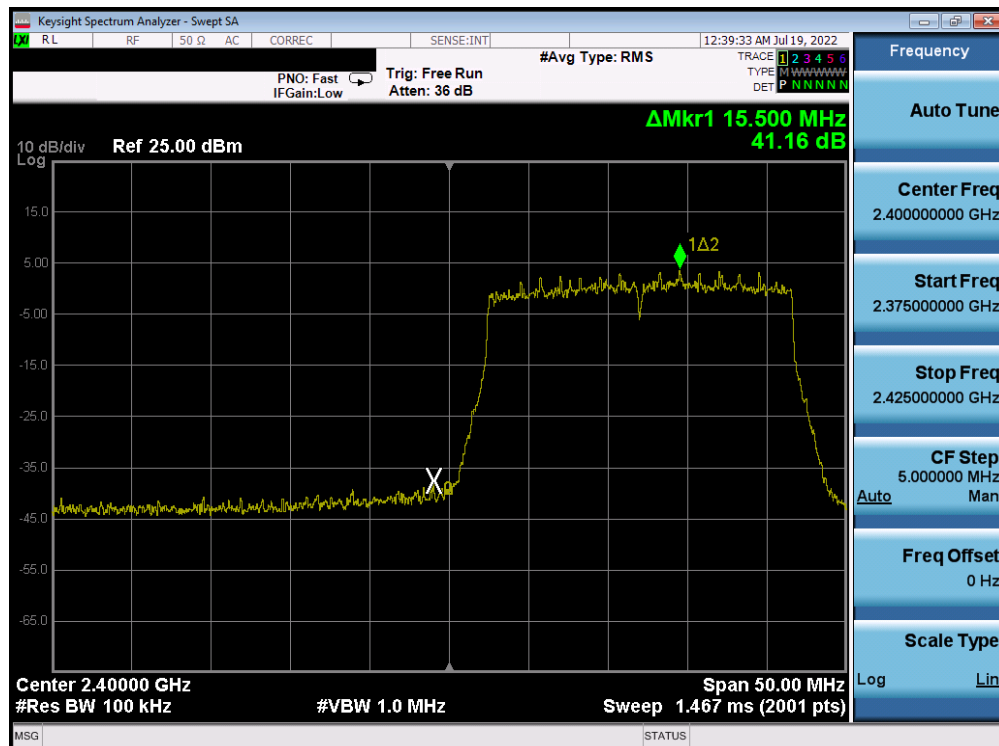
Plot 7-414. Band Edge Plot Antenna 2a (802.11ax (SU - 2.4GHz) – Ch. 1) – MCS5
