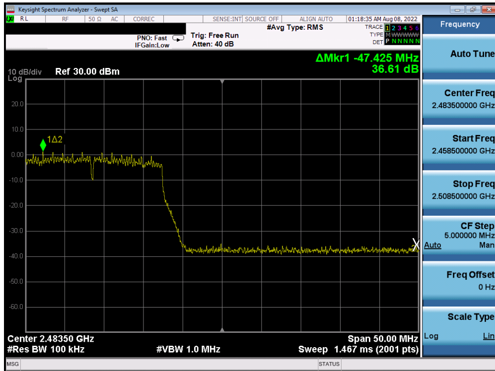
Plot 7-412. Band Edge Plot Antenna 2a (802.11n (2.4GHz) - Ch. 12) - MCS5
