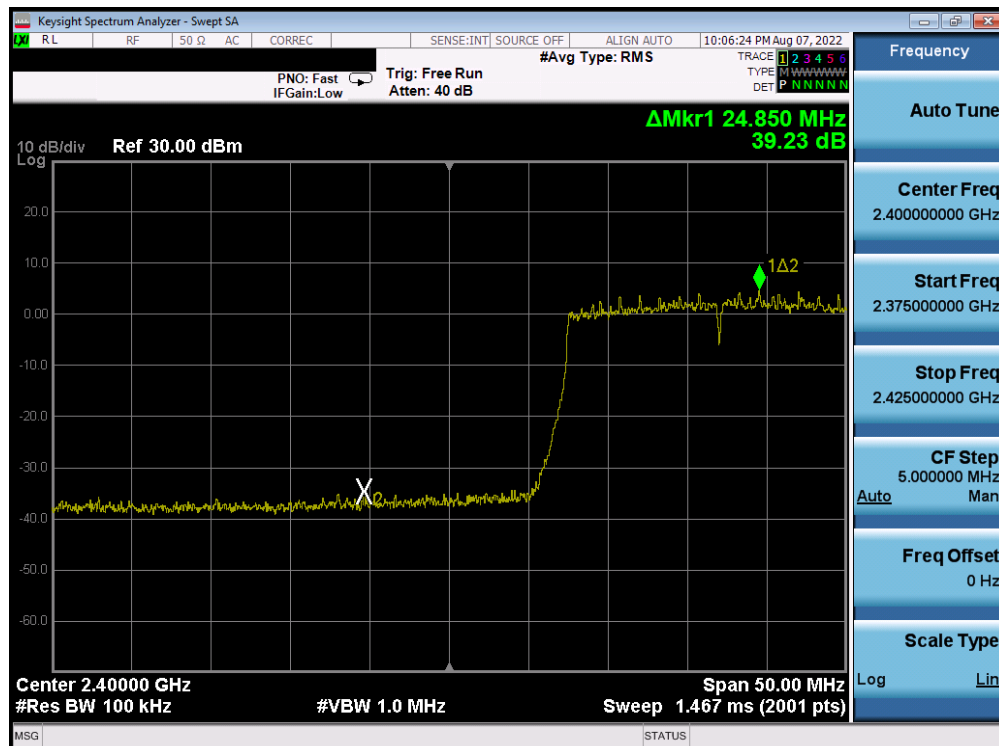
Plot 7-415. Band Edge Plot Antenna 2a (802.11ax (SU - 2.4GHz) – Ch. 2) – MCS5
