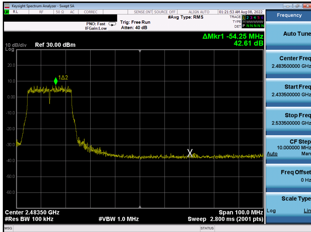
Plot 7-408. Band Edge Plot Antenna 2a (802.11n (2.4GHz) - Ch. 8) - MCS5
