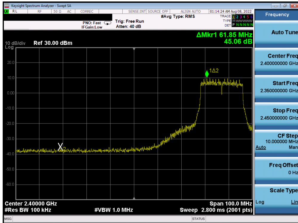
Plot 7-405. Band Edge Plot Antenna 2a (802.11n (2.4GHz) – Ch. 6 (low)) – MCS5
