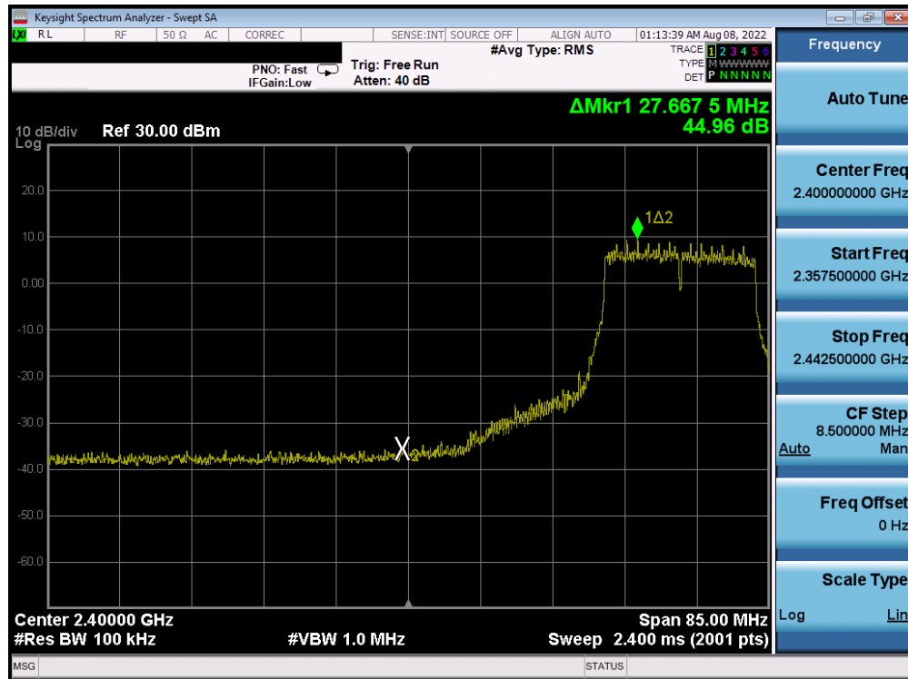
Plot 7-404. Band Edge Plot Antenna 2a (802.11n (2.4GHz) – Ch. 5) – MCS5
