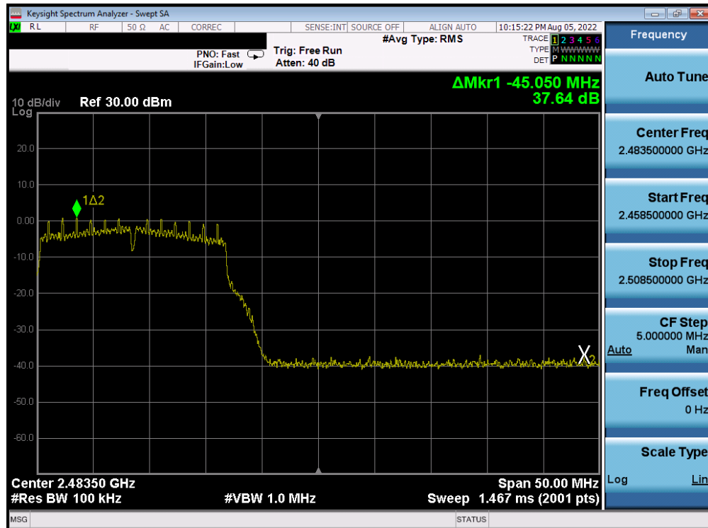
Plot 7-351. Band Edge Plot Antenna 2a (802.11g – Ch. 12) – 18Mbps
