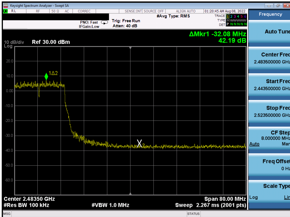
Plot 7-409. Band Edge Plot Antenna 2a (802.11n (2.4GHz) - Ch. 9) - MCS5
