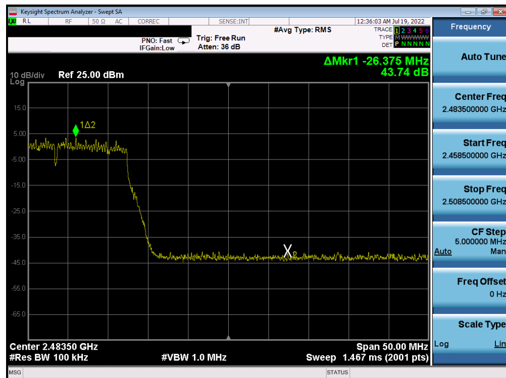
Plot 7-411. Band Edge Plot Antenna 2a (802.11n (2.4GHz) – Ch. 11) – MCS5
