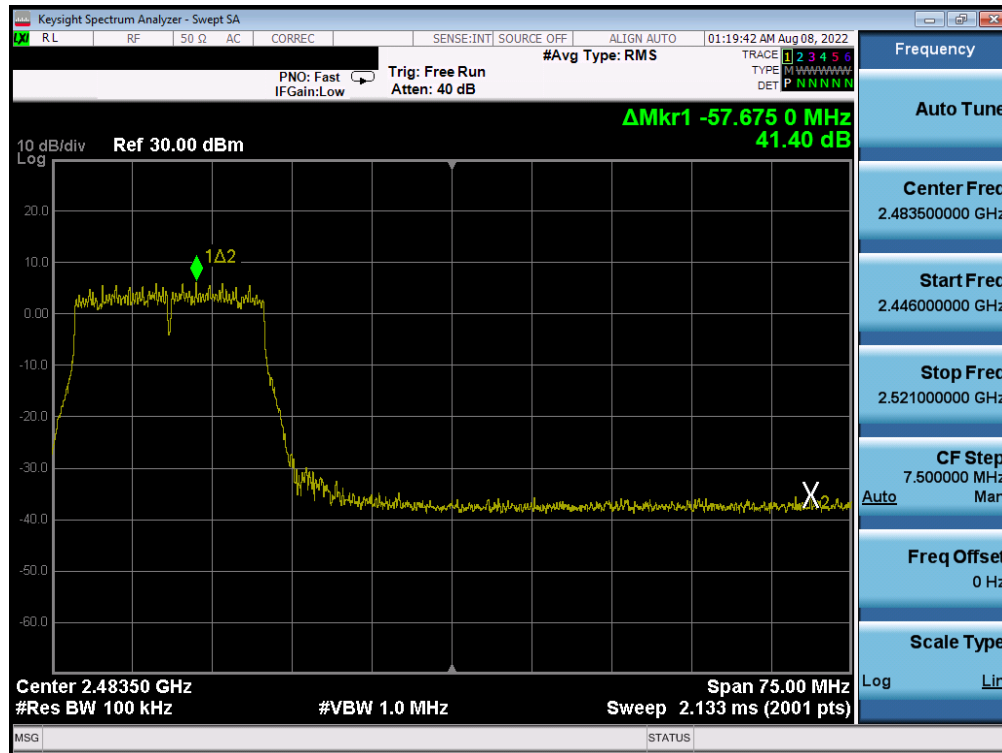
Plot 7-410. Band Edge Plot Antenna 2a (802.11n (2.4GHz) – Ch. 10) – MCS5
