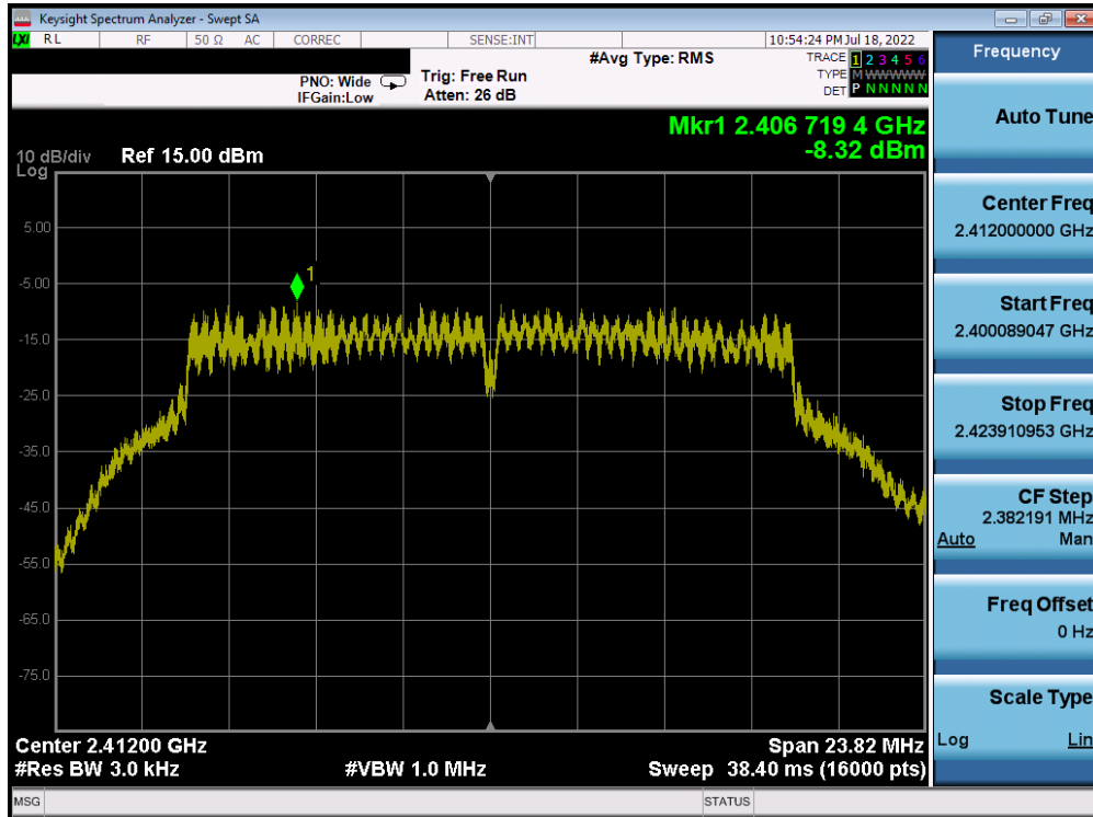
Plot 7-91. Power Spectral Density Plot Antenna 2a (802.11g – Ch. 1) – 12Mbps
