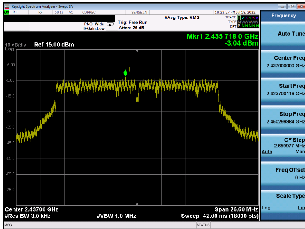
Plot 7-86. Power Spectral Density Plot Antenna 4a (802.11n (2.4GHz) – Ch. 6) – MCS5
