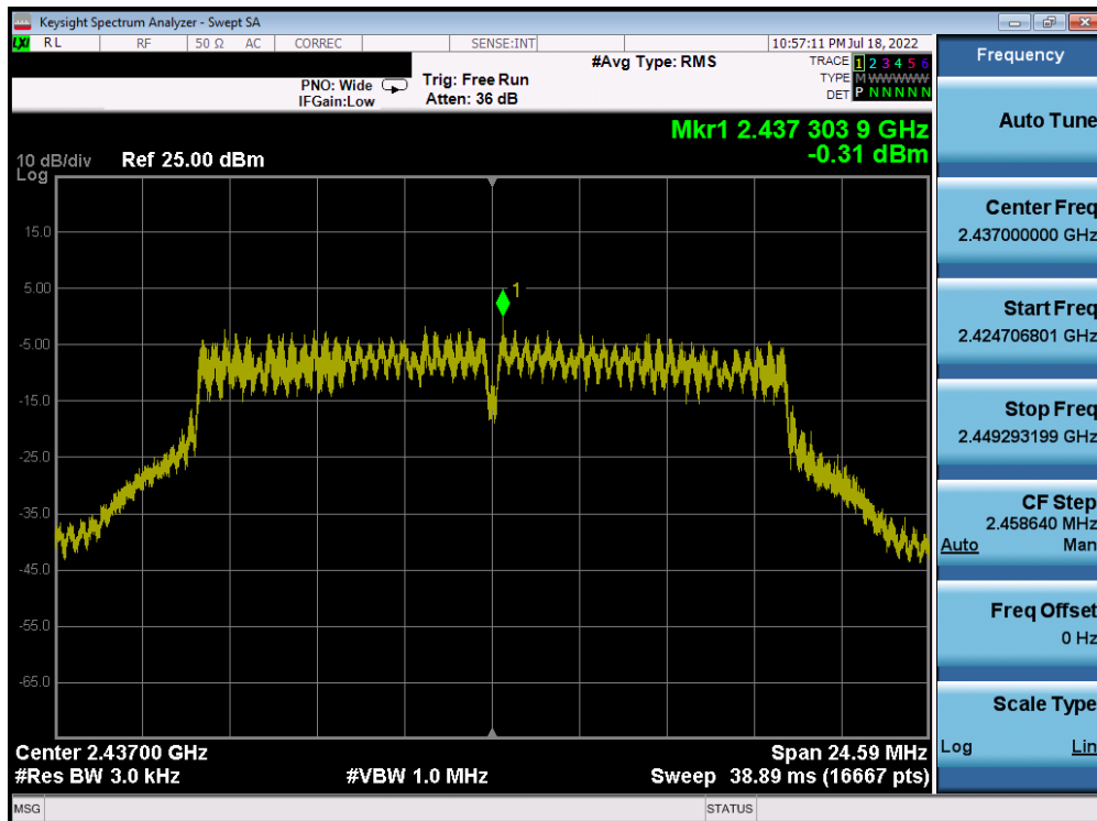
Plot 7-92. Power Spectral Density Plot Antenna 2a (802.11g – Ch. 6) – 12Mbps
