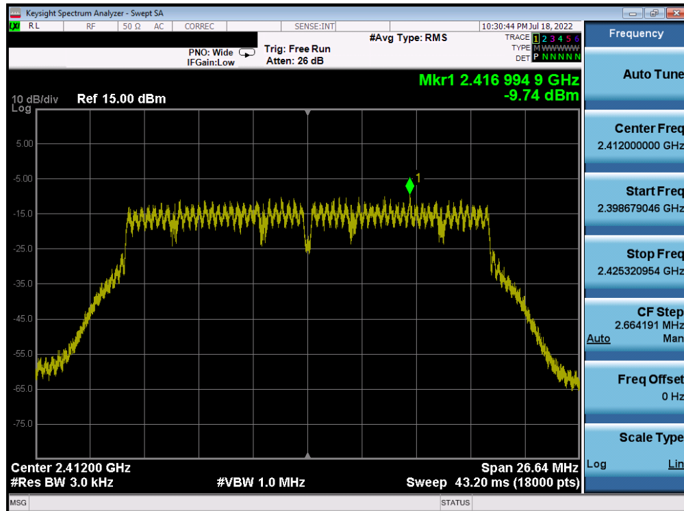
Plot 7-85. Power Spectral Density Plot Antenna 4a (802.11n (2.4GHz) – Ch. 1) – MCS5
