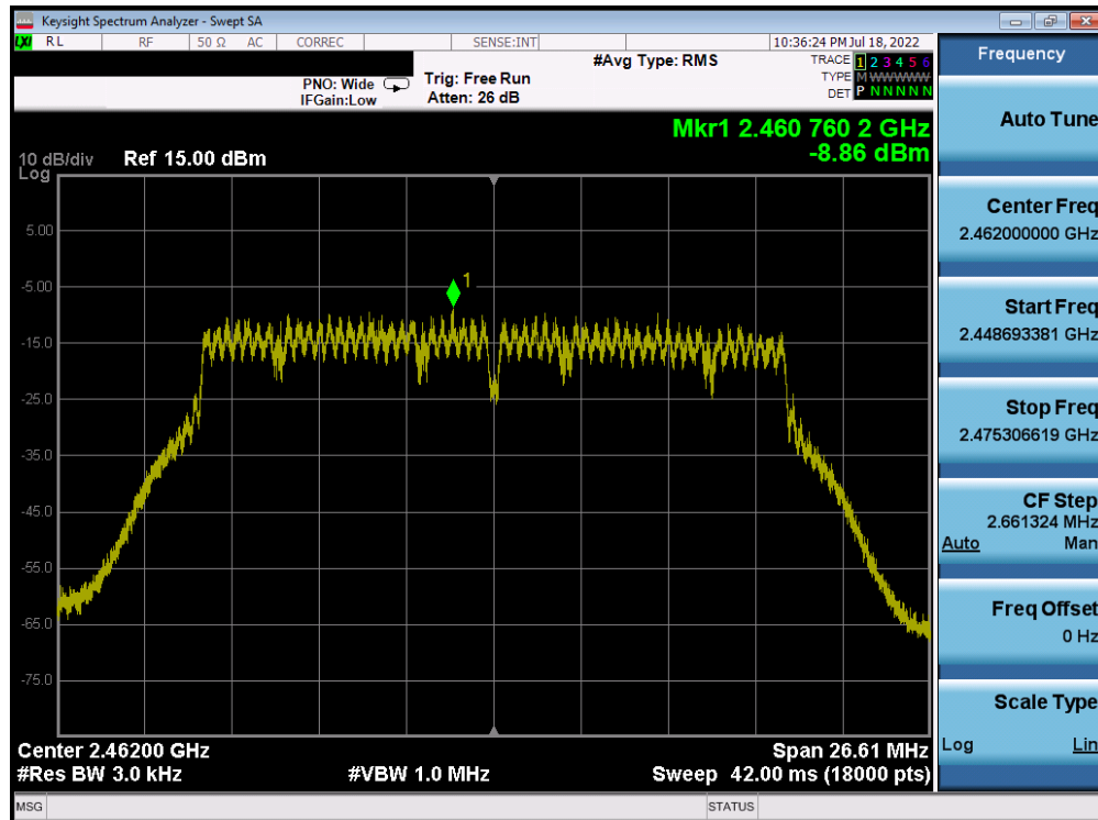
Plot 7-87. Power Spectral Density Plot Antenna 4a (802.11n (2.4GHz) – Ch. 11) – MCS5
