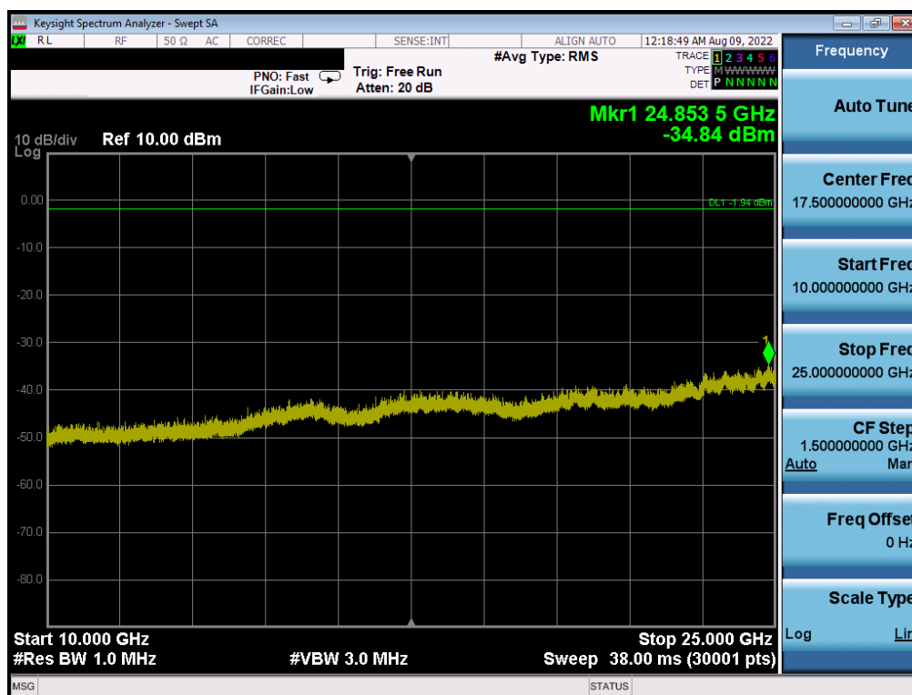
Plot 7-126. Conducted Spurious Plot Antenna 2a (802.11ax OFDMA – RU242 – Ch. 6)
