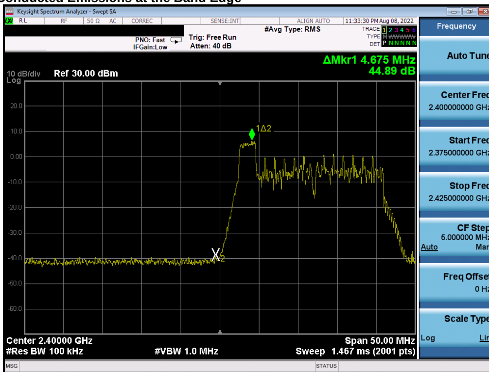
Plot 7-89. Band Edge Antenna 2a (802.11ax OFDMA – RU26 Index 0 – Ch. 1)
