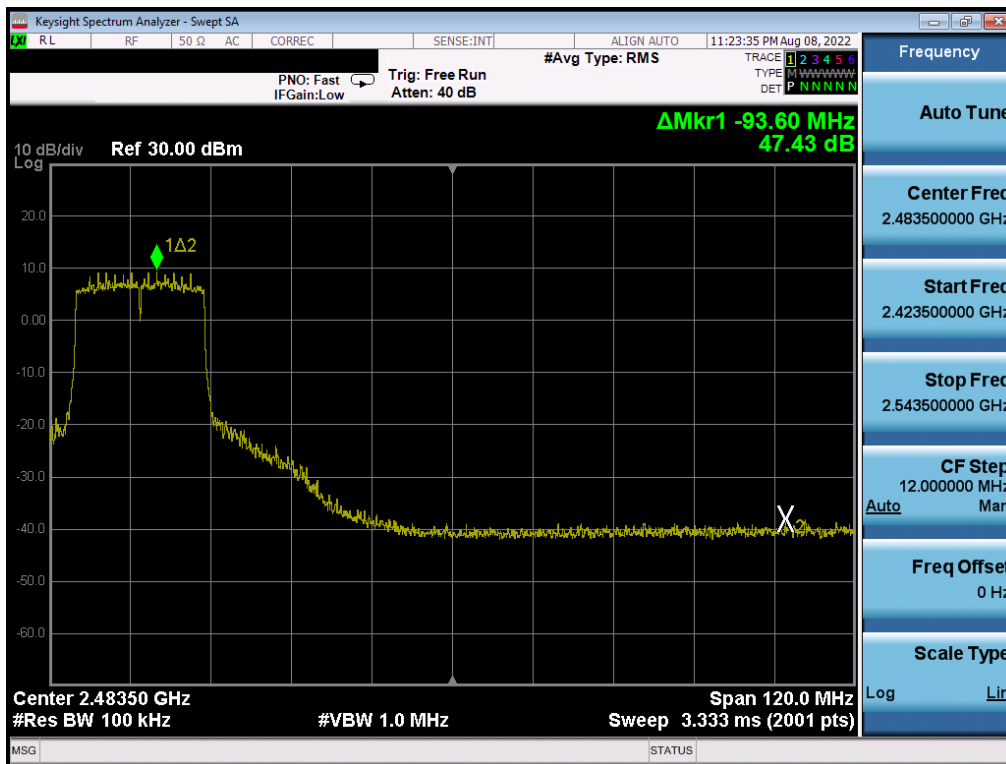
Plot 7-82. Band Edge Antenna 4a (802.11ax OFDMA – RU242 – Ch. 6 (high))
