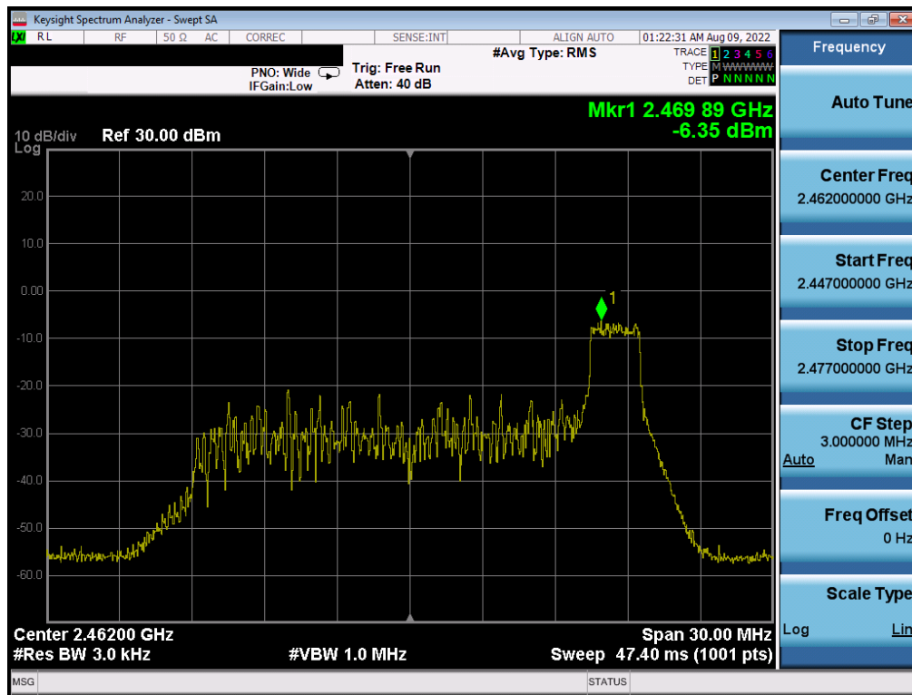
Plot 7-66. Power Spectral Density Plot CDD Antenna 2a (802.11ax OFDMA – RU26 Index 8 – Ch. 11)
