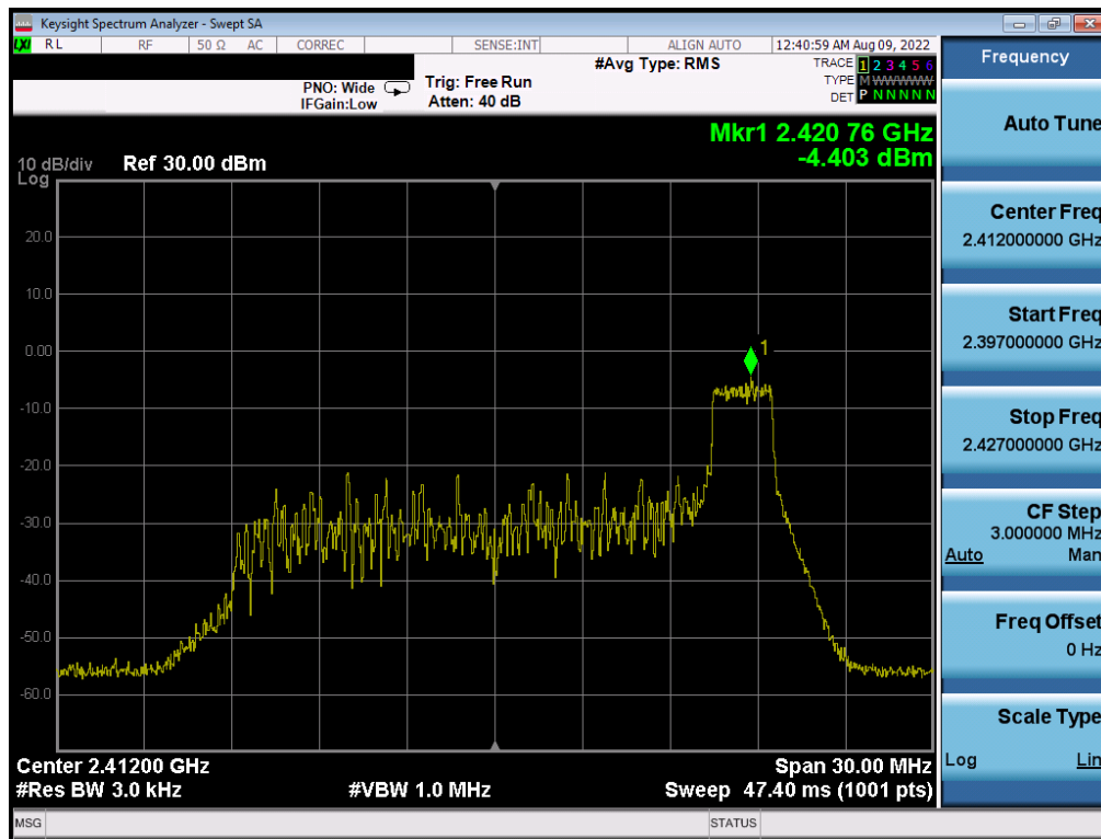
Plot 7-54. Power Spectral Density Plot CDD Antenna 2a (802.11ax OFDMA – RU26 Index 8 – Ch. 1)
