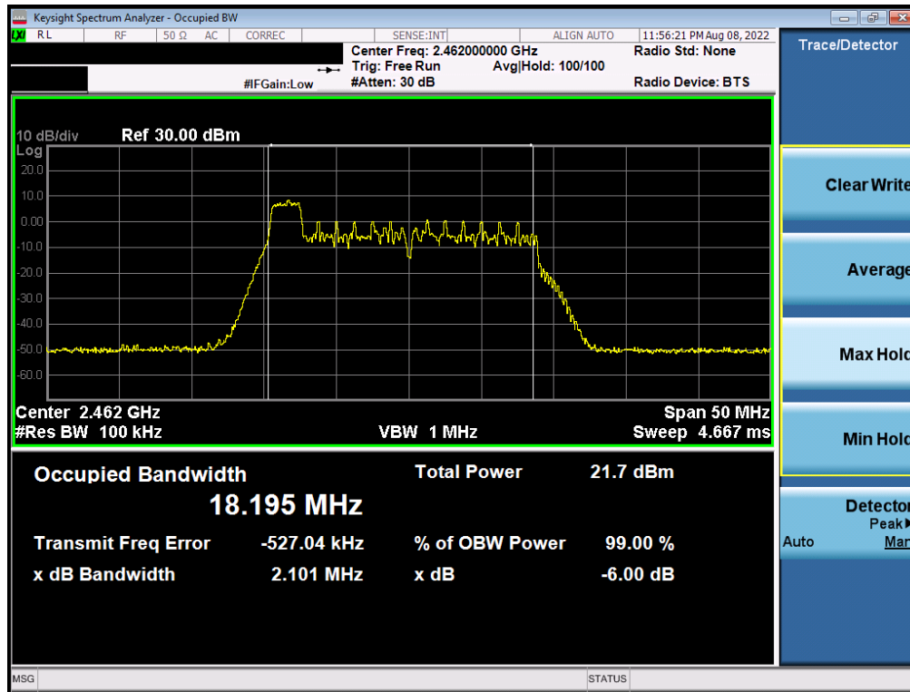
Plot 7-19. 6dB BW & 99% OBW Plot Antenna 2a (802.11ax OFDMA – RU26 Index 0 – Ch. 11)
