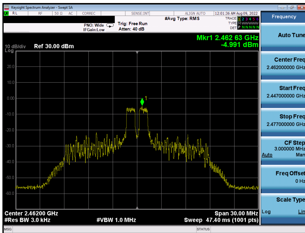
Plot 7-44. Power Spectral Density Plot Antenna 2a (802.11ax OFDMA – RU26 Index 4 – Ch. 11)
