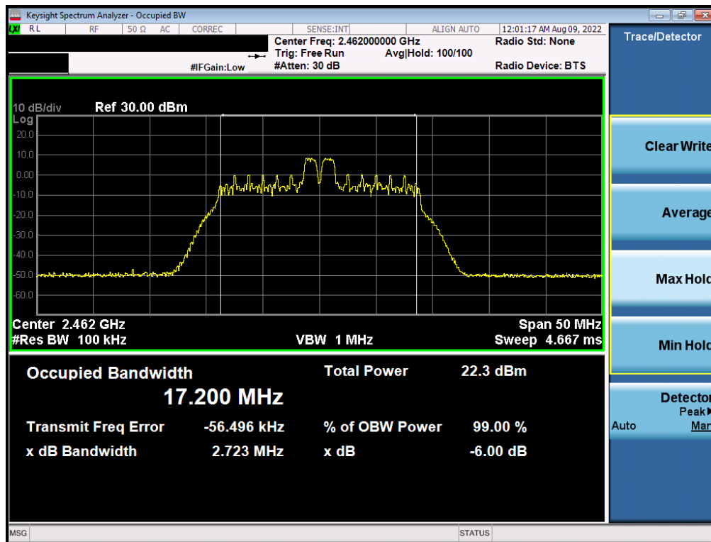
Plot 7-20. 6dB BW & 99% OBW Plot Antenna 2a (802.11ax OFDMA – RU26 Index 4 – Ch. 11)
