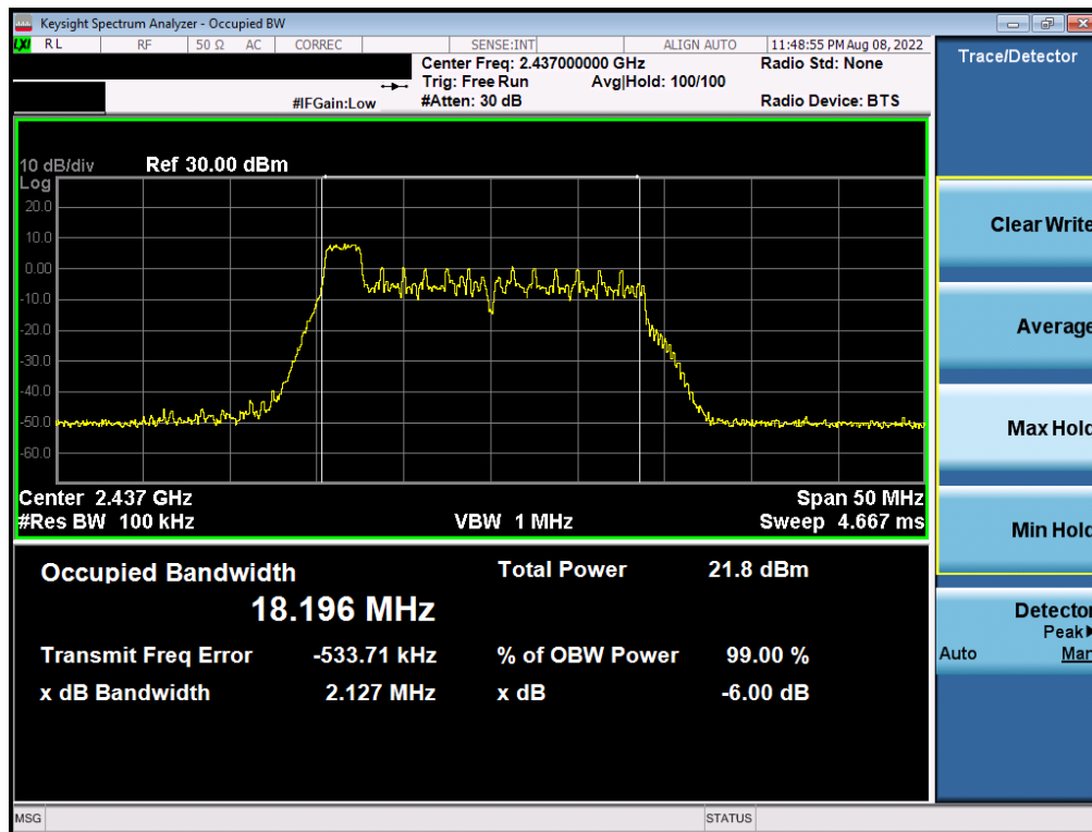
Plot 7-16. 6dB BW & 99% OBW Plot Antenna 2a (802.11ax OFDMA – RU26 Index 0 – Ch. 6)
