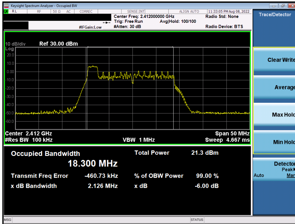
Plot 7-13. 6dB BW & 99% OBW Plot Antenna 2a (802.11ax OFDMA – RU26 Index 0 – Ch. 1)
