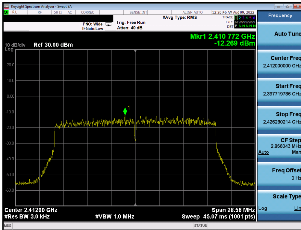
Plot 7-46. Power Spectral Density Plot Antenna 2a (802.11ax OFDMA – RU242 – Ch. 1)
