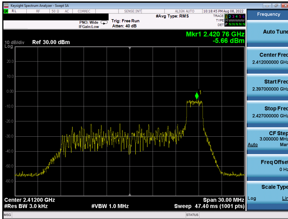
Plot 7-27. Power Spectral Density Plot Antenna 4a (802.11ax OFDMA – RU26 Index 8 – Ch. 1)
