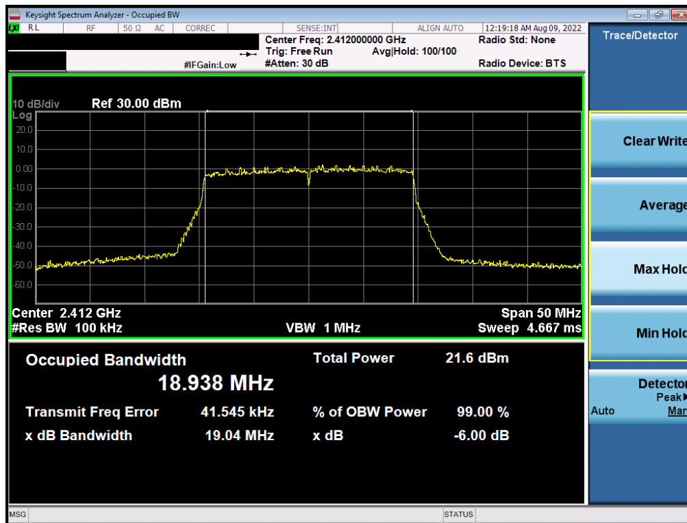
Plot 7-22. 6dB BW & 99% OBW Plot Antenna 2a (802.11ax OFDMA – RU242 – Ch. 1)
