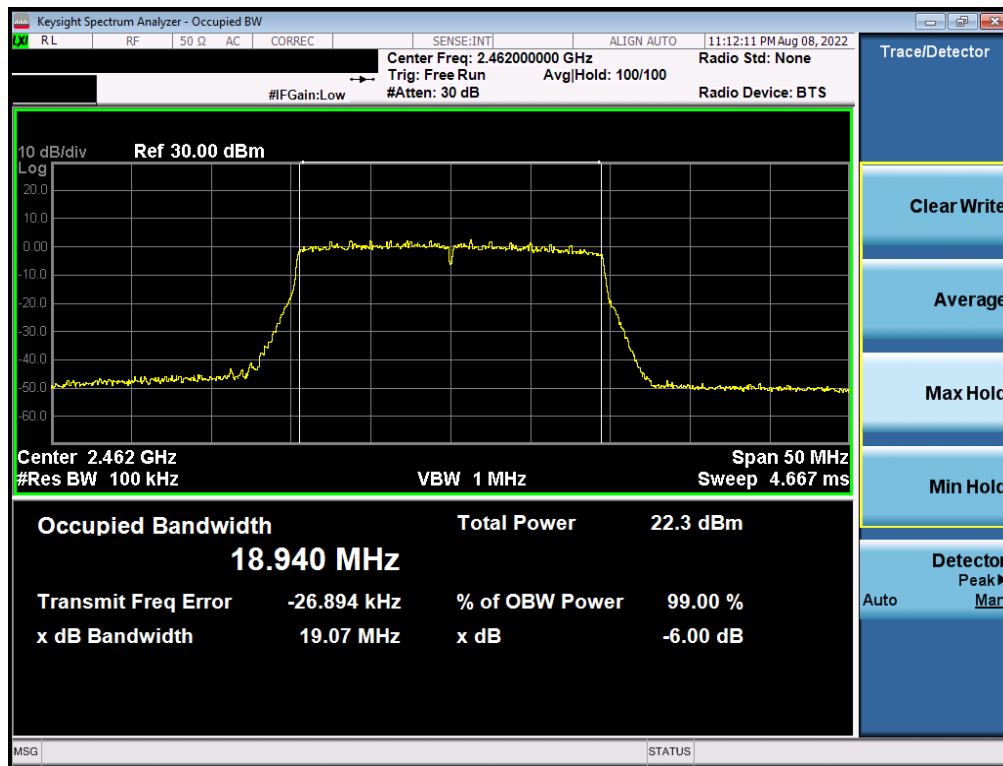
Plot 7-12. 6dB BW & 99% OBW Plot Antenna 4a (802.11ax OFDMA – RU242 – Ch. 11)
