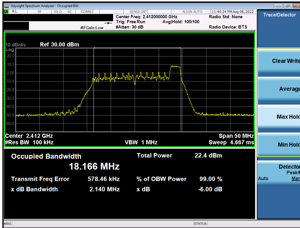
Plot 7-15. 6dB BW & 99% OBW Plot Antenna 2a (802.11ax OFDMA – RU26 Index 8 – Ch. 1)
