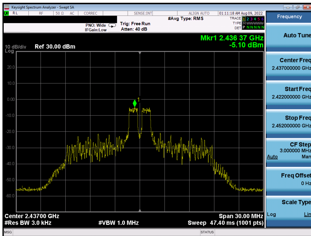
Plot 7-57. Power Spectral Density Plot CDD Antenna 4a (802.11ax OFDMA – RU26 Index 4 – Ch. 6)
