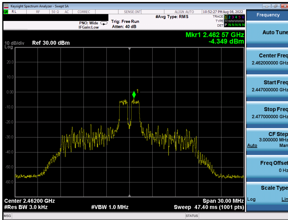
Plot 7-32. Power Spectral Density Plot Antenna 4a (802.11ax OFDMA – RU26 Index 4 – Ch. 11)
