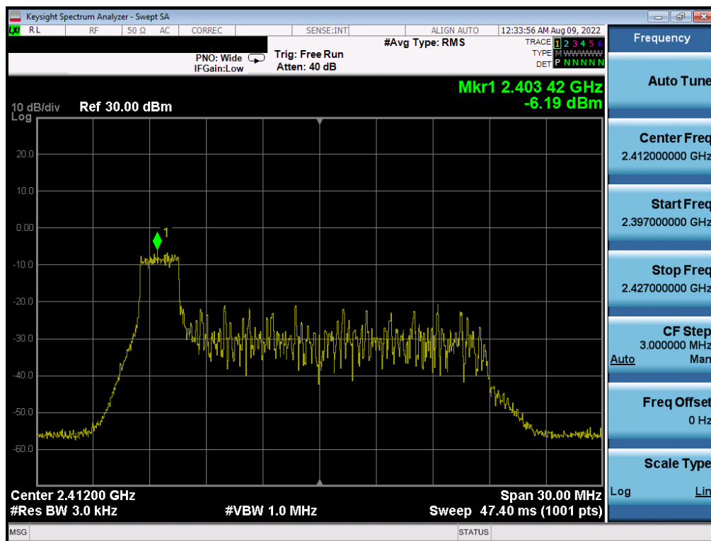
Plot 7-50. Power Spectral Density Plot CDD Antenna 2a (802.11ax OFDMA – RU26 Index 0 – Ch. 1)
