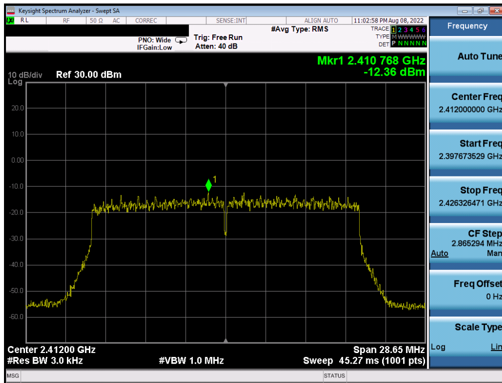
Plot 7-34. Power Spectral Density Plot Antenna 4a (802.11ax OFDMA – RU242 – Ch. 1)
