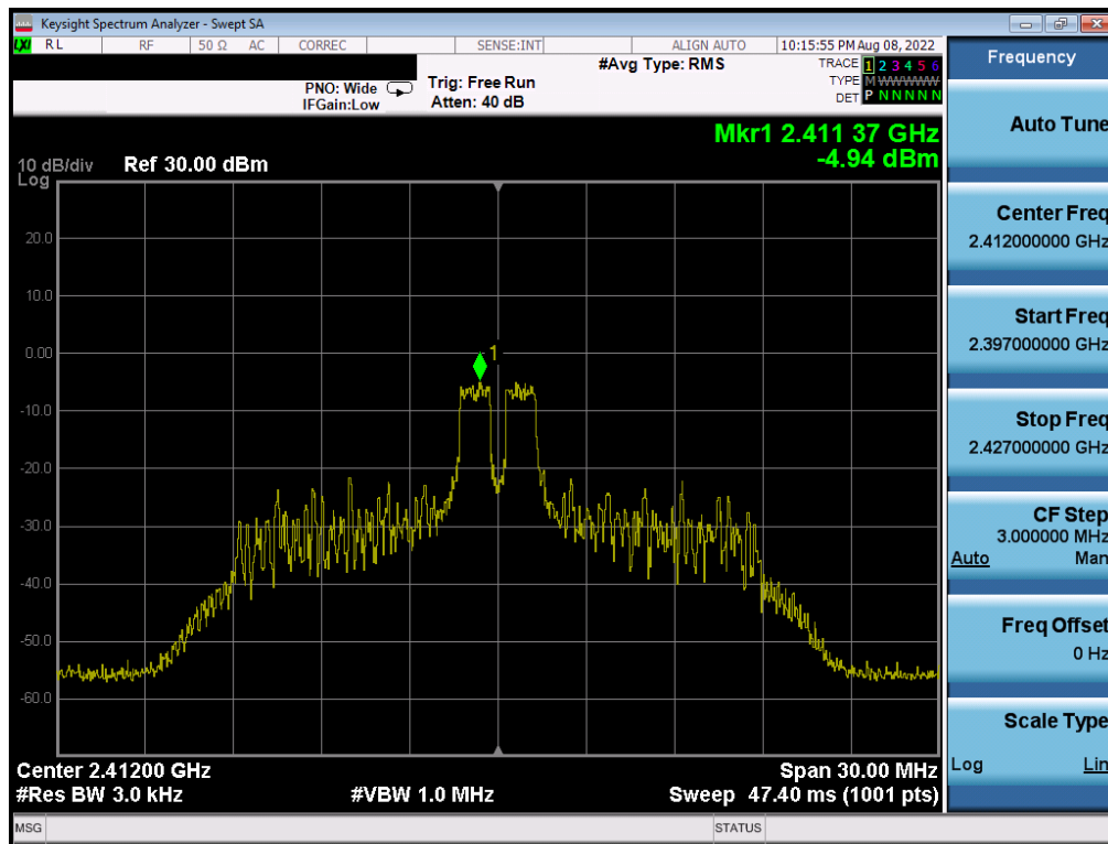
Plot 7-26. Power Spectral Density Plot Antenna 4a (802.11ax OFDMA – RU26 Index 4 – Ch. 1)
