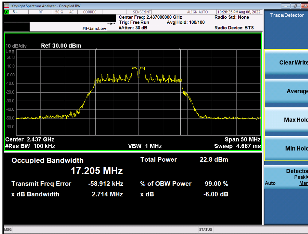
Plot 7-5. 6dB BW & 99% OBW Plot Antenna 4a (802.11ax OFDMA – RU26 Index 4 – Ch. 6)
