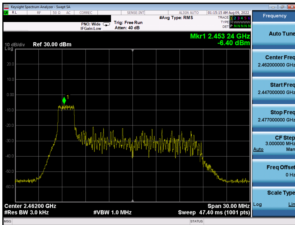
Plot 7-62. Power Spectral Density Plot CDD Antenna 2a (802.11ax OFDMA – RU26 Index 0 – Ch. 11)
