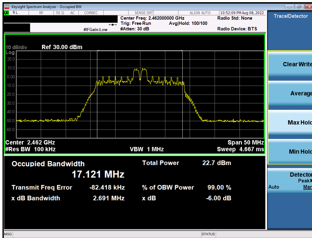
Plot 7-8. 6dB BW & 99% OBW Antenna 4a (802.11ax OFDMA – RU26 Index 4 – Ch. 11)
