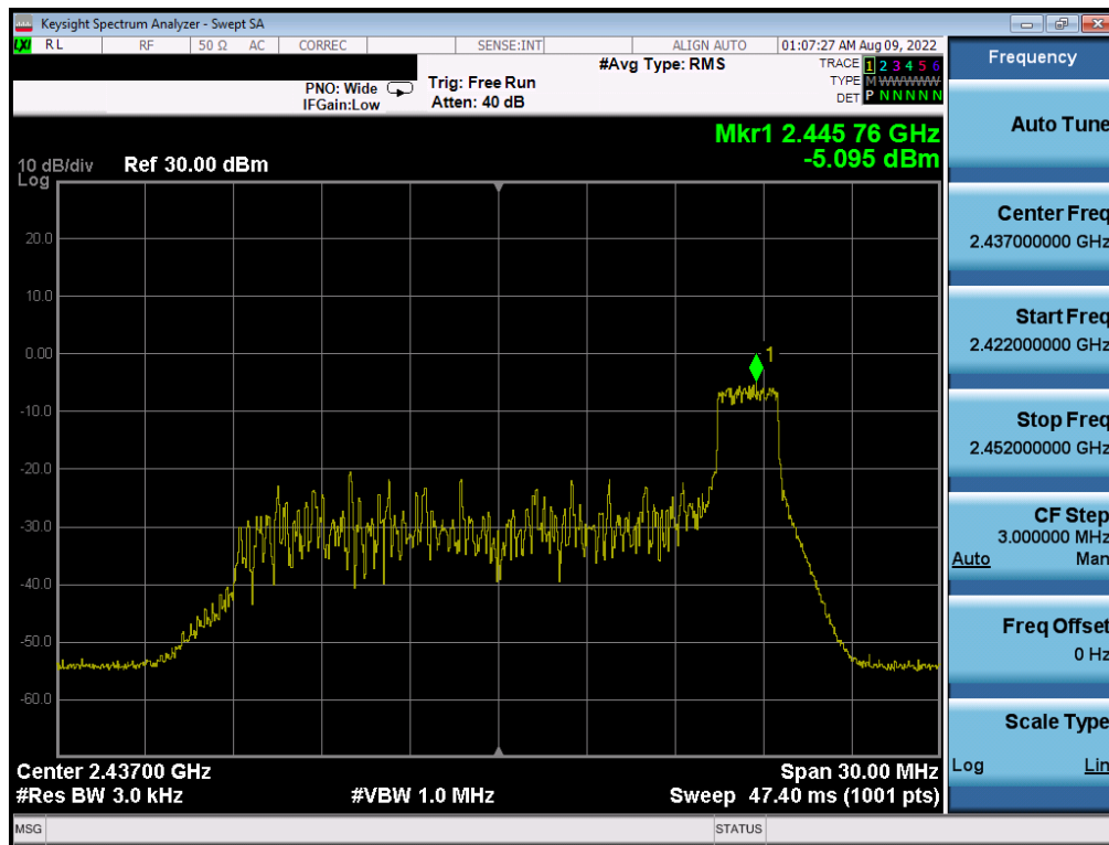
Plot 7-60. Power Spectral Density Plot CDD Antenna 2a (802.11ax OFDMA – RU26 Index 8 – Ch. 6)
