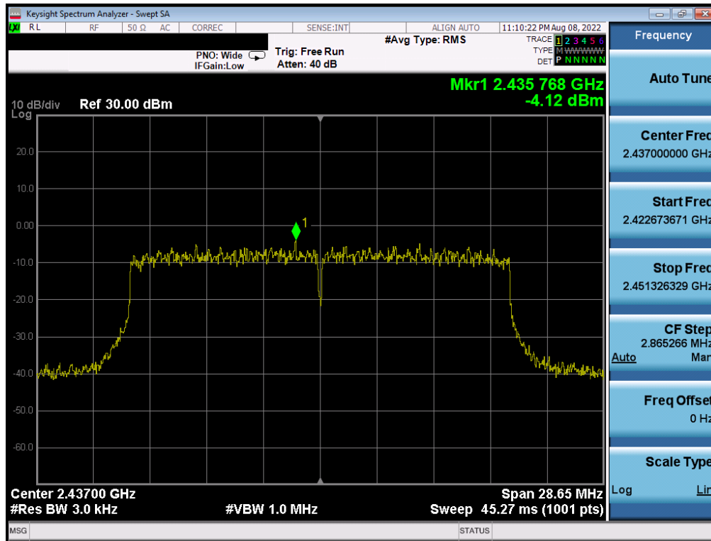
Plot 7-35. Power Spectral Density Plot Antenna 4a (802.11ax OFDMA – RU242 – Ch. 6)
