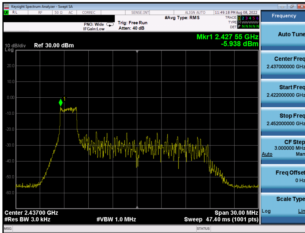
Plot 7-40. Power Spectral Density Plot Antenna 2a (802.11ax OFDMA – RU26 Index 0 – Ch. 6)
