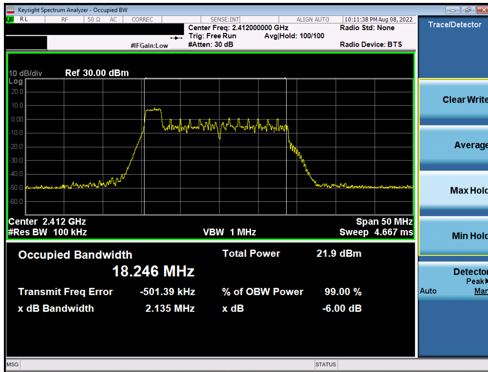
Plot 7-1. 6dB BW & 99% OBW Plot Antenna 4a (802.11ax OFDMA – RU26 Index 0 – Ch. 1)
