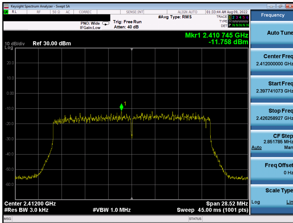
Plot 7-68. Power Spectral Density Plot CDD Antenna 2a (802.11ax OFDMA – RU242 – Ch. 1)
