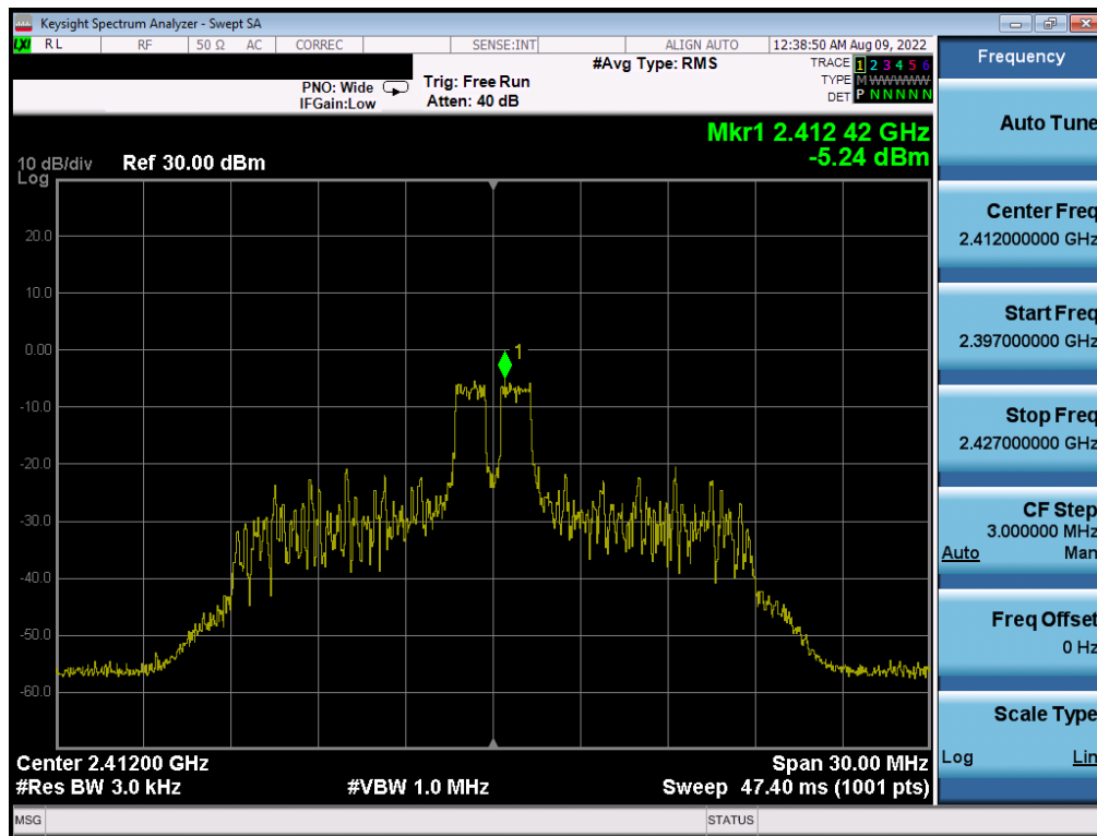
Plot 7-52. Power Spectral Density Plot CDD Antenna 2a (802.11ax OFDMA – RU26 Index 4 – Ch. 1)
