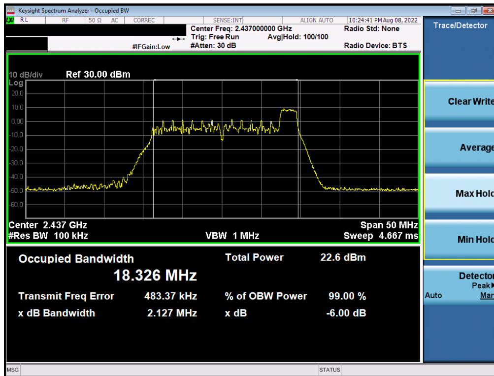
Plot 7-6. 6dB BW & 99% OBW Antenna 4a (802.11ax OFDMA – RU26 Index 8 – Ch. 6)
