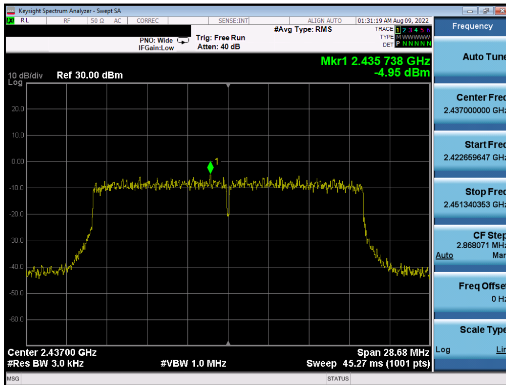
Plot 7-69. Power Spectral Density Plot CDD Antenna 4a (802.11ax OFDMA – RU242 – Ch. 6)
