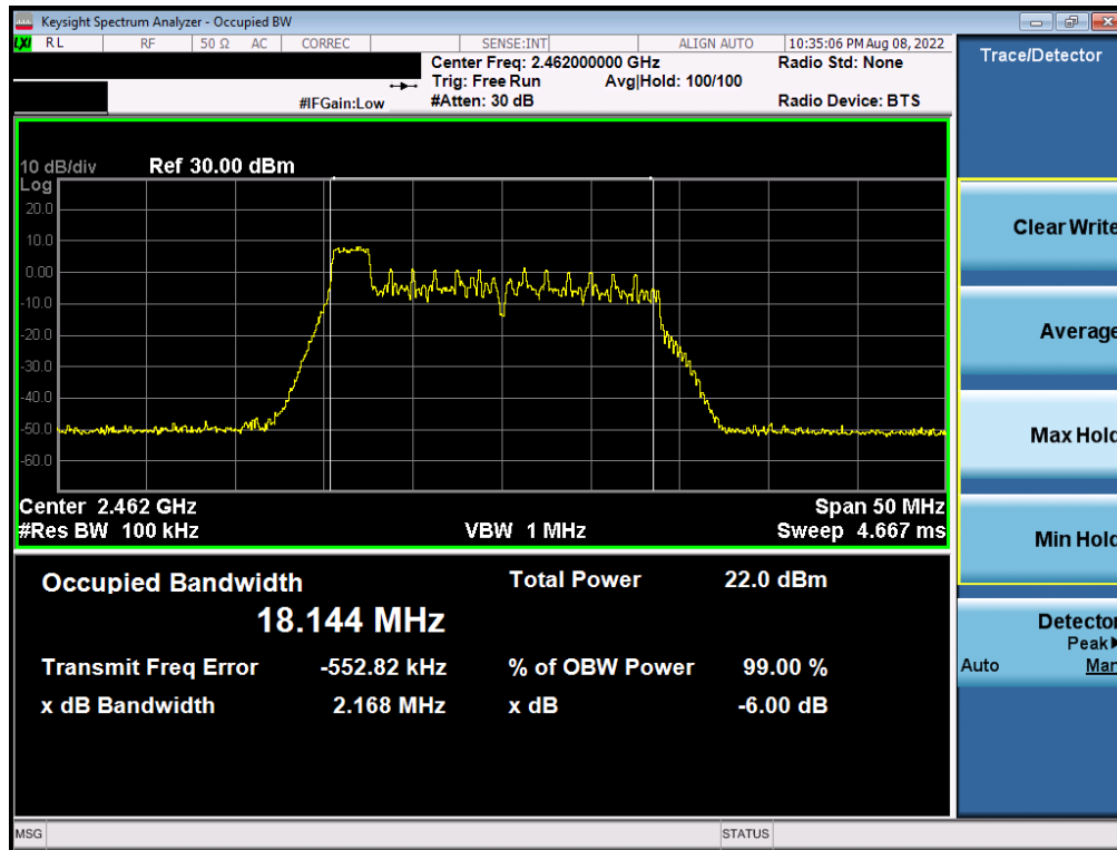
Plot 7-7. 6dB BW & 99% OBW Antenna 4a (802.11ax OFDMA – RU26 Index 0 – Ch. 11)
