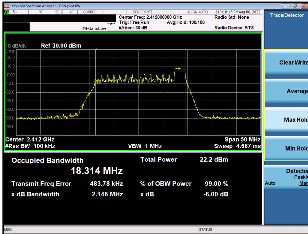
Plot 7-3. 6dB BW & 99% OBW Plot Antenna 4a (802.11ax OFDMA – RU26 Index 8 – Ch. 1)
