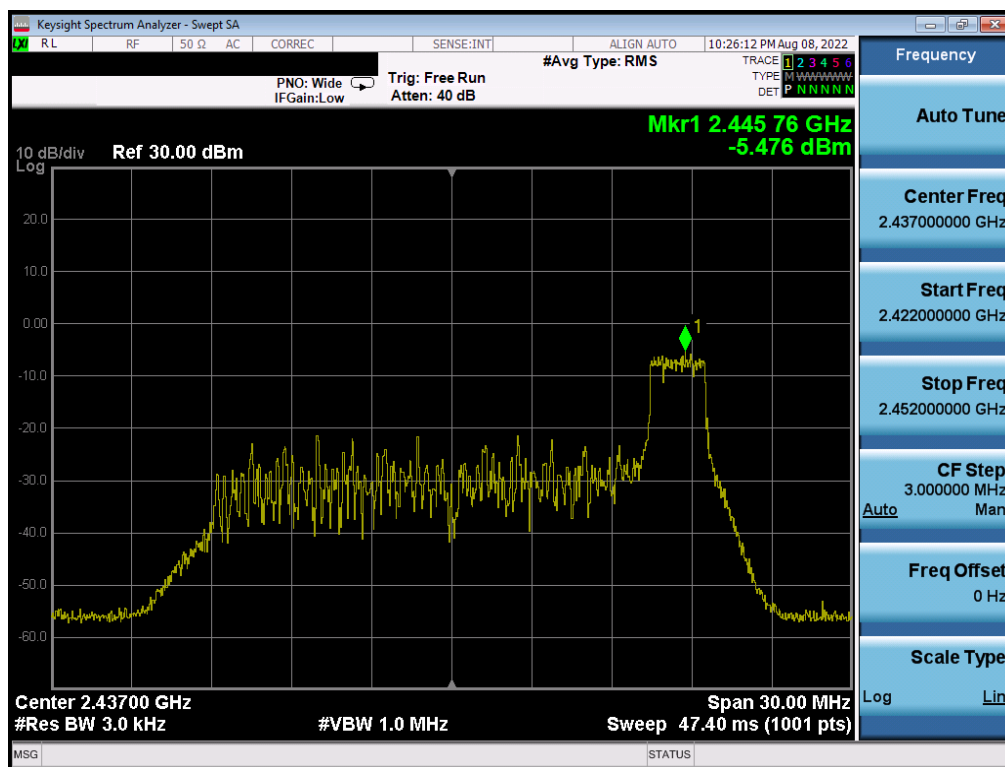
Plot 7-30. Power Spectral Density Plot Antenna 4a (802.11ax OFDMA – RU26 Index 8 – Ch. 6)
