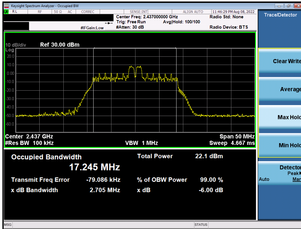
Plot 7-17. 6dB BW & 99% OBW Plot Antenna 2a (802.11ax OFDMA – RU26 Index 4 – Ch. 6)
