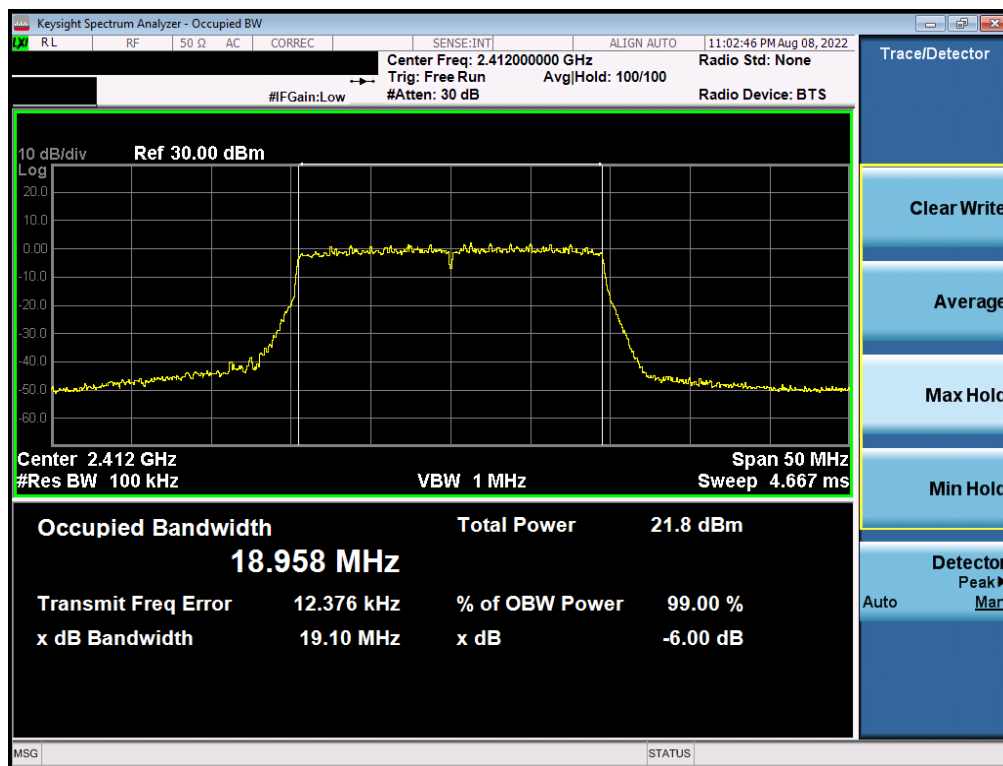
Plot 7-10. 6dB BW & 99% OBW Plot Antenna 4a (802.11ax OFDMA – RU242 – Ch. 1)
