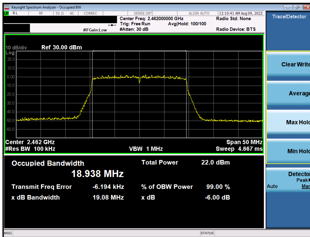
Plot 7-24. 6dB BW & 99% OBW Plot Antenna 2a (802.11ax OFDMA – RU242 – Ch. 11)
