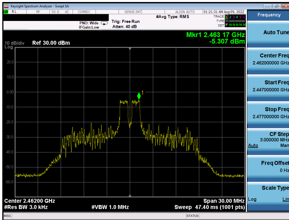
Plot 7-64. Power Spectral Density Plot CDD Antenna 2a (802.11ax OFDMA – RU26 Index 4 – Ch. 11)
