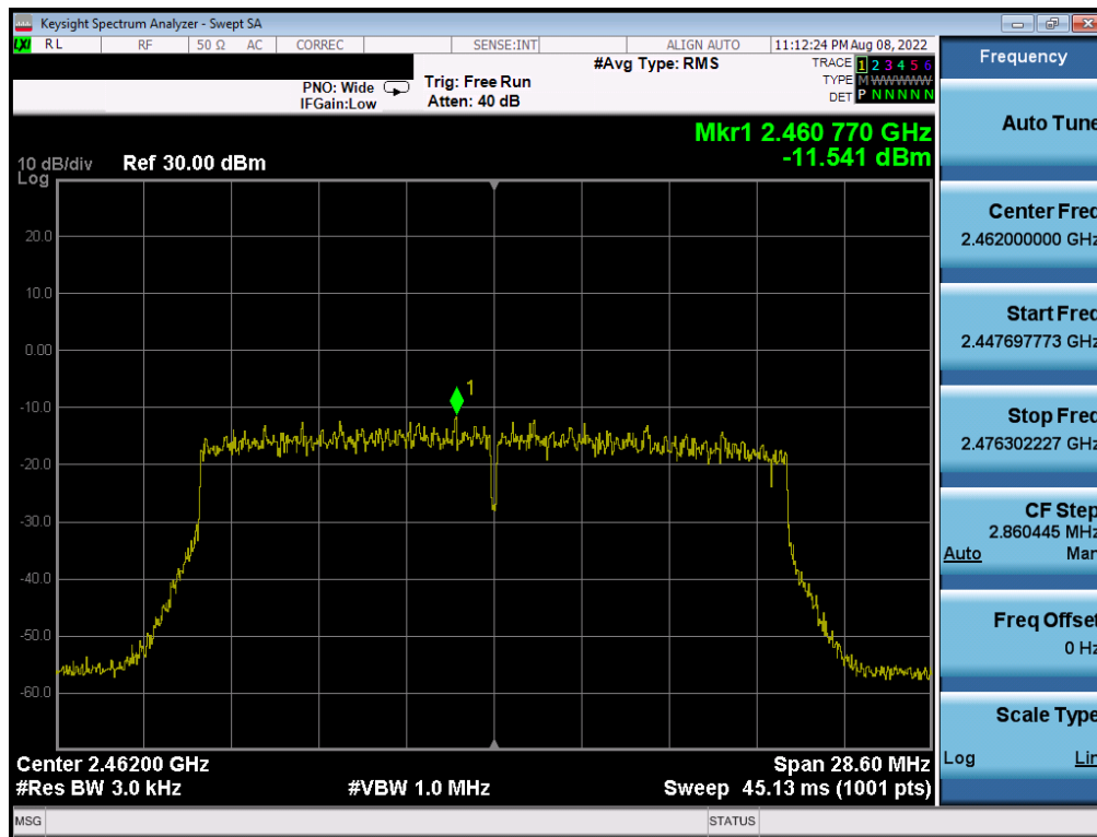
Plot 7-36. Power Spectral Density Plot Antenna 4a (802.11ax OFDMA – RU242 – Ch. 11)
