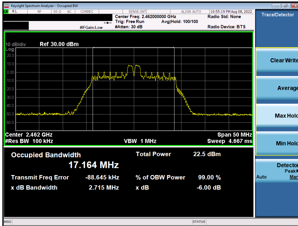
Plot 7-9. 6dB BW & 99% OBW Plot Antenna 4a (802.11ax OFDMA – RU26 Index 8 – Ch. 11)
