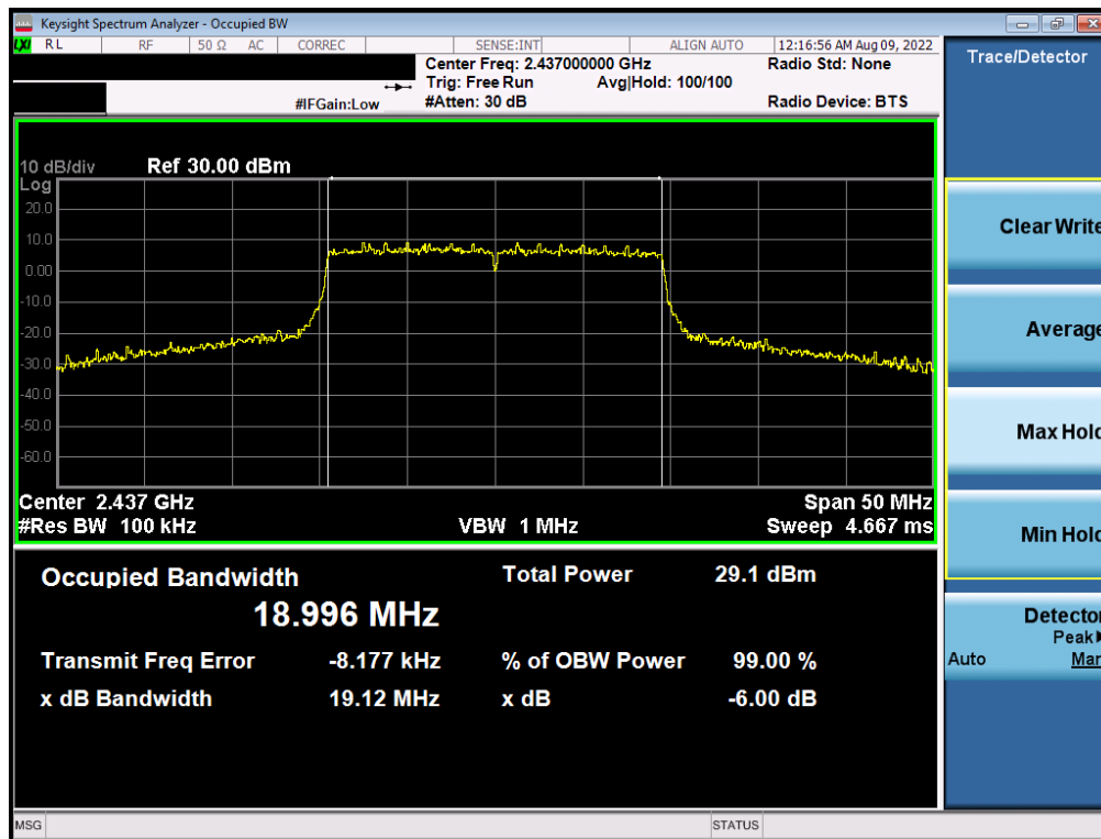
Plot 7-23. 6dB BW & 99% OBW Plot Antenna 2a (802.11ax OFDMA – RU242 – Ch. 6)
