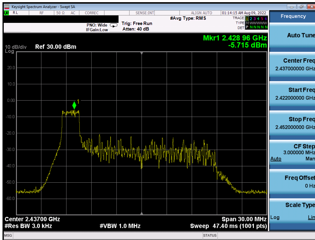
Plot 7-56. Power Spectral Density Plot CDD Antenna 2a (802.11ax OFDMA – RU26 Index 0 – Ch. 6)
