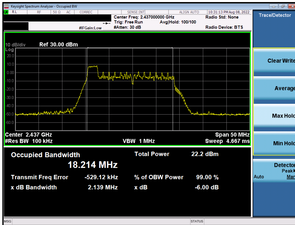
Plot 7-4. 6dB BW & 99% OBW Plot Antenna 4a (802.11ax OFDMA – RU26 Index 0 – Ch. 6)
