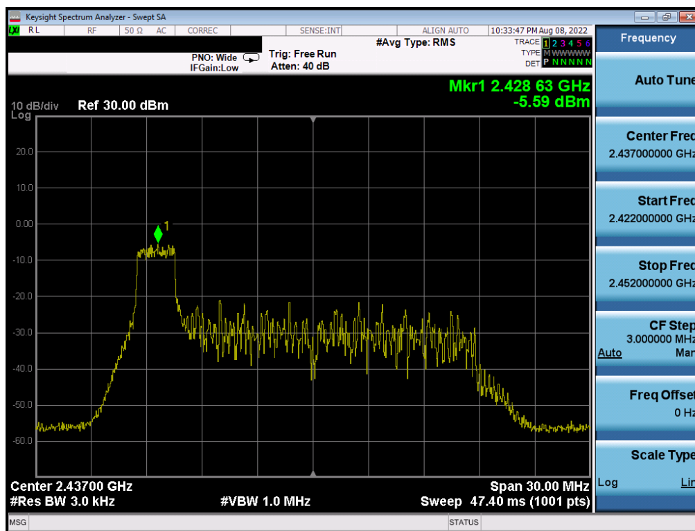
Plot 7-28. Power Spectral Density Plot Antenna 4a (802.11ax OFDMA – RU26 Index 0 – Ch. 6)
