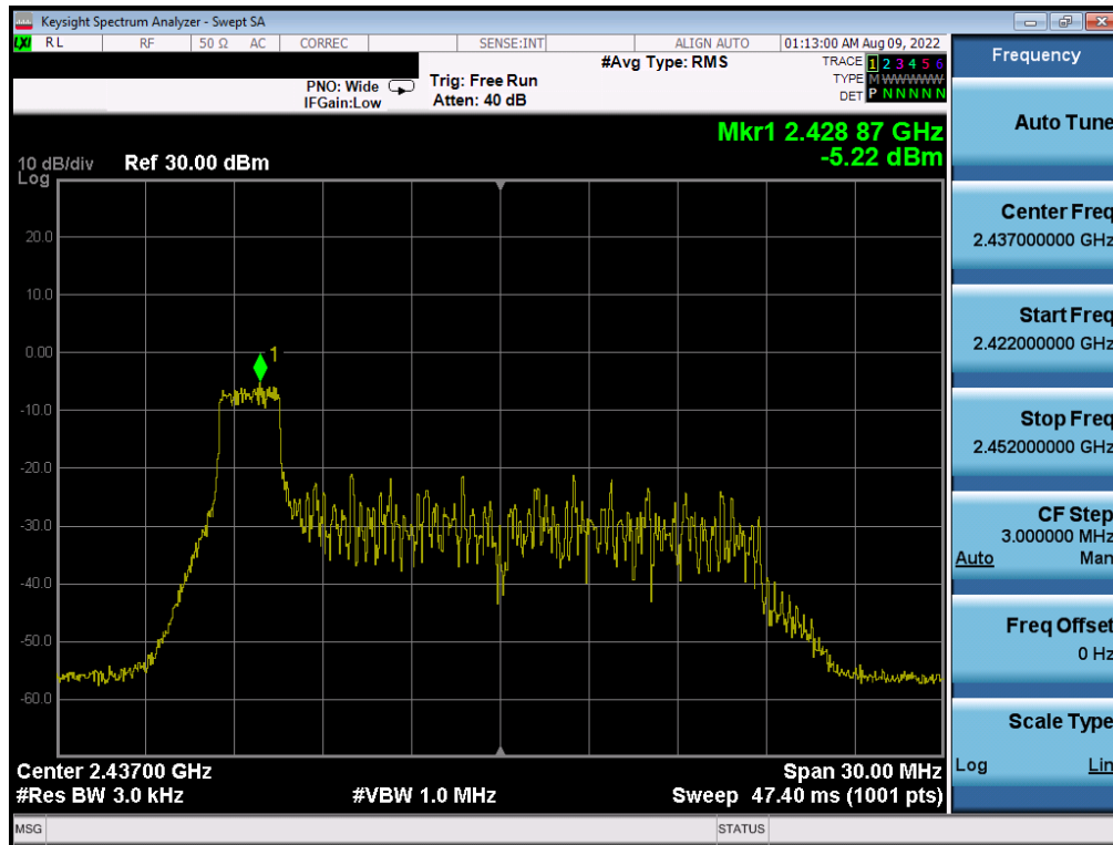
Plot 7-55. Power Spectral Density Plot CDD Antenna 4a (802.11ax OFDMA – RU26 Index 0 – Ch. 6)
