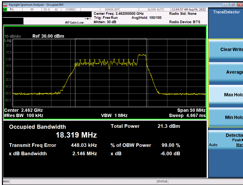
Plot 7-21. 6dB BW & 99% OBW Plot Antenna 2a (802.11ax OFDMA – RU26 Index 8 – Ch. 11)
