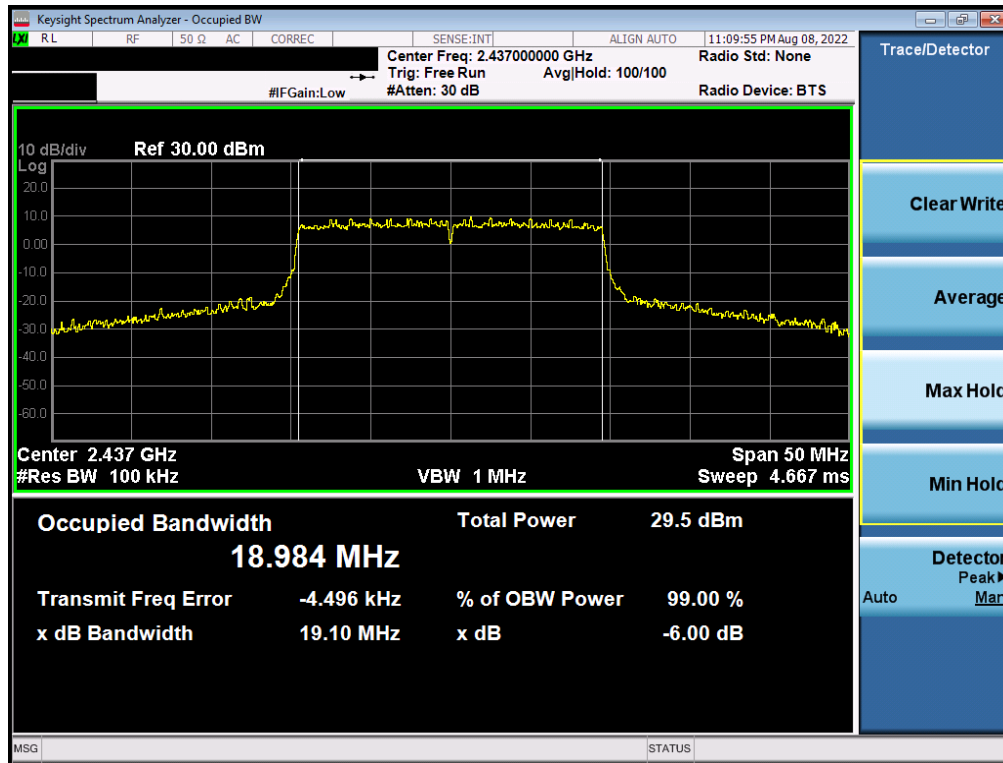
Plot 7-11. 6dB BW & 99% OBW Plot Antenna 4a (802.11ax OFDMA – RU242 – Ch. 6)
