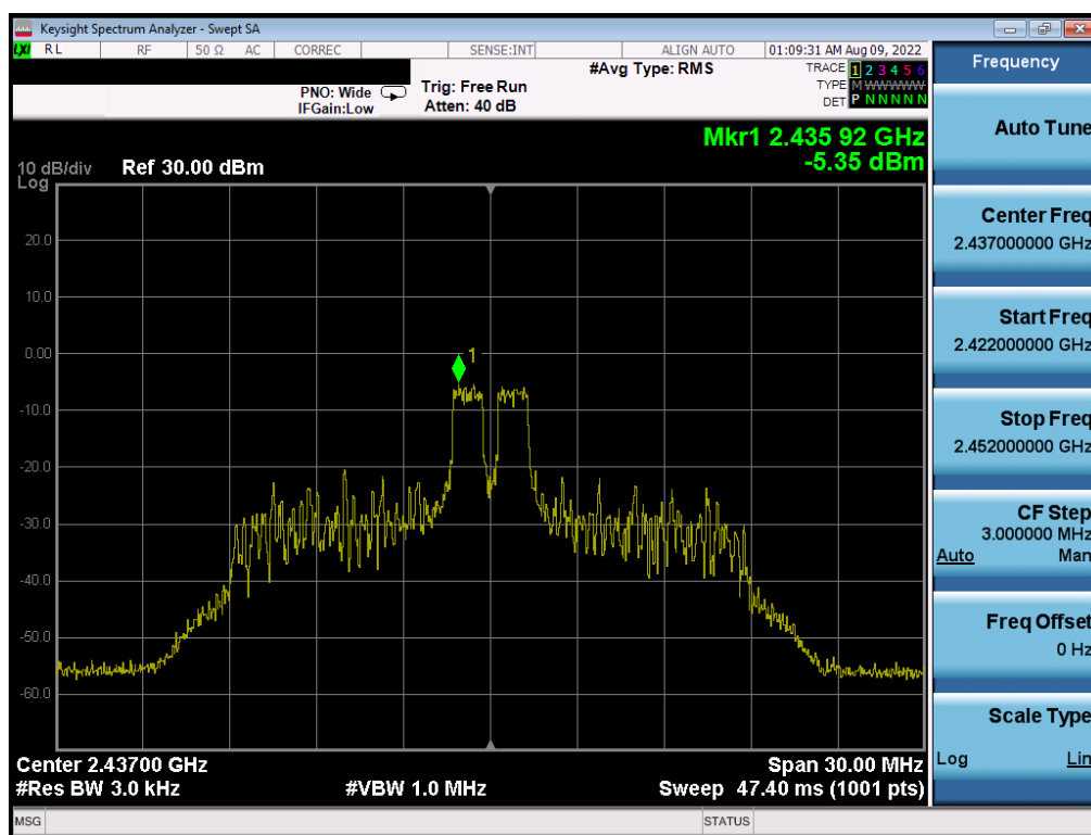
Plot 7-58. Power Spectral Density Plot CDD Antenna 2a (802.11ax OFDMA – RU26 Index 4 – Ch. 6)
