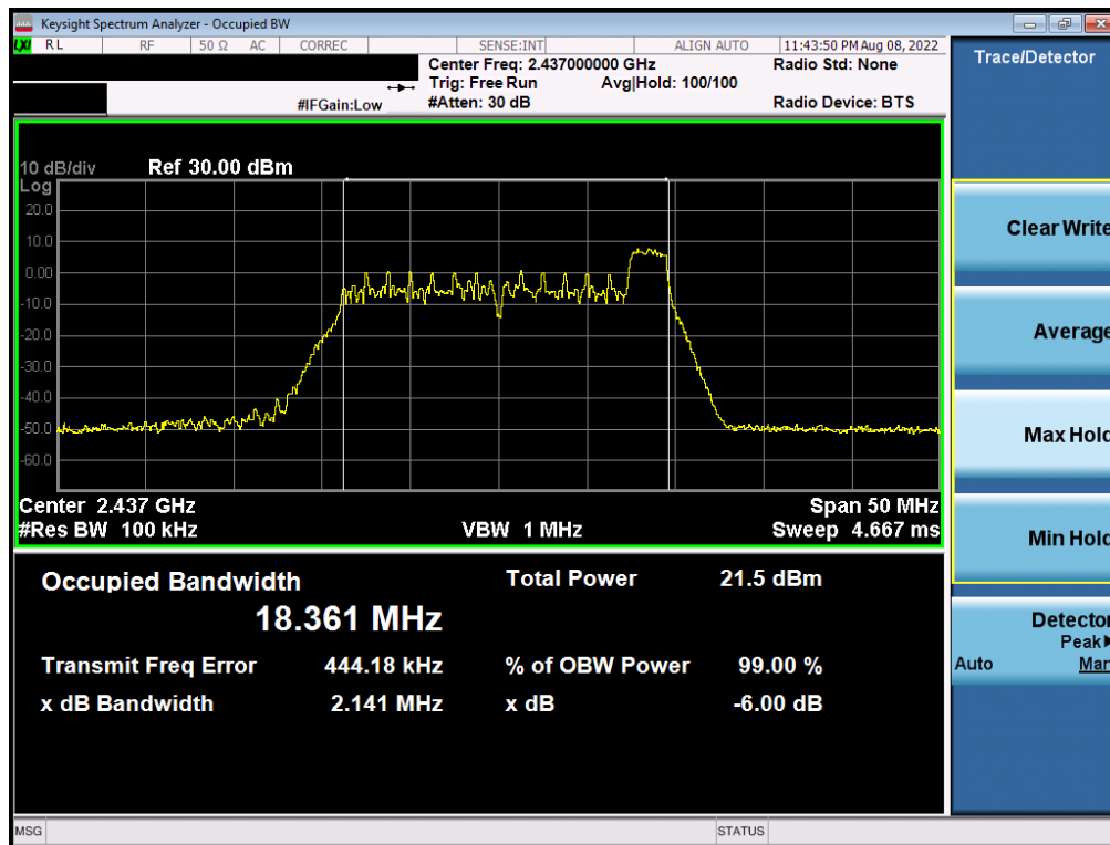
Plot 7-18. 6dB BW & 99% OBW Plot Antenna 2a (802.11ax OFDMA – RU26 Index 8 – Ch. 6)
