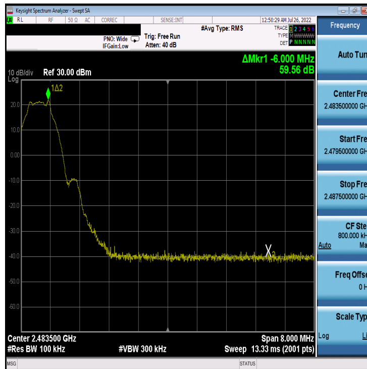
Plot 7-62. Band Edge Plot Antenna 4a (Bluetooth (LE), 1Mbps, ePA – Ch. 39)
