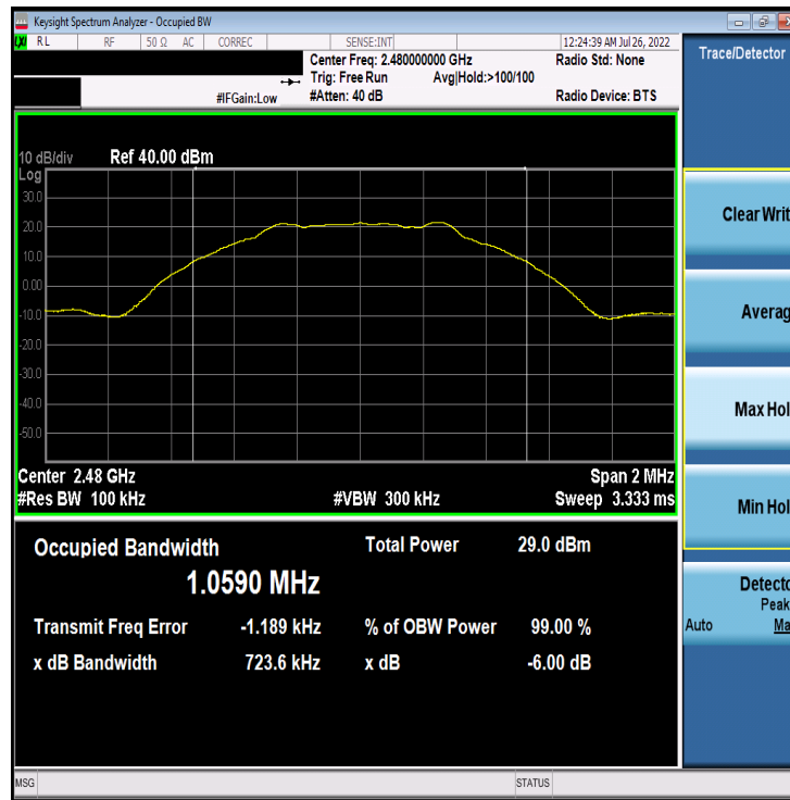
Plot 7-3. 6dB BW & 99% OBW Plot Antenna 4a (Bluetooth (LE), 1Mbps, ePA – Ch. 39)
