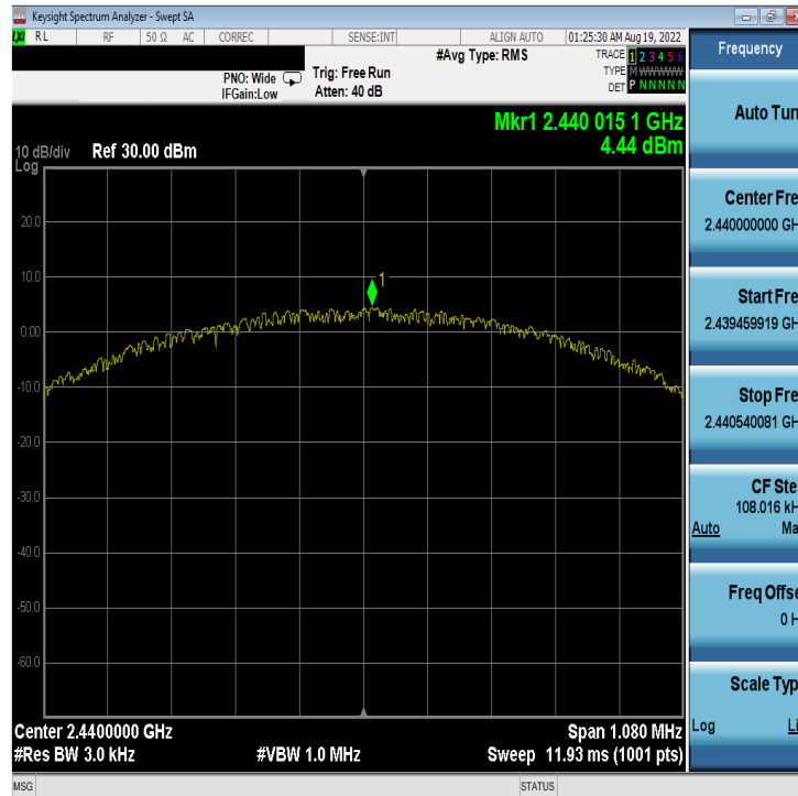
Plot 7-45. Power Spectral Density Plot Antenna 4a (Bluetooth (LE), 1Mbps, iPA – Ch. 19)
