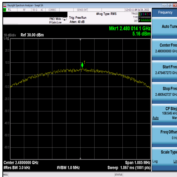
Plot 7-18. Power Spectral Density Plot Antenna 4a (Bluetooth (LE), 1Mbps, iPA – Ch. 39)
