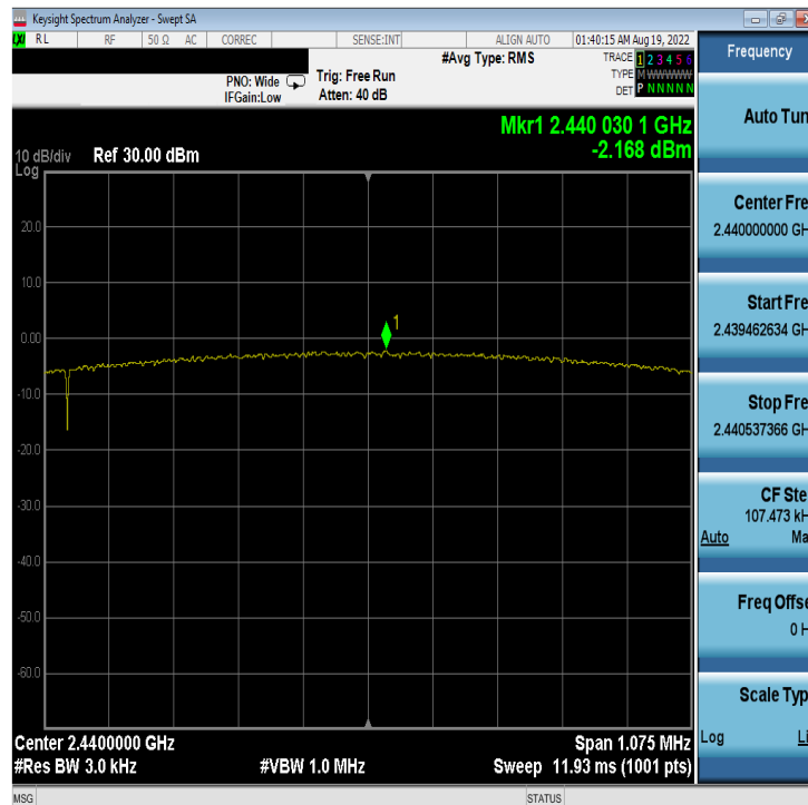
Plot 7-52. Power Spectral Density Plot Antenna 2a (Bluetooth (LE), 2Mbps, ePA – Ch. 19)
