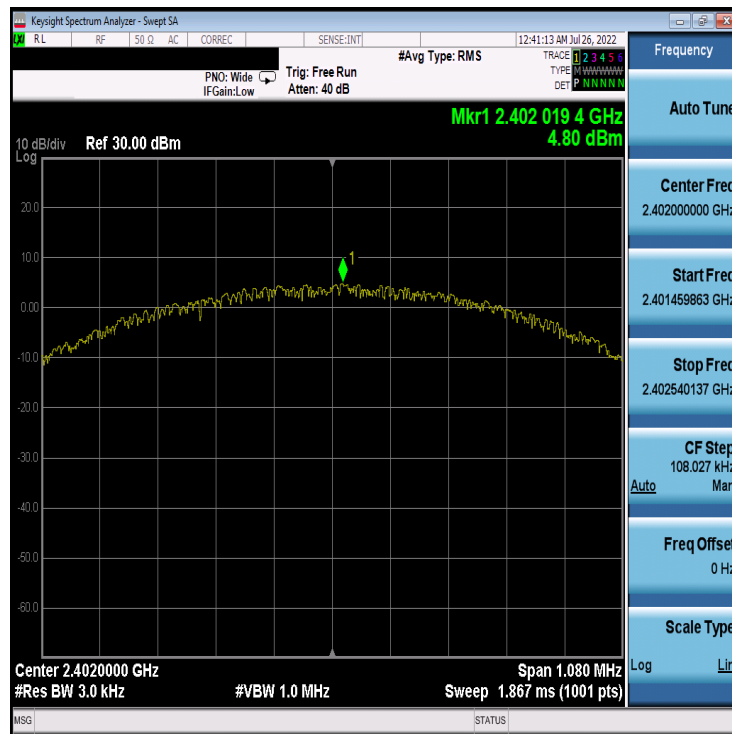
Plot 7-16. Power Spectral Density Plot Antenna 4a (Bluetooth (LE), 1Mbps, iPA – Ch. 0)
