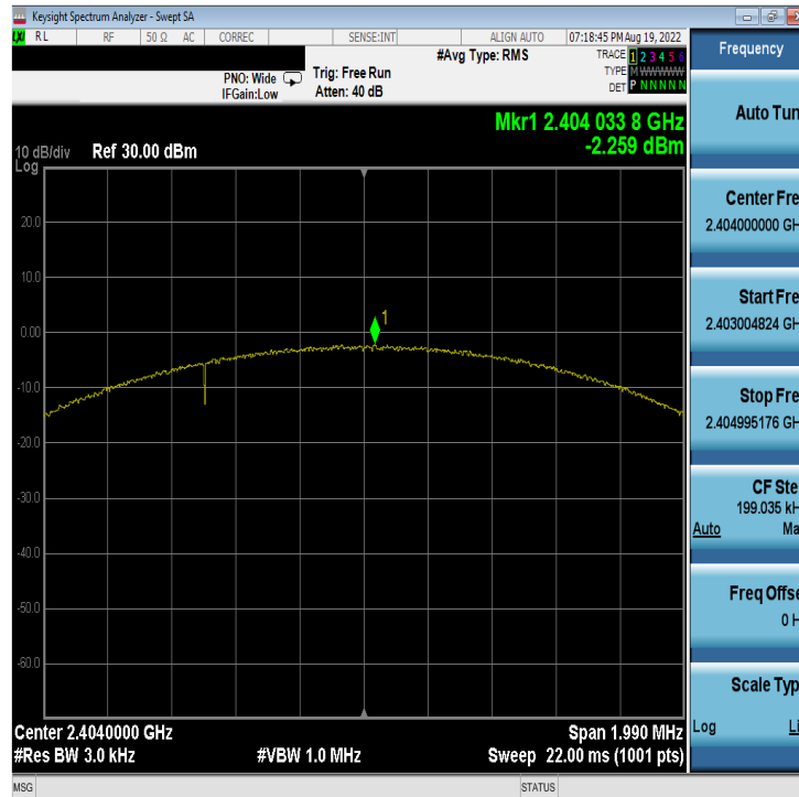
Plot 7-31. Power Spectral Density Plot Antenna 2a (Bluetooth (LE), 2Mbps, ePA – Ch. 1)
