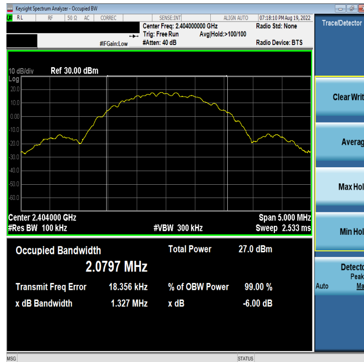
Plot 7-10. 6dB BW & 99% OBW Plot Antenna 2a (Bluetooth (LE), 2Mbps, ePA – Ch. 1)
