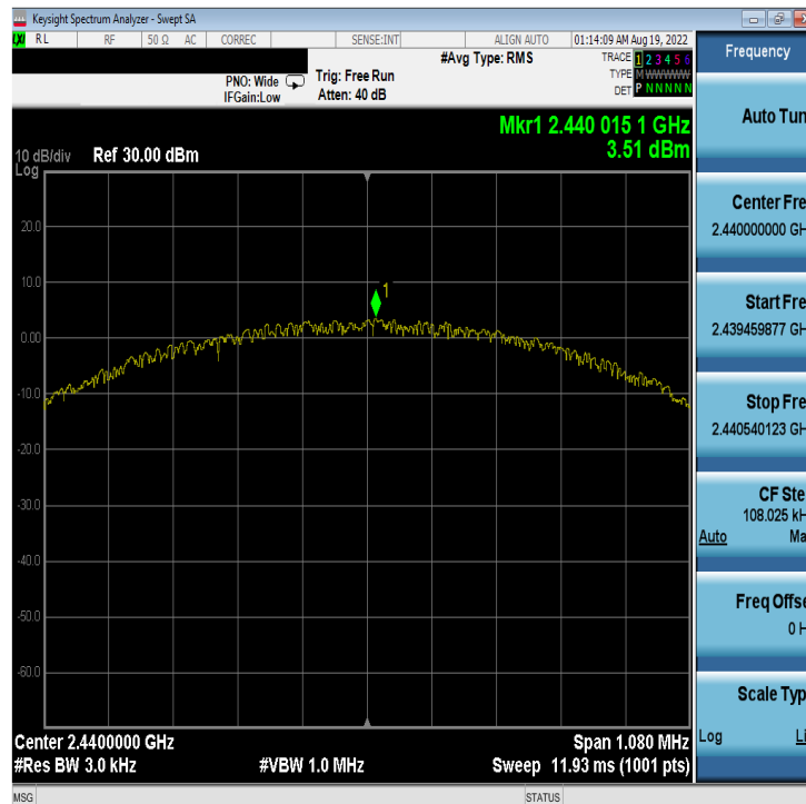
Plot 7-40. Power Spectral Density Plot Antenna 2a (Bluetooth (LE), 1Mbps, ePA – Ch. 19)
