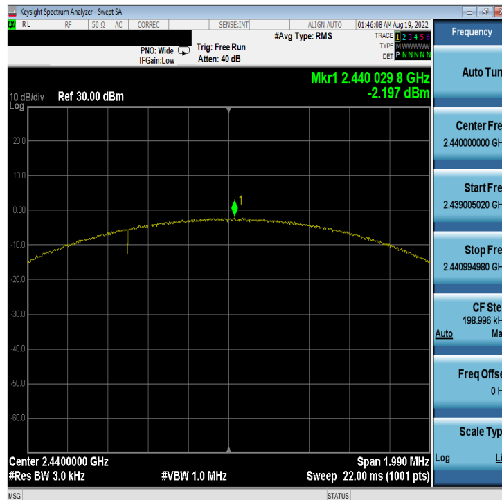
Plot 7-58. Power Spectral Density Plot Antenna 2a (Bluetooth (LE), 2Mbps, iPA – Ch. 19)
