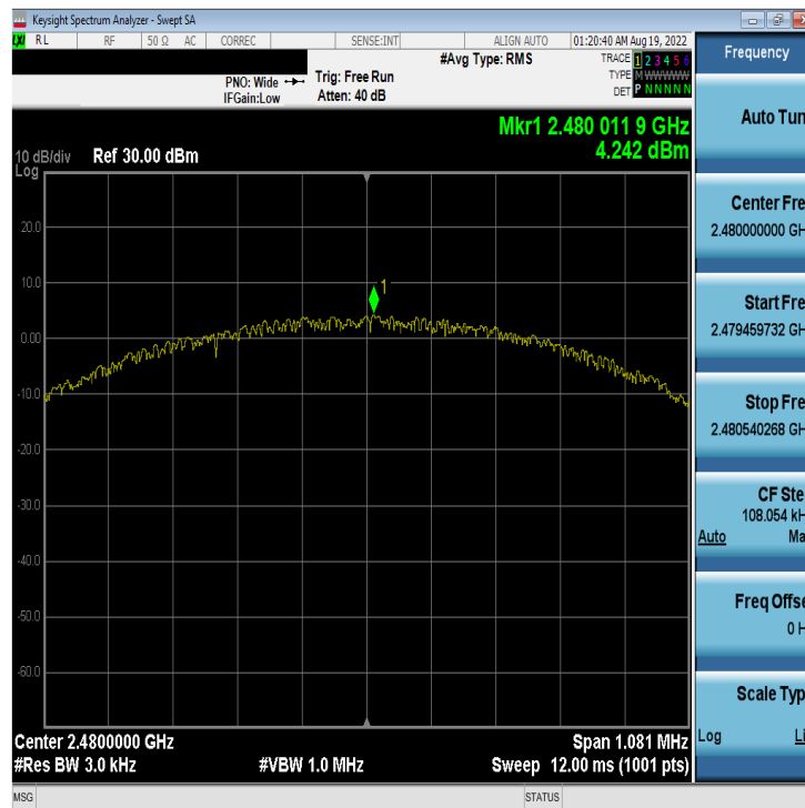
Plot 7-47. Power Spectral Density Plot Antenna 4a (Bluetooth (LE), 1Mbps, iPA – Ch. 39)
