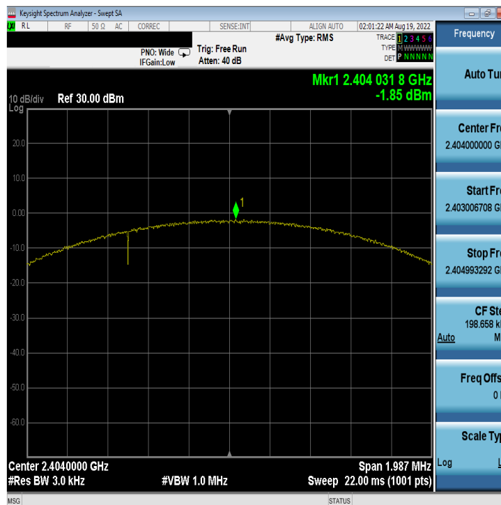
Plot 7-22. Power Spectral Density Plot Antenna 4a (Bluetooth (LE), 2Mbps, iPA – Ch. 1)
