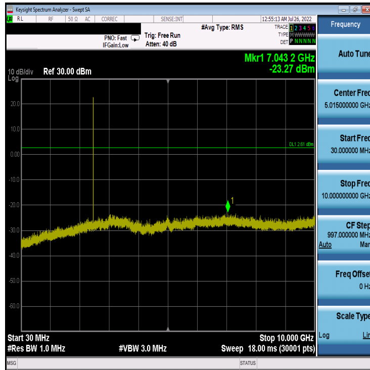
Plot 7-73. Conducted Spurious Plot Antenna 4a (Bluetooth (LE), 1Mbps, ePA – Ch. 39)
