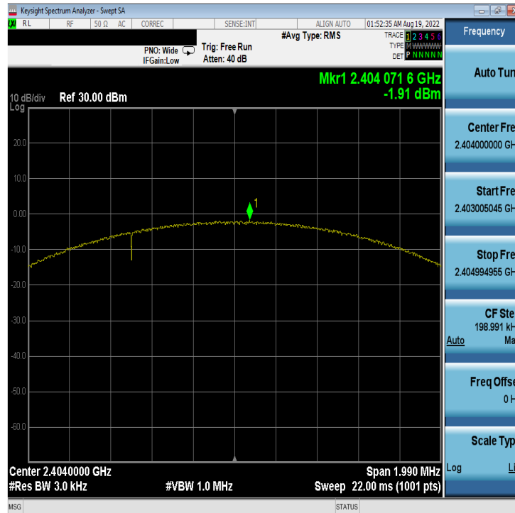
Plot 7-19. Power Spectral Density Plot Antenna 4a (Bluetooth (LE), 2Mbps, ePA – Ch. 1)
