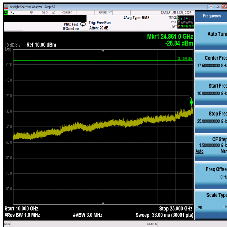
Plot 7-74. Conducted Spurious Plot Antenna 4a (Bluetooth (LE), 1Mbps, ePA – Ch. 39)
