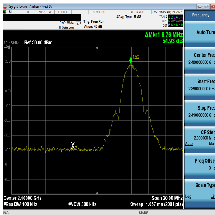
Plot 7-67. Band Edge Plot Antenna 2a (Bluetooth (LE), 2Mbps, ePA – Ch. 1)
