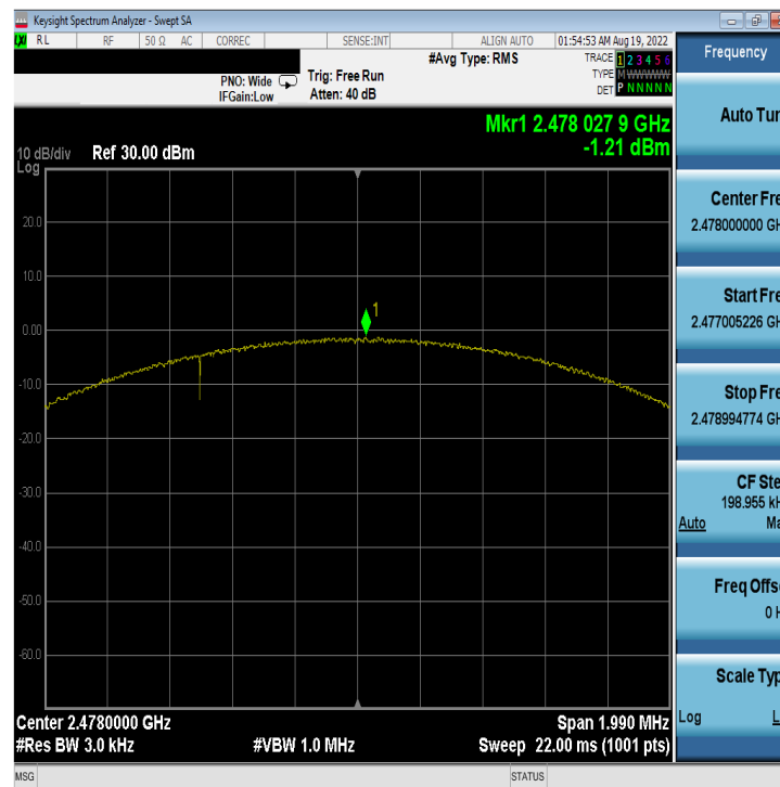
Plot 7-21. Power Spectral Density Plot Antenna 4a (Bluetooth (LE), 2Mbps, ePA – Ch. 38)
