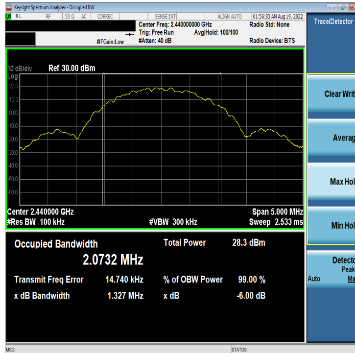
Plot 7-5. 6dB BW & 99% OBW Plot Antenna 4a (Bluetooth (LE), 2Mbps, ePA – Ch. 19)
