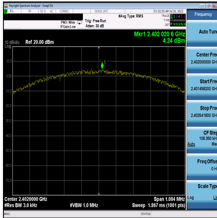
Plot 7-25. Power Spectral Density Plot Antenna 2a (Bluetooth (LE), 1Mbps, ePA – Ch. 0)
