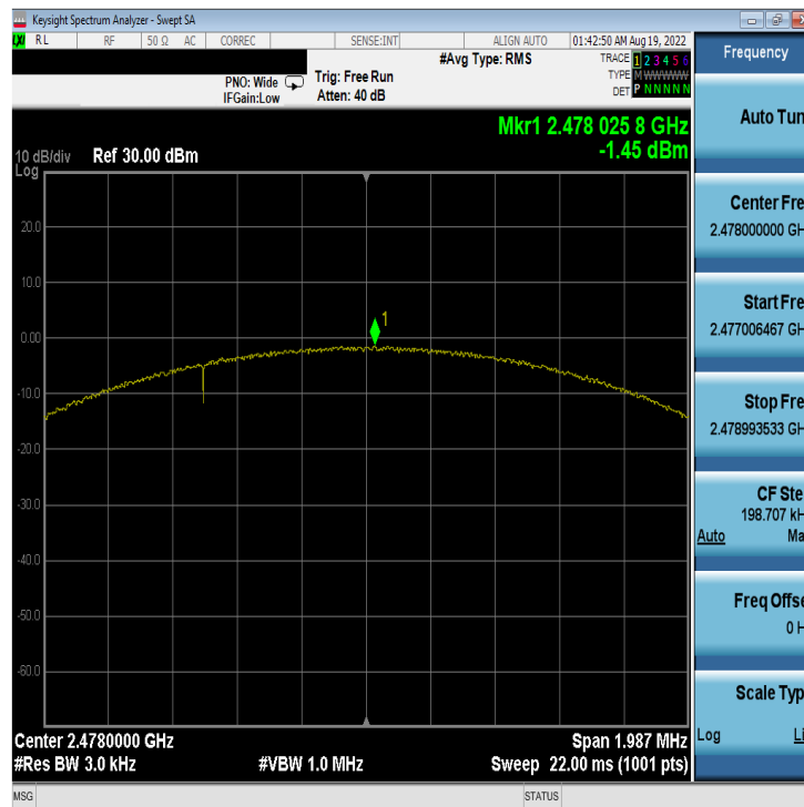
Plot 7-59. Power Spectral Density Plot Antenna 4a (Bluetooth (LE), 2Mbps, iPA – Ch. 38)
