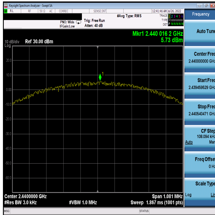
Plot 7-17. Power Spectral Density Plot Antenna 4a (Bluetooth (LE), 1Mbps, iPA – Ch. 19)
