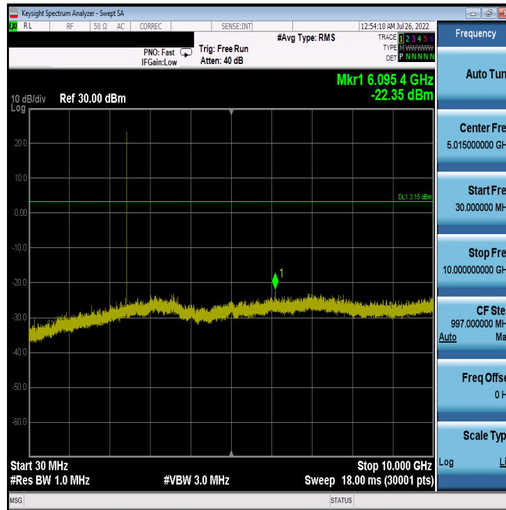
Plot 7-71. Conducted Spurious Plot Antenna 4a (Bluetooth (LE), 1Mbps, ePA – Ch. 19)
