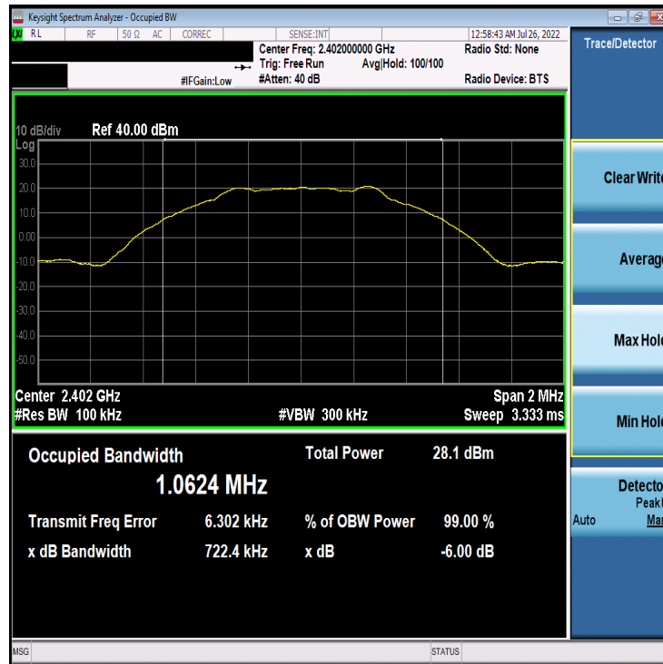
Plot 7-7. 6dB BW & 99% OBW Plot Antenna 2a (Bluetooth (LE), 1Mbps, ePA – Ch. 0)
