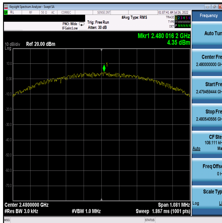
Plot 7-30. Power Spectral Density Plot Antenna 2a (Bluetooth (LE), 1Mbps, iPA – Ch. 39)
