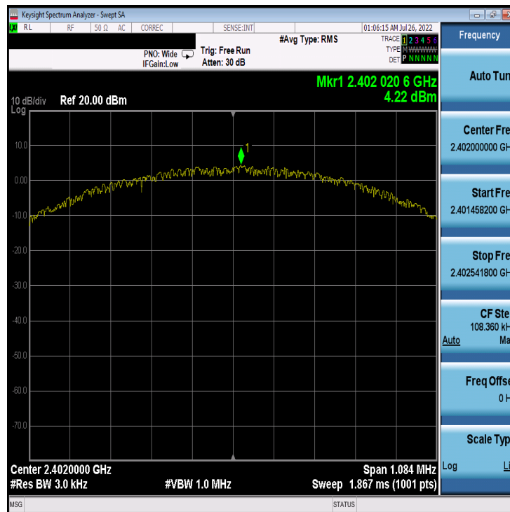
Plot 7-28. Power Spectral Density Plot Antenna 2a (Bluetooth (LE), 1Mbps, iPA – Ch. 0)
