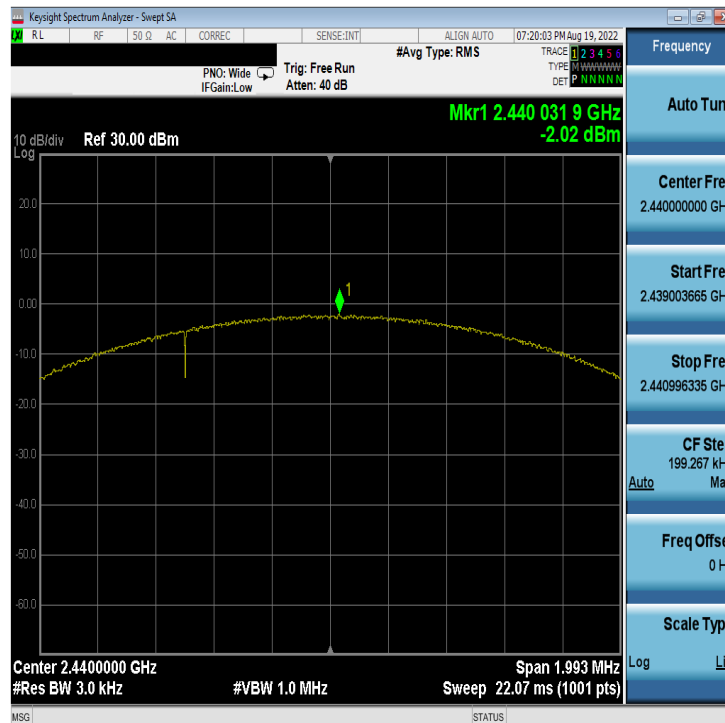
Plot 7-32. Power Spectral Density Plot Antenna 2a (Bluetooth (LE), 2Mbps, ePA – Ch. 19)
