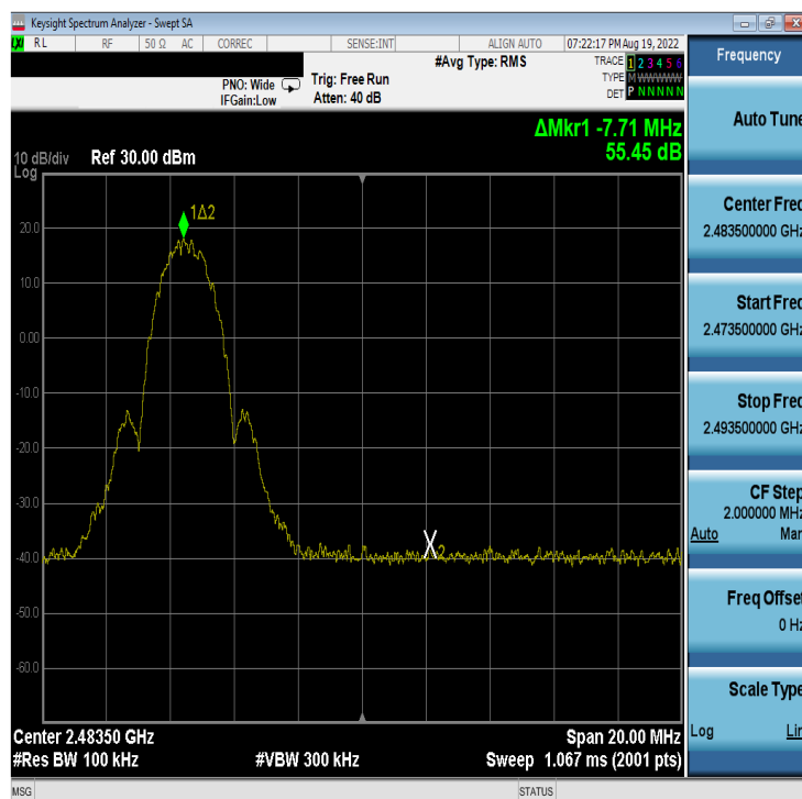
Plot 7-68. Band Edge Plot Antenna 2a (Bluetooth (LE), 2Mbps, ePA – Ch. 38)
