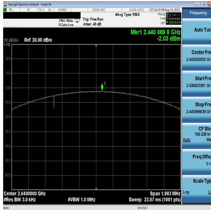
Plot 7-35. Power Spectral Density Plot Antenna 2a (Bluetooth (LE), 2Mbps, iPA – Ch. 19)
