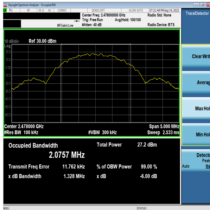
Plot 7-12. 6dB BW & 99% OBW Antenna 2a (Bluetooth (LE), 2Mbps, ePA – Ch. 38)
