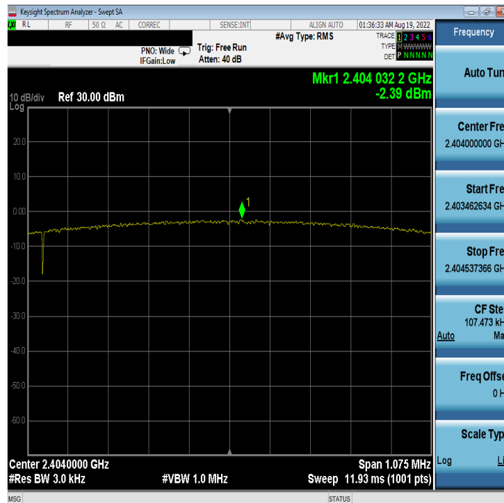
Plot 7-50. Power Spectral Density Plot Antenna 2a (Bluetooth (LE), 2Mbps, ePA – Ch. 1)
