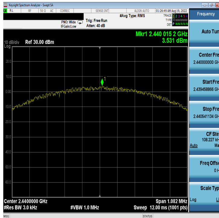
Plot 7-46. Power Spectral Density Plot Antenna 2a (Bluetooth (LE), 1Mbps, iPA – Ch. 19)
