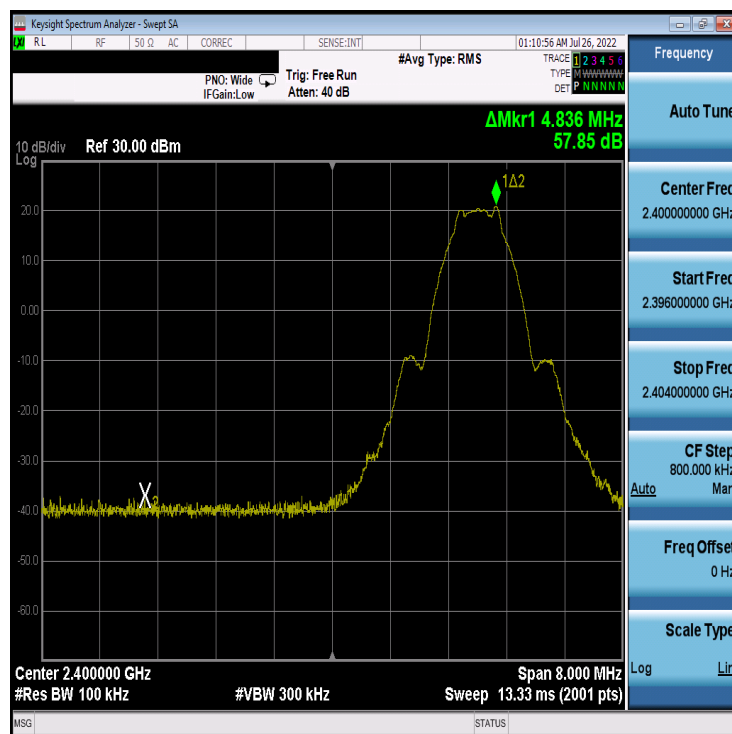
Plot 7-65. Band Edge Plot Antenna 2a (Bluetooth (LE), 1Mbps, ePA – Ch. 0)
