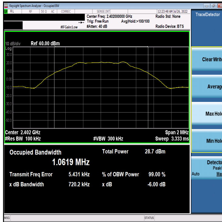
Plot 7-1. 6dB BW & 99% OBW Plot Antenna 4a (Bluetooth (LE), 1Mbps, ePA – Ch. 0)
