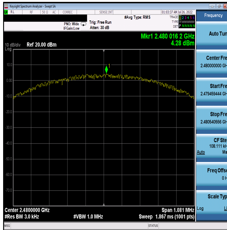
Plot 7-27. Power Spectral Density Plot Antenna 2a (Bluetooth (LE), 1Mbps, ePA – Ch. 39)
