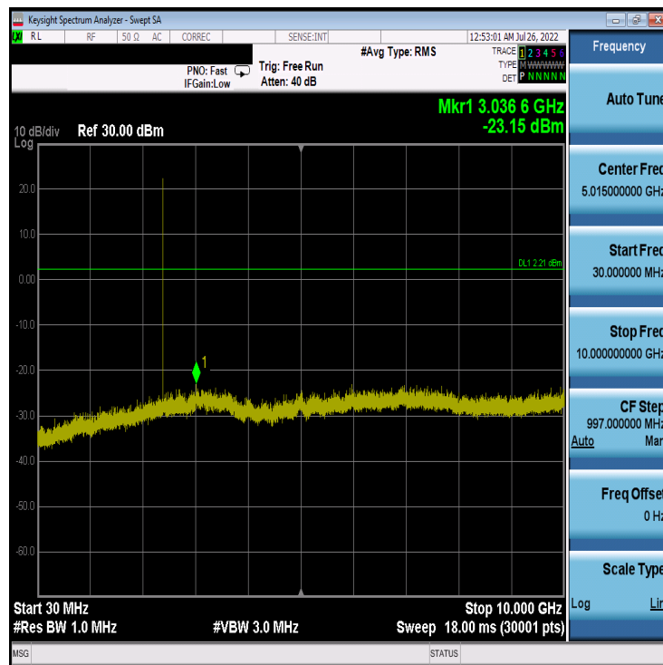
Plot 7-69. Conducted Spurious Plot Antenna 4a (Bluetooth (LE), 1Mbps, ePA – Ch. 0)
