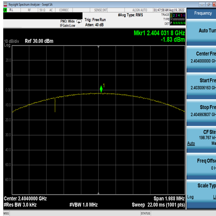
Plot 7-55. Power Spectral Density Plot Antenna 4a (Bluetooth (LE), 2Mbps, iPA – Ch. 1)
