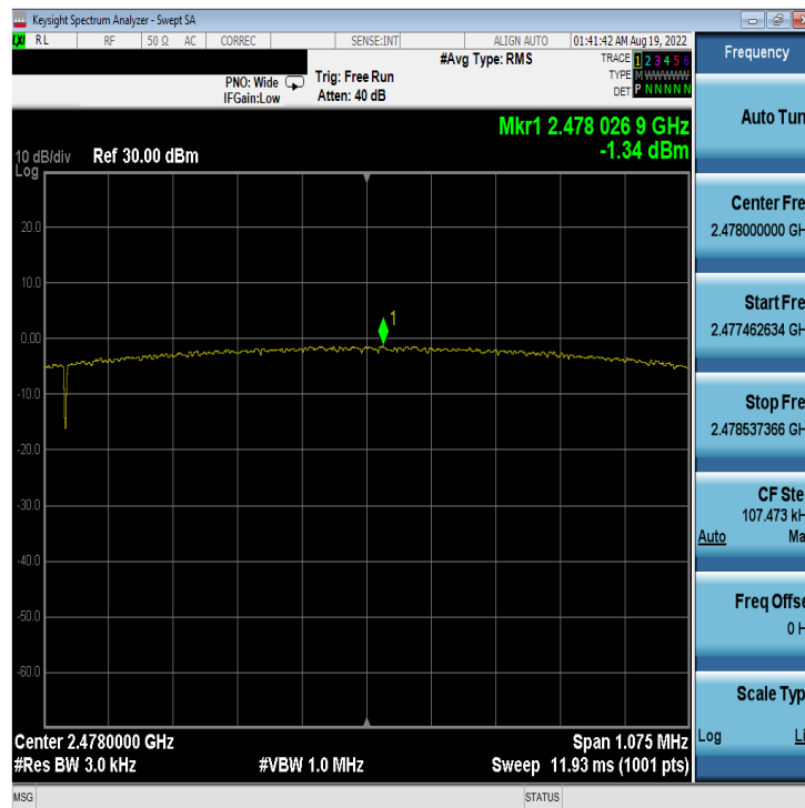
Plot 7-53. Power Spectral Density Plot Antenna 4a (Bluetooth (LE), 2Mbps, ePA – Ch. 38)
