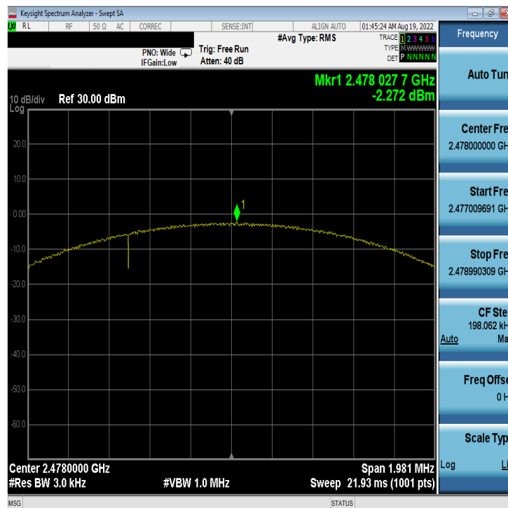
Plot 7-60. Power Spectral Density Plot Antenna 2a (Bluetooth (LE), 2Mbps, iPA – Ch. 38)
