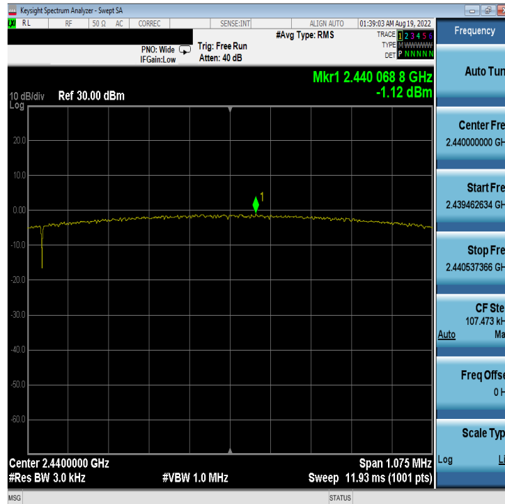
Plot 7-51. Power Spectral Density Plot Antenna 4a (Bluetooth (LE), 2Mbps, ePA – Ch. 19)
