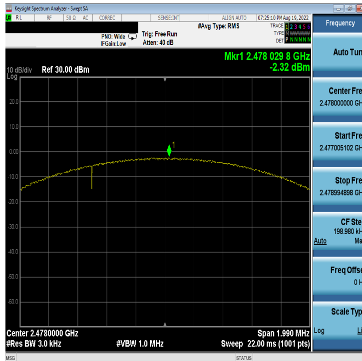
Plot 7-36. Power Spectral Density Plot Antenna 2a (Bluetooth (LE), 2Mbps, iPA – Ch. 38)
