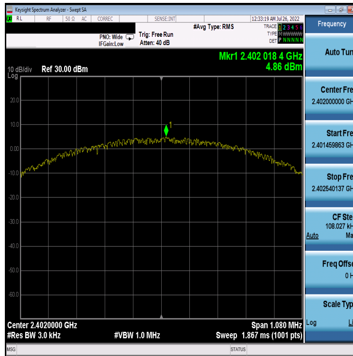
Plot 7-13. Power Spectral Density Plot Antenna 4a (Bluetooth (LE), 1Mbps, ePA – Ch. 0)
