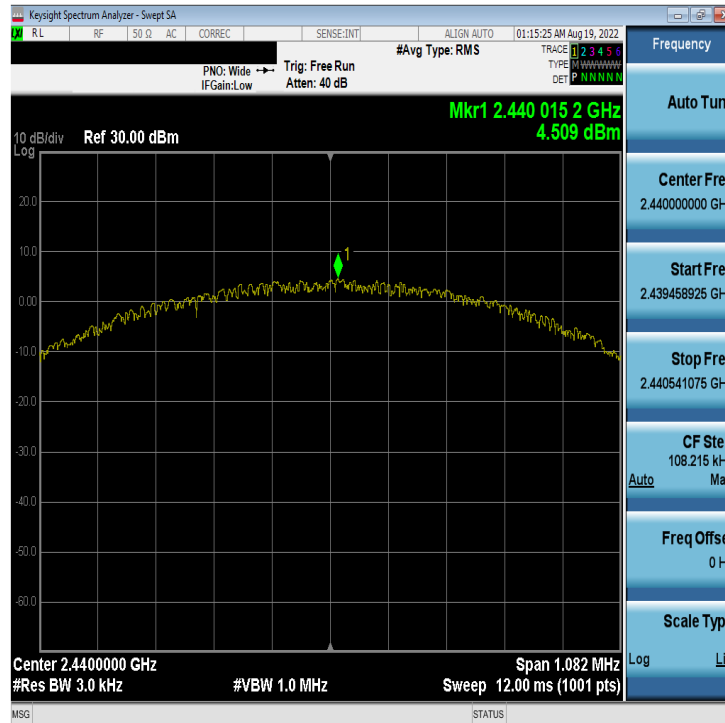
Plot 7-39. Power Spectral Density Plot Antenna 4a (Bluetooth (LE), 1Mbps, ePA – Ch. 19)
