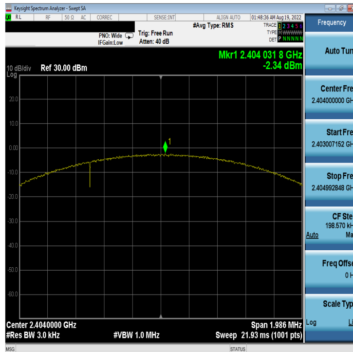
Plot 7-56. Power Spectral Density Plot Antenna 2a (Bluetooth (LE), 2Mbps, iPA – Ch. 1)
