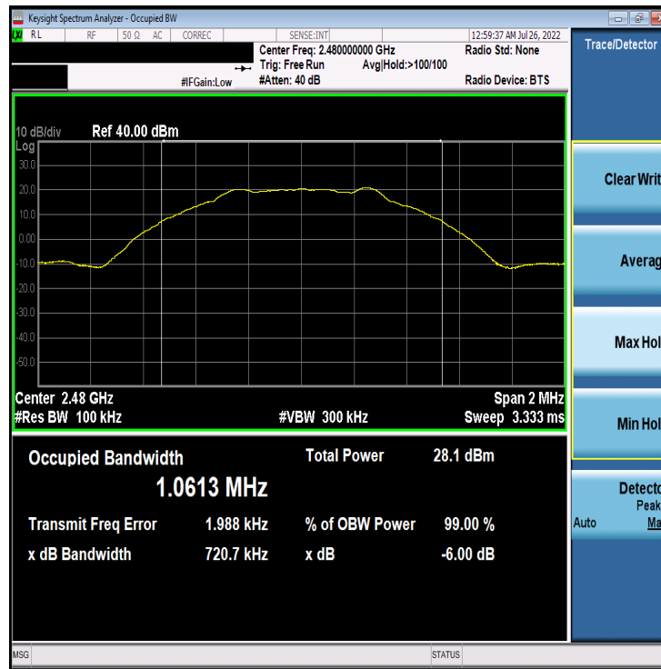
Plot 7-9. 6dB BW & 99% OBW Plot Antenna 2a (Bluetooth (LE), 1Mbps, ePA – Ch. 39)
