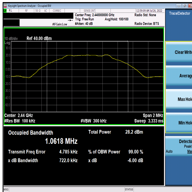
Plot 7-8. 6dB BW & 99% OBW Plot Antenna 2a (Bluetooth (LE), 1Mbps, ePA – Ch. 19)
