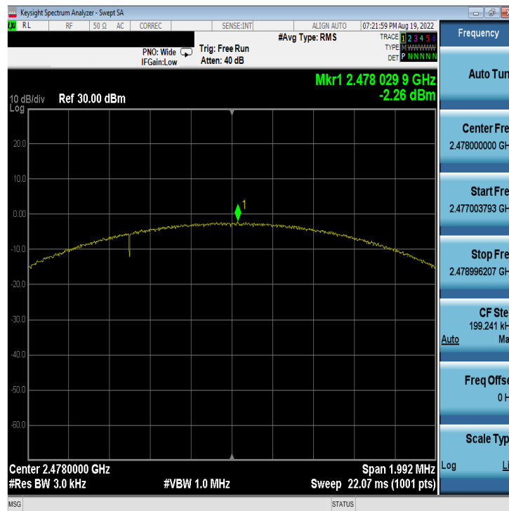
Plot 7-33. Power Spectral Density Plot Antenna 2a (Bluetooth (LE), 2Mbps, ePA – Ch. 38)
