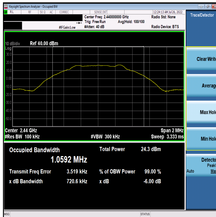
Plot 7-2. 6dB BW & 99% OBW Plot Antenna 4a (Bluetooth (LE), 1Mbps, ePA – Ch. 19)
