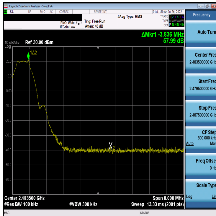
Plot 7-66. Band Edge Plot Antenna 2a (Bluetooth (LE), 1Mbps, ePA – Ch. 39)
