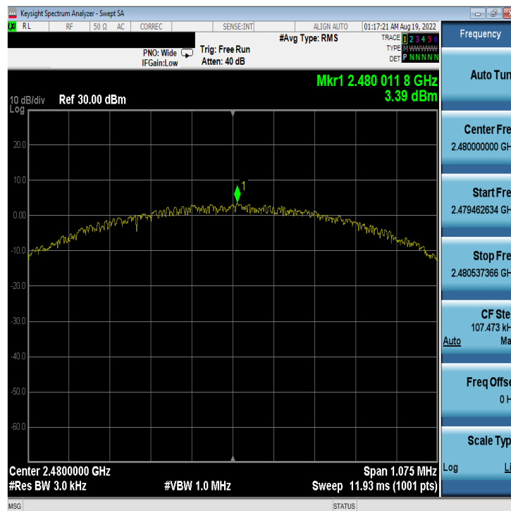
Plot 7-42. Power Spectral Density Plot Antenna 2a (Bluetooth (LE), 1Mbps, ePA – Ch. 39)
