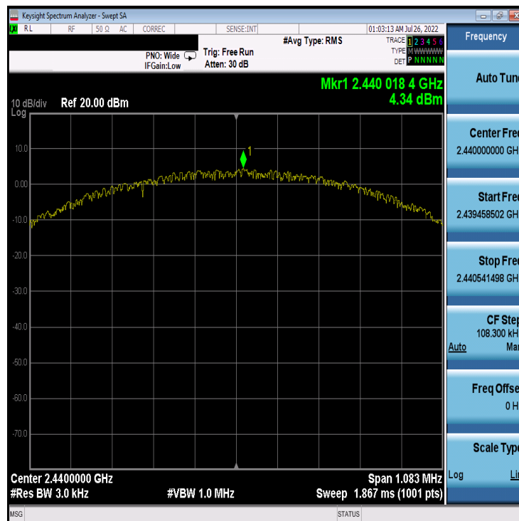
Plot 7-26. Power Spectral Density Plot Antenna 2a (Bluetooth (LE), 1Mbps, ePA – Ch. 19)
