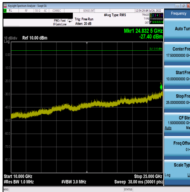
Plot 7-72. Conducted Spurious Plot Antenna 4a (Bluetooth (LE), 1Mbps, ePA – Ch. 19)
