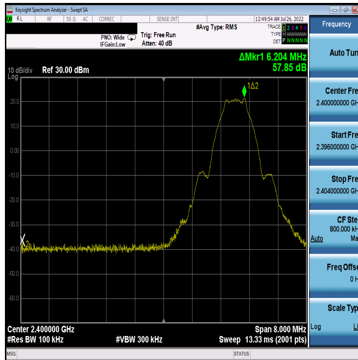
Plot 7-61. Band Edge Plot Antenna 4a (Bluetooth (LE), 1Mbps, ePA – Ch. 0)
