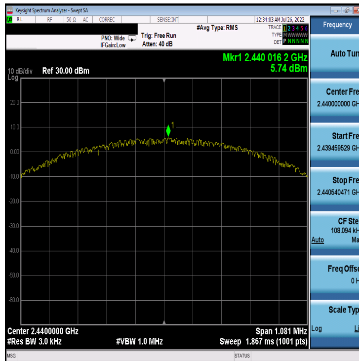
Plot 7-14. Power Spectral Density Plot Antenna 4a (Bluetooth (LE), 1Mbps, ePA – Ch. 19)
