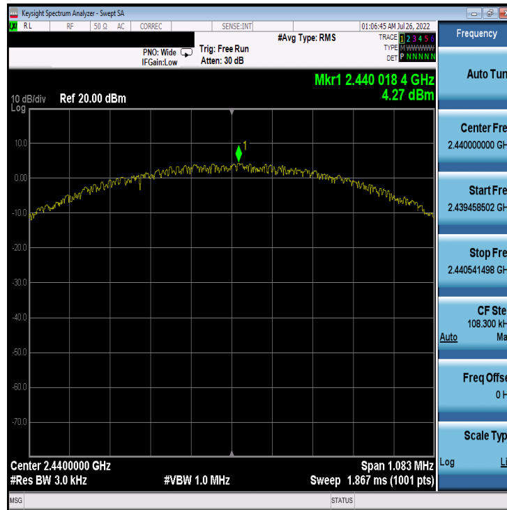
Plot 7-29. Power Spectral Density Plot Antenna 2a (Bluetooth (LE), 1Mbps, iPA – Ch. 19)
