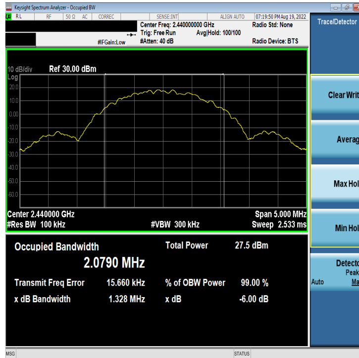
Plot 7-11. 6dB BW & 99% OBW Plot Antenna 2a (Bluetooth (LE), 2Mbps, ePA – Ch. 19)
