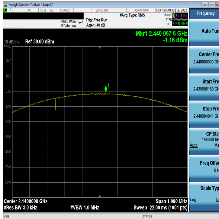
Plot 7-57. Power Spectral Density Plot Antenna 4a (Bluetooth (LE), 2Mbps, iPA – Ch. 19)
