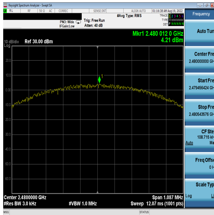
Plot 7-41. Power Spectral Density Plot Antenna 4a (Bluetooth (LE), 1Mbps, ePA – Ch. 39)
