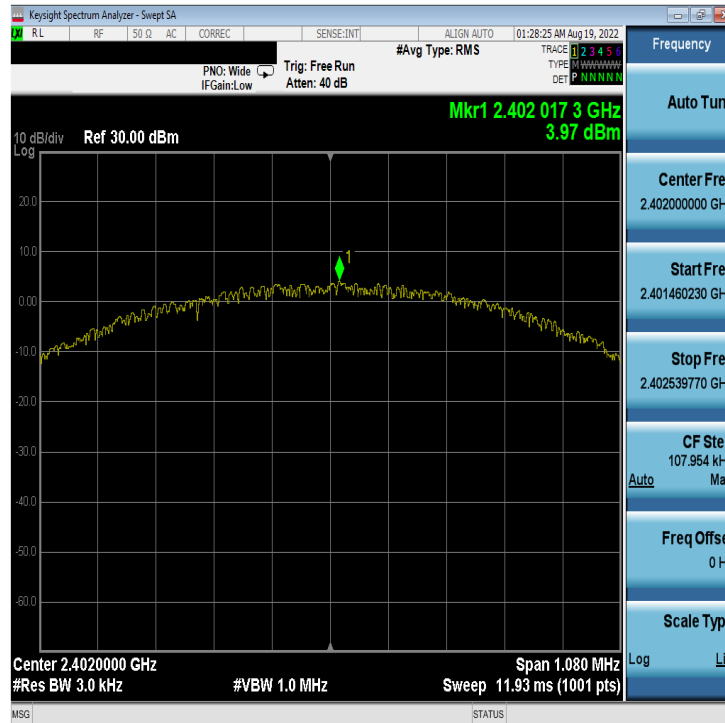
Plot 7-43. Power Spectral Density Plot Antenna 4a (Bluetooth (LE), 1Mbps, iPA – Ch. 0)
