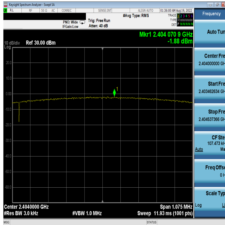
Plot 7-49. Power Spectral Density Plot Antenna 4a (Bluetooth (LE), 2Mbps, ePA – Ch. 1)
