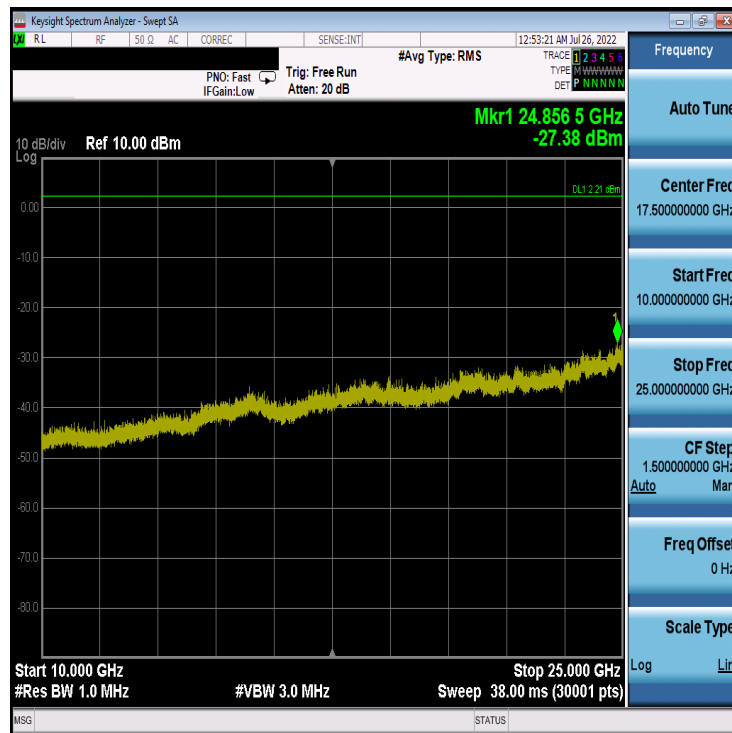
Plot 7-70. Conducted Spurious Plot Antenna 4a (Bluetooth (LE), 1Mbps, ePA – Ch. 0)
