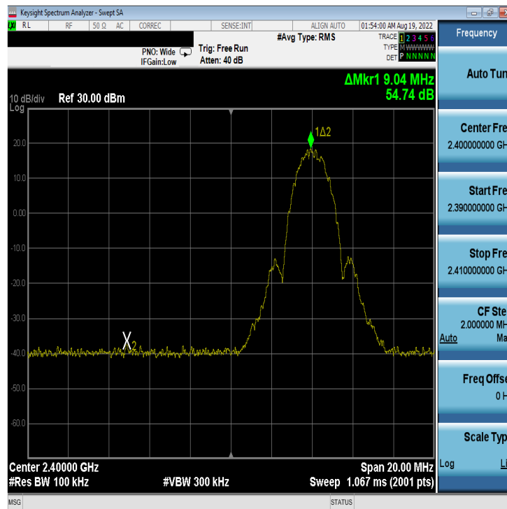
Plot 7-63. Band Edge Plot Antenna 4a (Bluetooth (LE), 2Mbps, ePA – Ch. 1)
