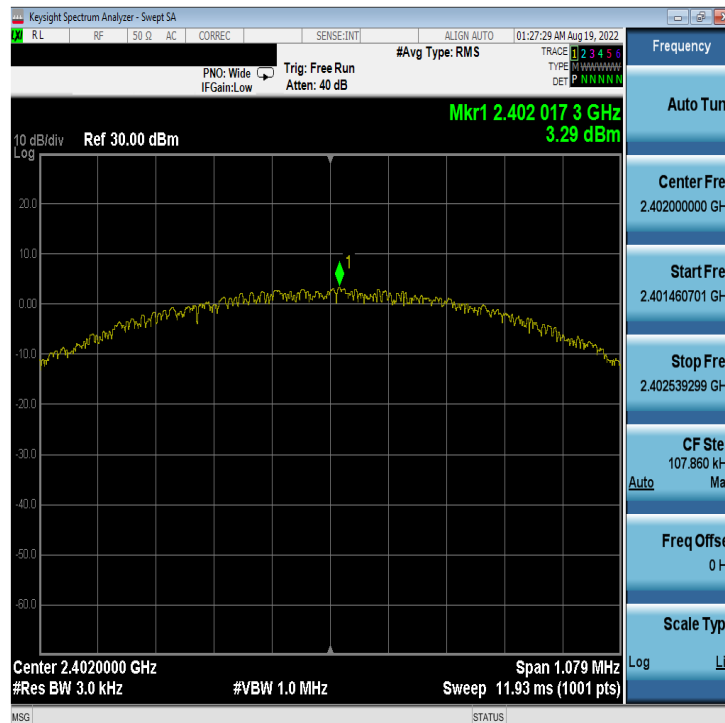
Plot 7-44. Power Spectral Density Plot Antenna 2a (Bluetooth (LE), 1Mbps, iPA – Ch. 0)
