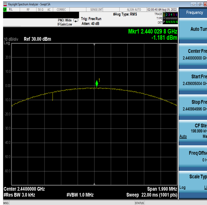
Plot 7-23. Power Spectral Density Plot Antenna 4a (Bluetooth (LE), 2Mbps, iPA – Ch. 19)
