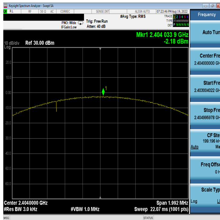
Plot 7-34. Power Spectral Density Plot Antenna 2a (Bluetooth (LE), 2Mbps, iPA – Ch. 1)
