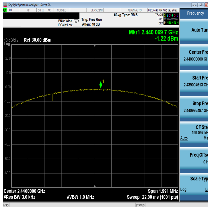
Plot 7-20. Power Spectral Density Plot Antenna 4a (Bluetooth (LE), 2Mbps, ePA – Ch. 19)
