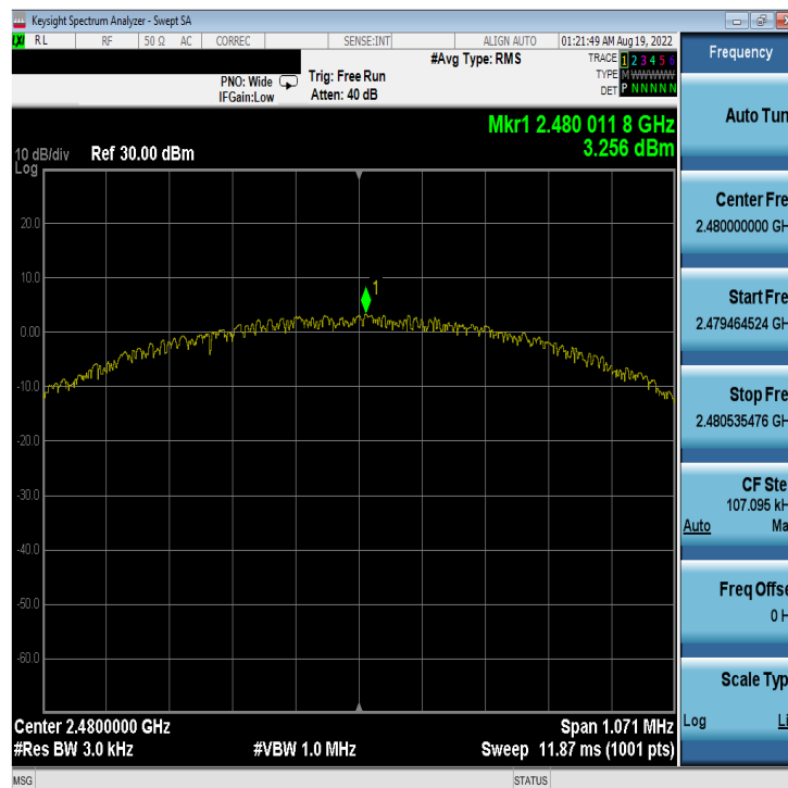
Plot 7-48. Power Spectral Density Plot Antenna 2a (Bluetooth (LE), 1Mbps, iPA – Ch. 39)
