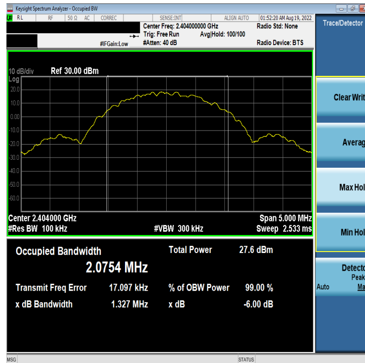
Plot 7-4. 6dB BW & 99% OBW Plot Antenna 4a (Bluetooth (LE), 2Mbps, ePA – Ch. 1)
