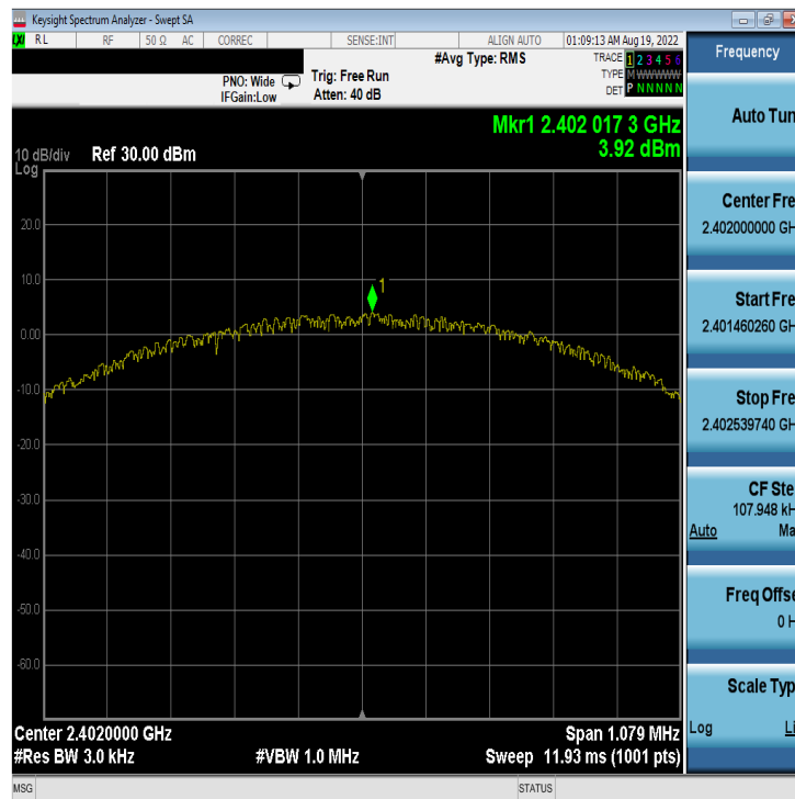
Plot 7-37. Power Spectral Density Plot Antenna 4a (Bluetooth (LE), 1Mbps, ePA – Ch. 0)
