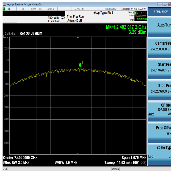
Plot 7-38. Power Spectral Density Plot Antenna 2a (Bluetooth (LE), 1Mbps, ePA – Ch. 0)
