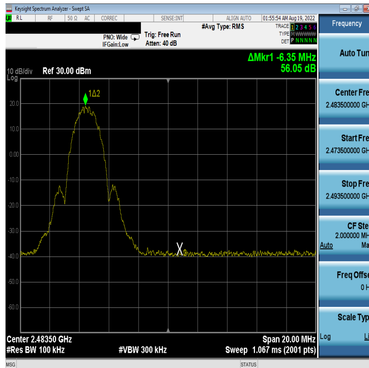
Plot 7-64. Band Edge Plot Antenna 4a (Bluetooth (LE), 2Mbps, ePA – Ch. 38)
