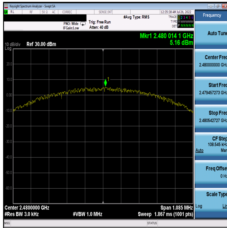
Plot 7-15. Power Spectral Density Plot Antenna 4a (Bluetooth (LE), 1Mbps, ePA – Ch. 39)
