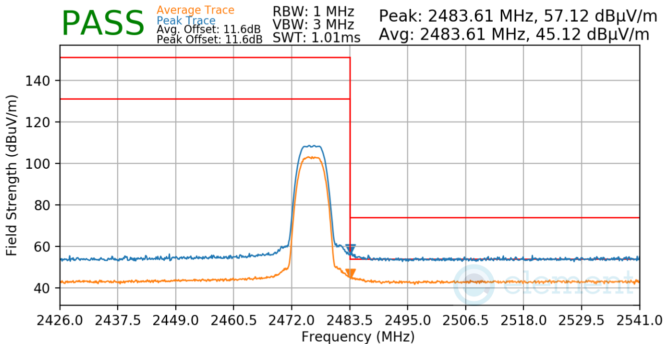
Plot 7-95. Radiated Restricted Upper Band Edge Measurement Antenna 4a
