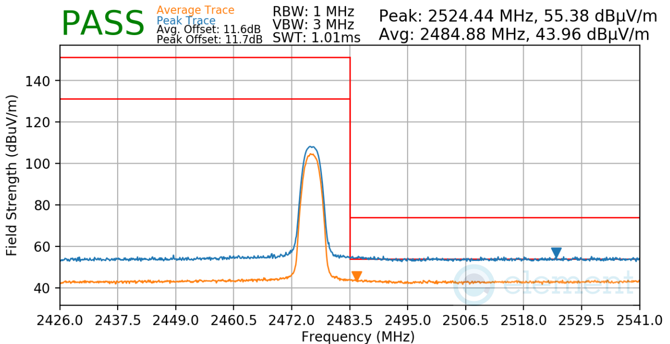
Plot 7-98. Radiated Restricted Upper Band Edge Measurement Antenna 2a
