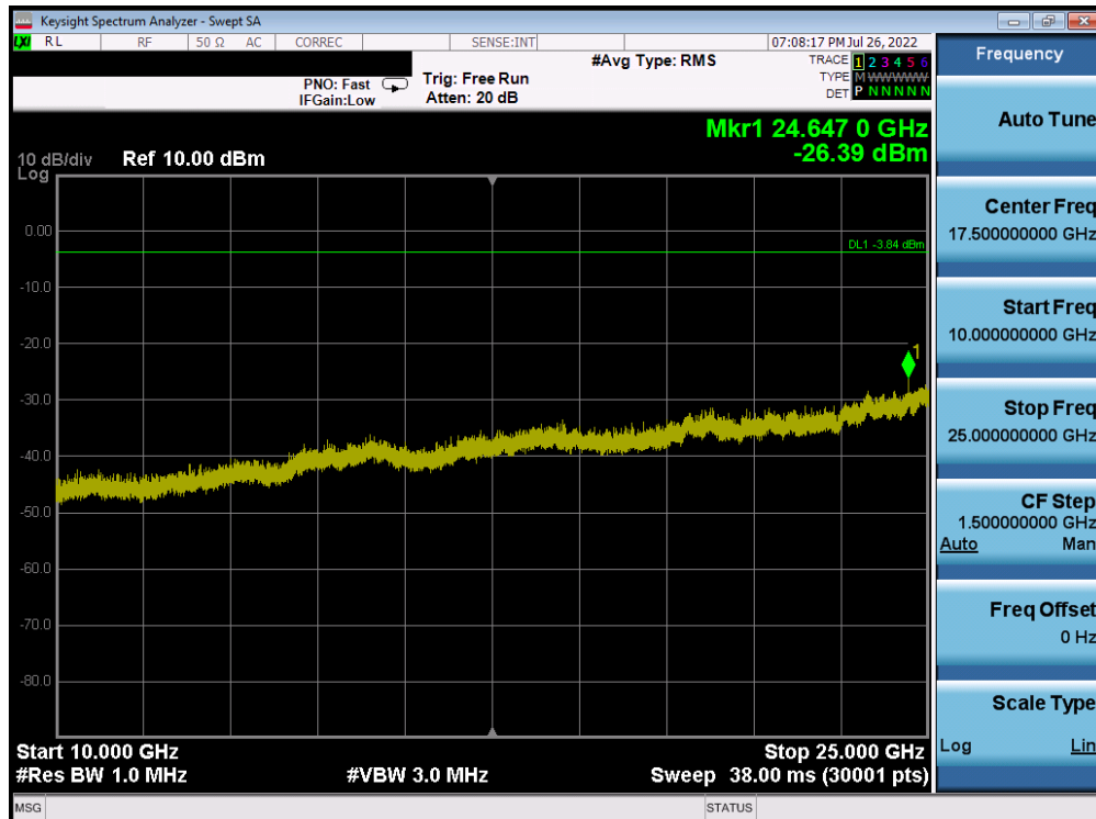
Plot 7-76. Conducted Spurious Plot Antenna 2a (Bluetooth (HDR4), 4 Mbps, ePA – Ch. 1)
