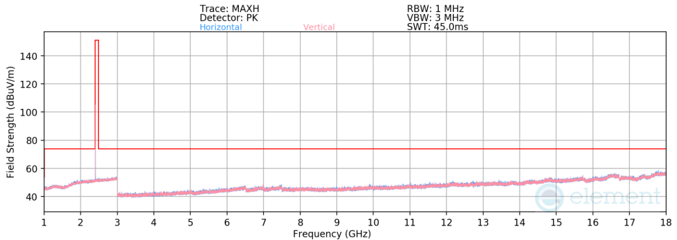
Plot 7-81. Radiated Spurious Emissions 1-18GHz Antenna 4a (4Mbps, HDR4, ePA – Ch. 1)
