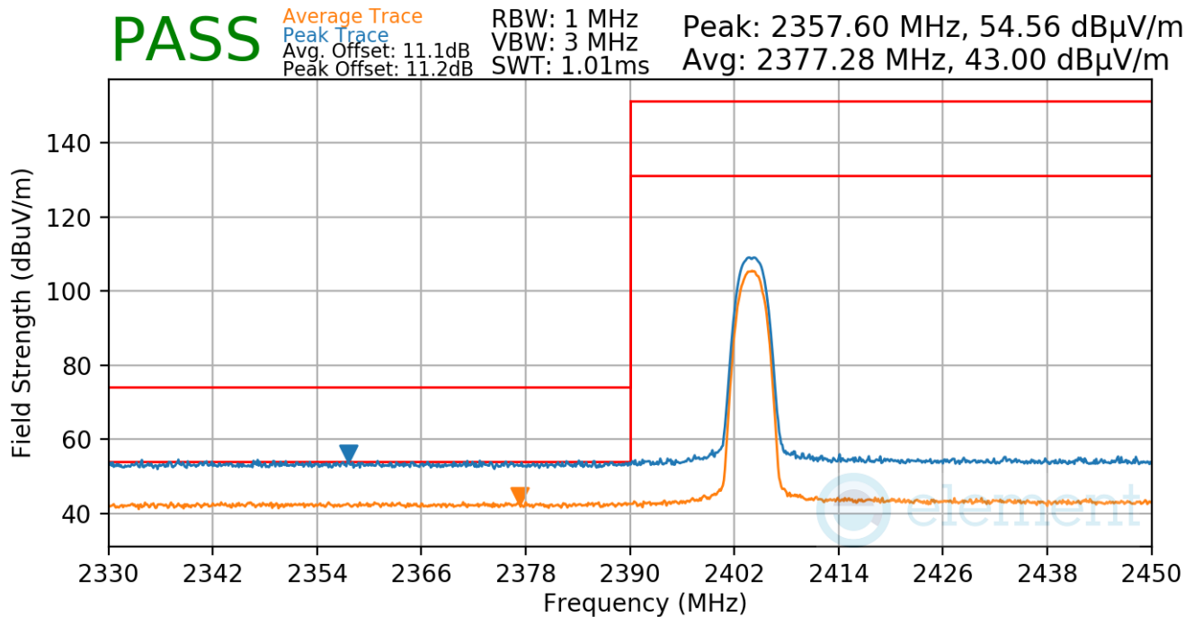
Plot 7-92. Radiated Restricted Lower Band Edge Measurement Antenna 4a
