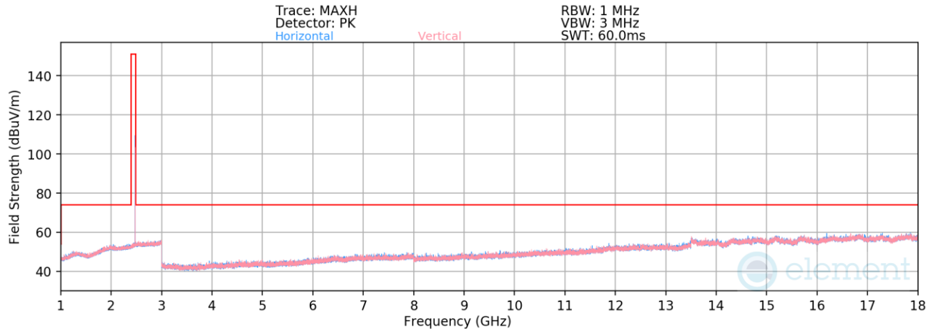
Plot 7-83. Radiated Spurious Emissions 1-18GHz Antenna 4a (4Mbps, HDR4, ePA – Ch. 73)
