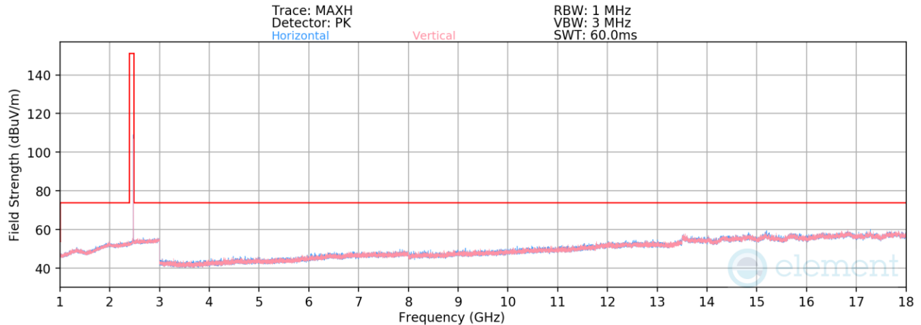
Plot 7-86. Radiated Spurious Emissions 1-18GHz Antenna 2a (4Mbps, HDR4, ePA – Ch. 73)
