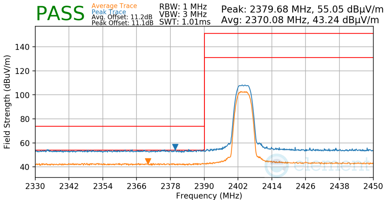
Plot 7-93. Radiated Restricted Lower Band Edge Measurement Antenna 4a
