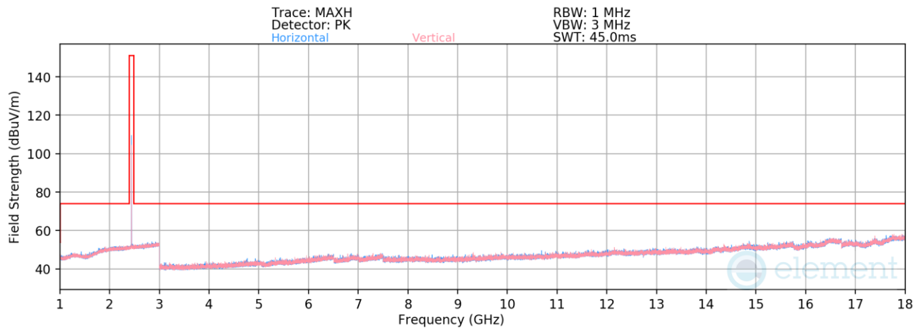
Plot 7-82. Radiated Spurious Emissions 1-18GHz Antenna 4a (4Mbps, HDR4, ePA – Ch. 38)
