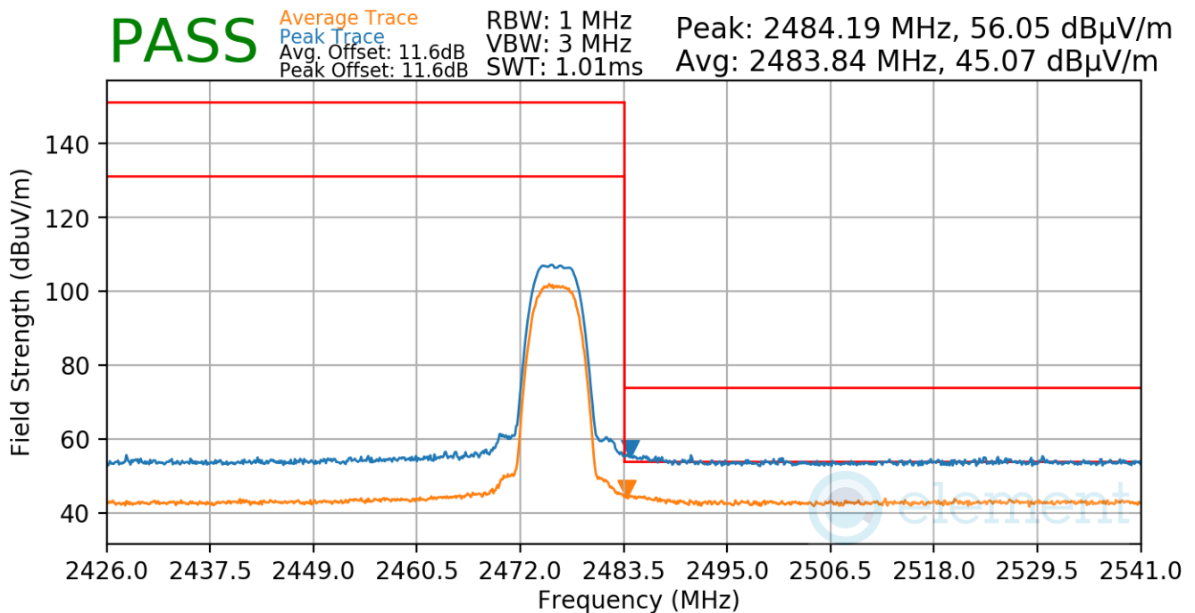
Plot 7-99. Radiated Restricted Upper Band Edge Measurement Antenna 2a
