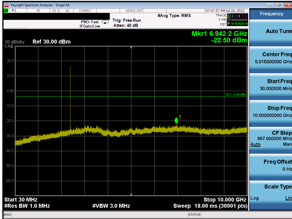
Plot 7-75. Conducted Spurious Plot Antenna 2a (Bluetooth (HDR4), 4 Mbps, ePA – Ch. 1)
