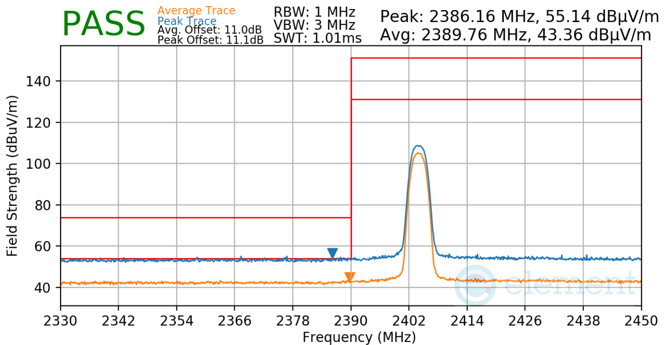
Plot 7-96. Radiated Restricted Lower Band Edge Measurement Antenna 2a
