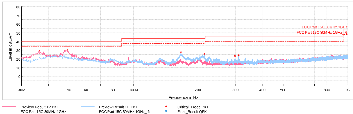
Plot 7-104. Radiated Spurious Emissions Below 1GHz TxBF (HDR4 ePA – Ch.38 with AC/DC Adapter)
