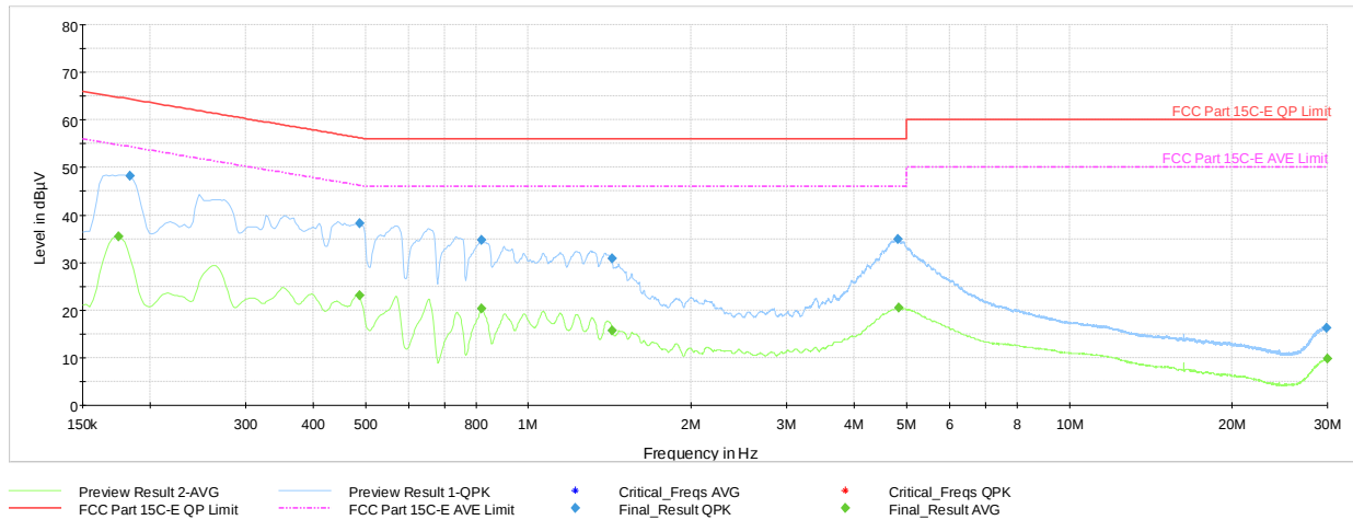
Plot 7-106. AC Line Conducted Plot with Bluetooth HDR Tx BF (N, 4Mbps ePA - Ch.38 with AC/DC Adapter)
