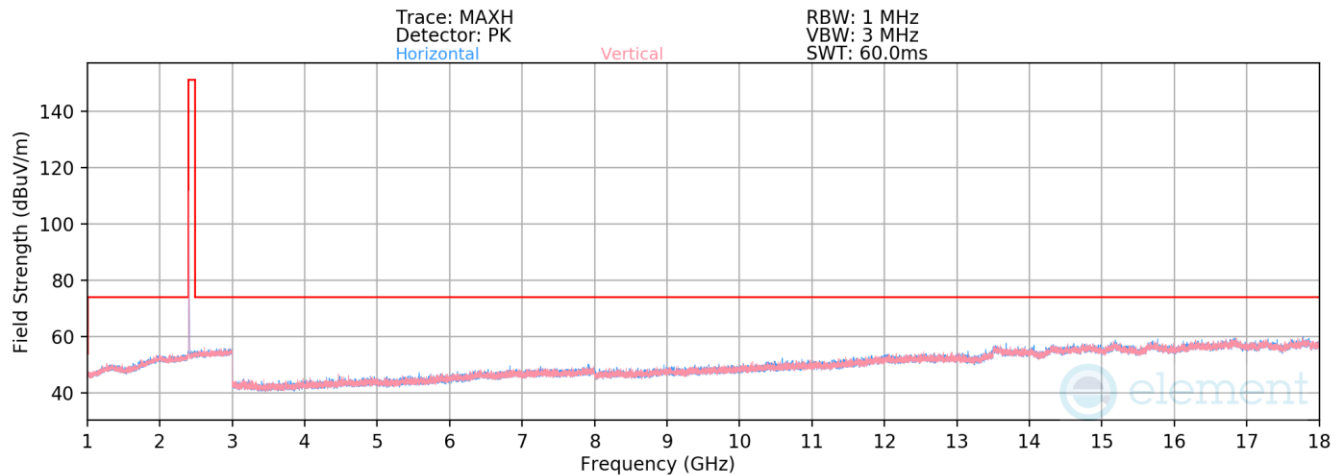
Plot 7-84. Radiated Spurious Emissions 1-18GHz Antenna 2a (4Mbps, HDR4, ePA – Ch. 1)
