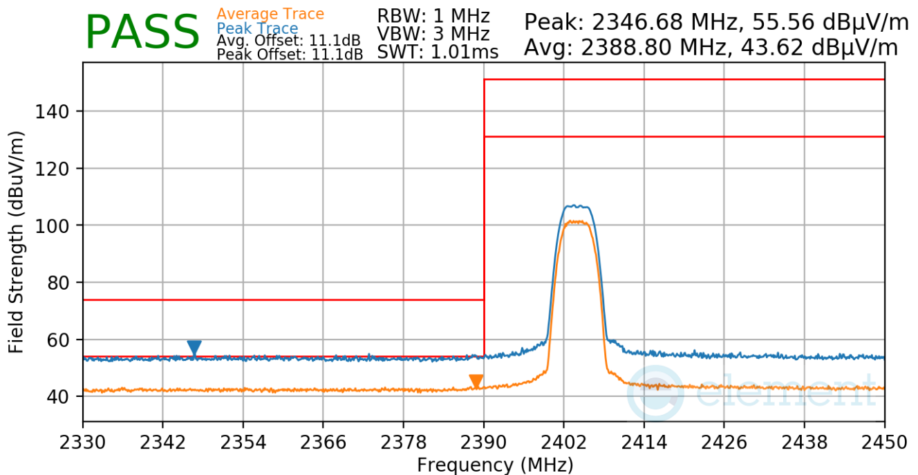
Plot 7-97. Radiated Restricted Lower Band Edge Measurement Antenna 2a
