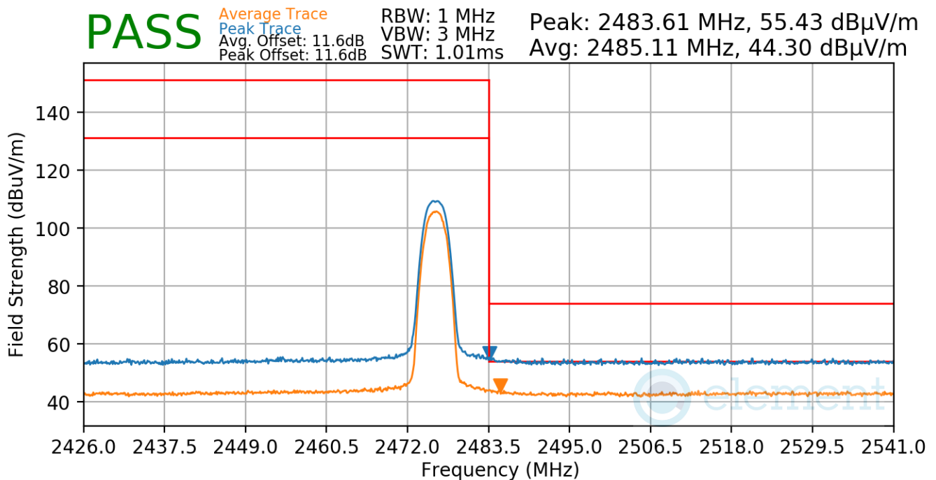
Plot 7-94. Radiated Restricted Upper Band Edge Measurement Antenna 4a
