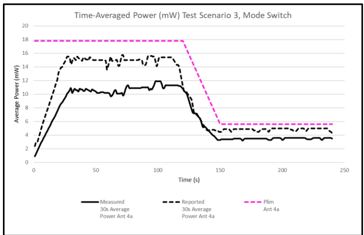
Figure J-8 30s Average Power vs. Time during Mode Switch
