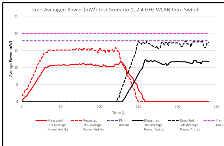
Figure J-2 30s Average Power vs. Time, 2.4 GHz
