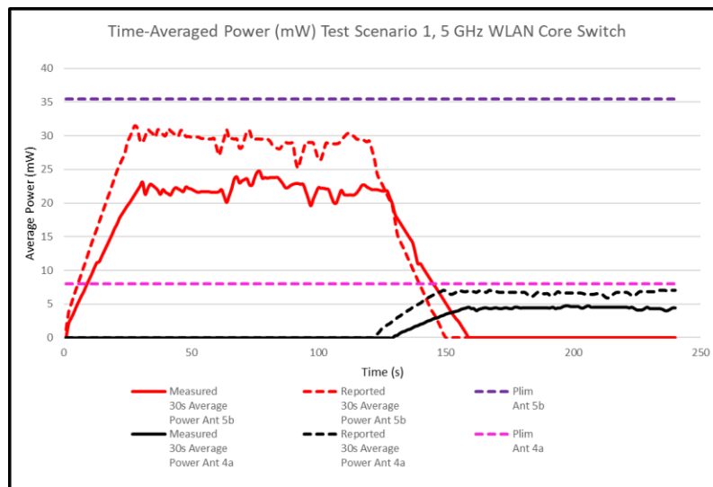
Figure J-4 30s Average Power vs. Time, 5 GHz
