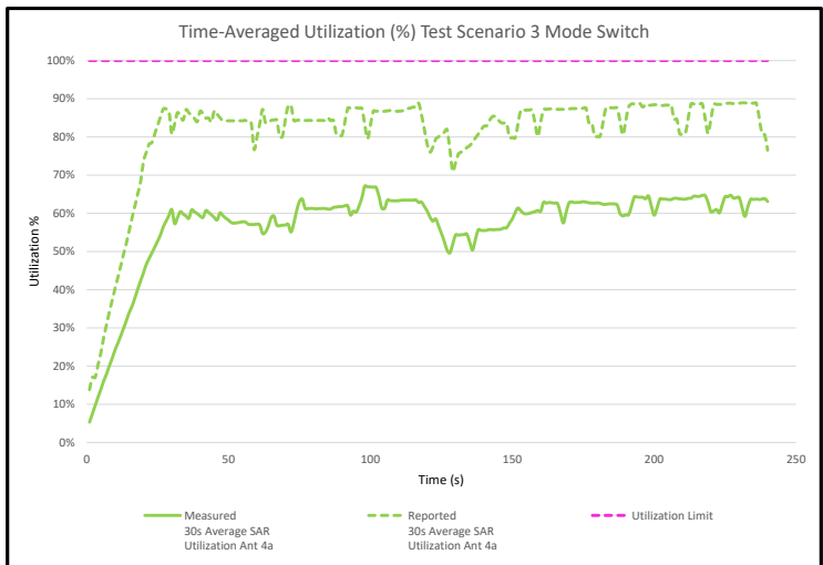
Figure J-7 30s Average Utilization vs. Time during Mode Switch
