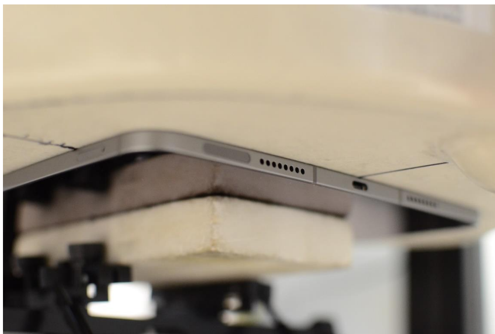
Test Setup Photo 10 – Body, Back Side at 0.0 cm – Antenna 1
