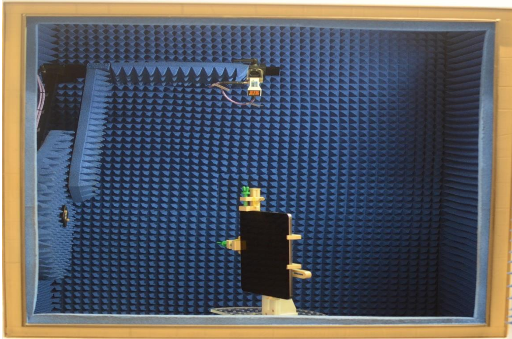
Test Setup Photo 7 – mmW NR Radiated Measurement Setup (Figure 7-1)
