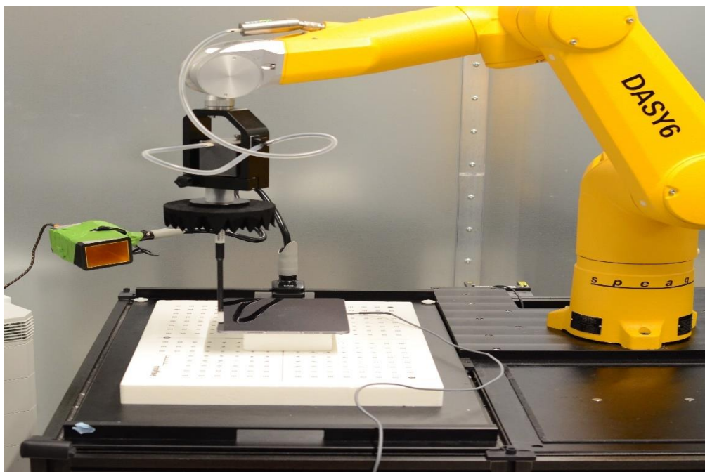
Test Setup Photo 9 – Power Density Measurement Setup, Front Surface (Figure 7-2)
