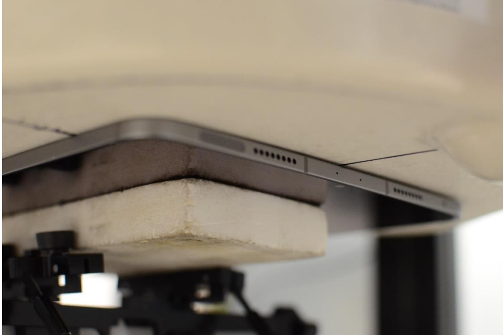
Test Setup Photo 11 – Body, Back Side at 0.0 cm – Antenna 4B
