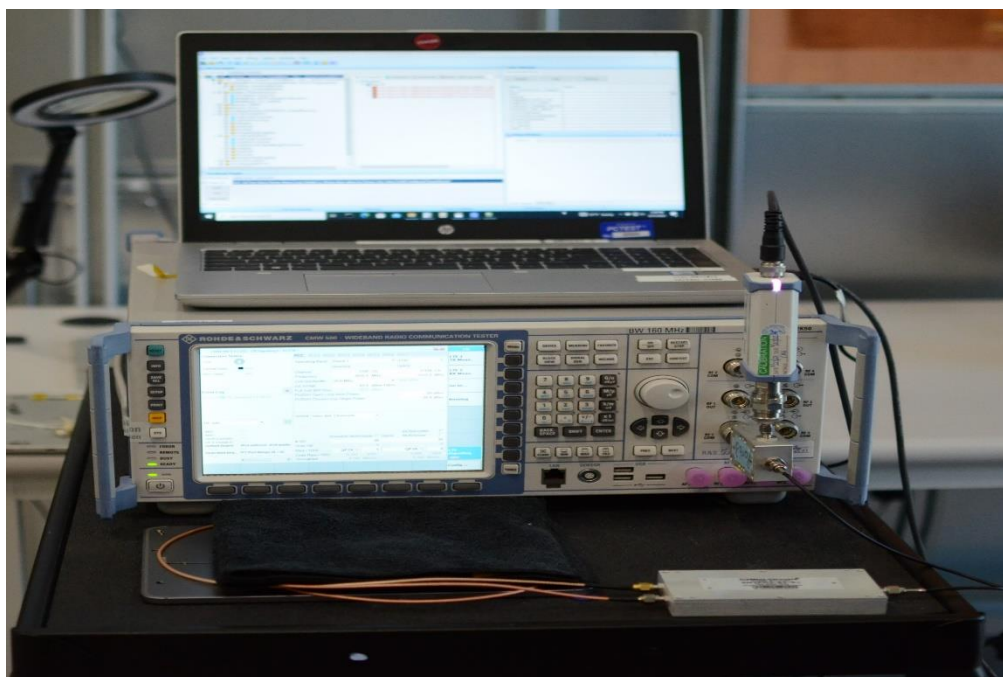
Test Setup Photo 4 – Conducted Test Setup (Figure 6-1b)
