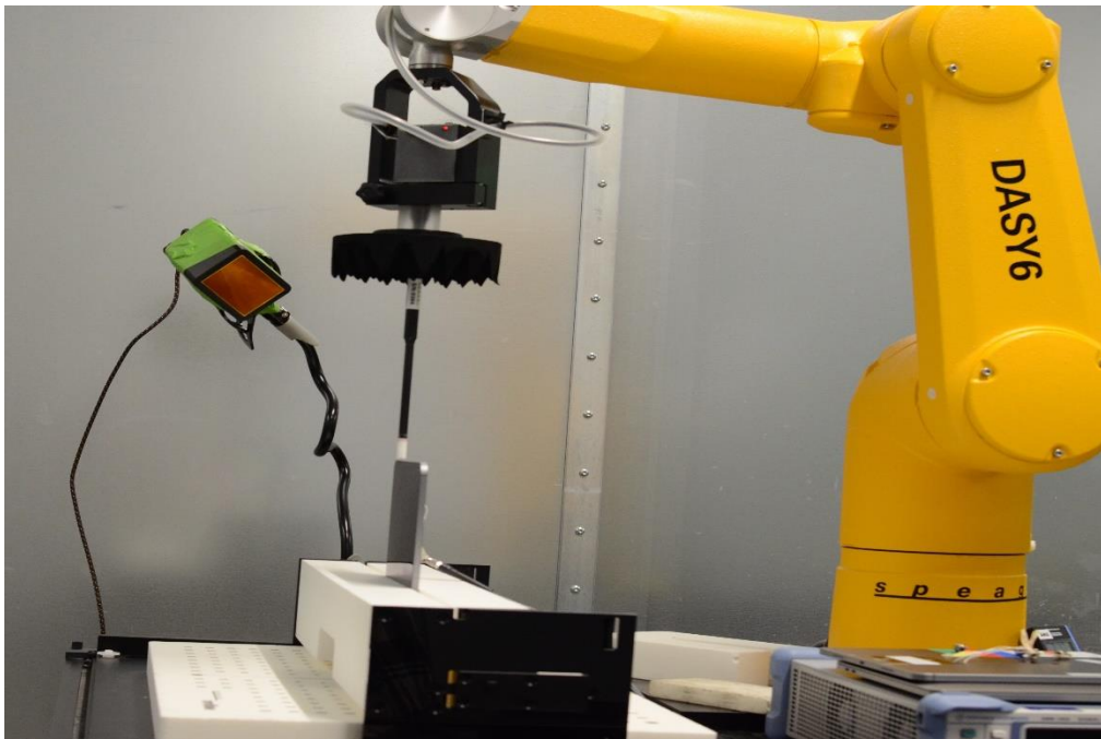
Test Setup Photo 8 – Power Density Measurement Setup, Bottom Edge (Figure 7-2)
