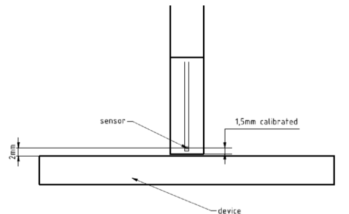
Figure D-2 EUmmWVx Probe
