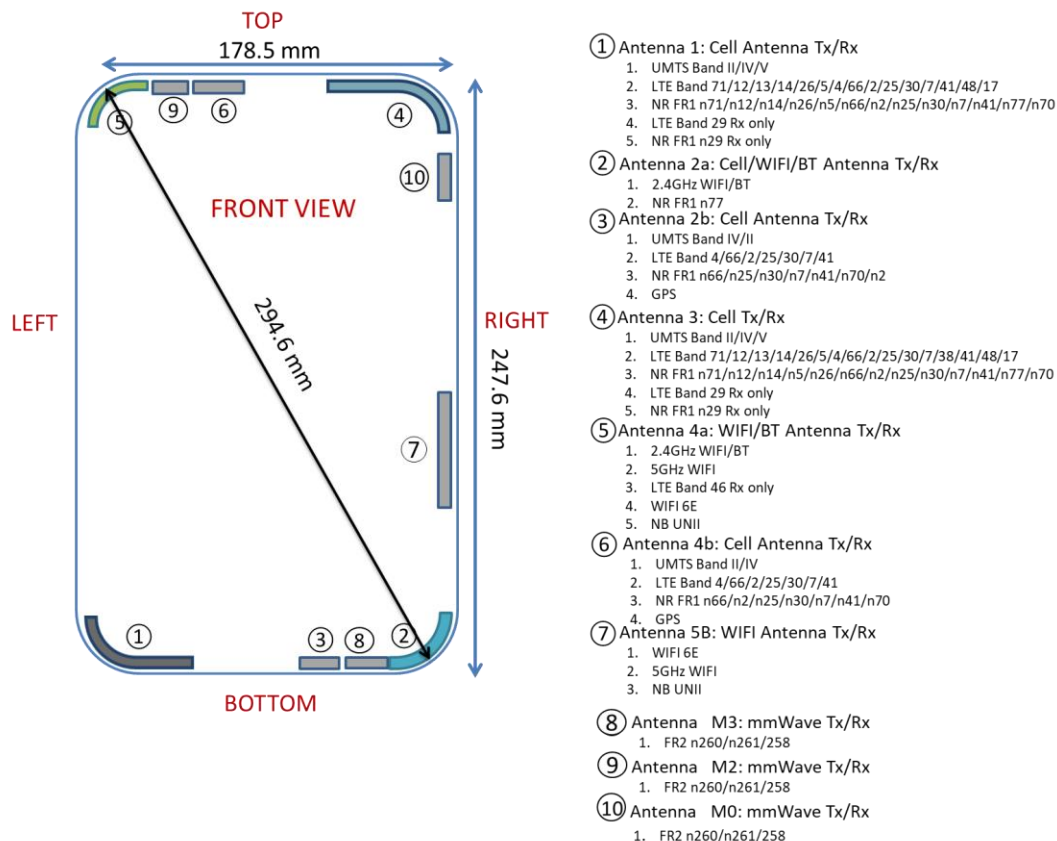
Figure D-1 DUT Antenna Locations
