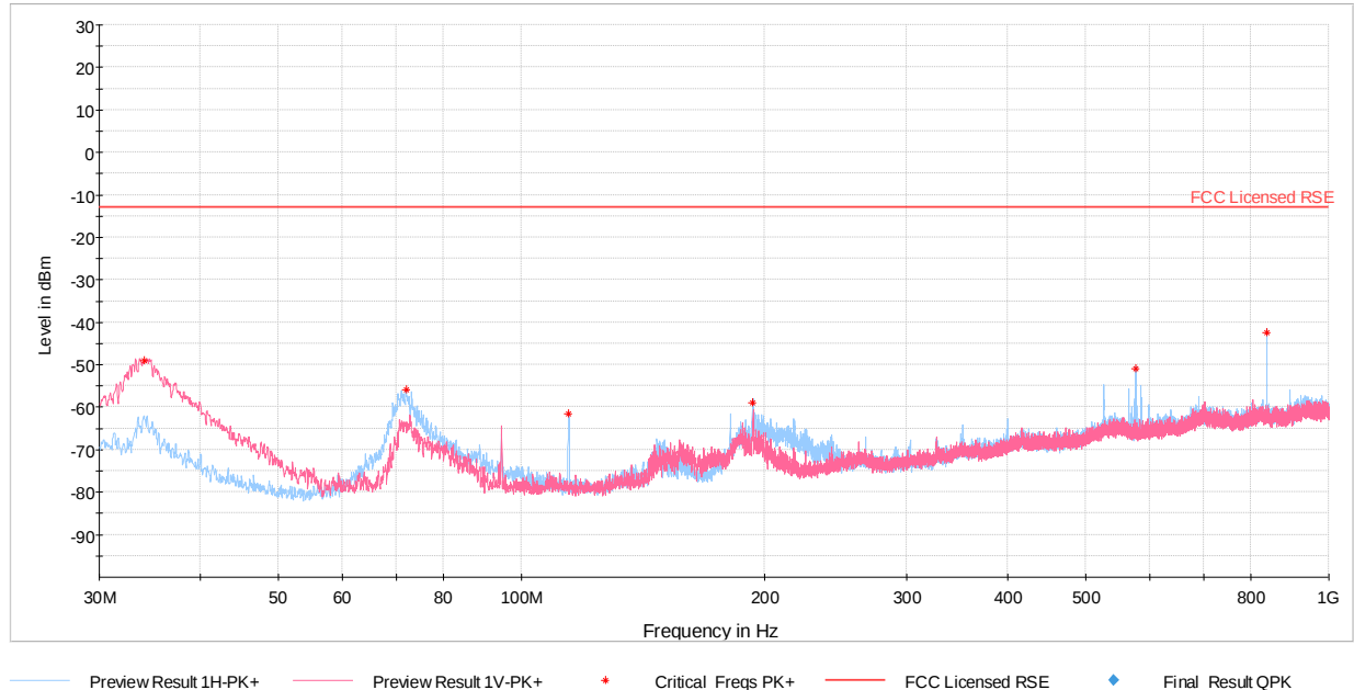
Plot 7-591. Ant M2 - RSE Plot (Band n260 -100MHz-1CC SISO Dual Pol – QPSK – Mid Channel)
