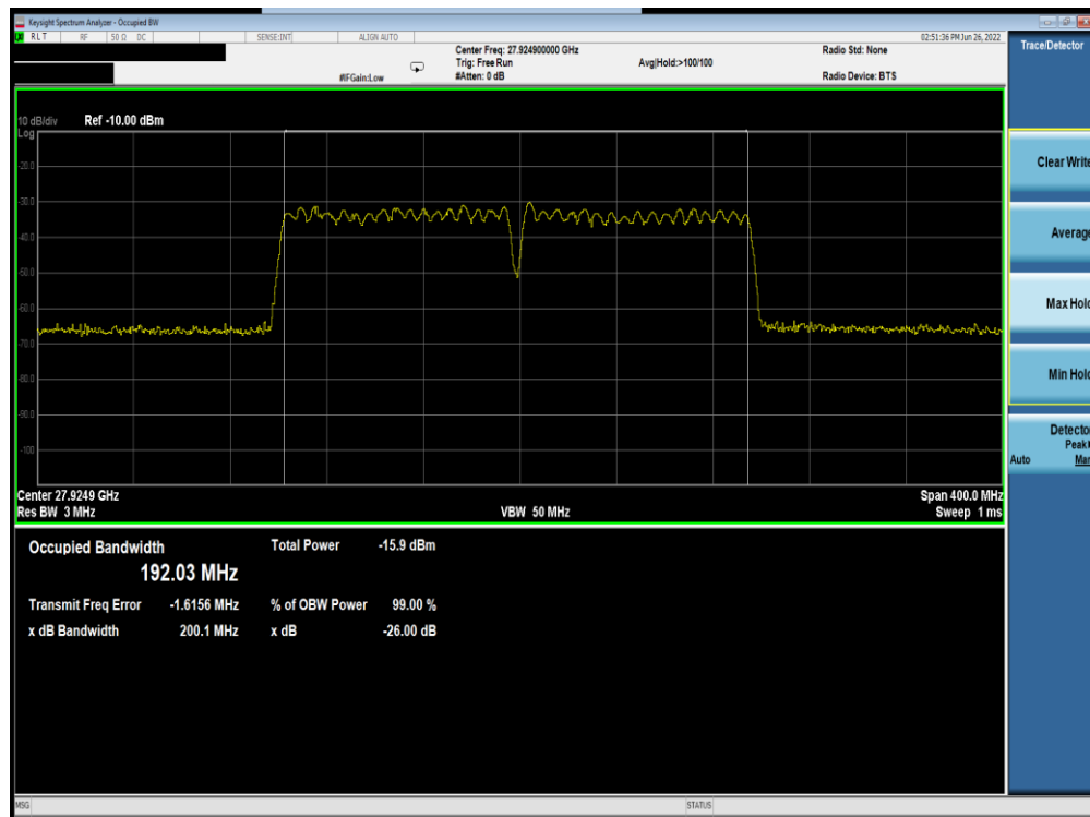
Plot 7-278. Ant M0 OBW (Band n261-100MHz-2CC SISO Dual Pol DFTs-OFDM – QPSK – Mid Channel)
