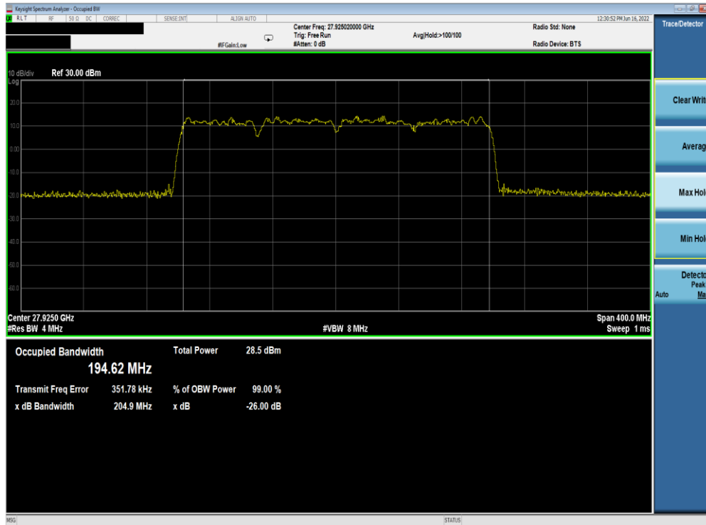
Plot 7-251. Ant M0 OBW (Band n261-50MHz-4CC SISO Dual Pol DFTs-OFDM – 16QAM – Mid Channel)
