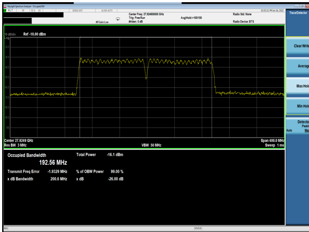
Plot 7-279. Ant M0 OBW (Band n261-100MHz-2CC SISO Dual Pol DFTs-OFDM – 16QAM – Mid Channel)
