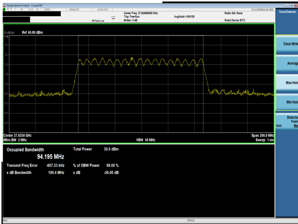
Plot 7-262. Ant M0 OBW (Band n261-100MHz-1CC MIMO CP-OFDM – 64QAM – Mid Channel)
