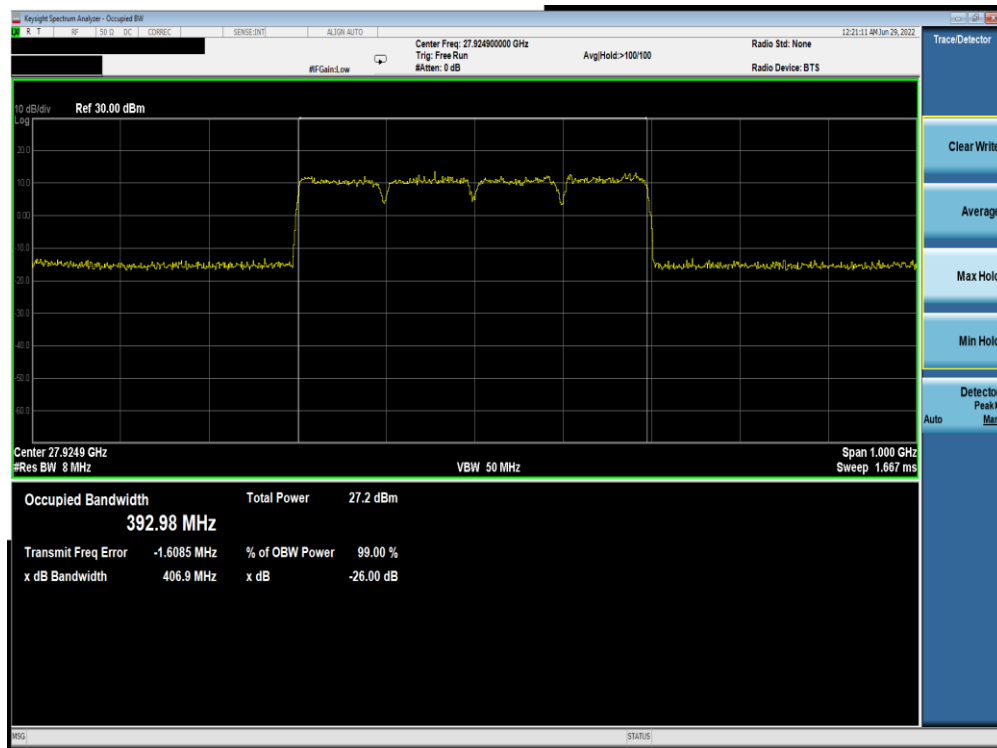
Plot 7-301. Ant M0 OBW (Band n261-100MHz-4CC SISO DFTs-OFDM – 64QAM – Mid Channel)
