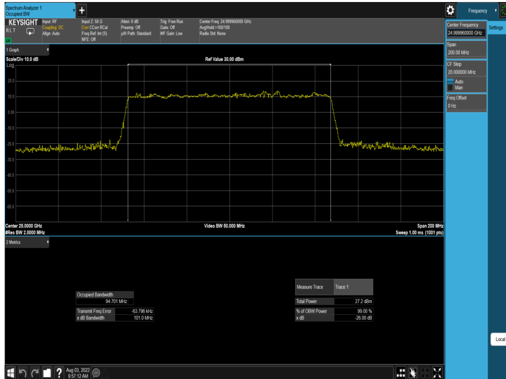
Plot 7-143. Ant M0 OBW (Band n258-R2-100MHz-1CC SISO CP-OFDM – 64QAM – Mid Channel)
