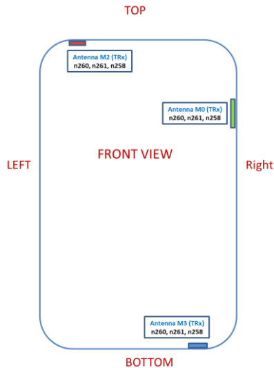
Figure 3-1 Location of mmW antenna modules
