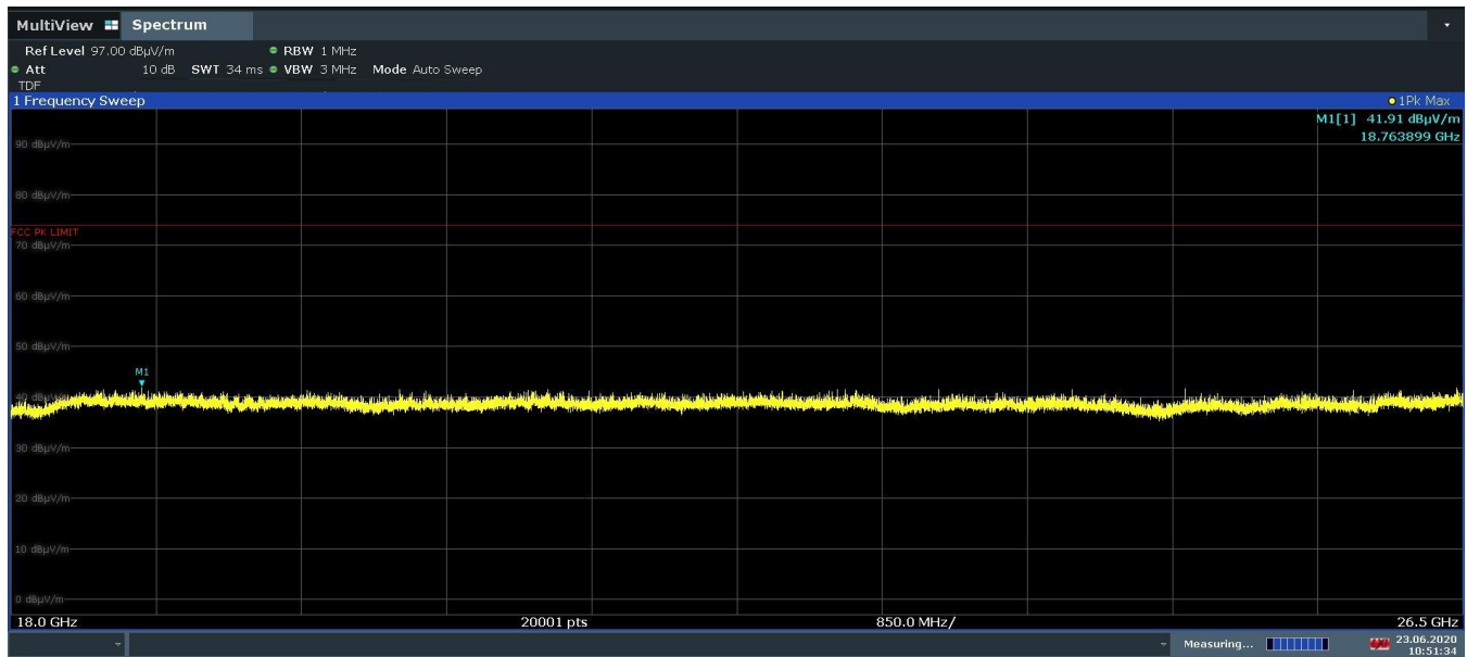
Plot 7-25. Radiated Spurious Emissions Above 18GHz (1Mbps – Ch.19, ePA, Ant. Pol. V)
