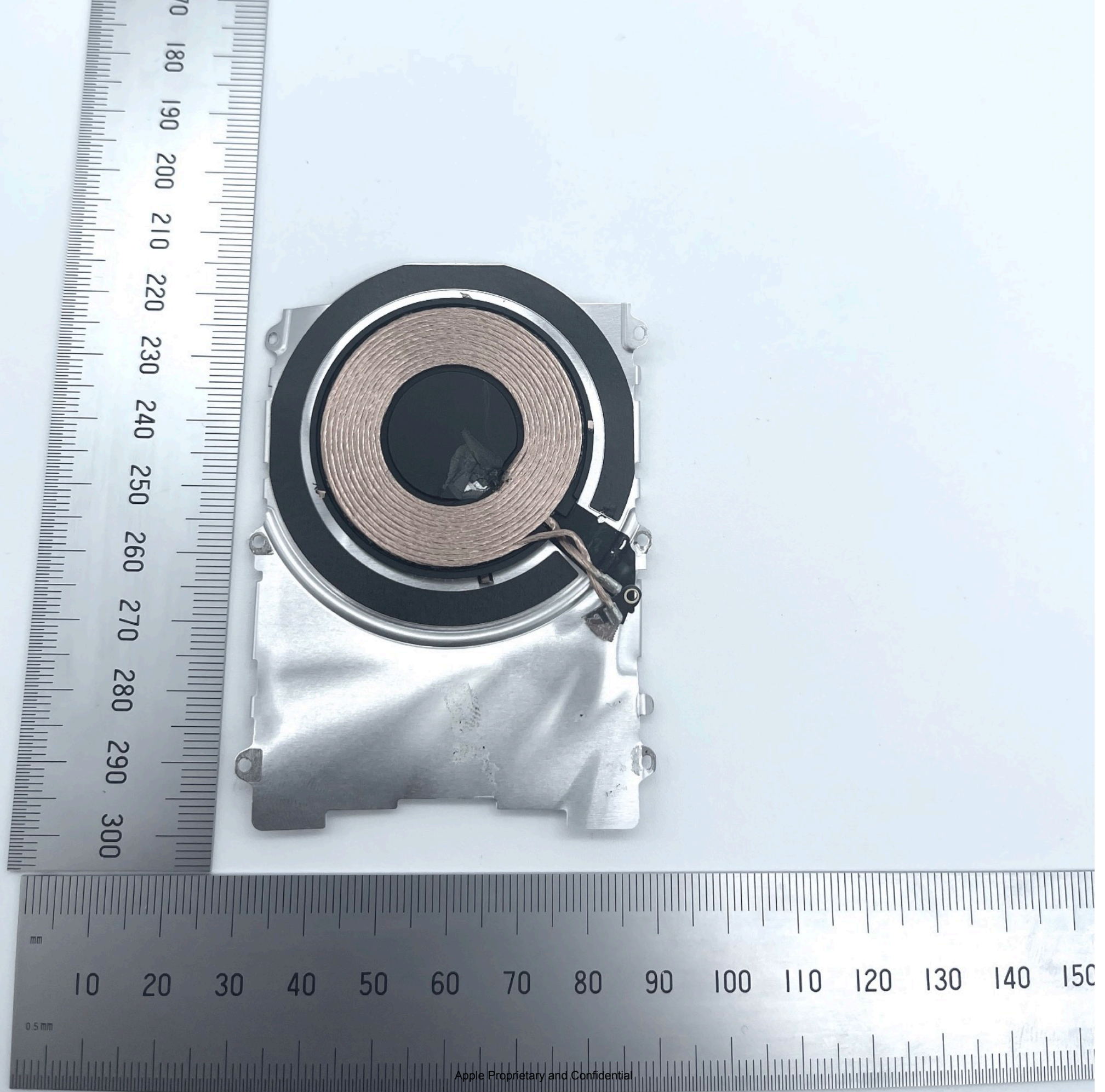
A2384 Charging Coil
